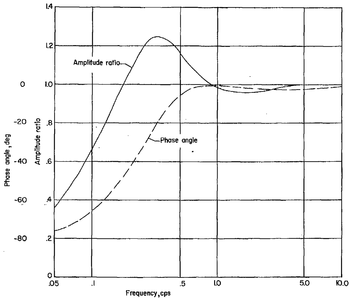
Figure 4.- Frequency-response function which describes the performance of vane-airplane combination as gust-measuring instrument, \left[ \frac{\alpha_v}{\alpha_g} \right] . V = 220 feet per second.
