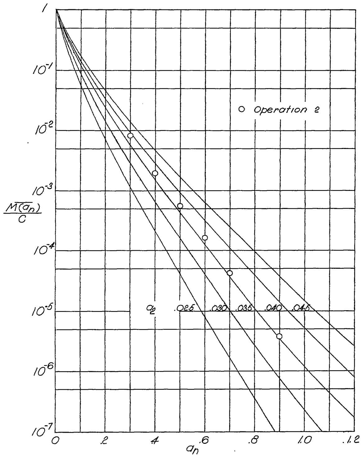
Figure 3.- Number of peak accelerations exceeding given values for case b.
