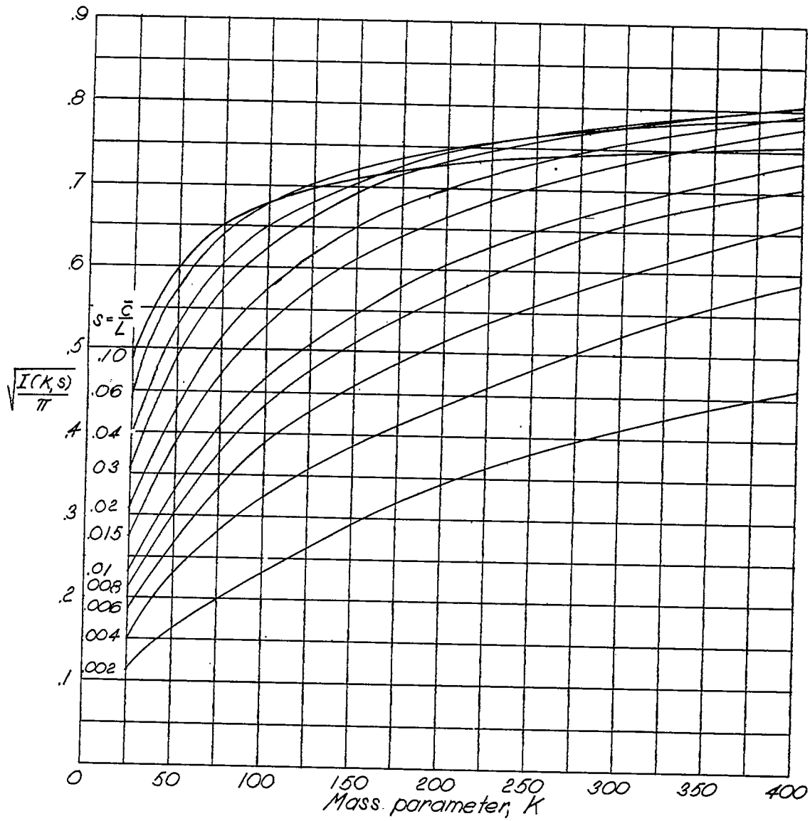
Figure 5.- Gust response factor \sqrt{\frac{I(K,s)}{\pi}} .
