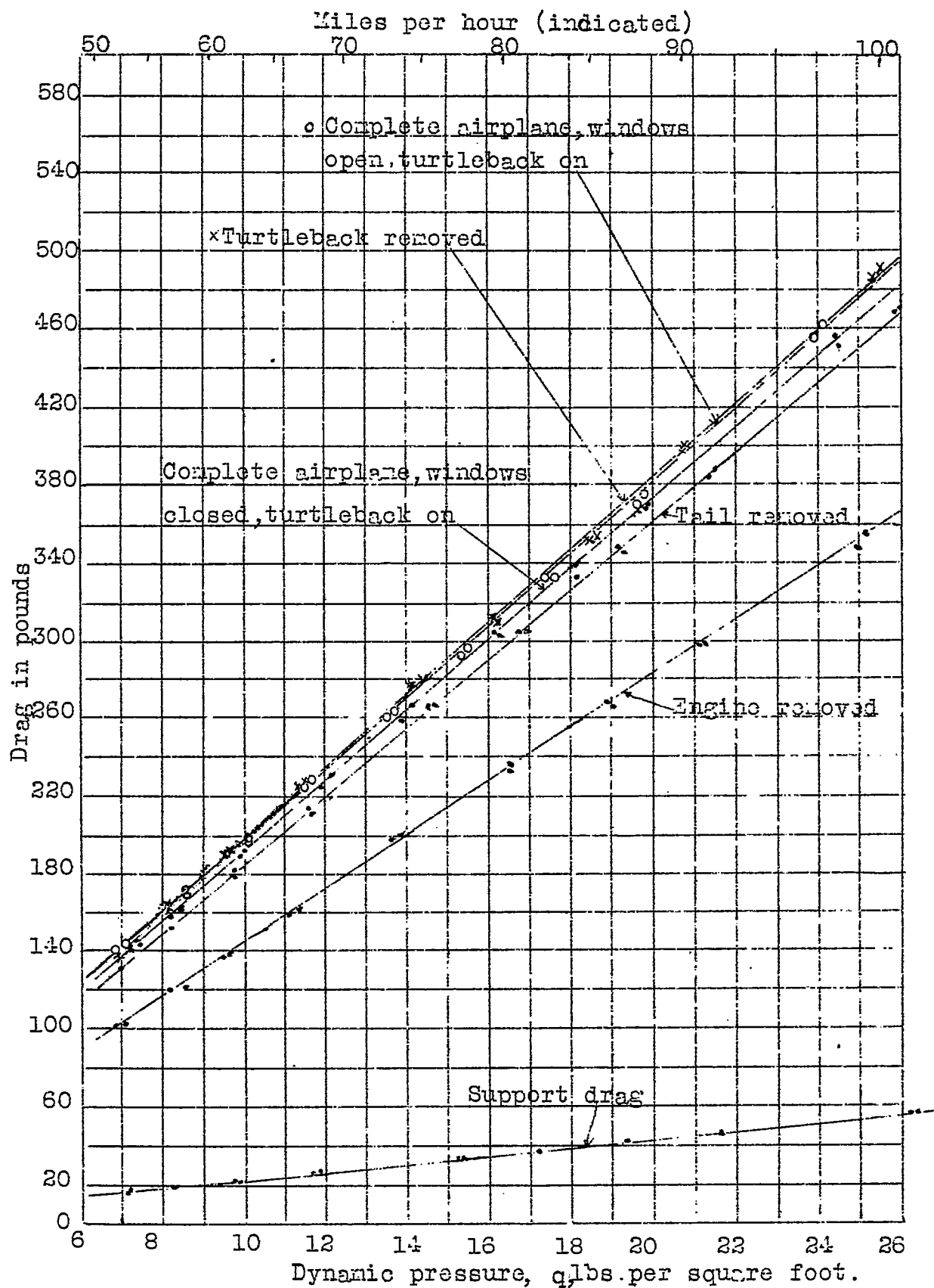
Fig. 12 Fairchild airplane with wing.
