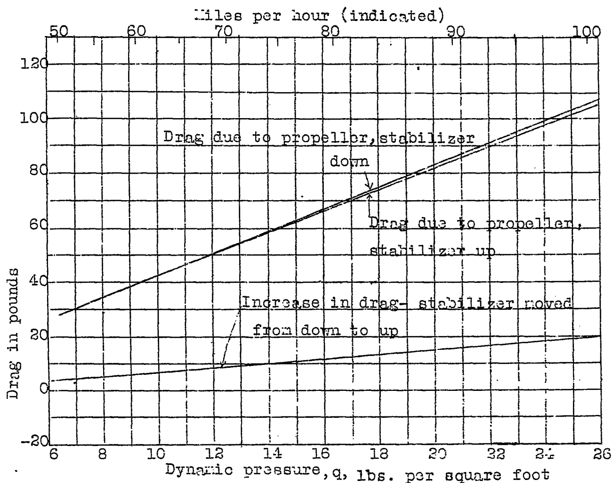
Fig. 17 Fairchild airplane with wing. Drag of component parts.
