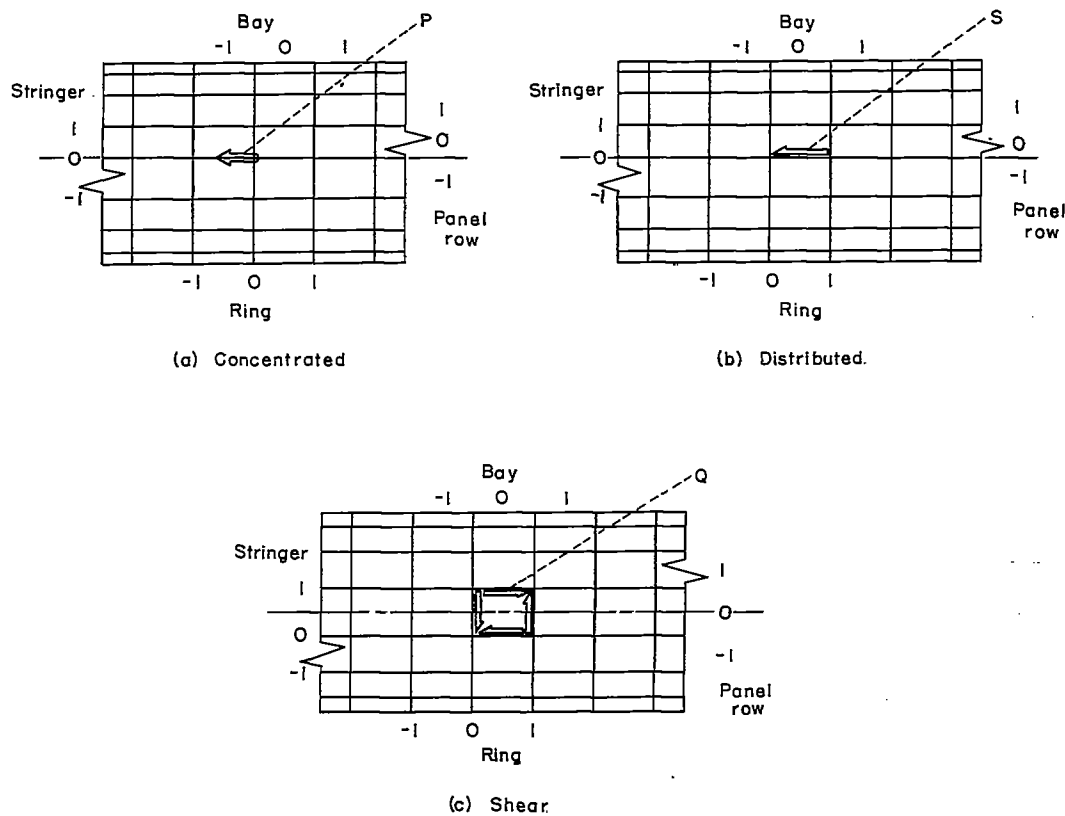
Figure 2.- Perturbation loads
