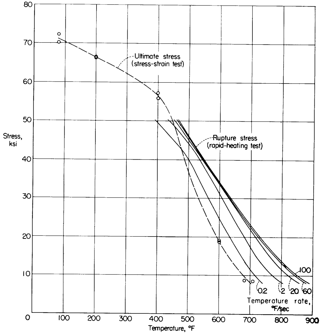
Figure 19.- Tensile rupture stress of 2024-T3 aluminum alloy for temperature rates from 0.2° F to 100° F per second and ultimate tensile stress of stress-strain tests for 1/2-hour exposure.
