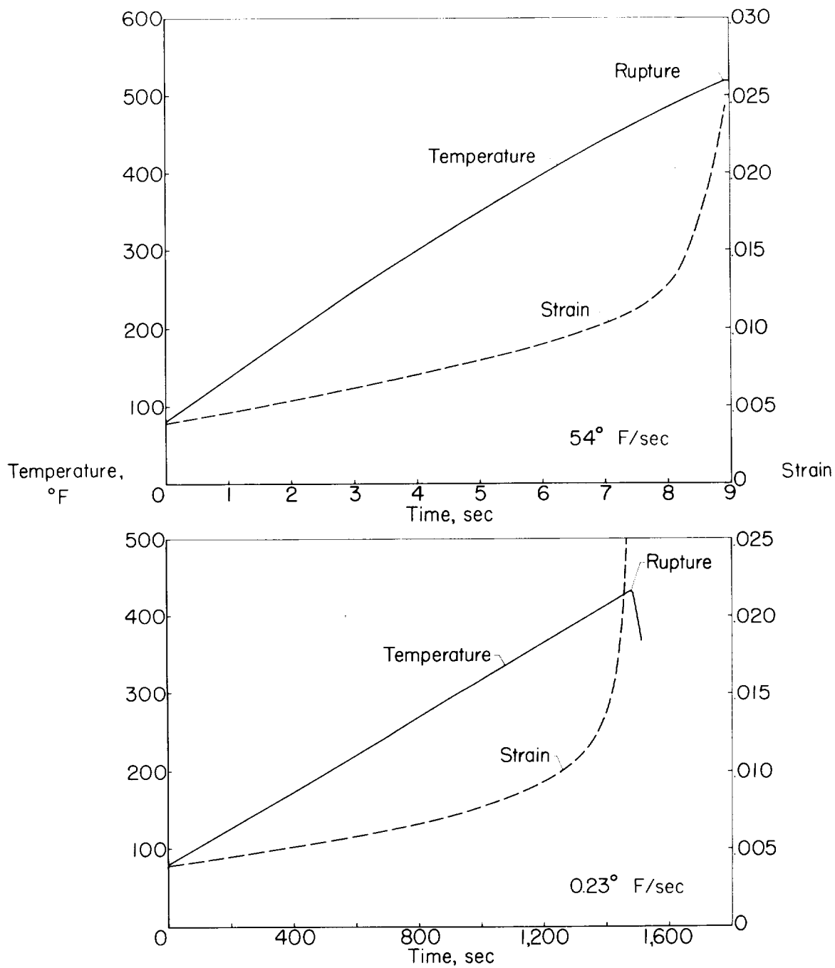
Figure 7.- Temperature- and strain-time curves for tests of 7075-T6 aluminum alloy at 54° F and 0.23° F per second at 40 ksi.
