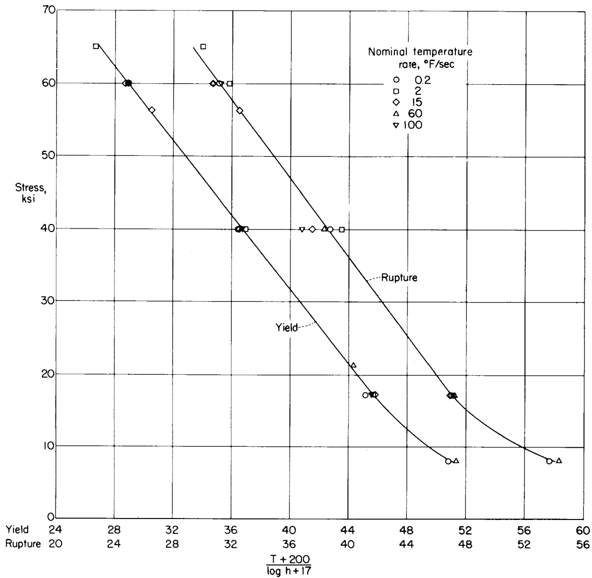
Figure 23.- Master yield- and rupture-stress curves for 7075-T6 aluminum alloy based on linear temperature parameter. (T is in °F and h is in °F per second.)
