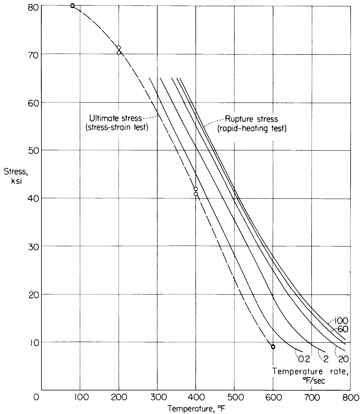
Figure 18.- Tensile rupture stress of 7075-T6 aluminum alloy for temperature rates from 0.2° F to 100° F per second and ultimate tensile stress of stress-strain tests for 1/2-hour exposure.
