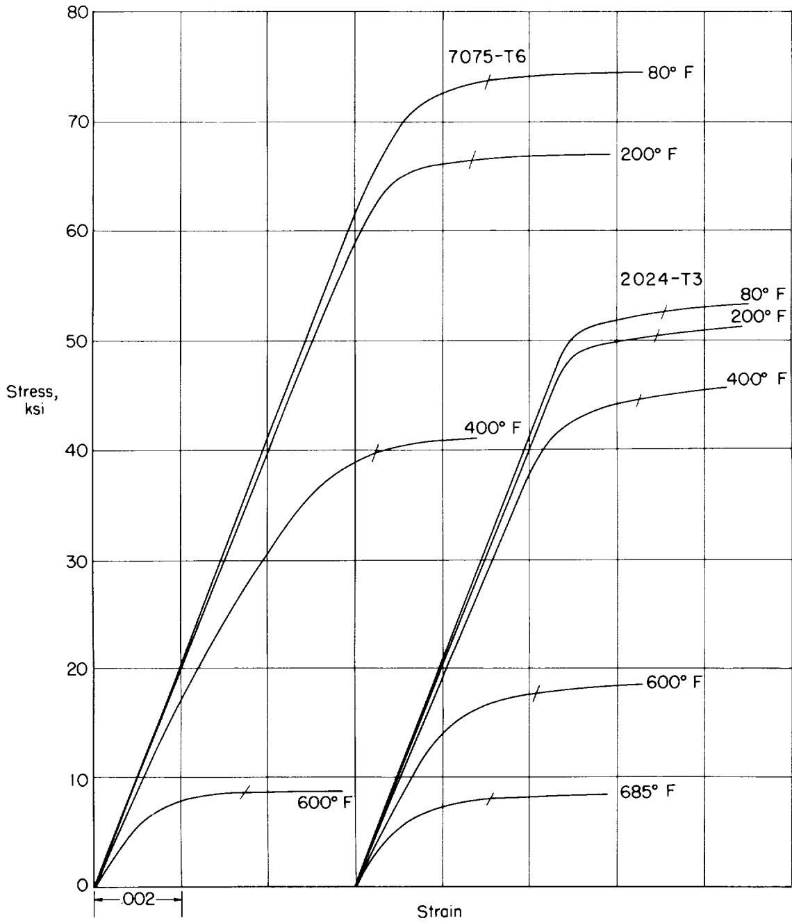
Figure 9.- Elevated-temperature tensile stress-strain curves for 7075-T6 and 2024-T3 aluminum-alloy sheet.
