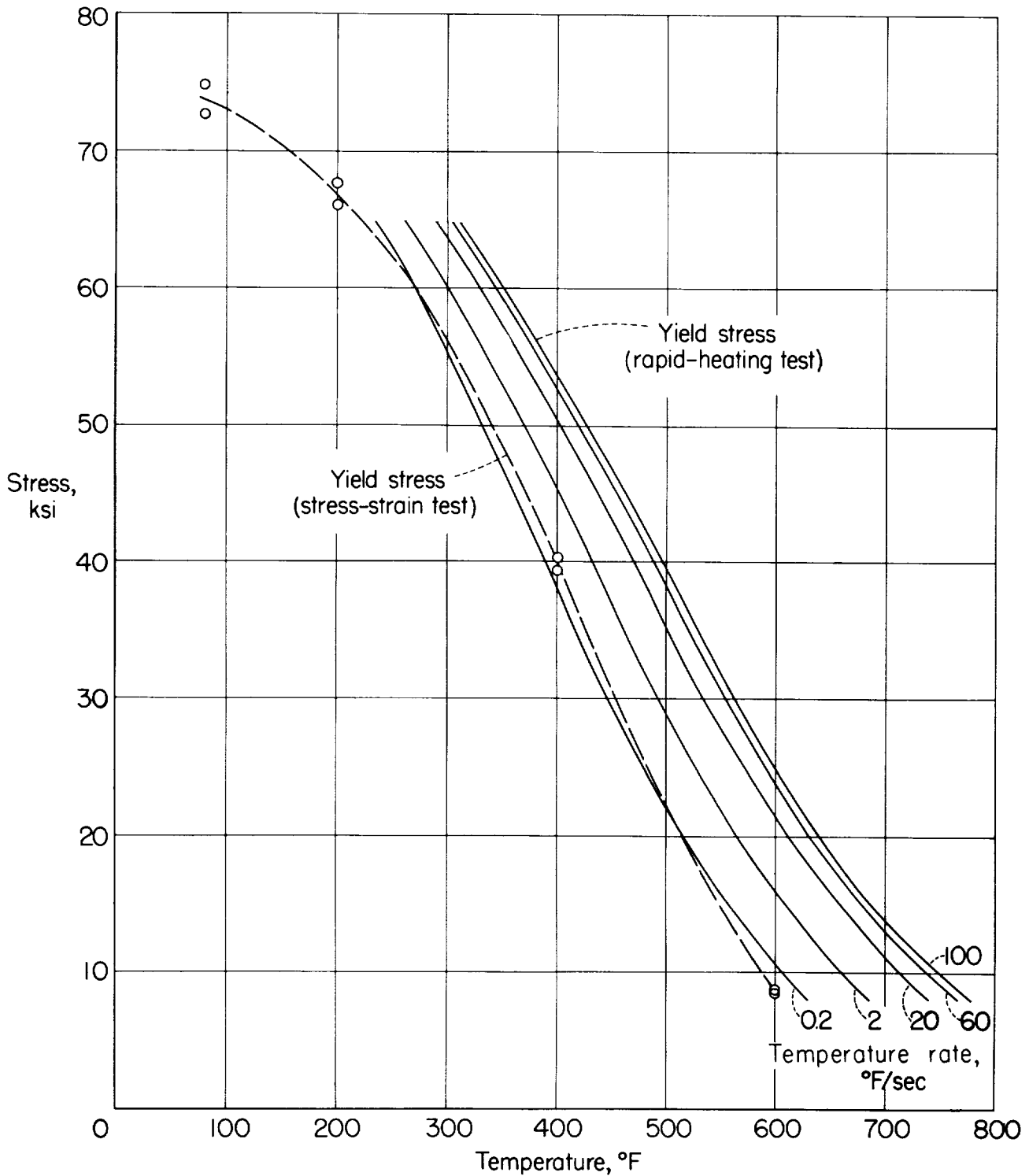
Figure 14.- Tensile yield stress of 7075-T6 aluminum alloy for temperature rates from 0.2° F to 100° F per second and of stress-strain tests for 1/2-hour exposure.
