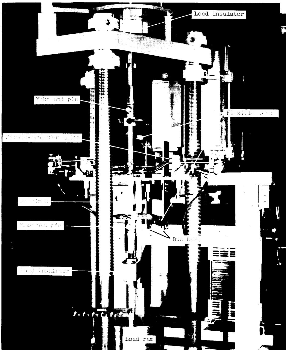
Figure 3.- View of specimen mounted in position for testing.
