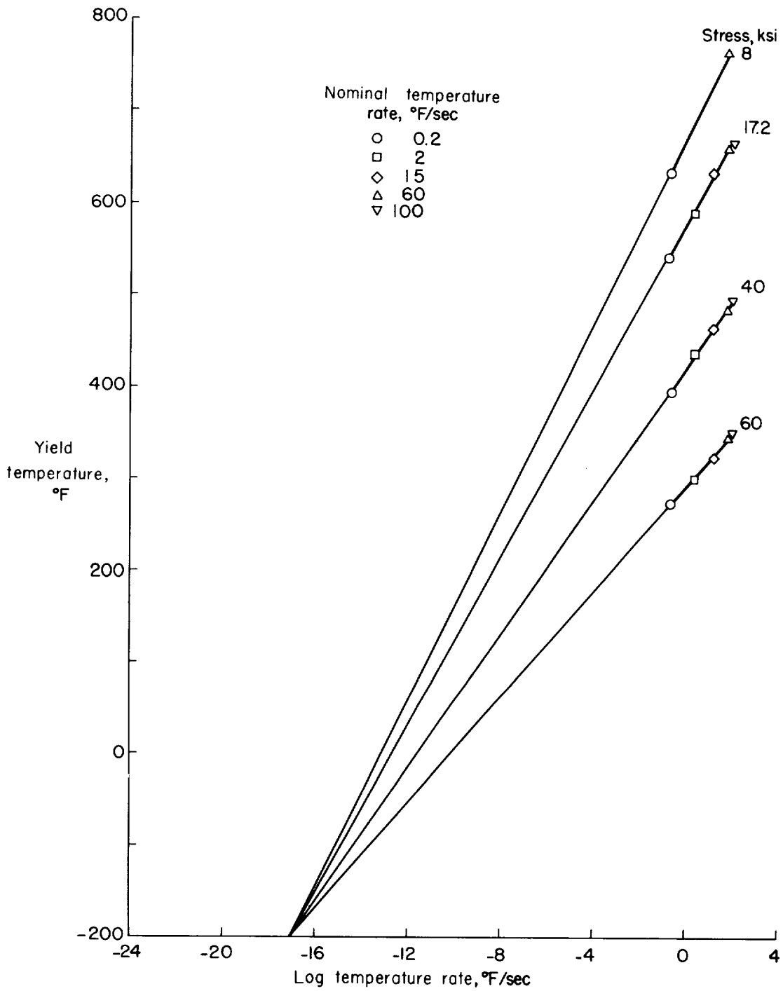
Figure 21.- Variation of yield temperature with logarithm of temperature rate of 7075-T6 aluminum alloy for various stresses.
