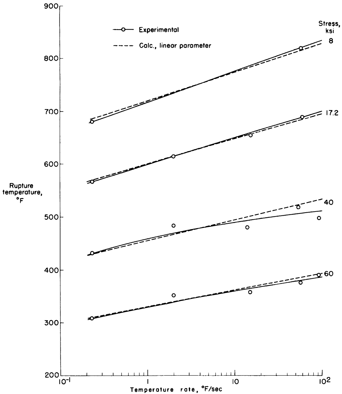
Figure 16.- Experimental and calculated rupture temperatures of 7075-T6 aluminum alloy for temperature rates from 0.2° F to 100° F per second for various stresses.
