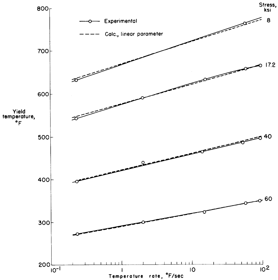
Figure 12.- Experimental and calculated yield temperatures of 7075-T6 aluminum alloy for temperature rates from 0.2° F to 100° F per second for various stresses.
