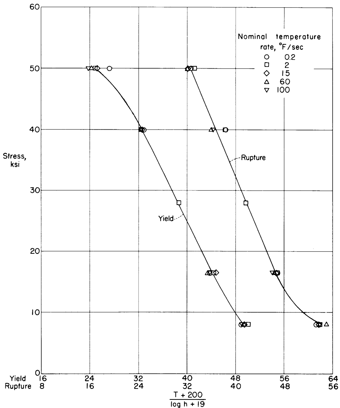
Figure 24.- Master yield- and rupture-stress curves for 2024-T3 aluminum alloy based on linear temperature parameter. (T is in °F and h is in °F per second.)
