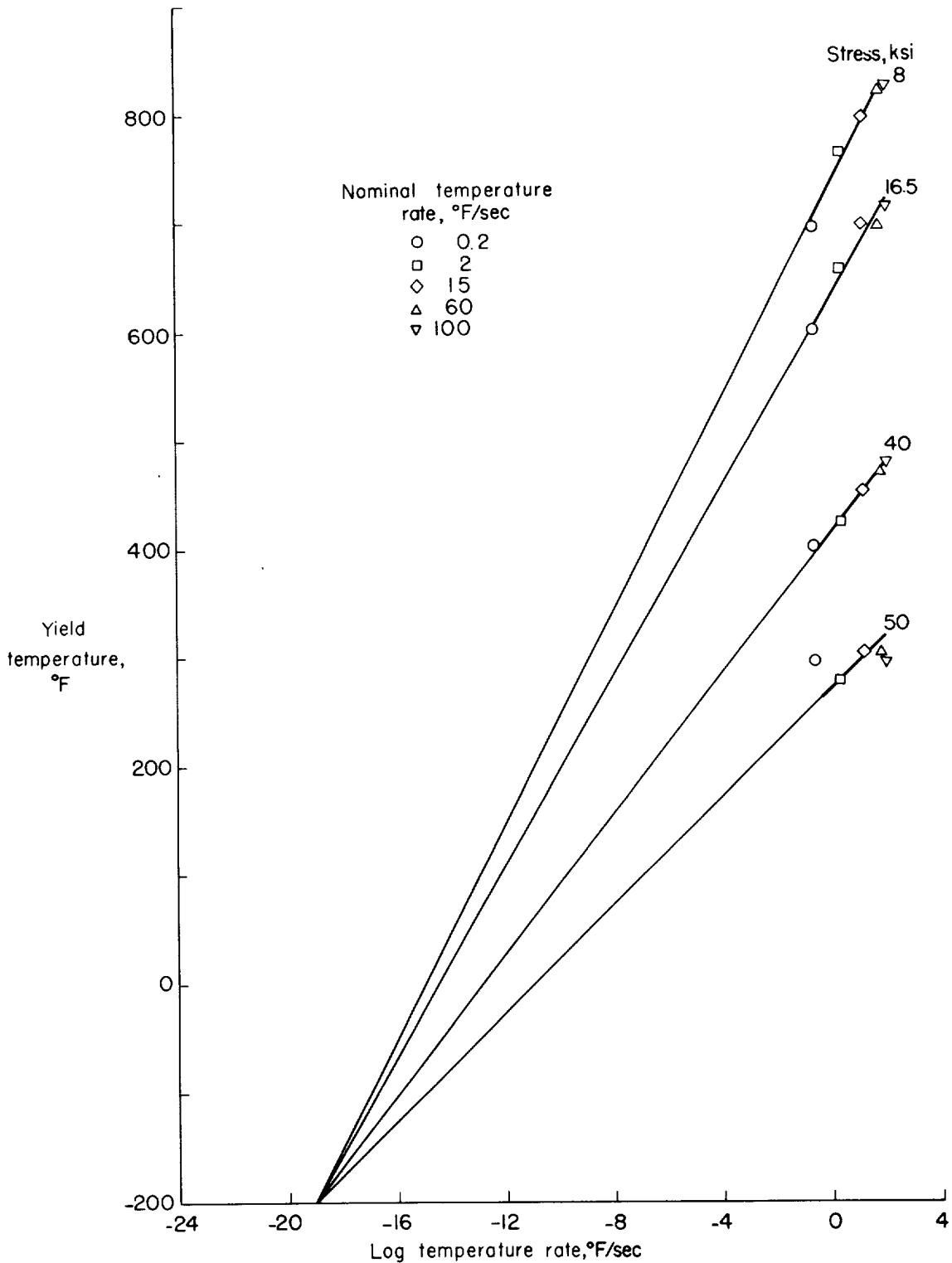
Figure 22.- Variation of yield temperature with logarithm of temperature rate of 2024-T3 aluminum alloy for various stresses.
