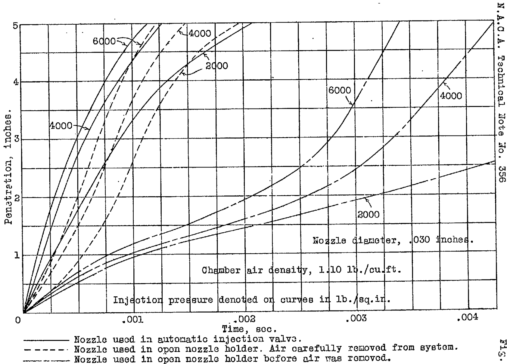
Fig. 12 Spray penetrations with open and closed nozzle.
