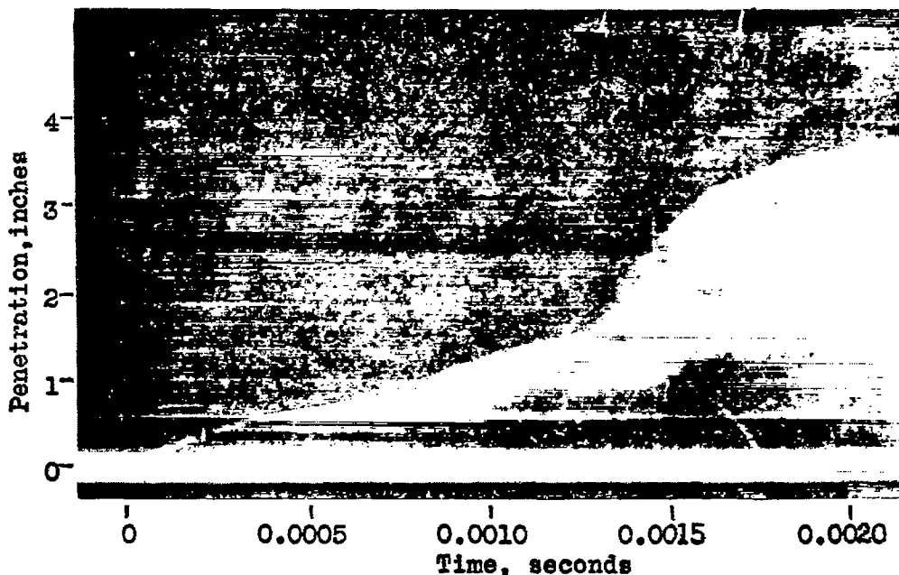
Fig.11 Spray penetration photograph made with an open nozzle and with a ball check-valve 2.5" from nozzle. Nozzle diameter . . . . . 0.020 in. Injection pressure. . . . . 4000 lb./sq.in. Chamber air density . . . . . 1.10 lb./cu.ft.
