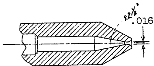
c-Tapered orifice.
