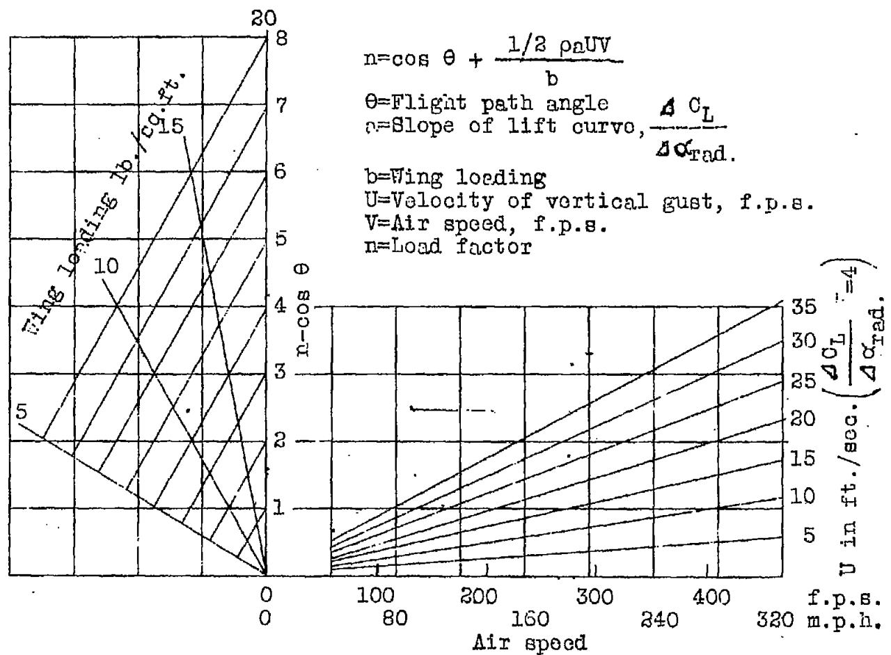
Fig. 4 Applied load factors in bumpy air. Biplane
