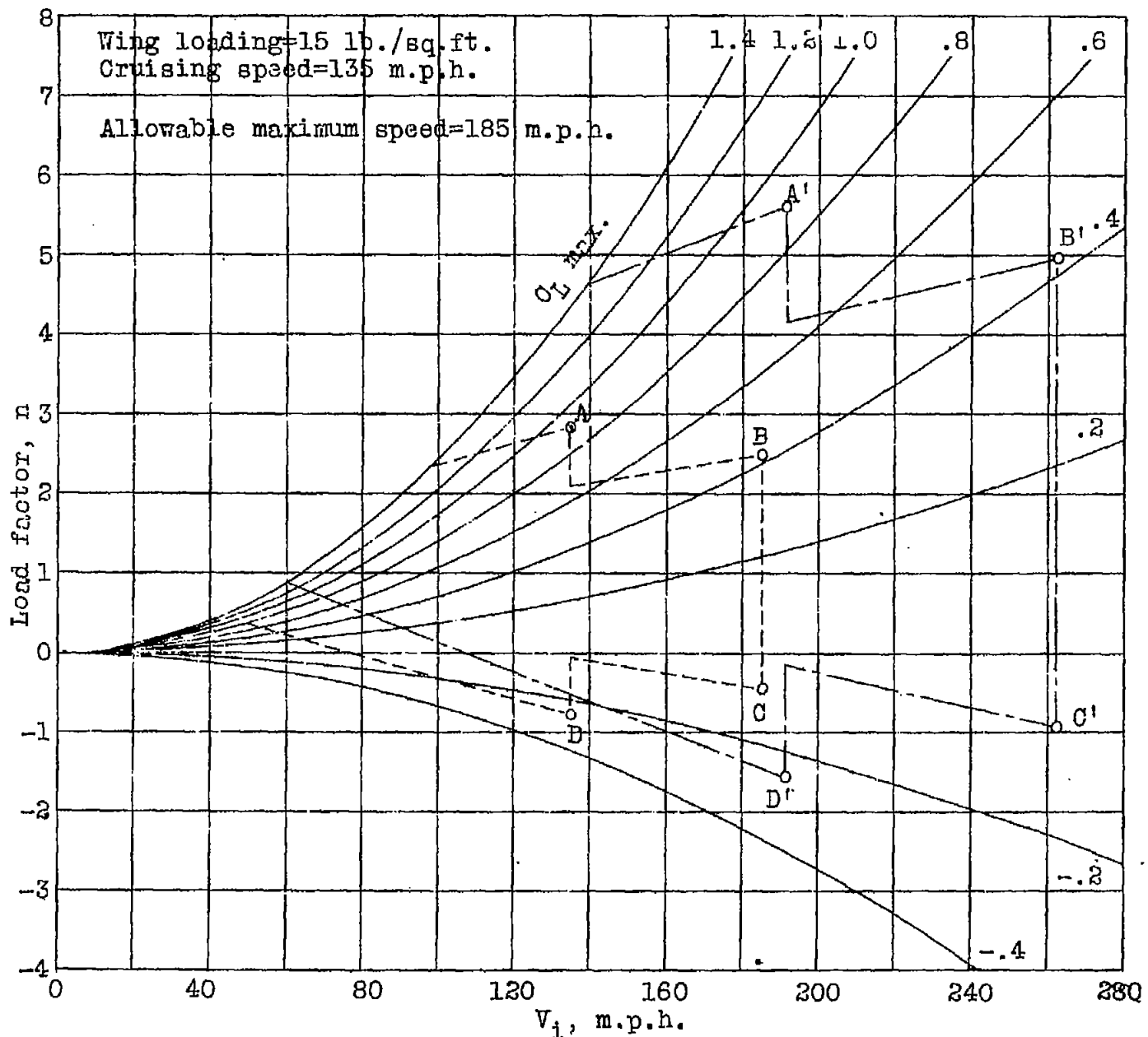
Fig. 6 Load factor chart for a transport airplane.
