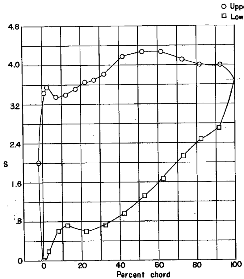
(a) M_1 = .235 ; M_2 = .468 ; C_{w1} = .0198 ; \theta = 90.6^\circ
