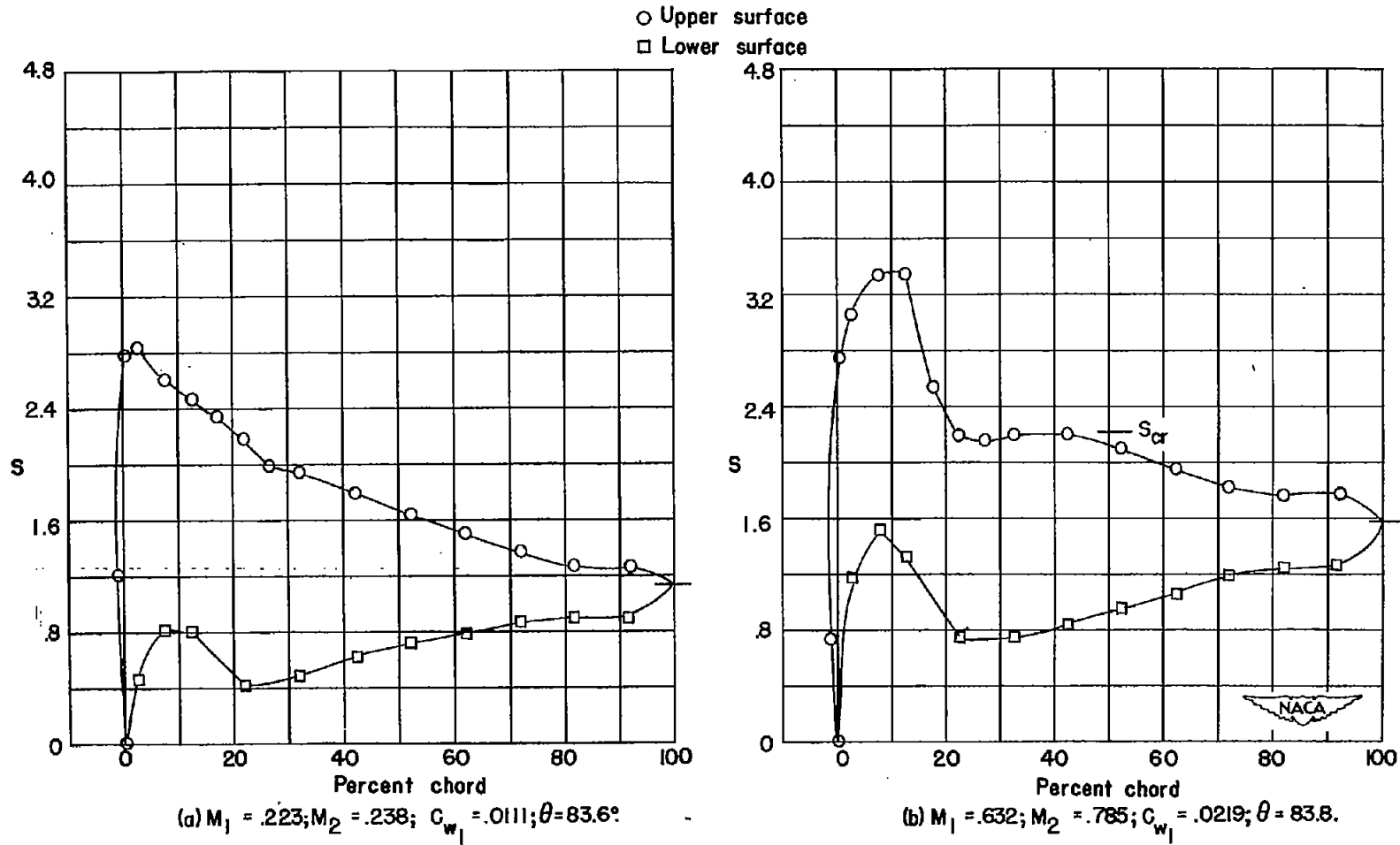
Figure 46.- High-speed pressure distributions for cascade combinations \beta_1 = 40^\circ , \alpha_1 = 56.1^\circ , \sigma = 1.8 , and primary turbine blade section, \theta_c = 95^\circ .
