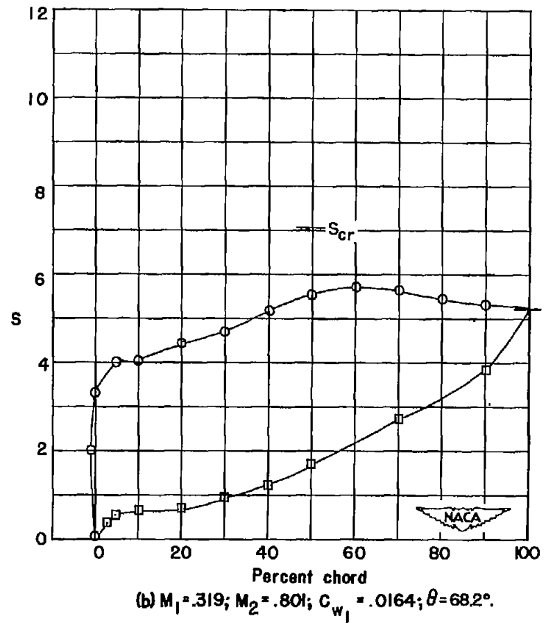
Figure 31.- High-speed pressure distributions for cascade combinations \beta_1 = 10^\circ , \alpha_1 = 48.4^\circ , \sigma = 1.8 , and primary turbine blade section, \theta_c = 80^\circ .
