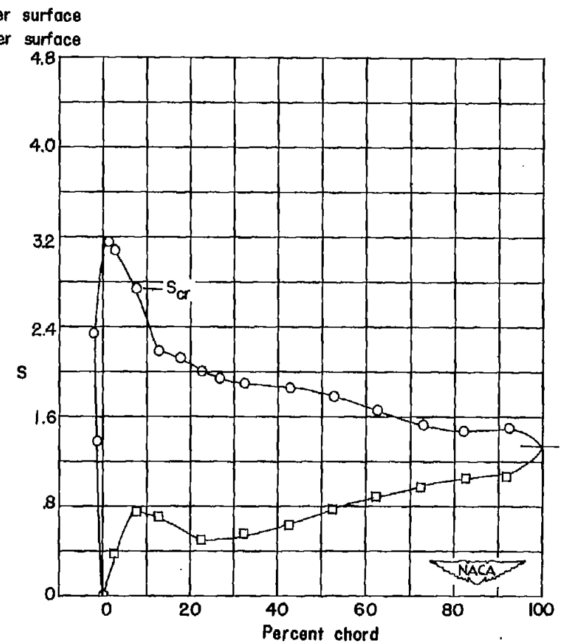
(b) M_1 = .549 ; M_2 = .629 ; C_{w1} = .0193 ; \theta = 91.0^\circ .
