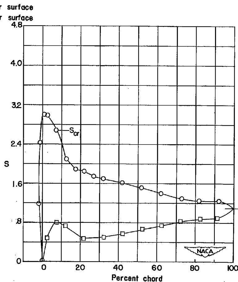
(b) M_1 = .556 ; M_2 = .565 ; C_{w_1} = .0155 ; \theta = 87.5^\circ .
