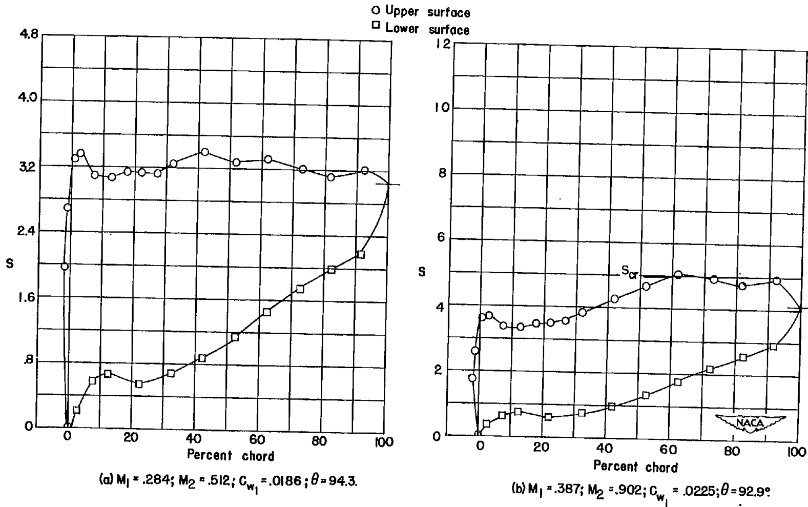
Figure 45.- High-speed pressure distributions for cascade combinations \beta_1 = 35^\circ , \alpha_1 = 66.1^\circ , \sigma = 1.8 , and primary turbine blade section, \theta_c = 95^\circ .
