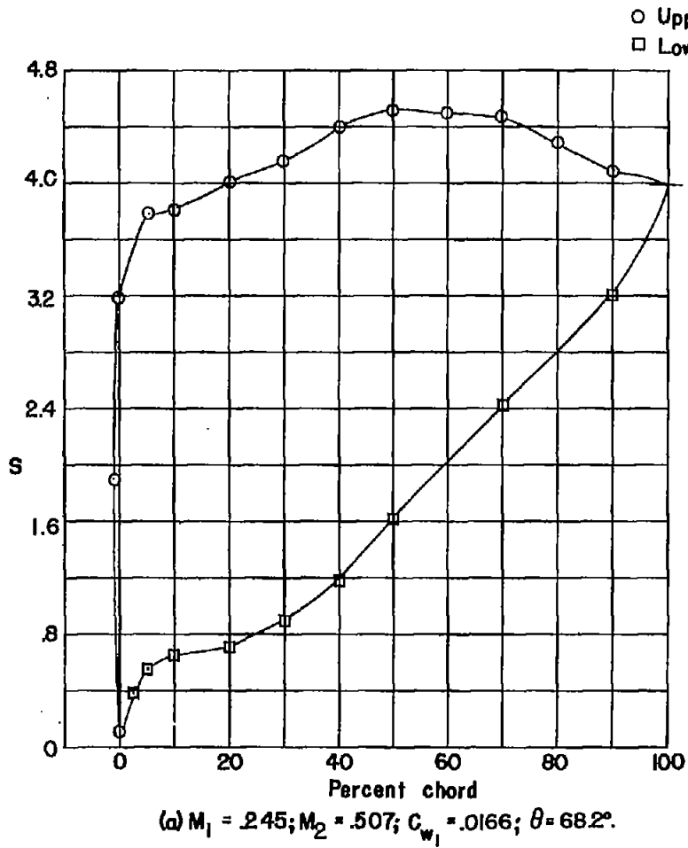
Figure 31.- High-speed pressure distributions for cascade combinations \beta_1 = 10^\circ , \alpha_1 = 48.4^\circ , \sigma = 1.8 , and primary turbine blade section, \theta_c = 80^\circ .
