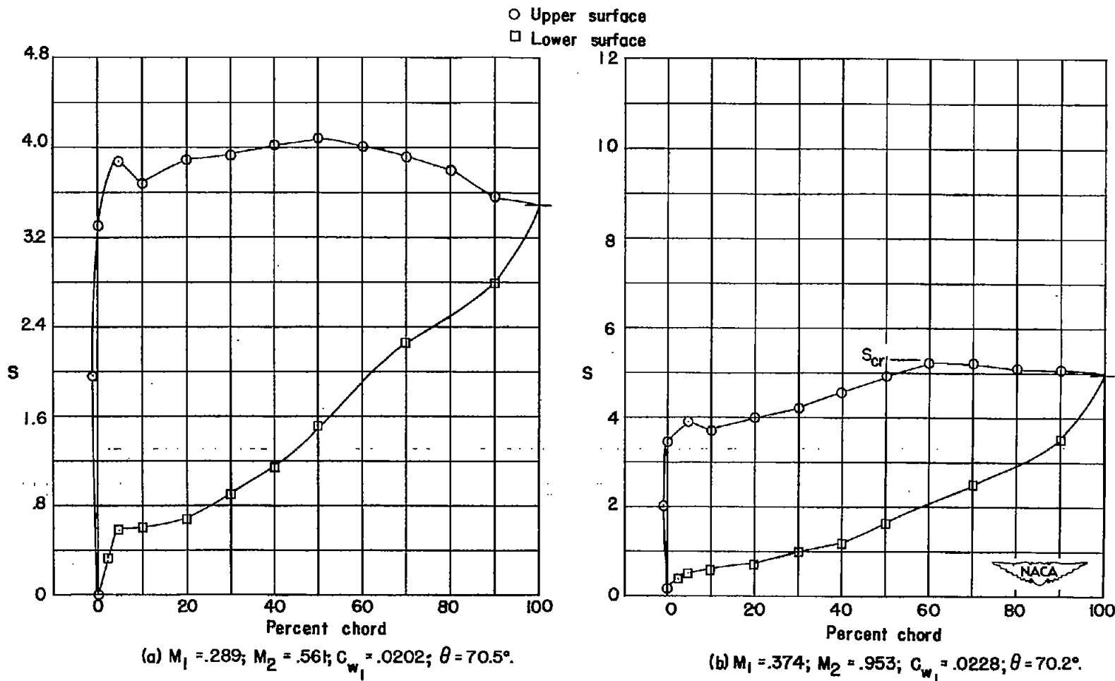
Figure 32.- High-speed pressure distributions for cascade combinations \beta_1 = 15^\circ, \alpha_1 = 50.4^\circ, \sigma = 1.8 , and primary turbine blade section, \theta_c = 80^\circ .
