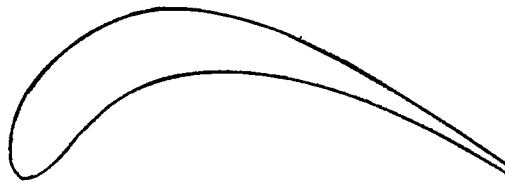
Primary turbine blade section, \theta_c = 110^\circ , t/c = 15 percent
