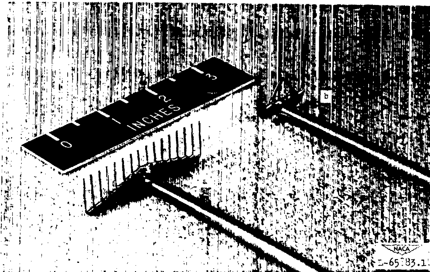
(a) Total head rake.
