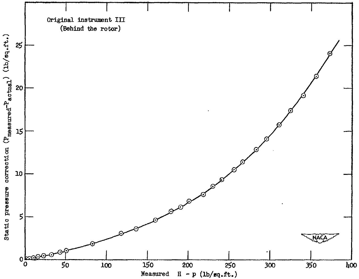
Figure 6.- A typical calibration curve.
