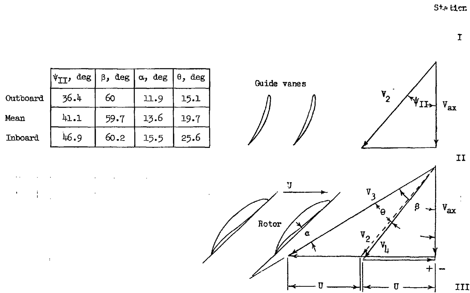
Figure 3.- Velocity diagram at design conditions.
