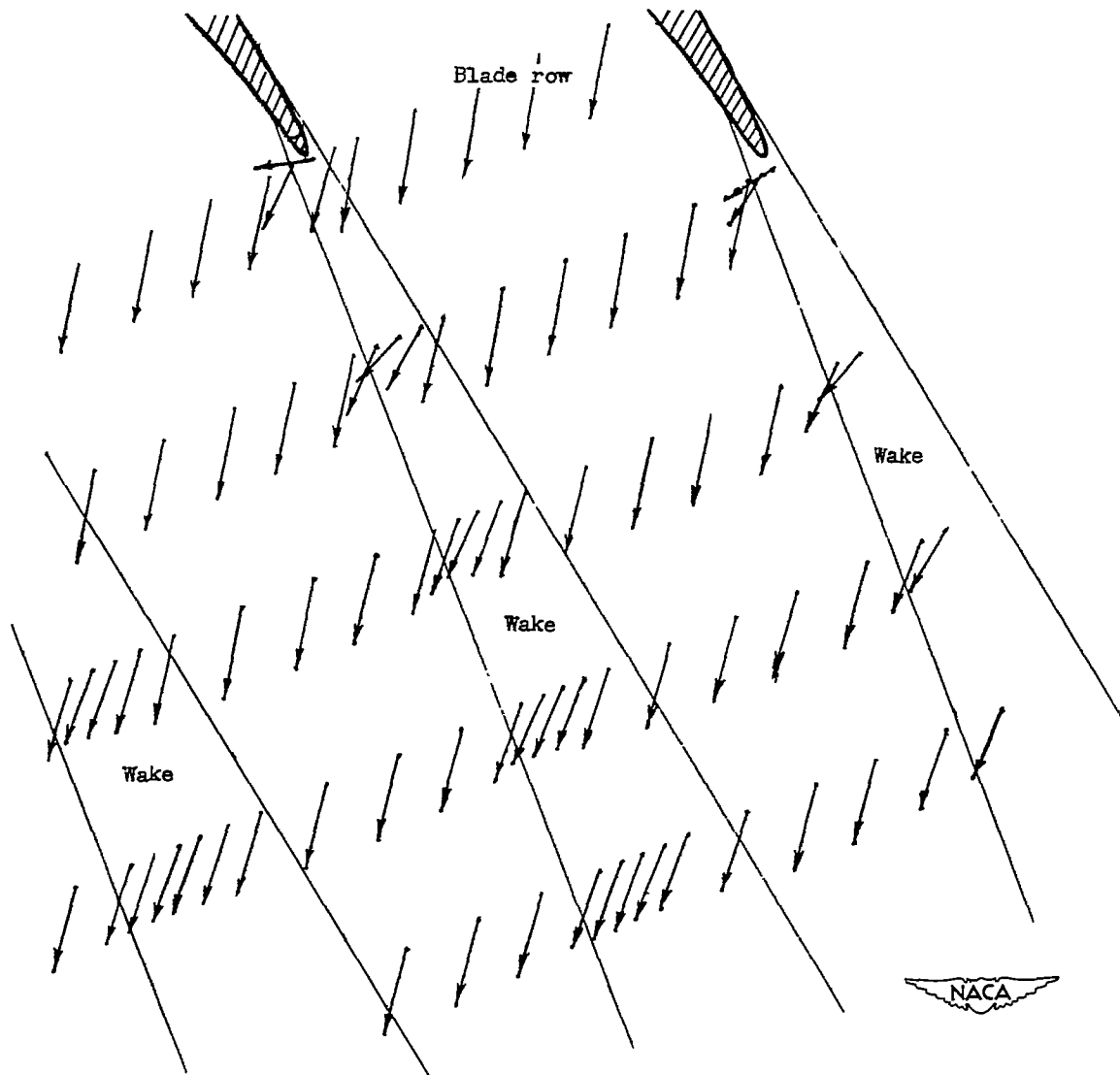
(b) Velocity distribution behind the rotor in stationary coordinates.
