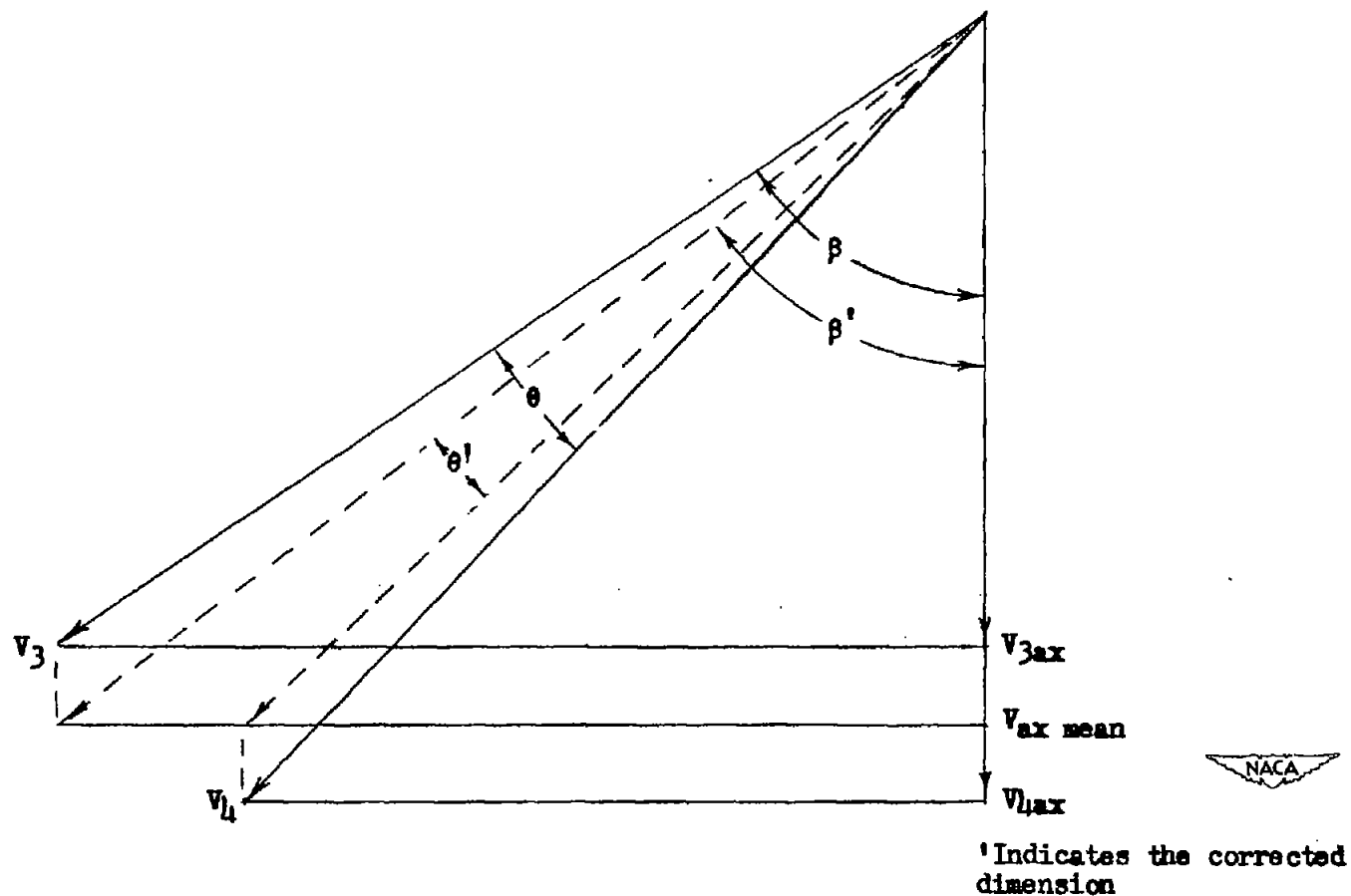
Figure 13.- A vector diagram demonstrating the method of correcting the air angles by using a mean axial velocity.
