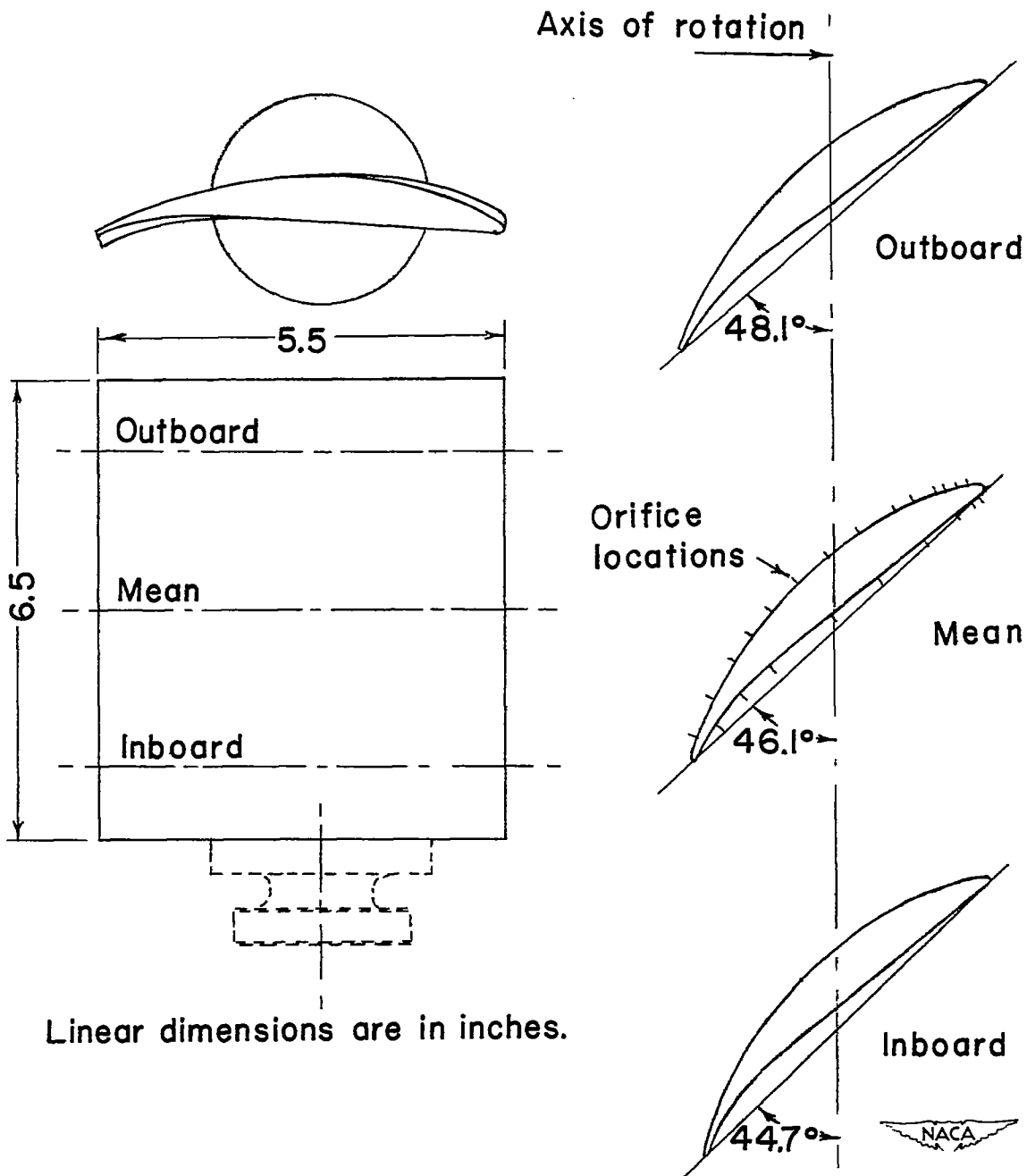
Figure 2.- Sketch of rotor blades.
