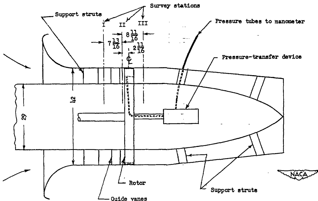
(b) Schematic sketch of test section. (All linear dimensions are in inches.)
