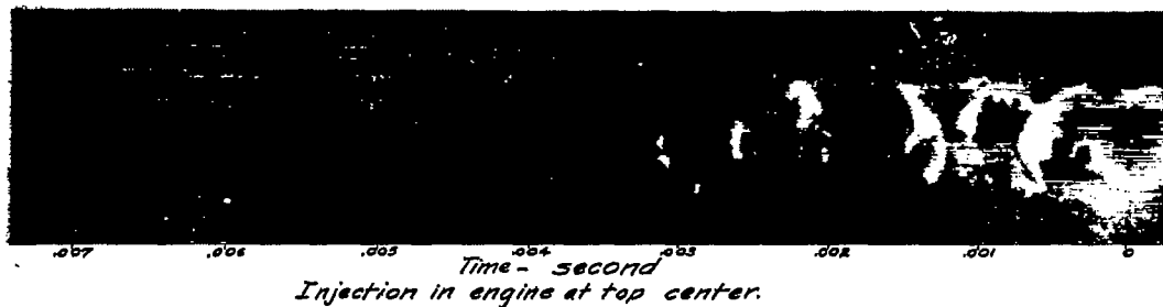
Injection valve in horizontal position. Engine speed 1500 r.p.m.
