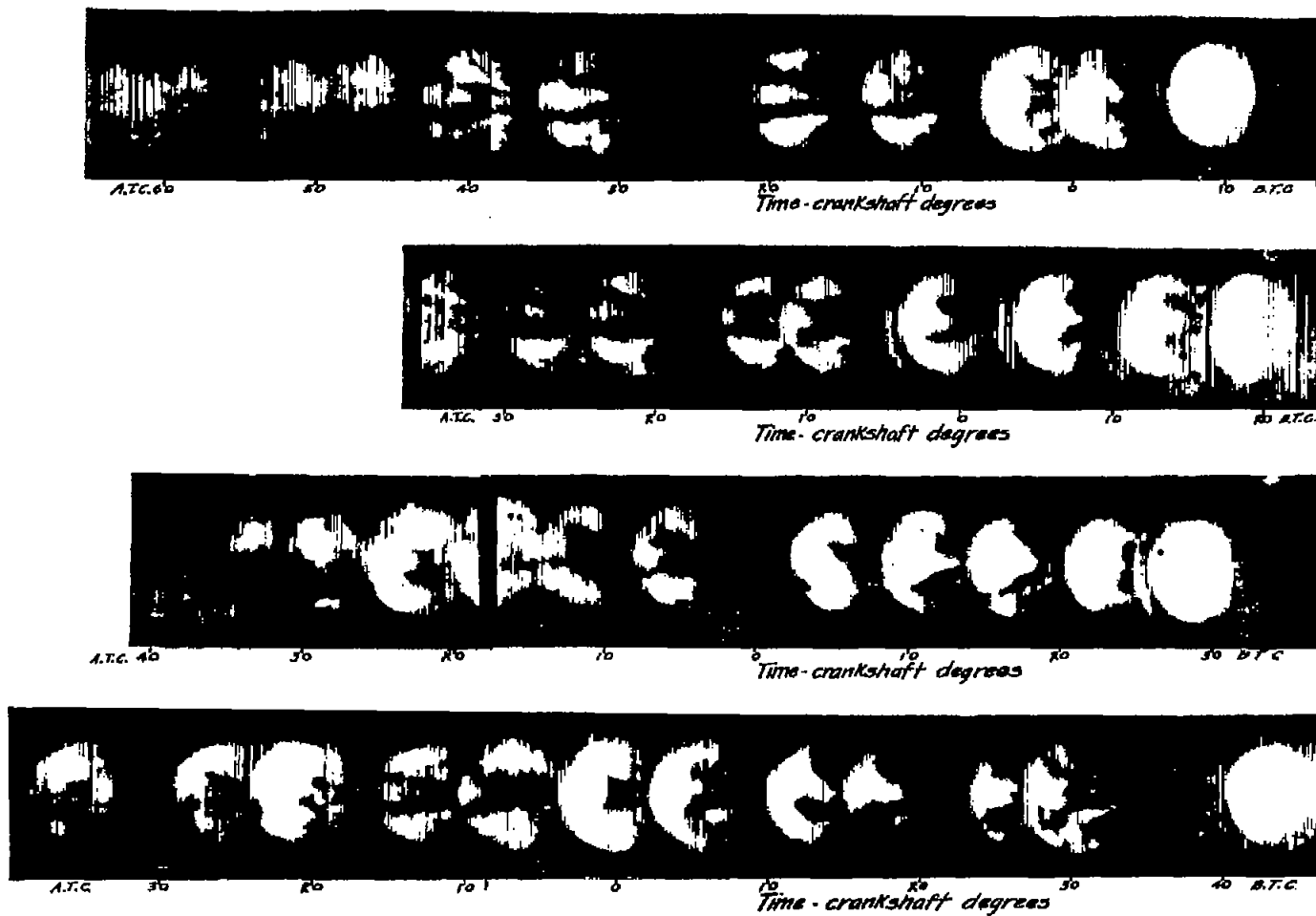
Fig.12 Effect of air flow on the fuel spray. Injection valve in vertical position. Injection pressure, 4000 lb./sq. in. Engine speed, 1500 r.p.m. Safety fuel.
