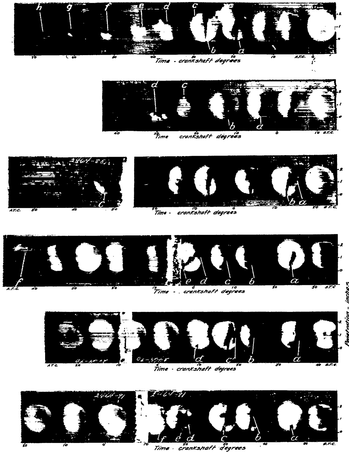
Fig. 8 Effect of air flow on the fuel spray. Injection valve in horizontal position. Injection pressure, 4000 lb./sq. in. Engine speed, 1500 r.p.m.
