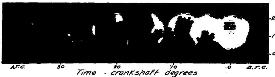
Fig. 4 Reproducibility of fuel spray. Injection valve in horizontal position. Injection pressure, 4000 lb. per sq. in. Engine speed, 1500 r.p.m.
