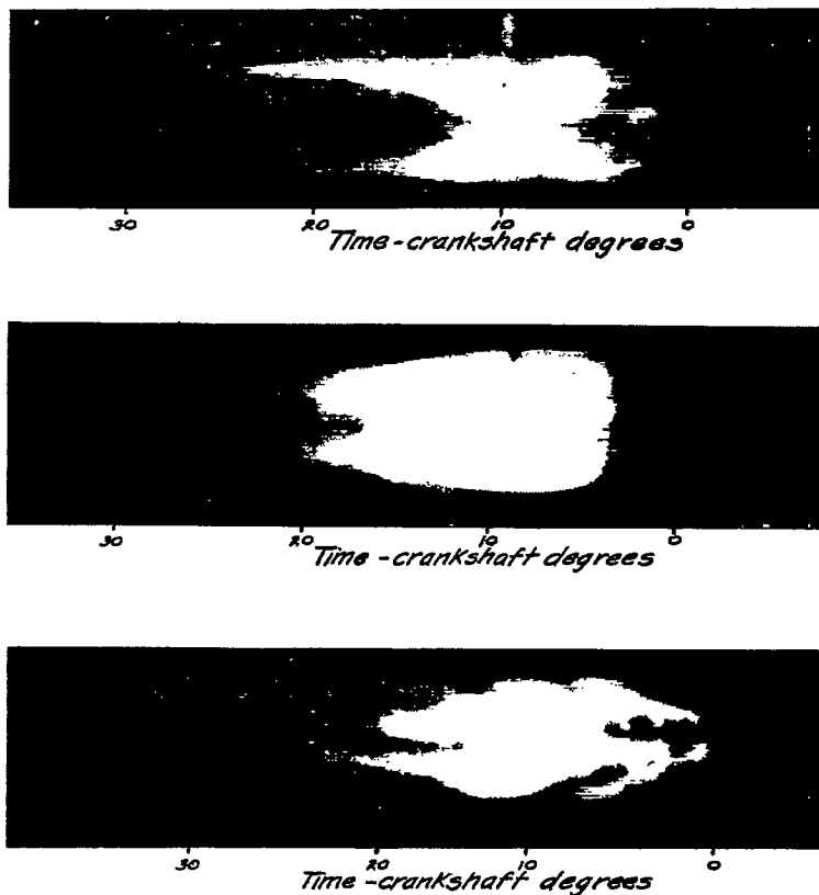
Fig. 15 Combustion with ignition lag of several engine revolutions. Injection valve in vertical position. Injection pressure, 4000 lb. per sq. in. Engine speed, 1500 r.p.m.
