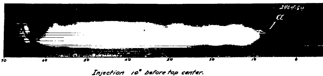
Fig. 15 Combustion with ignition lag of several engine revolutions. Injection valve in vertical position. Injection pressure, 4000 lb. per sq. in. Engine speed, 1500 r.p.m.
