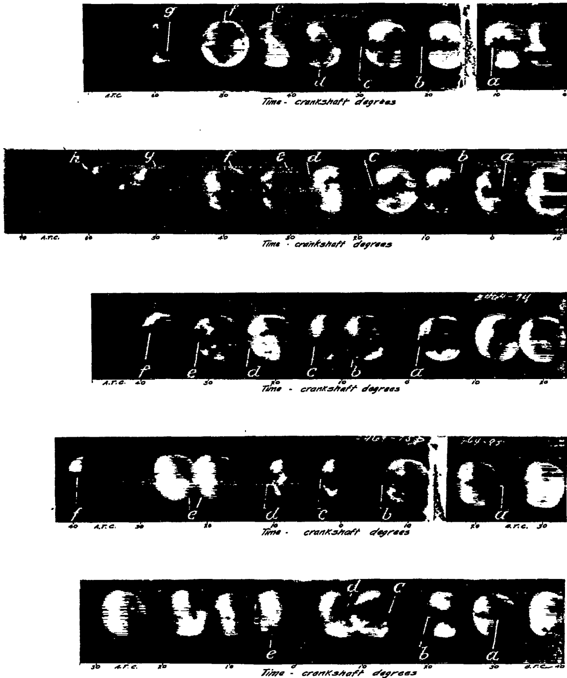
Fig. 9 Effect of air flow on the fuel spray. Injection valve in vertical position. Injection pressure, 4000 lb./sq.in. Engine speed, 1500 r.p.m.
