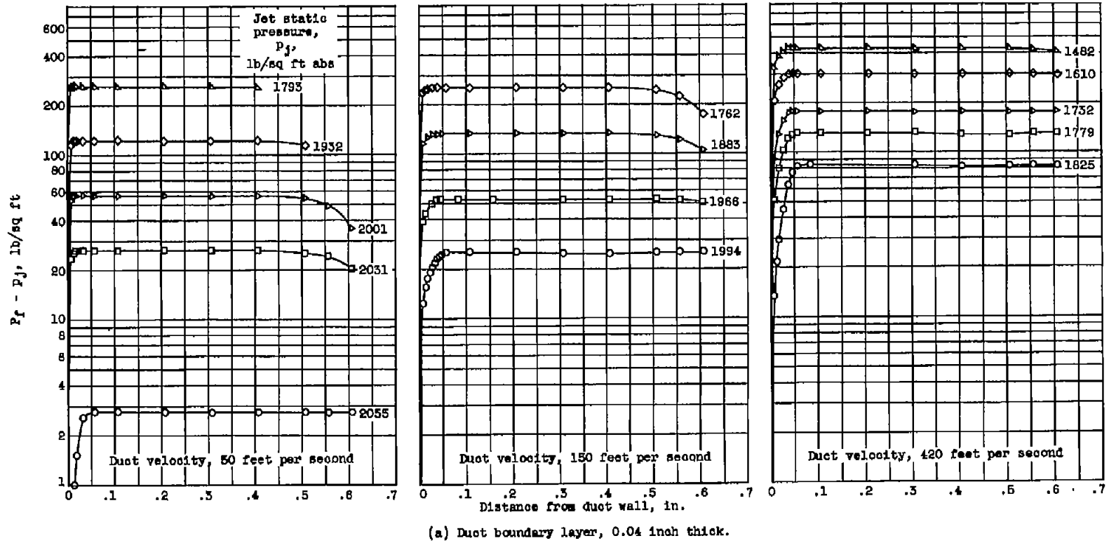
Figure 6. - Pressure profiles measured at face of 0.623-inch-high step louver at various flow conditions.
