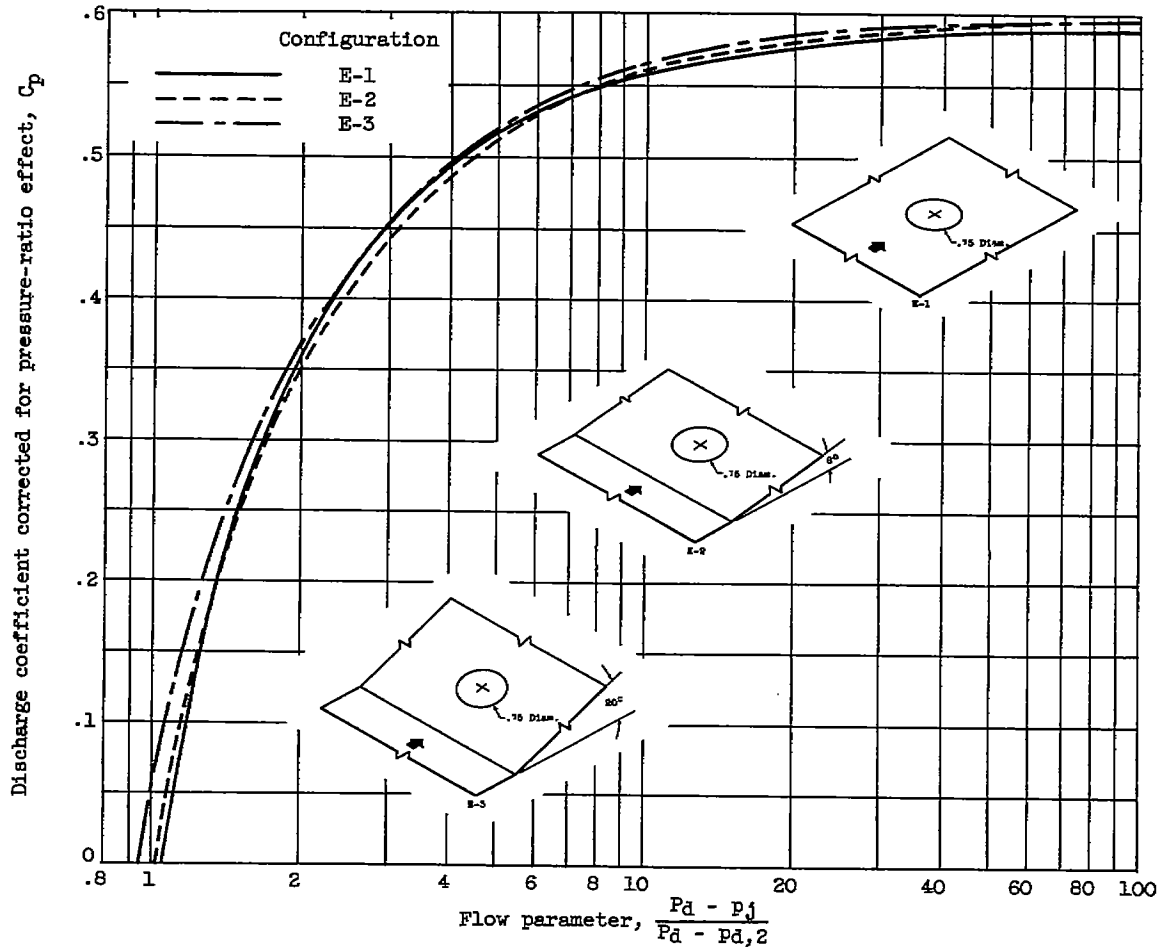
(a) Flush circular hole with 0.75-inch diameter.
