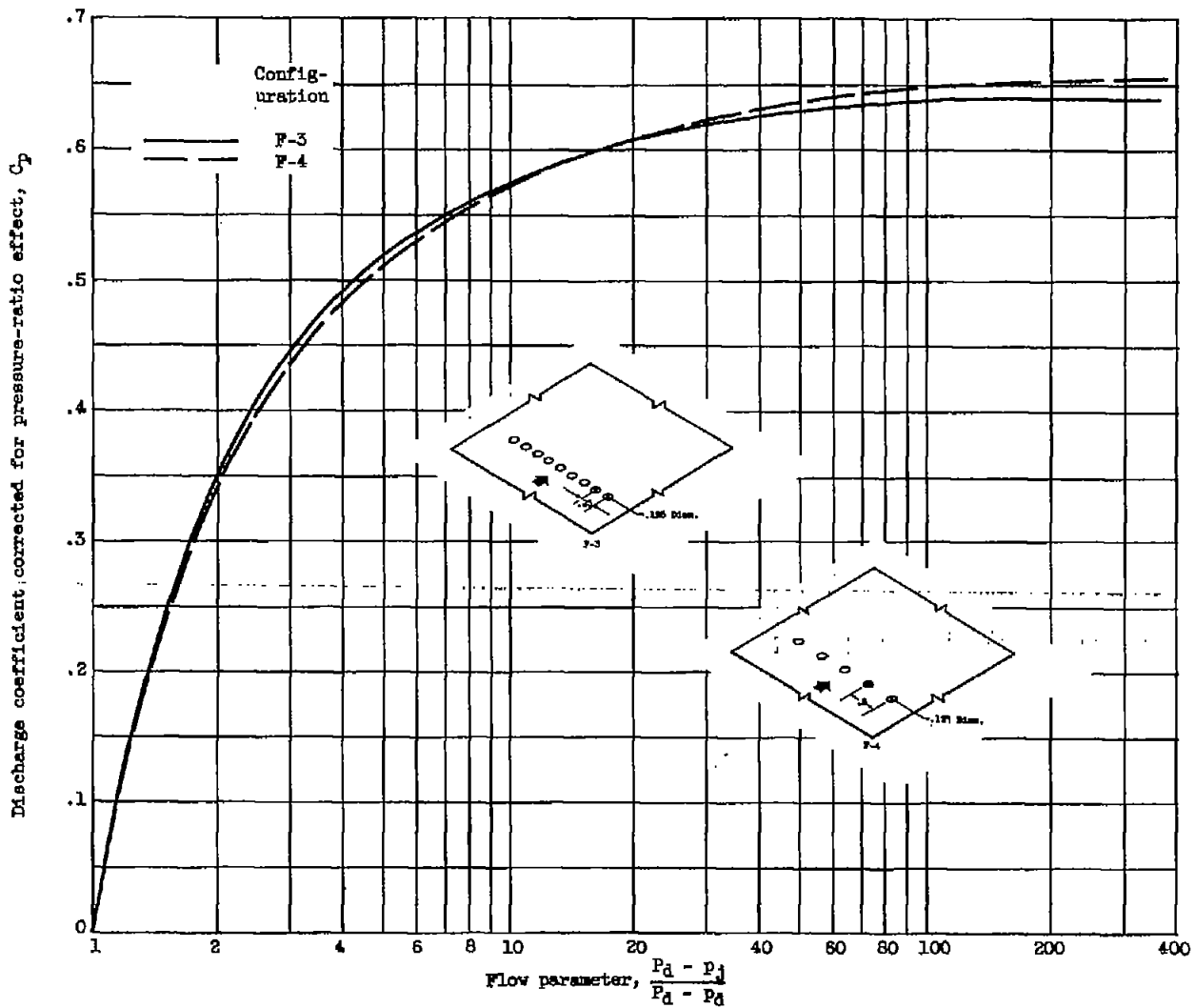
(b) Holes side by side.
