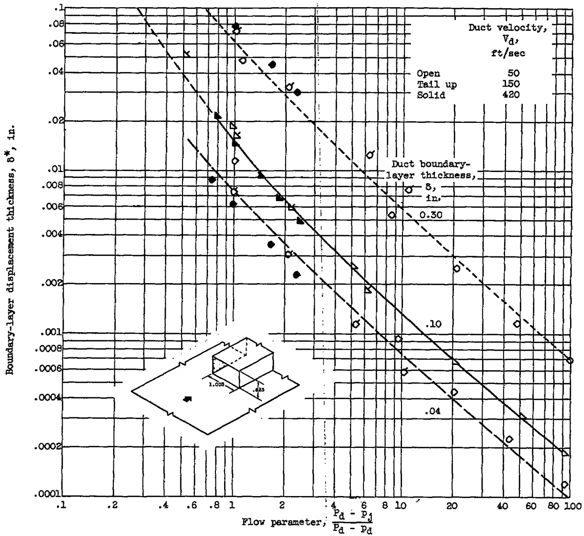
Figure 9. - Variation in boundary-layer displacement thickness at face of louver with flow parameter for three duct boundary-layer conditions.
