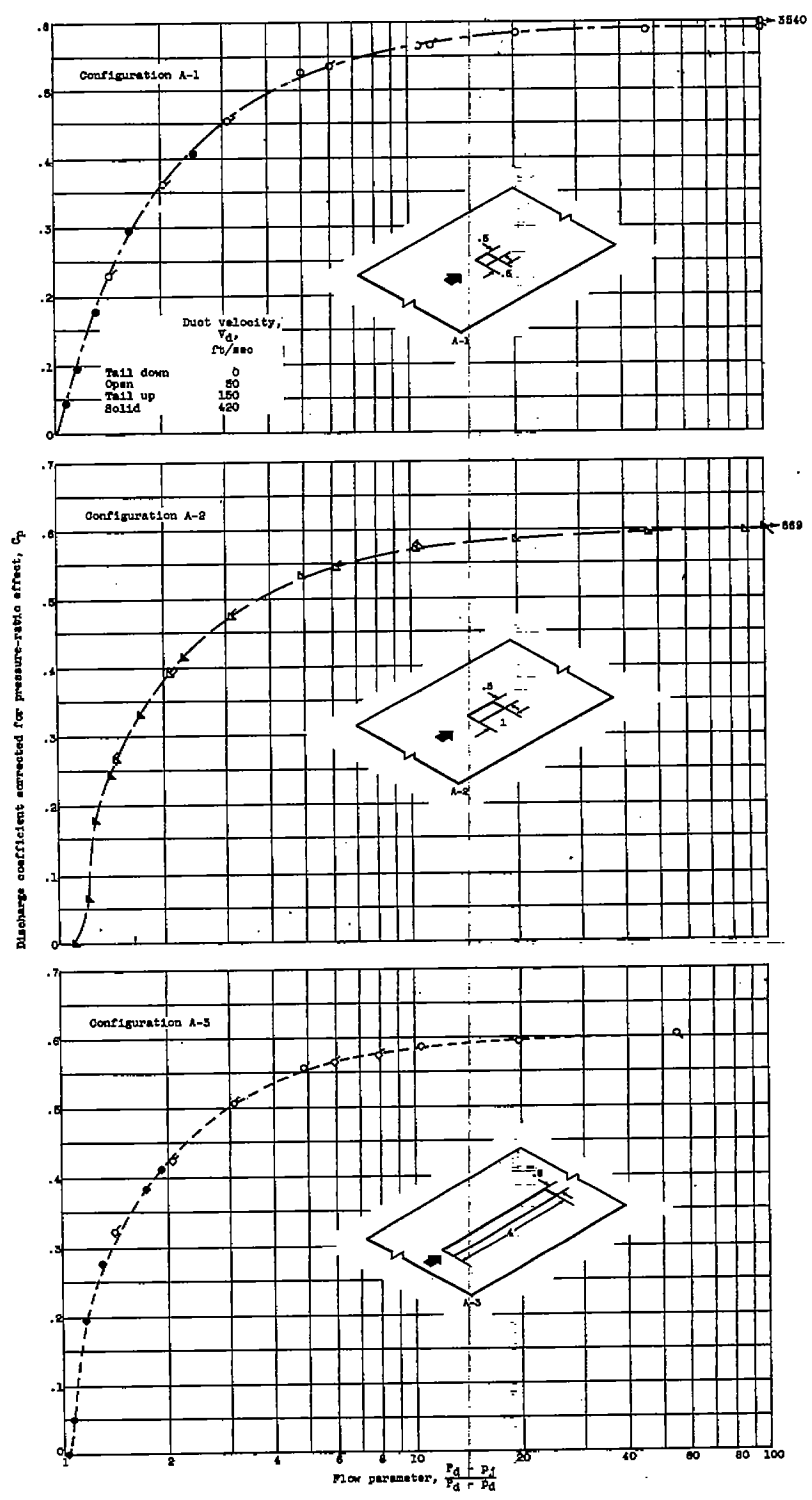
(a) Flush rectangular holes.
