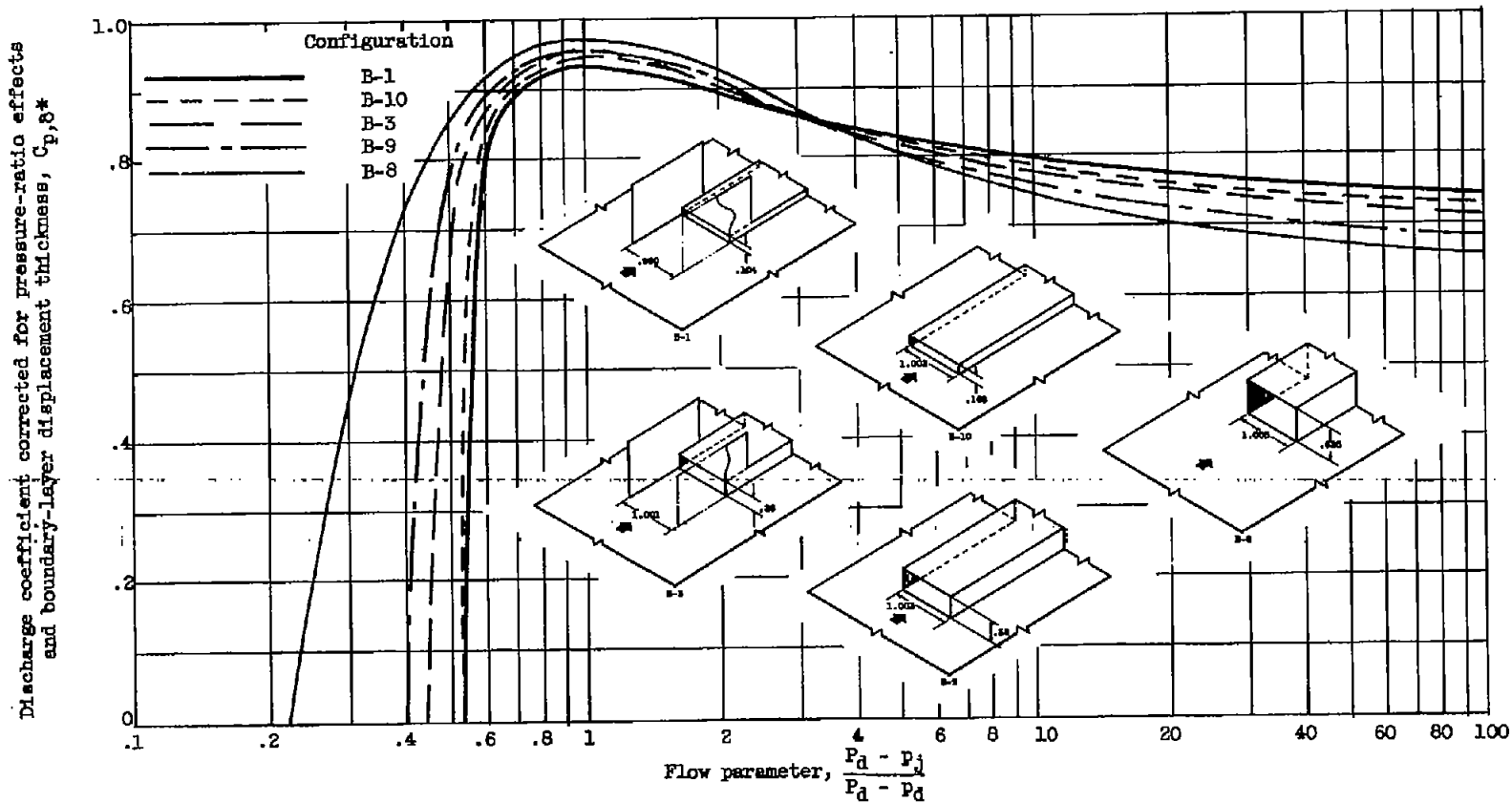
Figure 15. - Effect of step louver height on corrected discharge coefficient.
