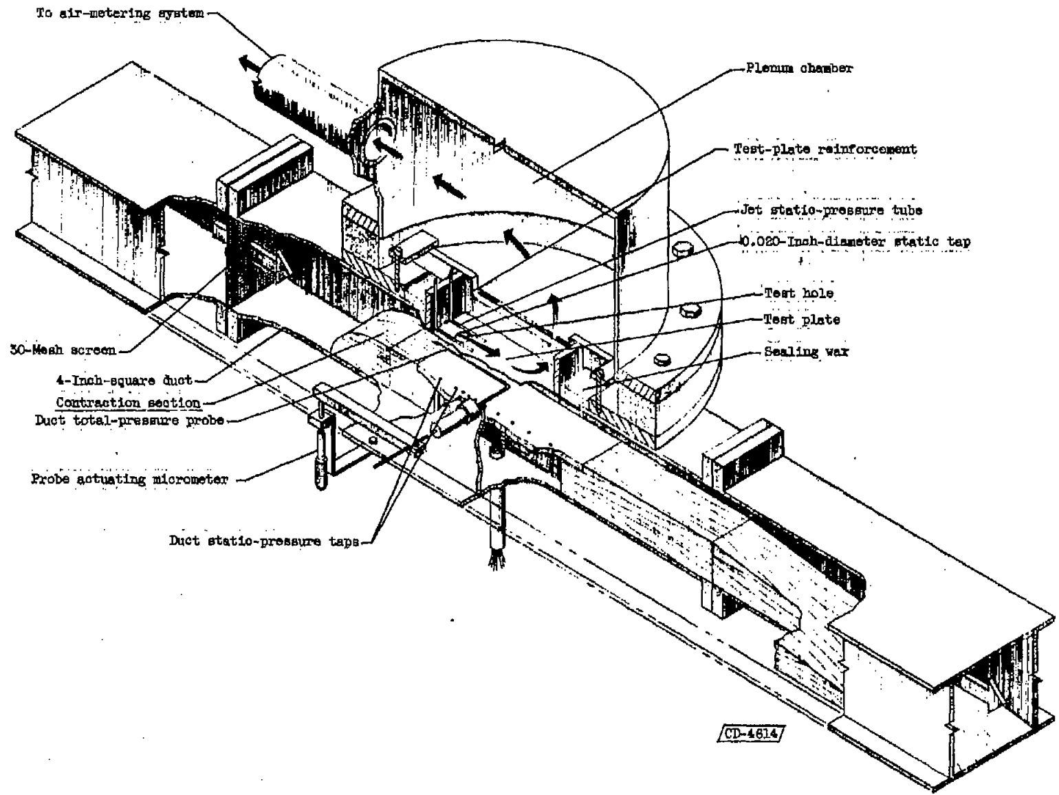
(a) Test plate flush with duct wall.
