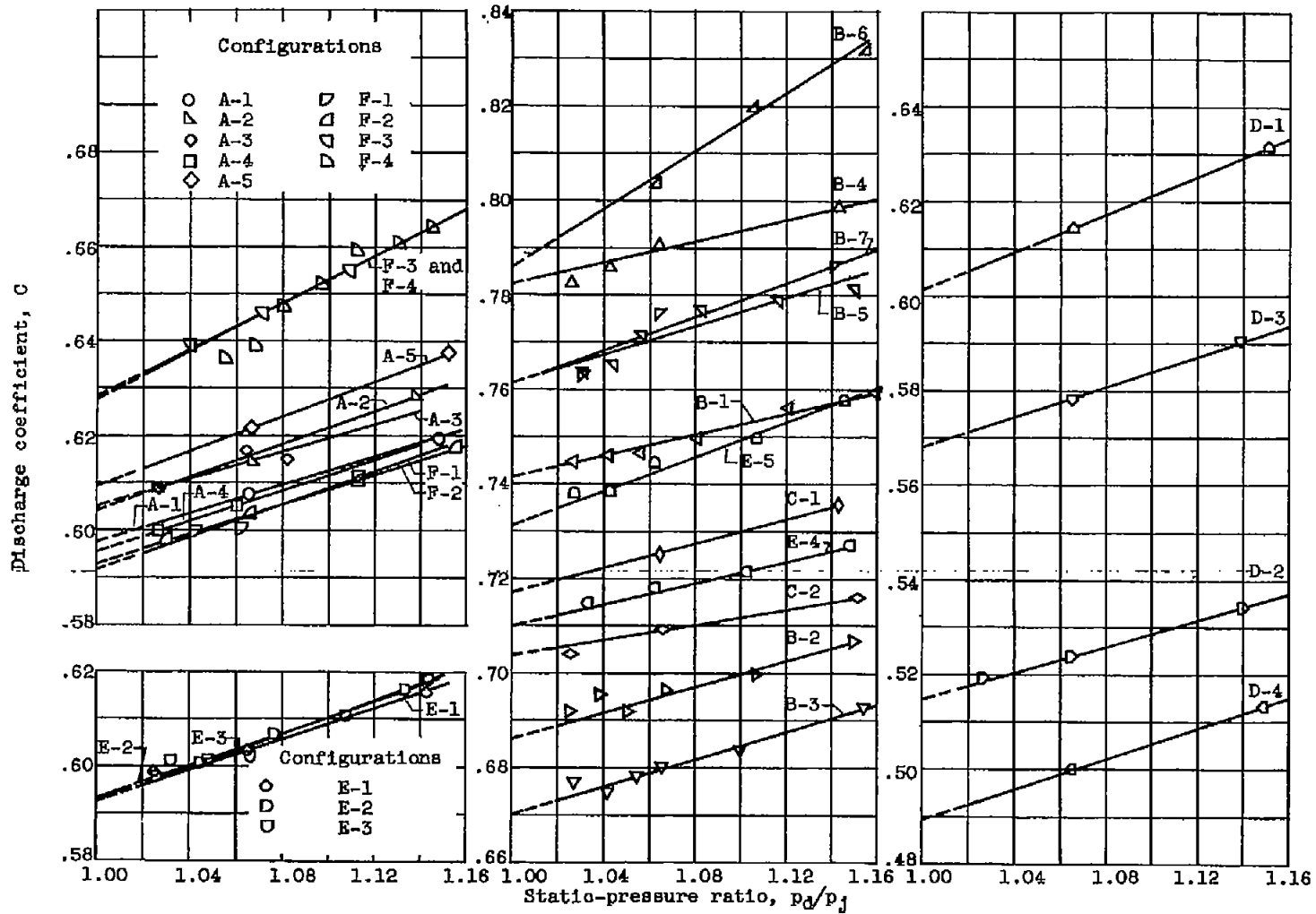
(a) Flush holes.
