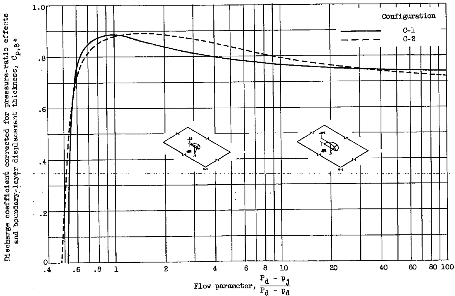
Figure 18. - Effect of height of thumbnail-type scoops on corrected discharge coefficient.
