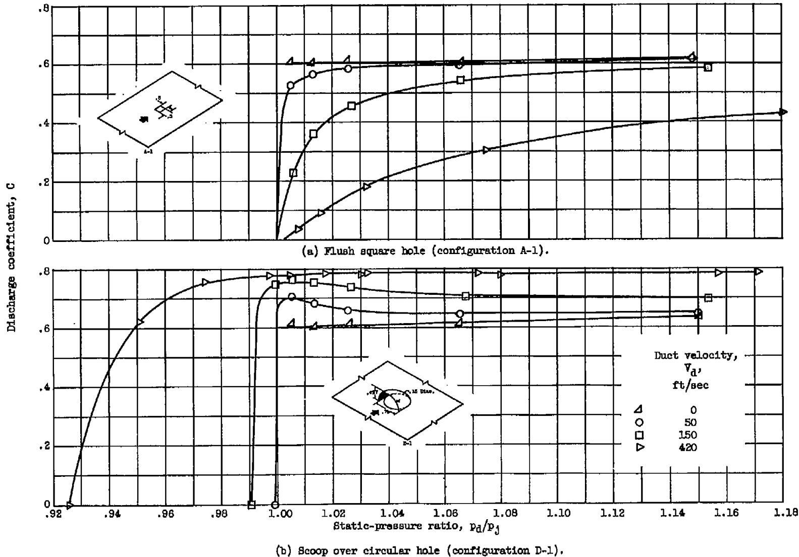
Figure 2. - Effect of static-pressure ratio on discharge coefficient at various duct velocities.
