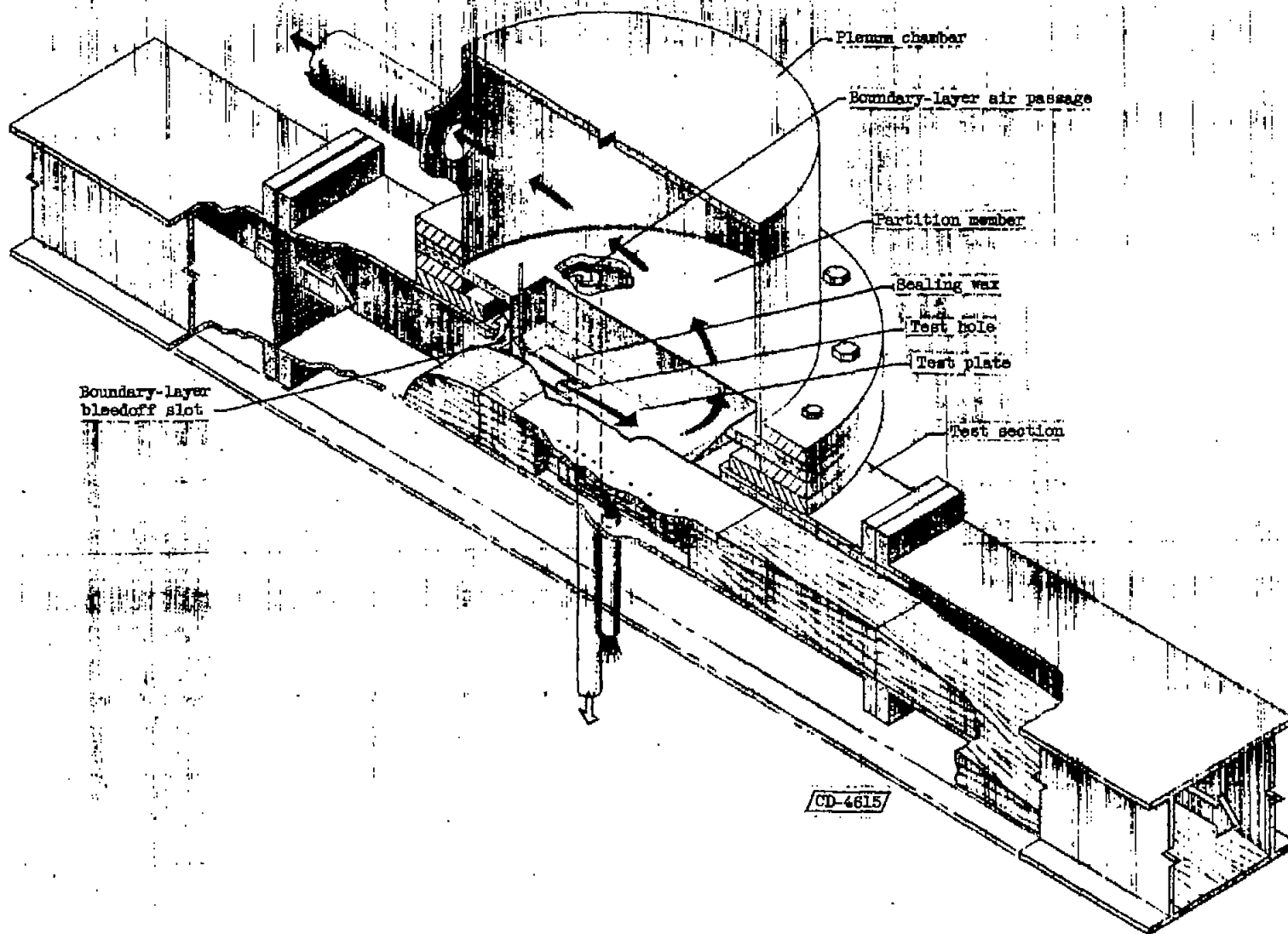
Figure 1. - Concluded. Details of test apparatus for study of discharge coefficients.
