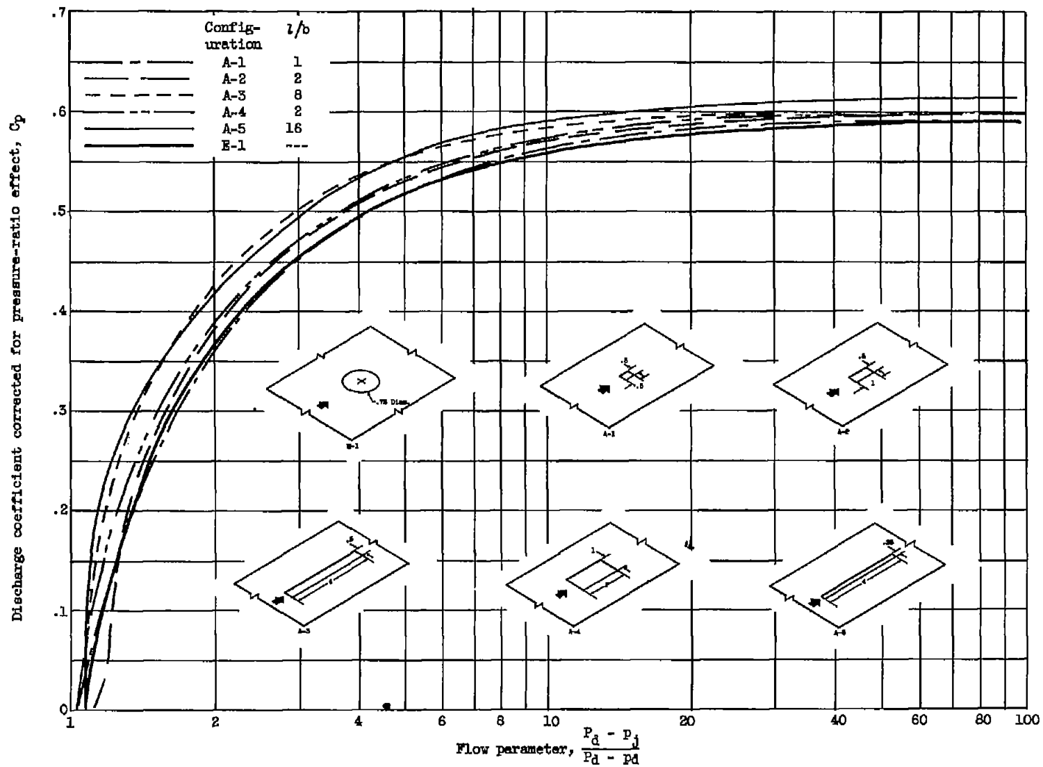
Figure 14. - Effect of flush rectangular hole dimensions on corrected discharge coefficient. (Curve for circular flush hole included for comparison.)
