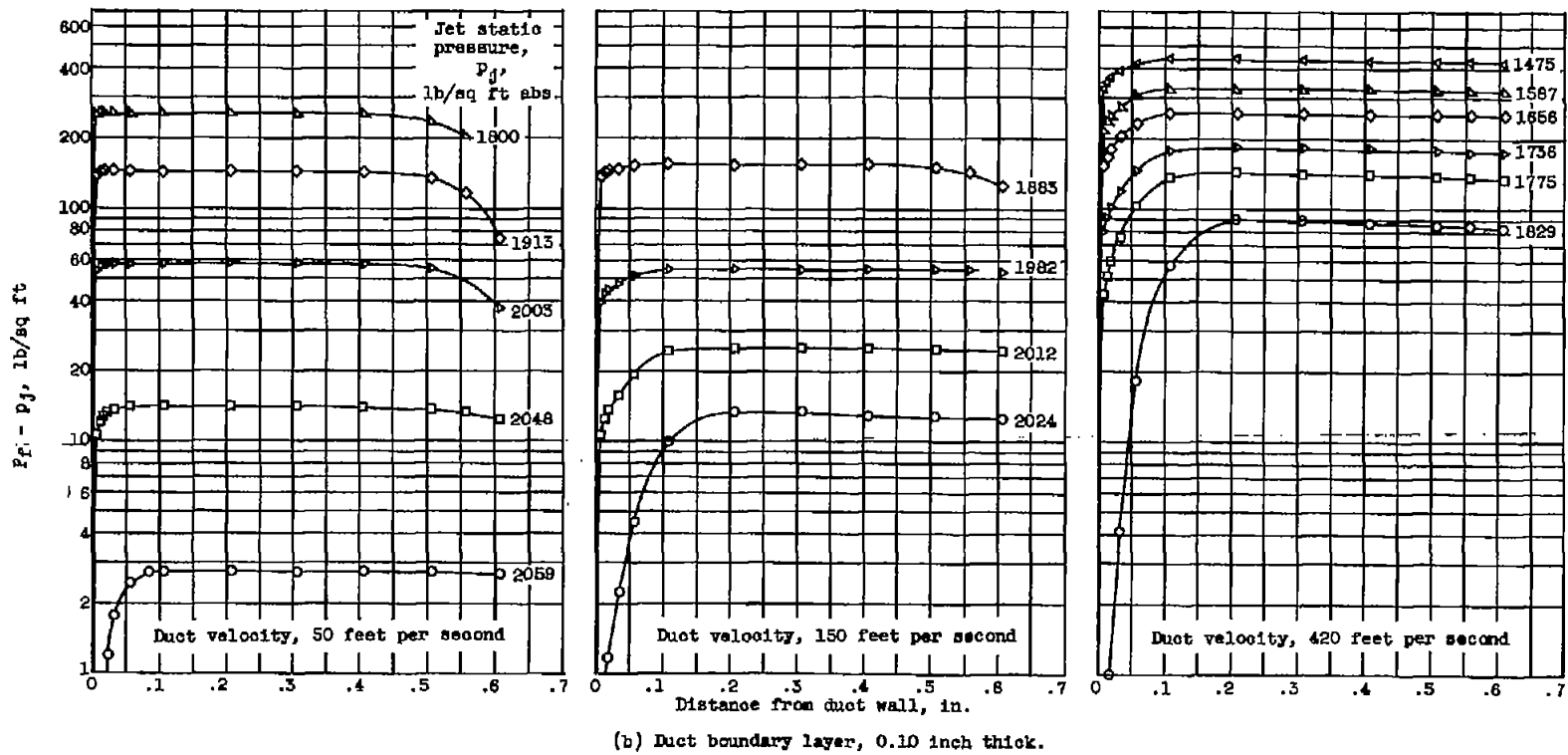
Figure 8. - Continued. Pressure profiles measured at face of 0.623-inch-high step louver at various flow conditions.
