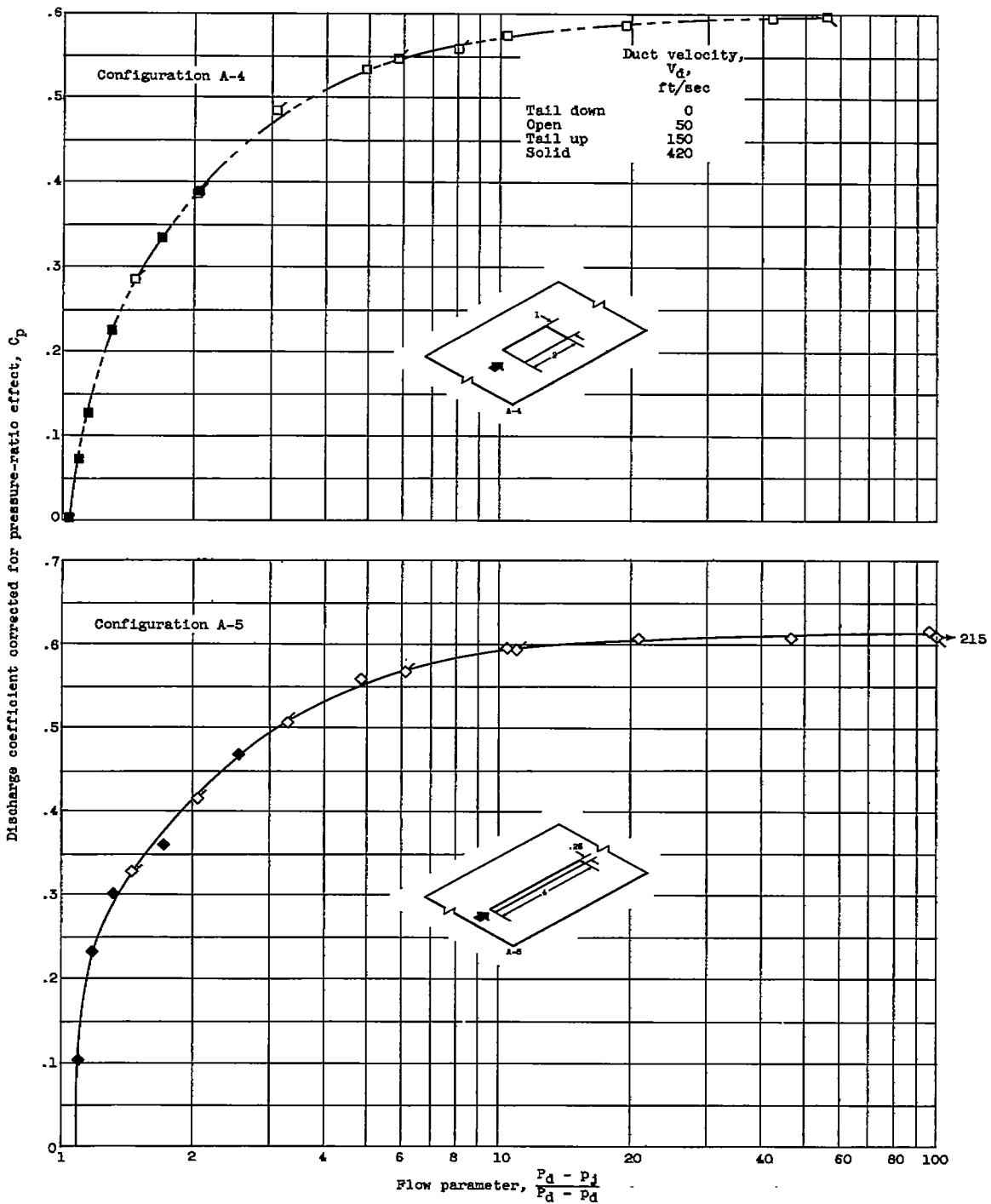
Figure 13. - Continued. Variation of corrected discharge coefficient with flow parameter.
