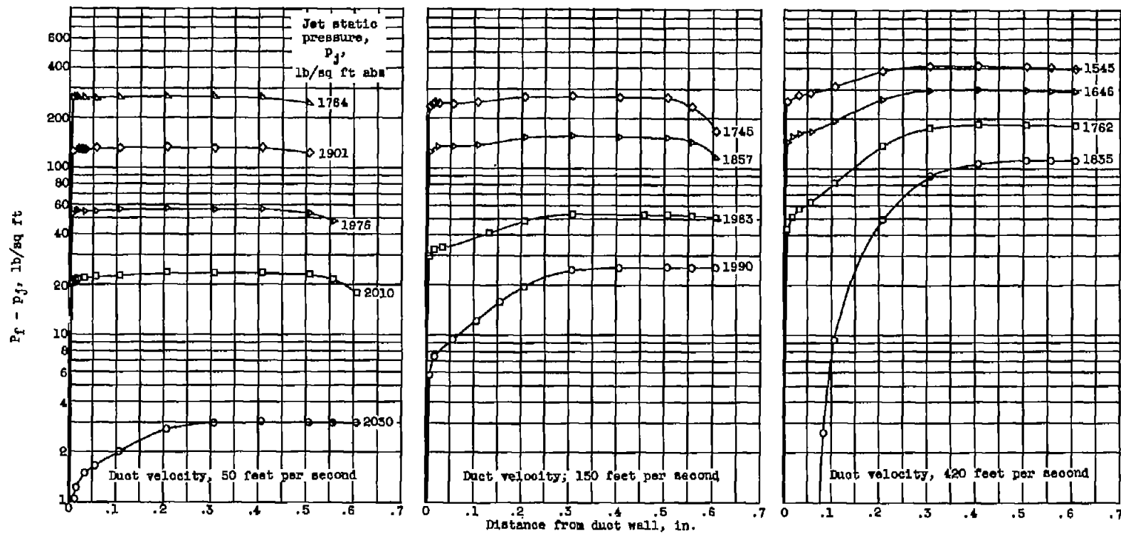
(c) Duct boundary layer, 0.30 inch thick.
