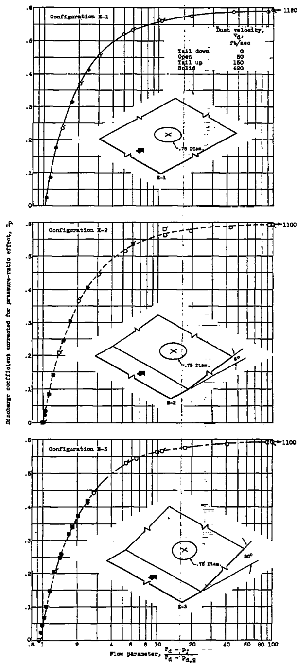
(e) Flush hole or step louver on inclined wall.
