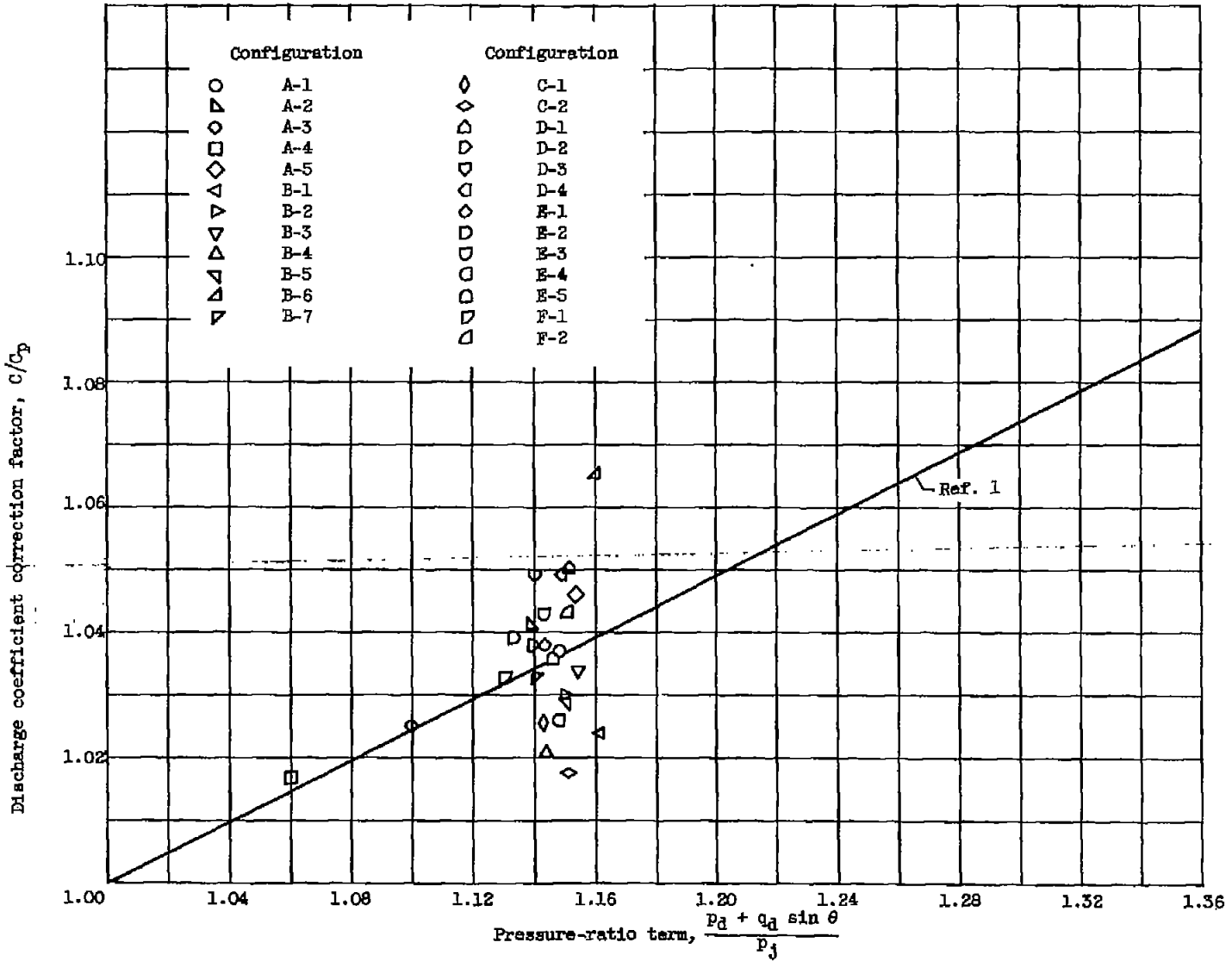
Figure 5. - Pressure-ratio correction factor for discharge coefficients.
