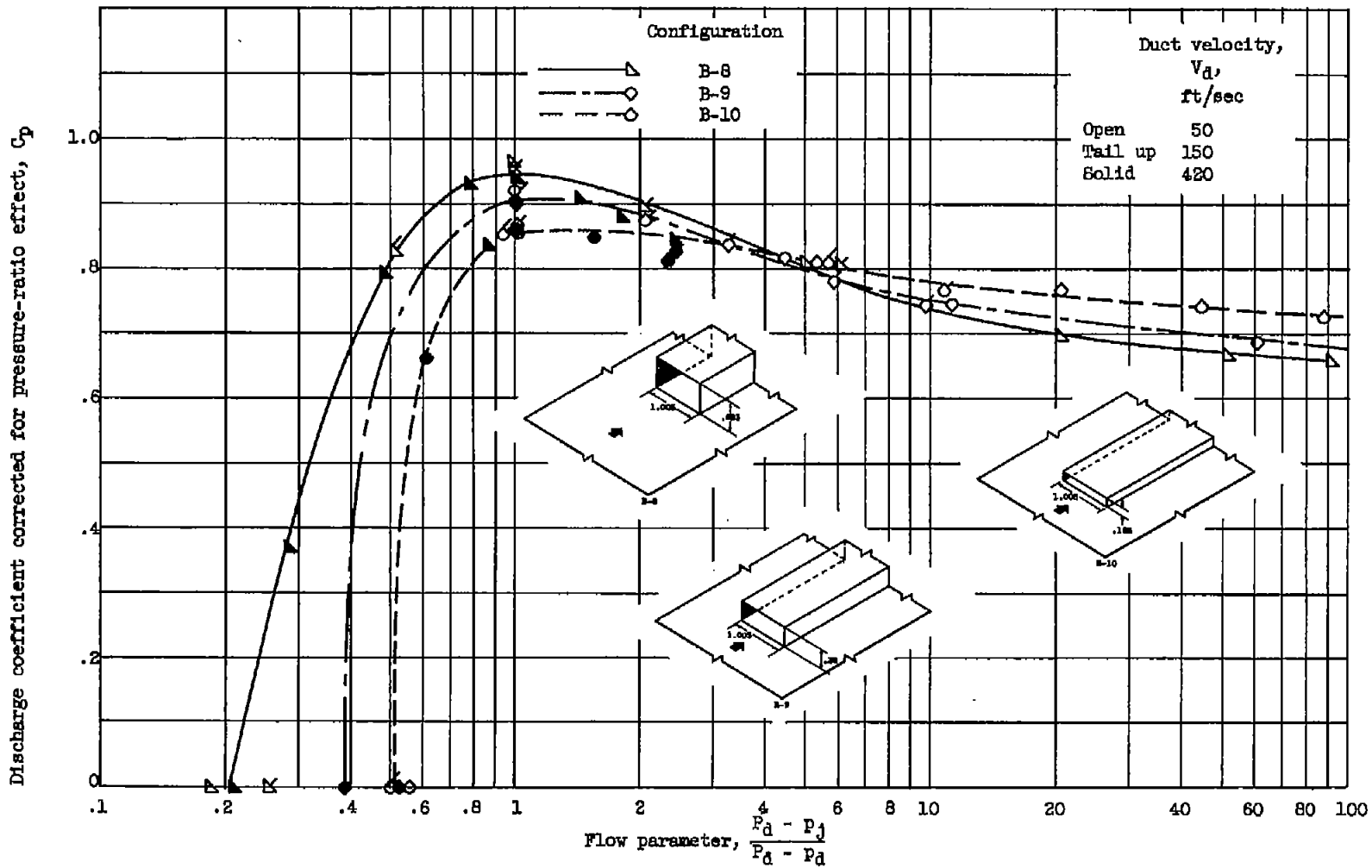
Figure 6. - Comparison of discharge coefficients for three heights of step louvers. Duct boundary layer, 0.10 inch thick. Discharge coefficients not corrected for boundary-layer effects.
