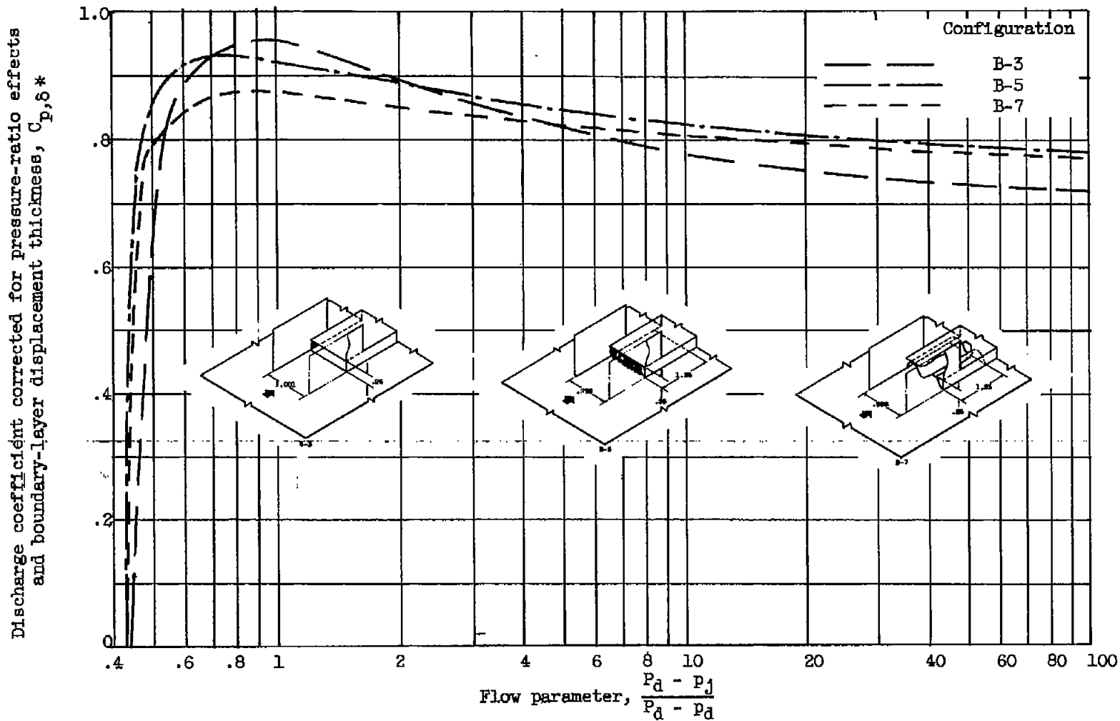
Figure 16. - Concluded. Effect of step louver overlap and corrugated spacer within the overlap on corrected discharge coefficient.
