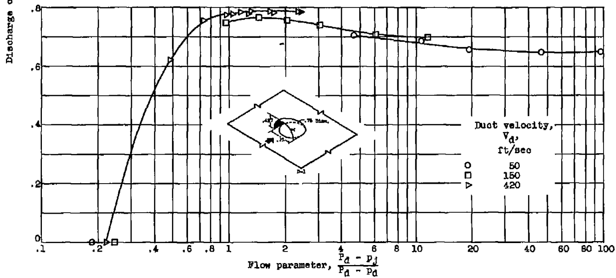
(b) Scoop over circular hole (configuration D-1).
