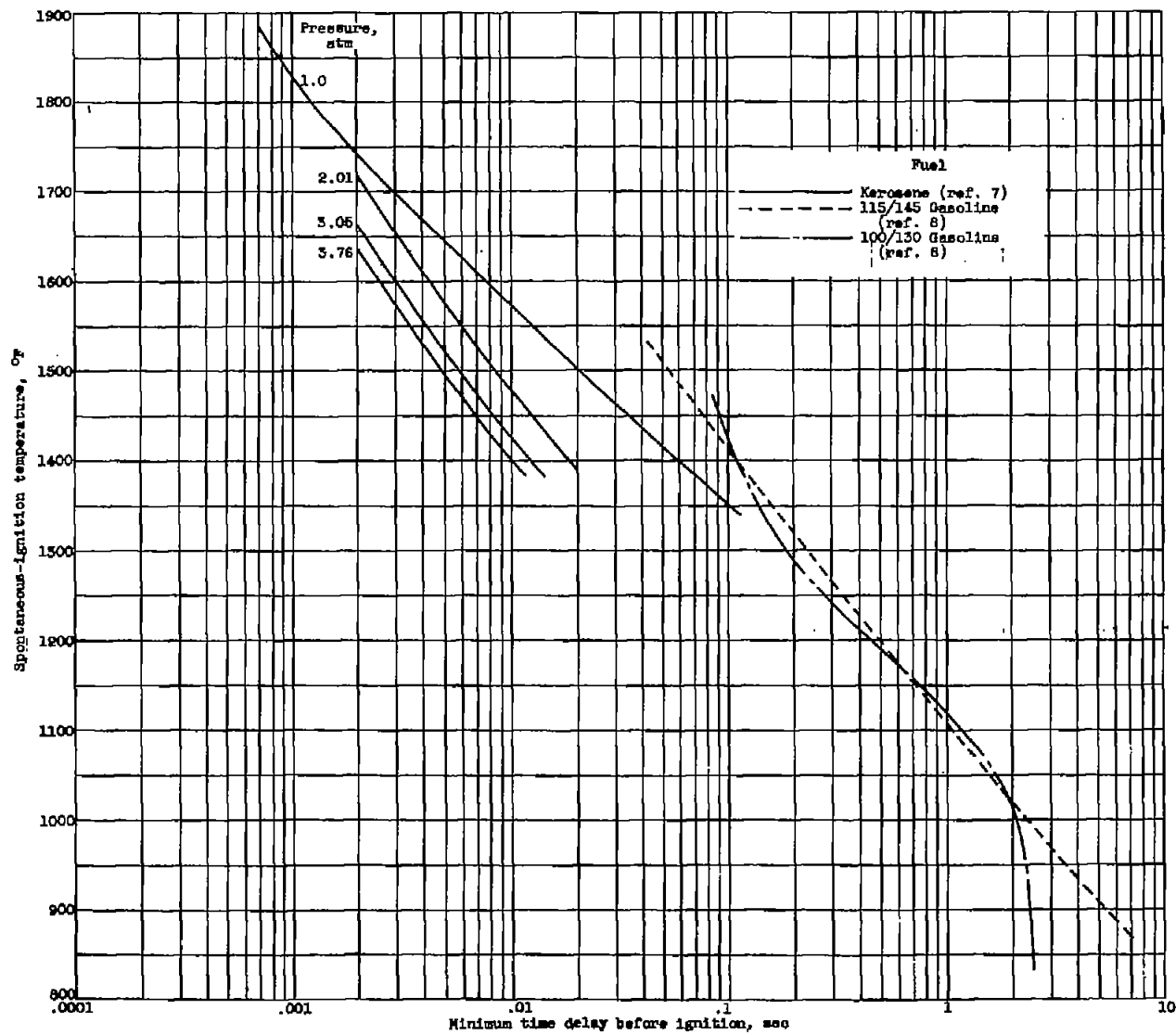
(b) Kerosene and 115/145 and 100/130 aviation gasolines. Figure 8. - Concluded. Ignition characteristics of aviation fuels.
