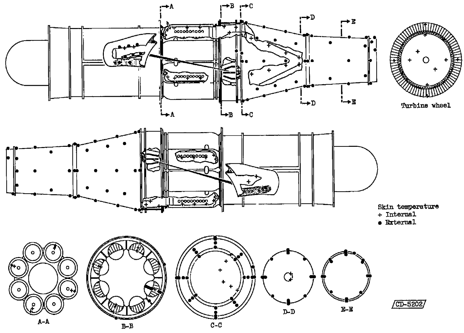
Figure 6. - Thermocouple locations on J47 engine.
