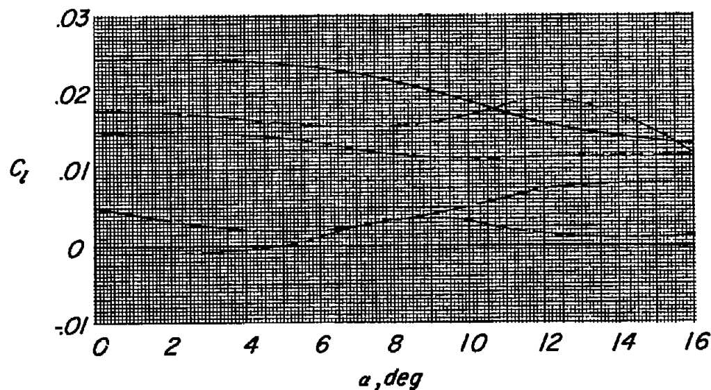
Figure 26.- Effect of span of the spoiler-slot-deflector and butterfly-valve arrangement on the aileron effectiveness for \delta_a = \pm 10^\circ on the 1/4-scale model of the X-5 airplane. \frac{(x_d)_{\Lambda=0^\circ}}{c_{\Lambda=0^\circ}} = 0.35.
