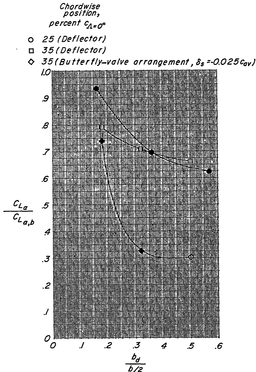
Figure 5.- Variation of lift-curve-slope reduction with span of deflector at the 25- and 35-percent-chord locations and of the butterfly-valve arrangement at the 35-percent-chord location on the 1/4-scale model of the X-5 airplane. \delta_d = -0.15c_{av} . Solid symbols indicate nonlinear lift curves.
