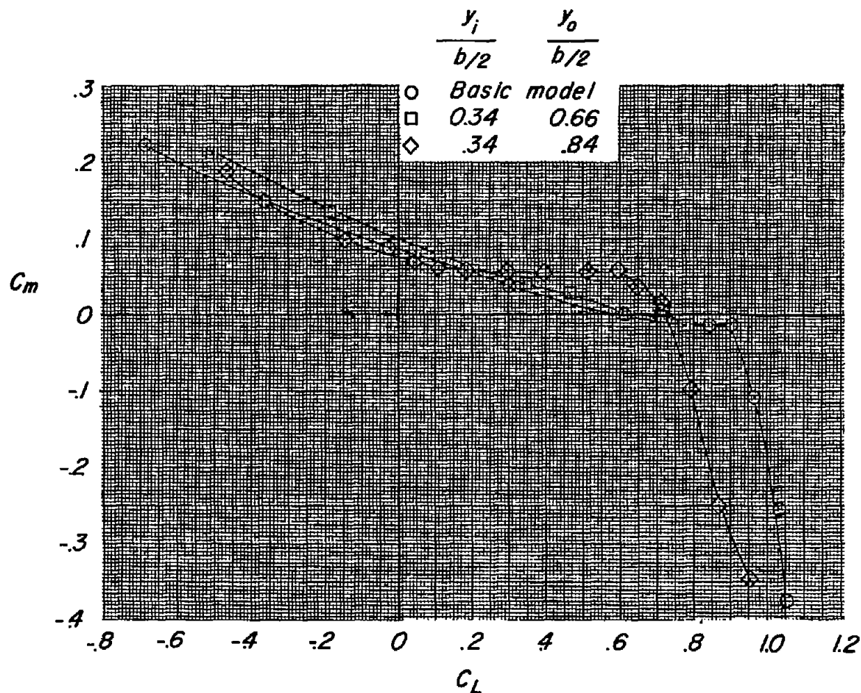
Figure 8.- Effect of span of butterfly-valve arrangement on the longitudinal stability of the X-5 model. \delta_B = -0.025c_{av} ; \delta_d = -0.075c ; \frac{(x_d)_{\Lambda=0^\circ}}{c_{\Lambda=0^\circ}} = 0.35 ; i_t = -5^\circ .
