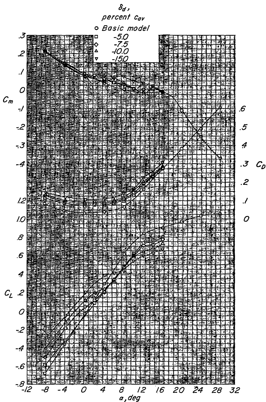
Figure 20.- Longitudinal aerodynamic characteristics of the 1/4-scale model of the X-5 airplane with butterfly-valve arrangement.
