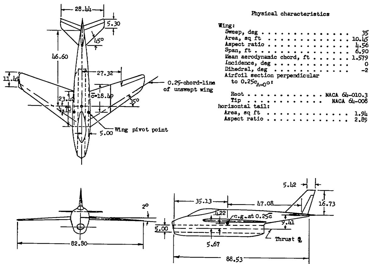
(a) 1/4-scale model of the Bell X-5 airplane.
