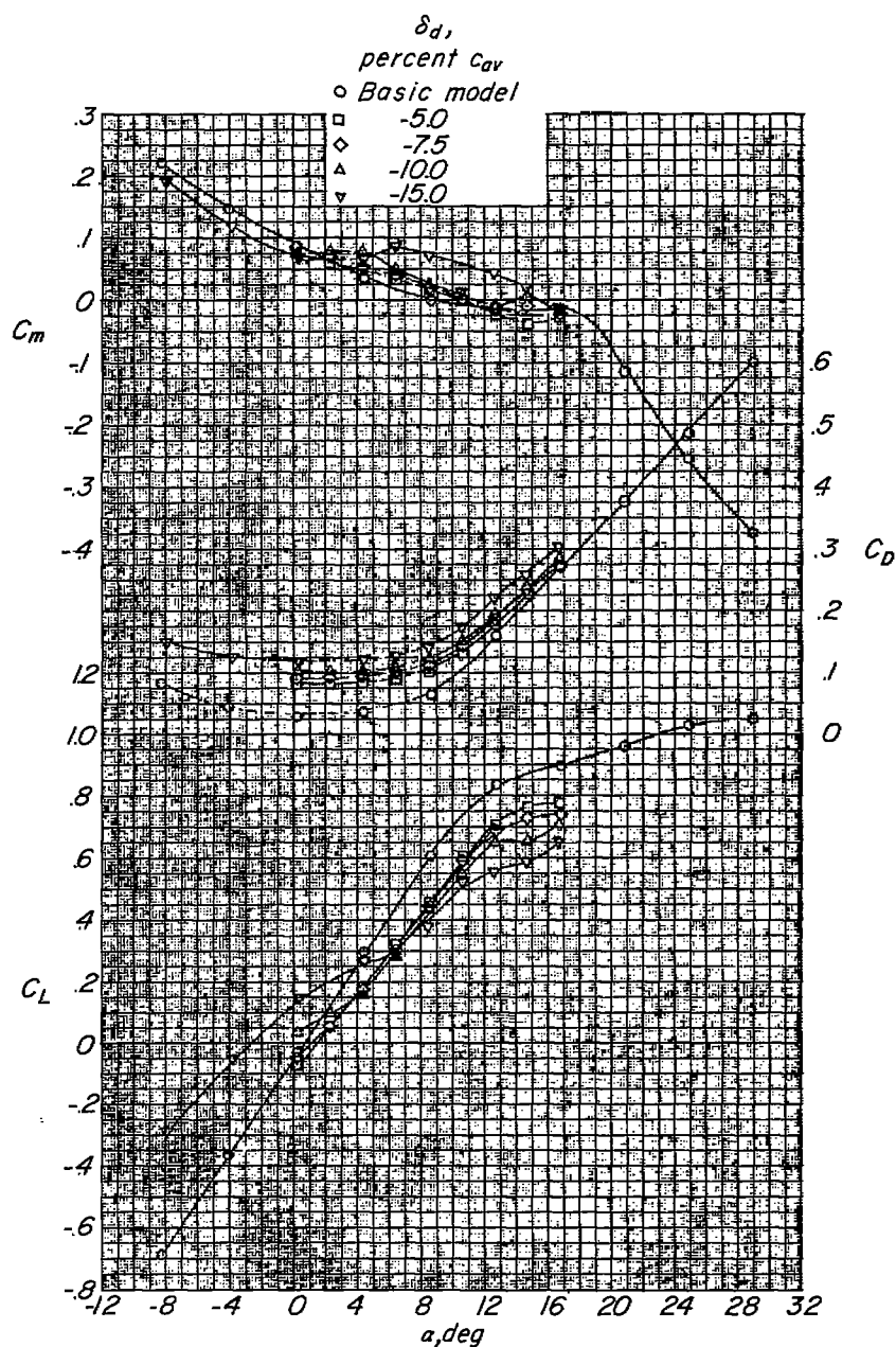
Figure 18.- Longitudinal aerodynamic characteristics of the 1/4-scale model of the X-5 airplane with a spoiler-slot-deflector. \delta_s = -0.025c_{av} ; \frac{(x_d)_{\Lambda=0^\circ}}{c_{\Lambda=0^\circ}} = 0.35 ; \frac{y_1}{b/2} = 0.34 ; \frac{y_0}{b/2} = 0.66 ; i_t = -5^\circ .
