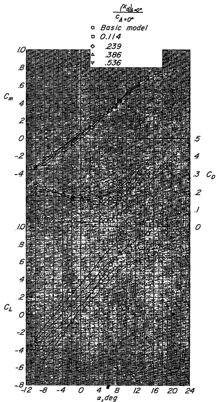
Figure 11.- Longitudinal aerodynamic characteristics of the high-aspect-ratio model with deflectorors. \delta_d = -0.15c ; \frac{y_1}{b/2} = 0.29 ; \frac{y_0}{b/2} = 0.96 .
