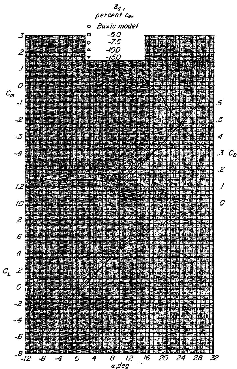
Figure 14.- Longitudinal aerodynamic characteristics of the 1/4-scale model of the X-5 airplane with a spoiler-slot-deflector. \delta_s = -0.025c_{av} ; \frac{(x_d)_{\Lambda=0^\circ}}{c_{\Lambda=0^\circ}} = 0.35 ; \frac{y_1}{b/2} = 0.34 ; \frac{y_0}{b/2} = 0.84 ; i_t = -5^\circ .
