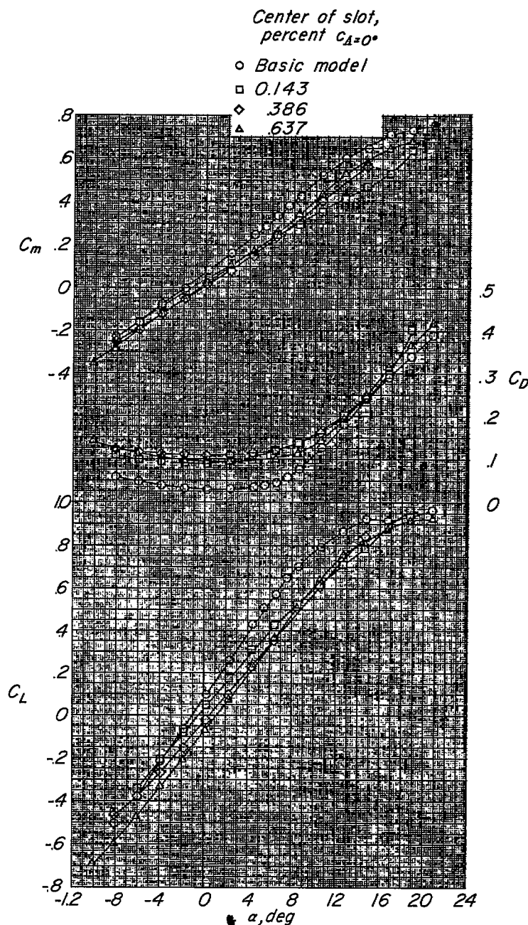
Figure 12.- Longitudinal aerodynamic characteristics of the high-aspect-ratio model with spoiler-slot-deflector. \delta_d = -0.075c ; \delta_s = -0.075c ; \frac{y_1}{b/2} = 0.29 ; \frac{y_0}{b/2} = 0.49 ; slot width, 0.097c ; \Lambda=0^\circ .
