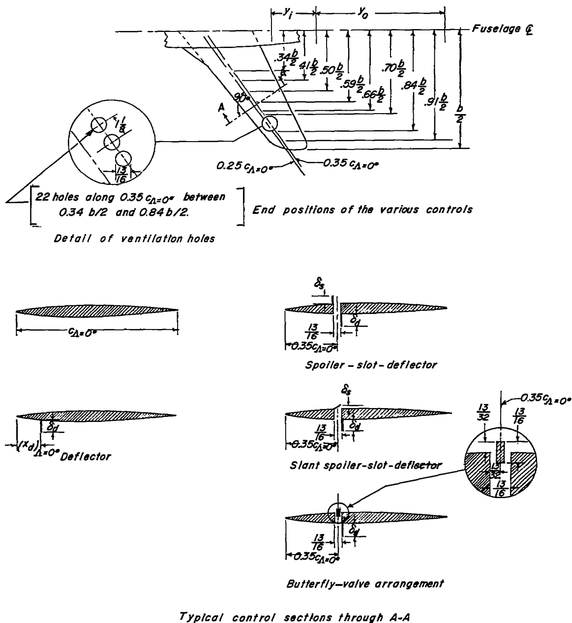
Figure 2.- Detail of controls on the 1/4-scale model of the Bell X-5 airplane. (All dimensions are in inches unless otherwise noted.)
