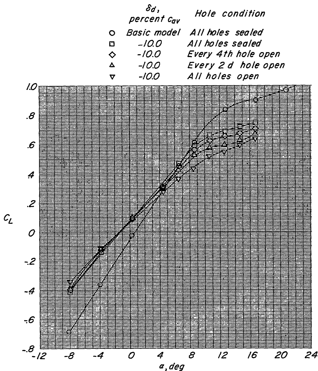
Figure 7.- Effect of ventilation on the lift-curve slope of the 1/4-scale model of the X-5 airplane with deflector. \frac{(x_d)_{\Lambda=0^\circ}}{c_{\Lambda=0^\circ}} = 3.5 ; \frac{y_1}{b/2} = 0.34 ; \frac{y_o}{b/2} = 0.84 ; i_t = -5^\circ .
