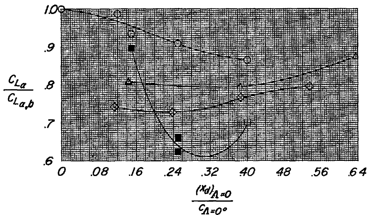
Figure 3.- Variation of lift-curve-slope reduction with chordwise location for deflector on the 1/4-scale model of the X-5 airplane and for deflector and spoiler-slot-deflector on the high-aspect-ratio model. Solid symbols indicate nonlinear lift curves.
