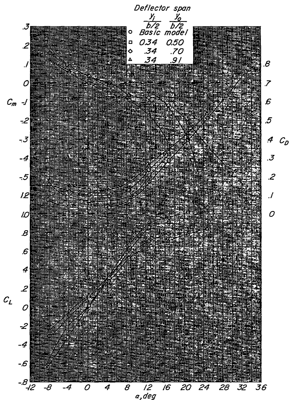
Figure 21.- Longitudinal aerodynamic characteristics of the 1/4 -scale model of the X-5 airplane with deflectors. \delta_d = -0.15c_{av} ;
