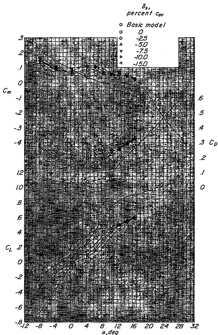
Figure 24.- Longitudinal aerodynamic characteristics of the 1/4-scale model of the X-5 airplane with spoiler-slot-deflector. \delta_d = -0.15c_{av} ; \frac{(x_d)_{\Lambda=0^\circ}}{c_{\Lambda=0^\circ}} = 0.35 ; \frac{y_1}{b/2} = 0.34 ; \frac{y_0}{b/2} = 0.84 ; i_t = -5^\circ .
