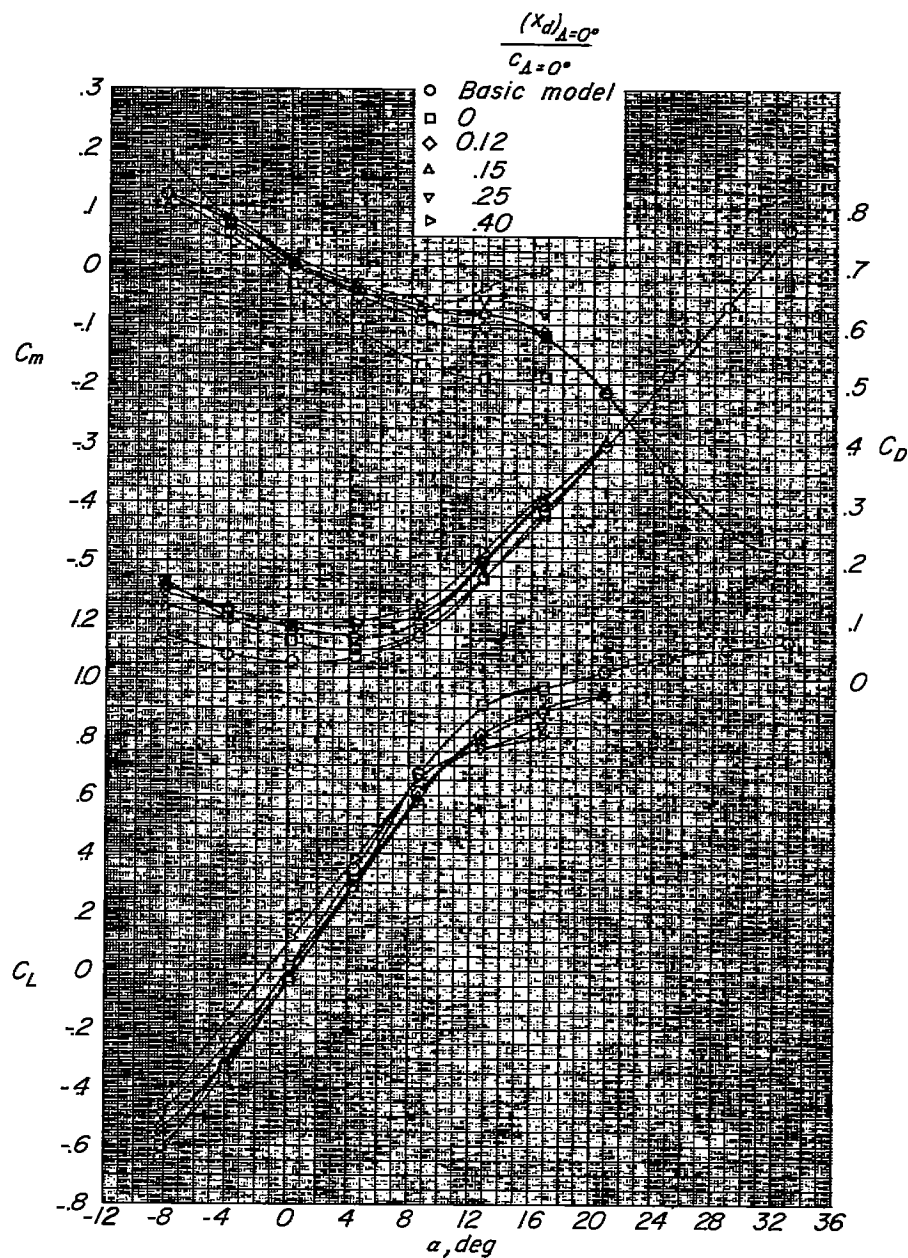
Figure 9.- Longitudinal aerodynamic characteristics of the 1/4-scale model of the X-5 airplane with deflectors. \delta_d = -0.075c_{av} ; \frac{y_1}{b/2} = 0.34 ; \frac{y_o}{b/2} = 0.91 ; i_t = -3/4^\circ .
