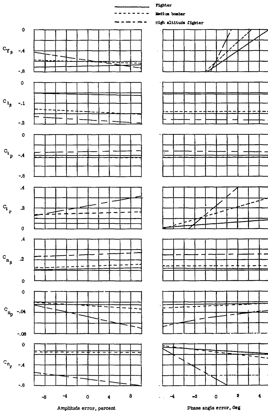
Figure 10.- Variation of the stability derivatives produced by errors in the amplitude and phase angle of \beta .
