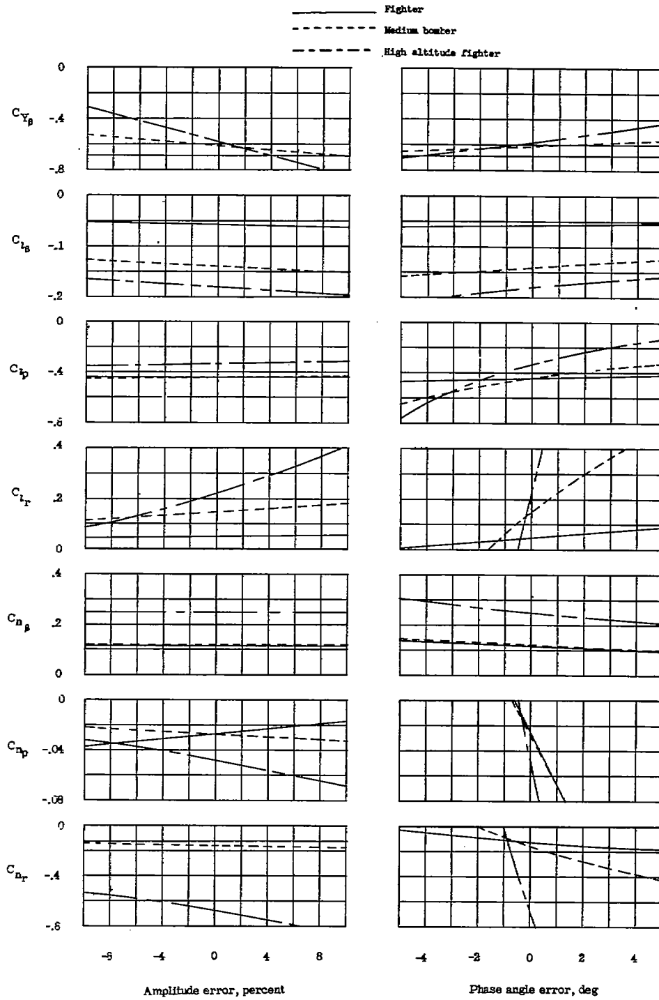
Figure 5.- Variation of the stability derivatives produced by errors in the amplitude and phase angle of the Dutch roll ratio D\phi/\beta .
