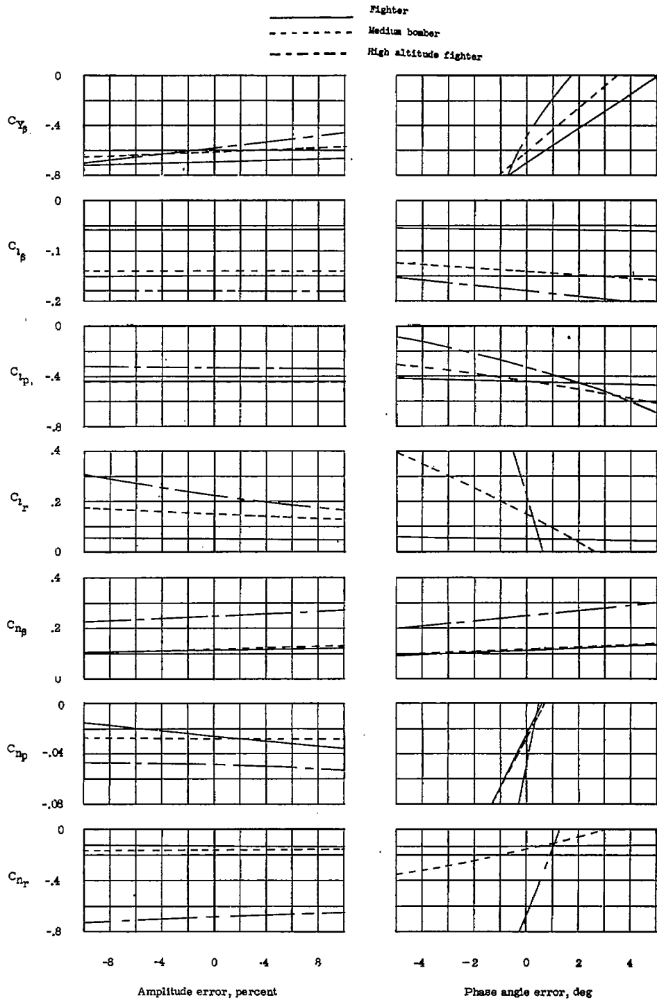
Figure 6.- Variation of the stability derivatives produced by errors in the amplitude and phase angle of the Dutch roll ratio D\psi/\beta .
