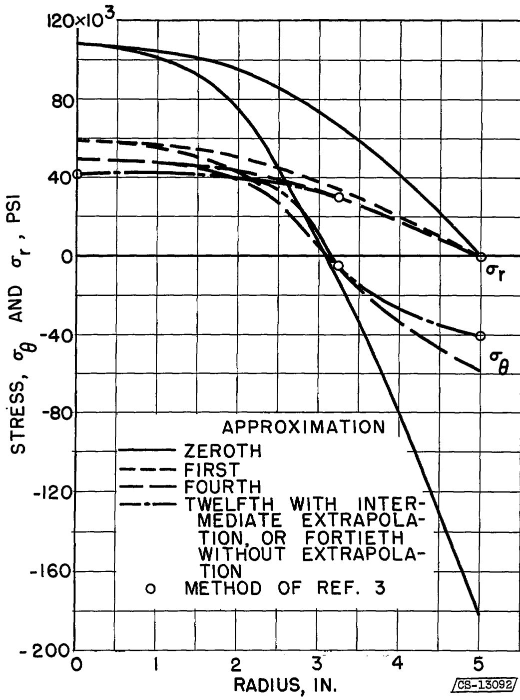
(b) Stress.
