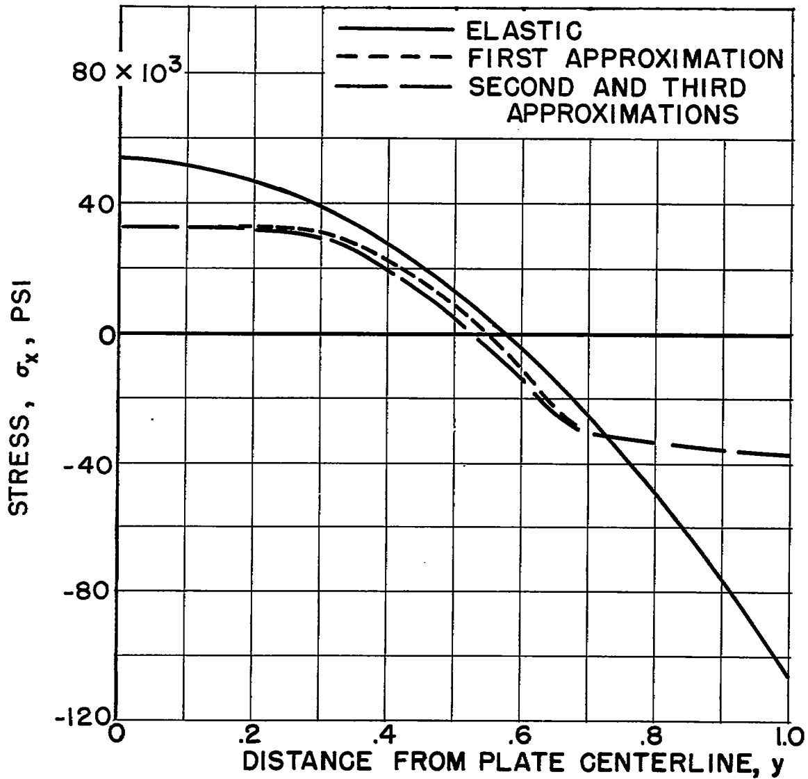
(b) Stress.
