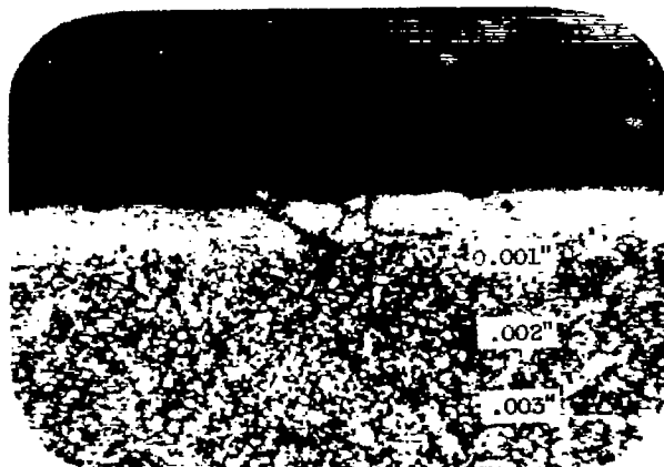
(c) Longitudinal section; X500; 210 \times 10^6 stress cycles.
