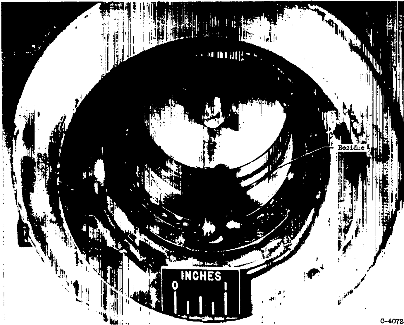
Figure 6. - Viscous residue formed when running with a sebacate at 450° F.
