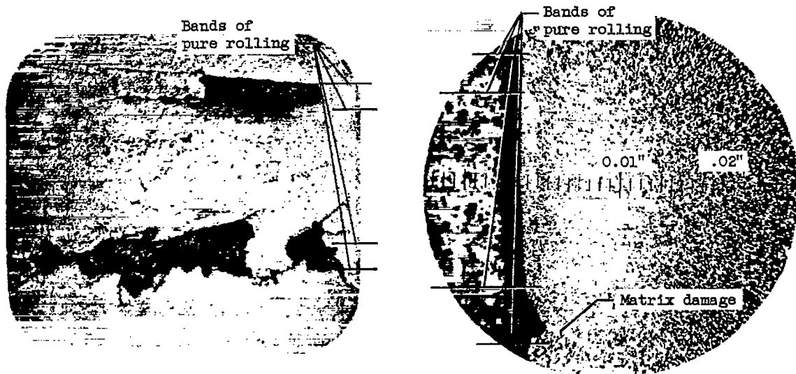
(a) Track surface; X75; spalling along bands of pure rolling.
