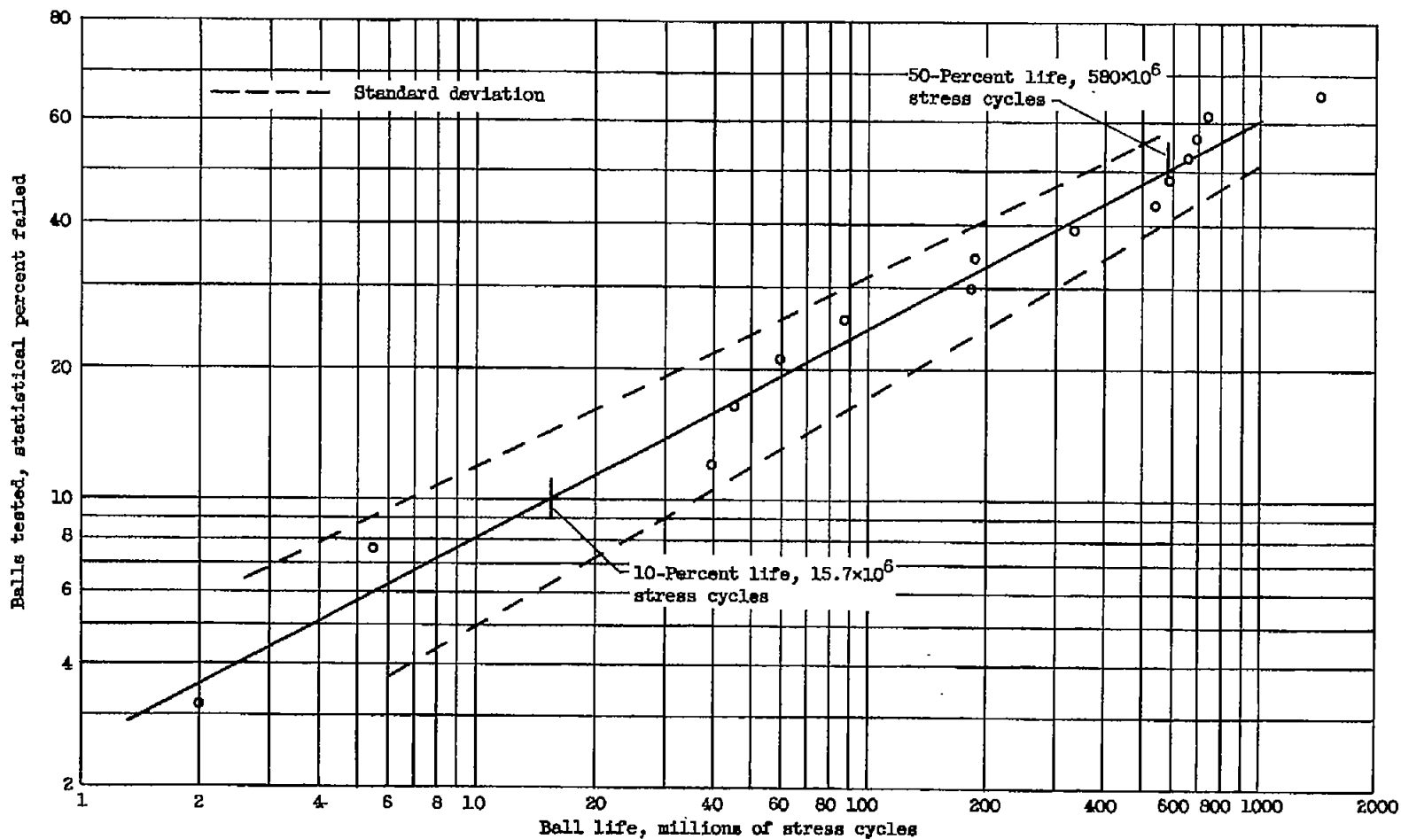
Figure 2. - Fatigue life for 1/2-inch AISI M-1 balls. Lubricant, di(2-ethylhexyl)sebacate; test temperature, 100° F; maximum Hertz compressive stress, 650,000 pounds per square inch.
