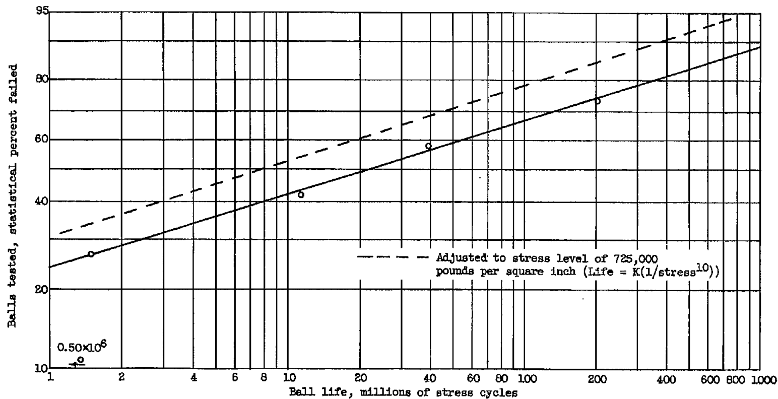
Figure 9. - Concluded. Fatigue life for 1/2-inch AISI M-1 balls. Test temperature, 450° F.
