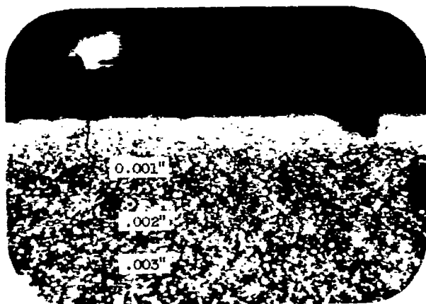
(a) Longitudinal section; X500; 53 \times 10^6 stress cycles.
