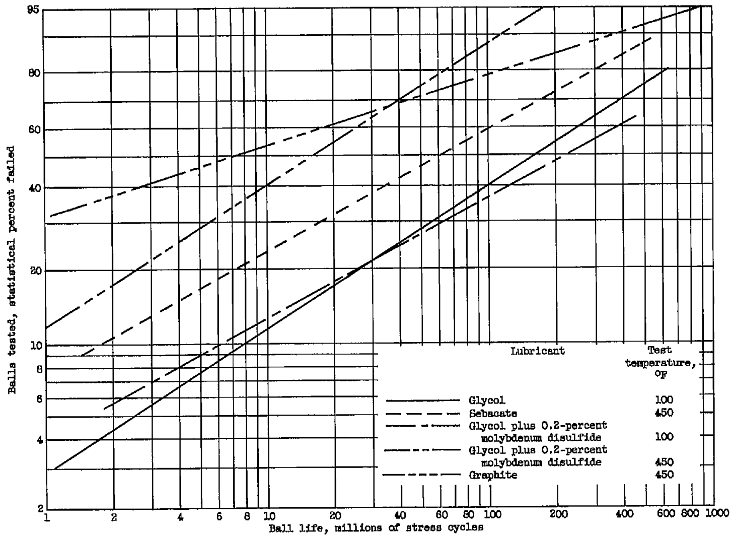
Figure 10. - Fatigue life for 1/2-inch AISI M-1 balls with various lubricants. Maximum Hertz compressive stress, 725,000 pounds per square inch.
