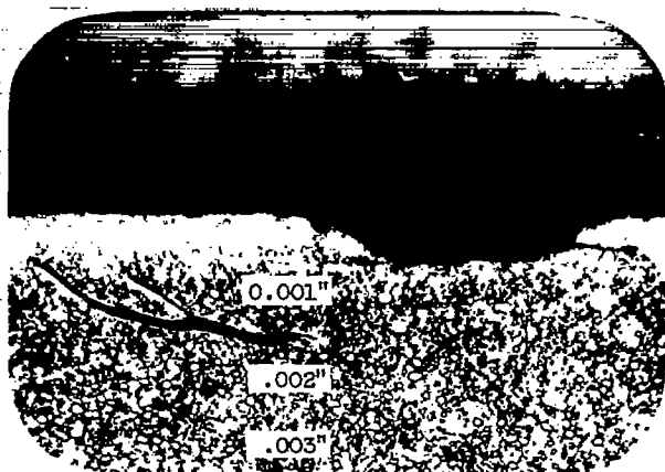
(e) Longitudinal section; X500; 330 \times 10^6 stress cycles.
