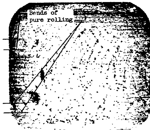
(b) Ball surface; X75; 53 \times 10^6 stress cycles.
