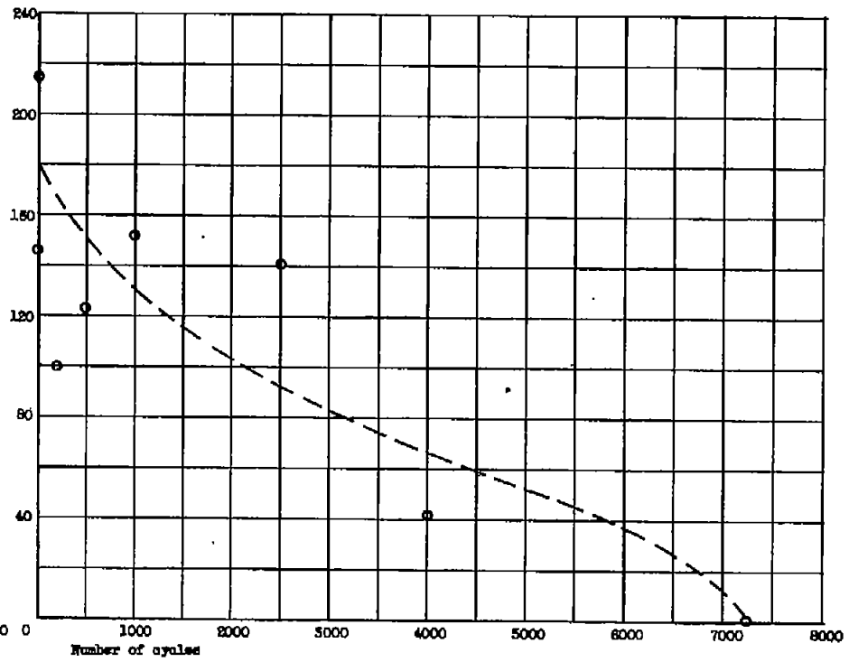
(b) Inconel 650 at 56,500 psi.
