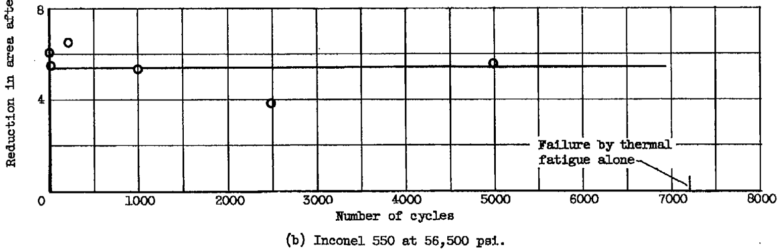
Figure 10. - Effect of prior thermal cycling with 60 seconds at maximum temperature on stress-rupture ductility at 1350° F. Maximum cycling temperature, 1350° F; minimum cycling temperature, 200° F; 30 seconds of heating, 60 seconds at 1350° F, 30 seconds of cooling; 15 seconds at 200° F.
