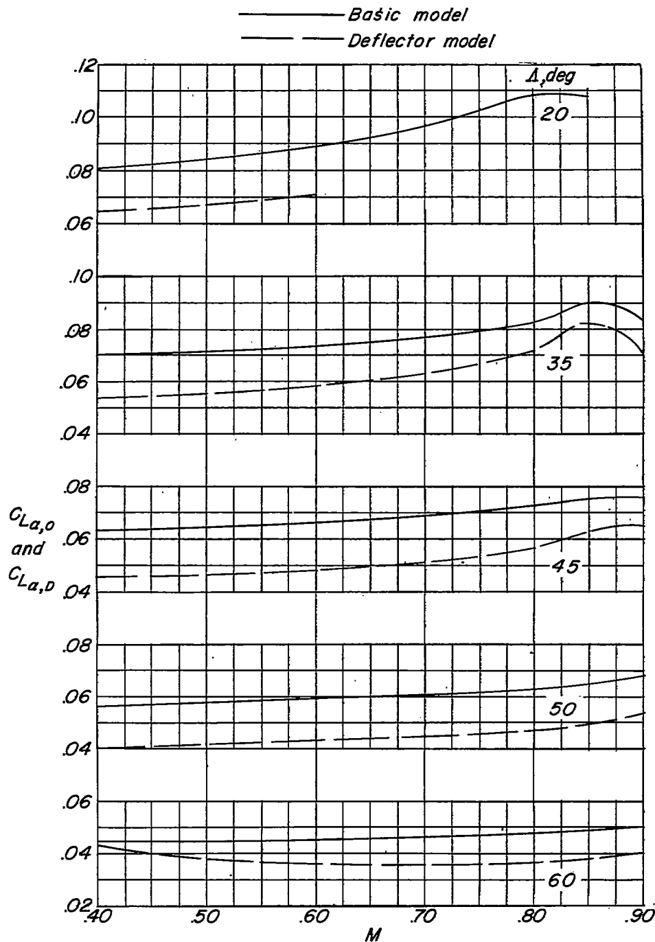
Figure 6.- Variation of lift-curve slope with Mach number for the basic model and the model equipped with deflectors (slopes measured at \alpha = 0^\circ ).
