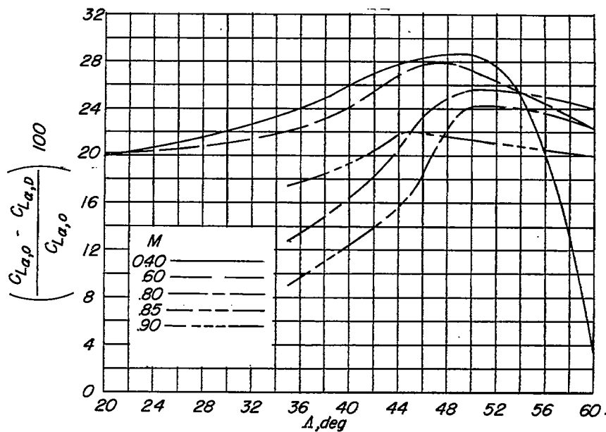
(a) Percent lift-curve-slope reduction as a function of wing sweep.
