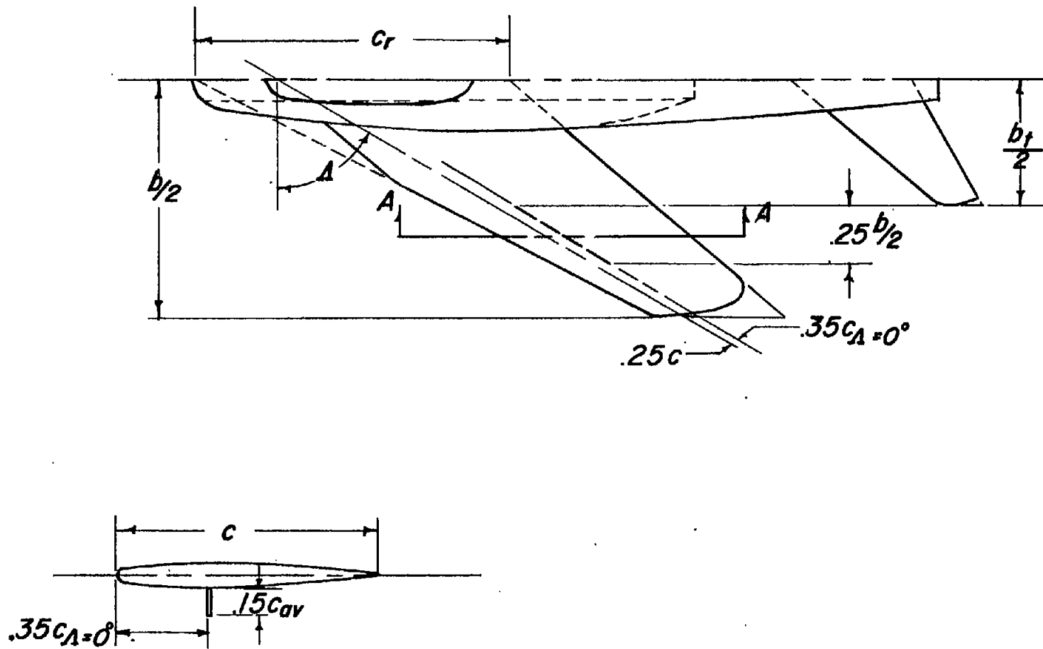
Typical deflector section A-A
