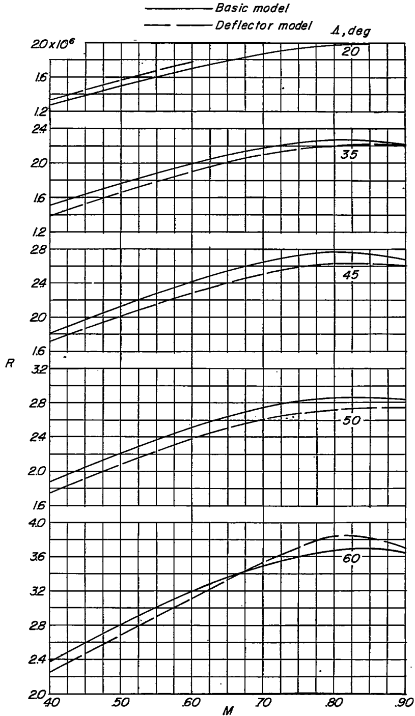
Figure 2.- Variation with Mach number of test Reynolds number based on wing mean aerodynamic chord.
