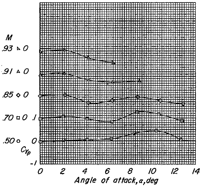
(a) 3.6-4-.6-006 wing.
