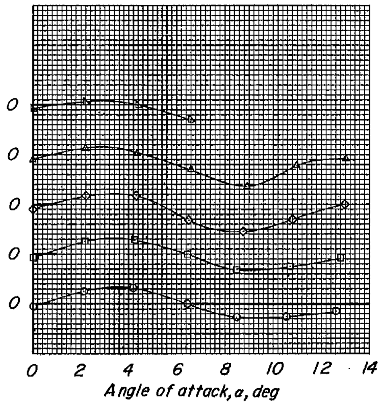
(b) 32.6-4-.6-006 wing.
