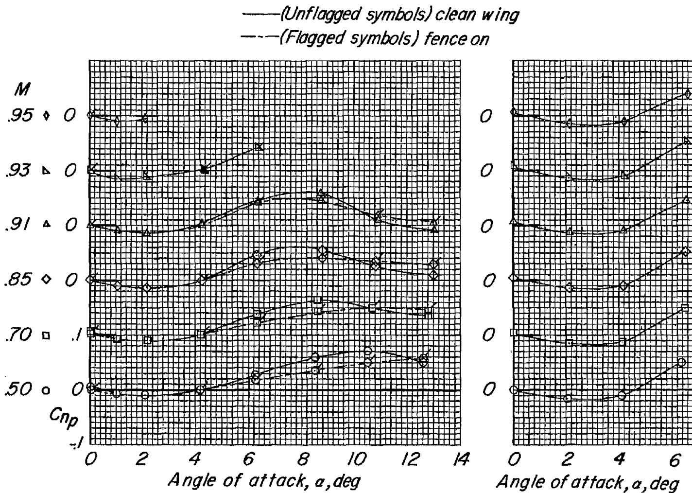
(c) 45-4-.6-006 wing.
