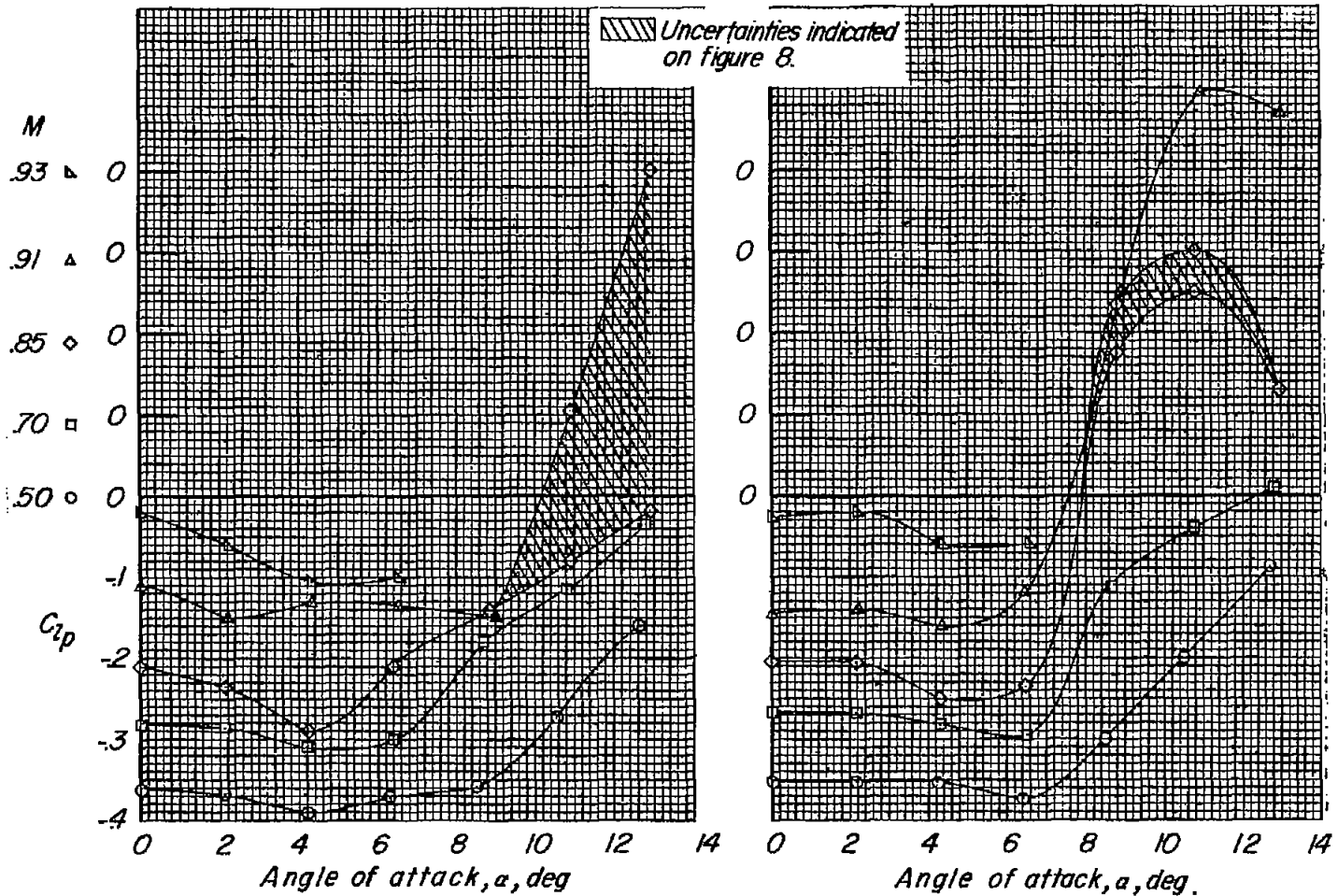
(a) 3.6-4-.6-006 wing.
