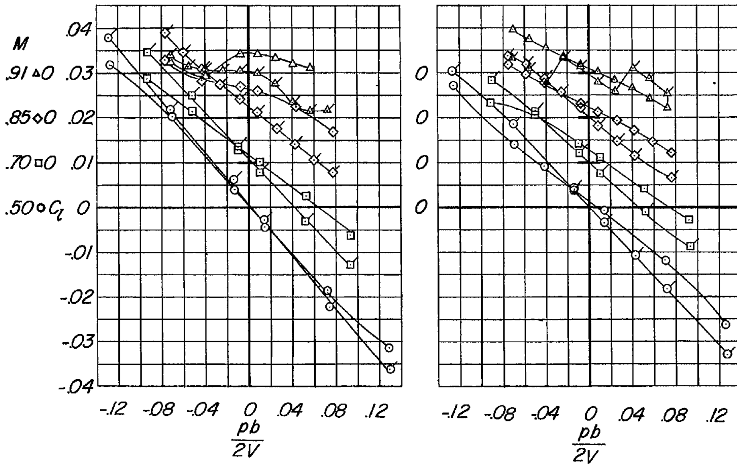
(c) 45-4-.6-006 wing.
