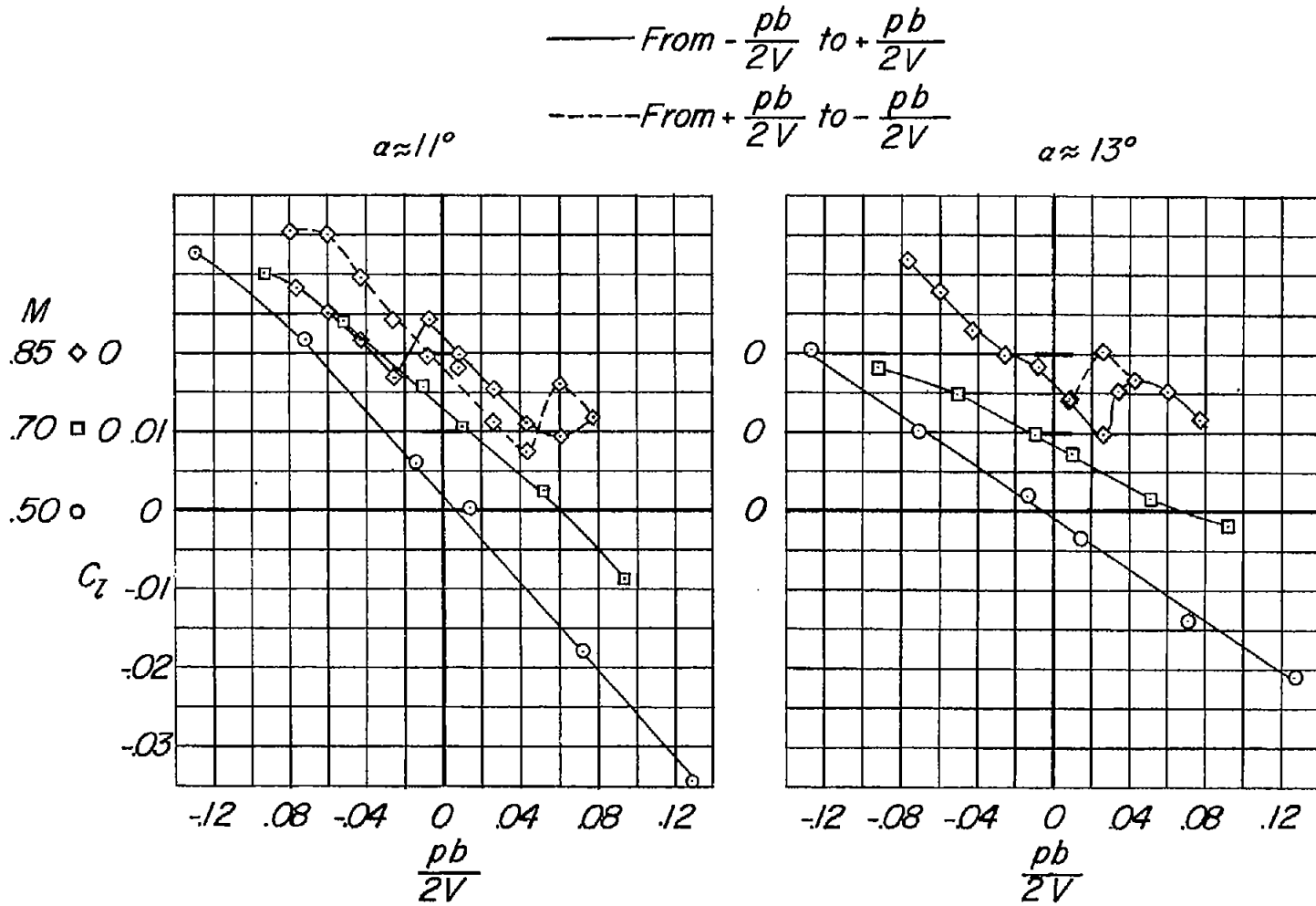
(a) 3.6-4-.6-006 wing.
