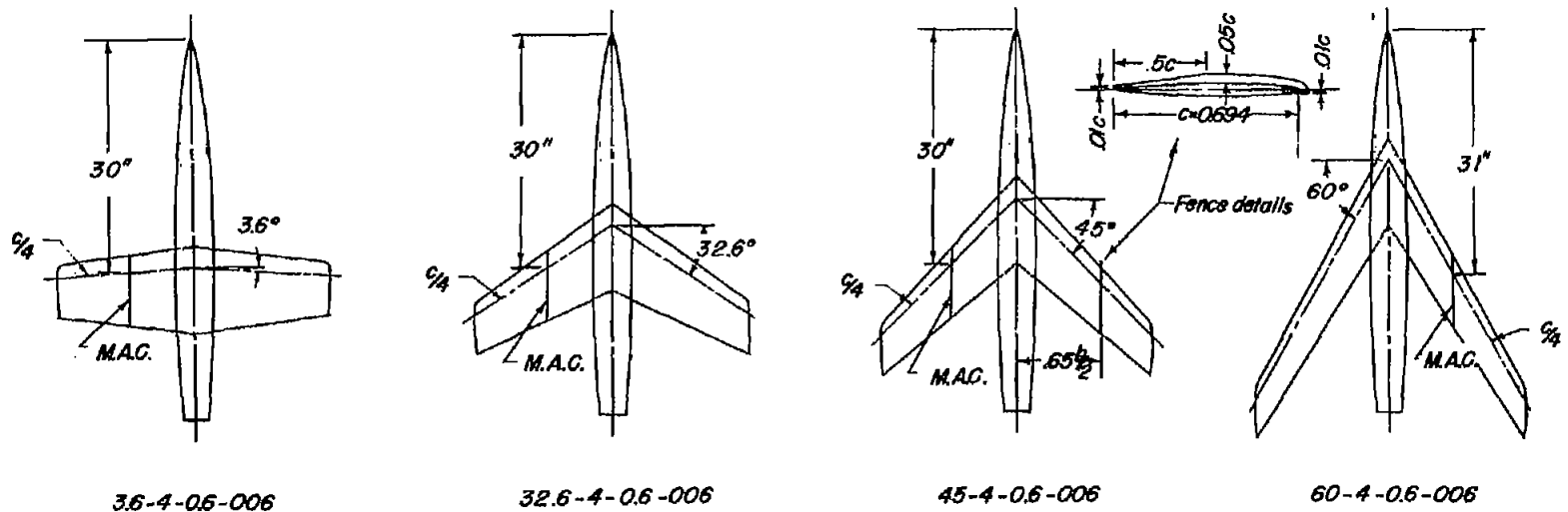
Figure 2.- Sketch of four wing-fuselage configurations.
