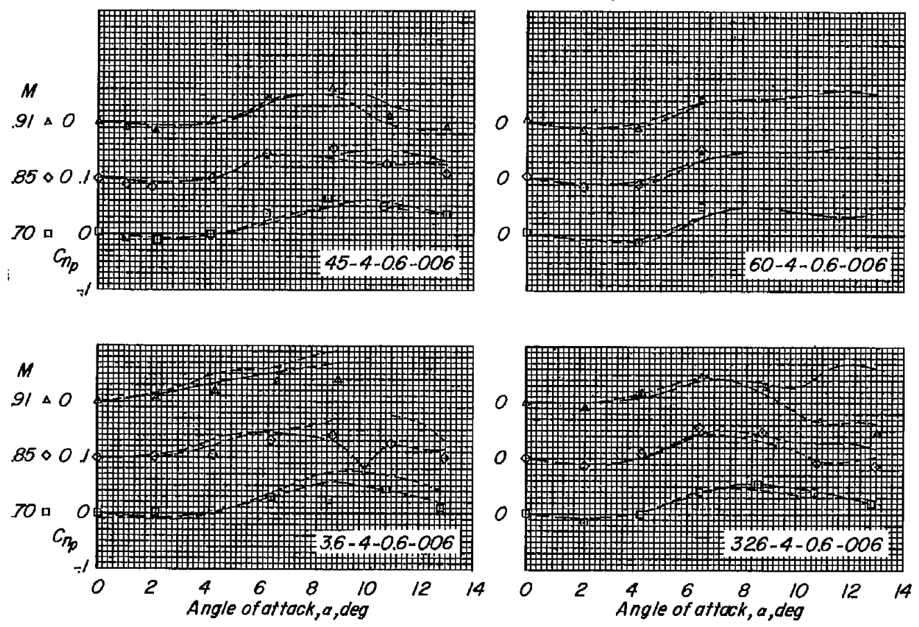
Figure 22.- Comparison of experimental and calculated variation of C_{np} with angle of attack.
