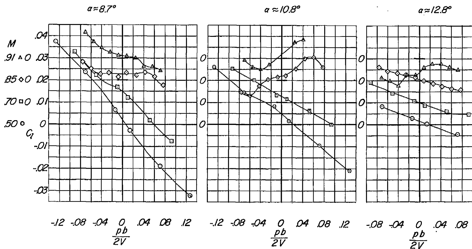
(b) 32.6-4-.6-006 wing.
