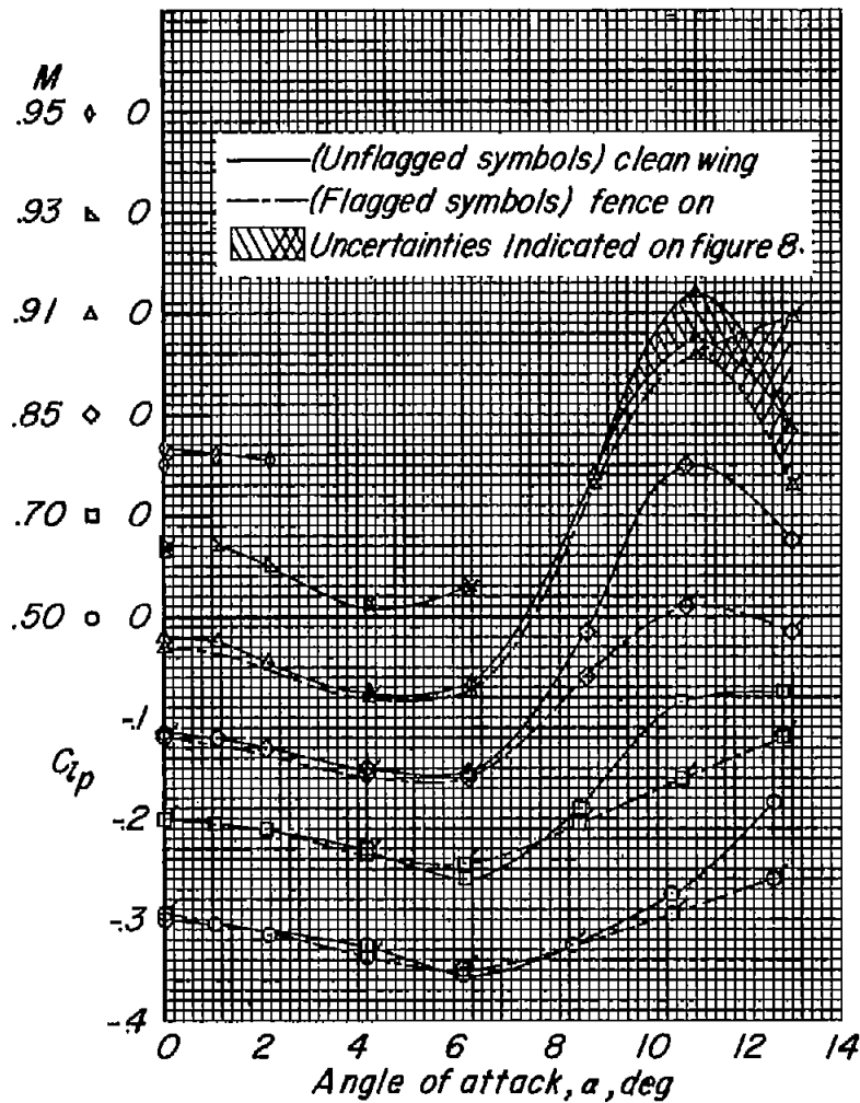
(c) 45-4-.6-006 wing.
