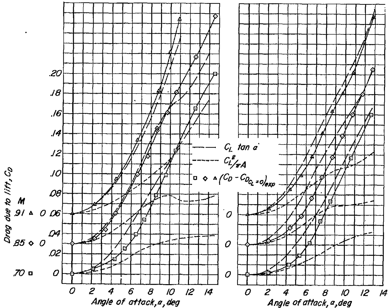
(a) 3.6-4-.6-006 wing.
