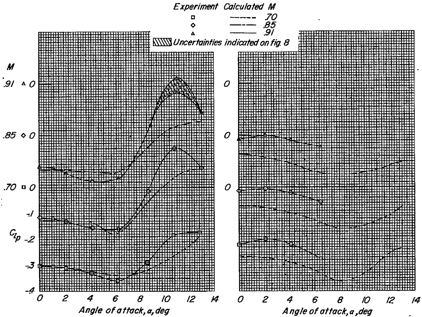
(c) 45-4-.6-006 wing.
