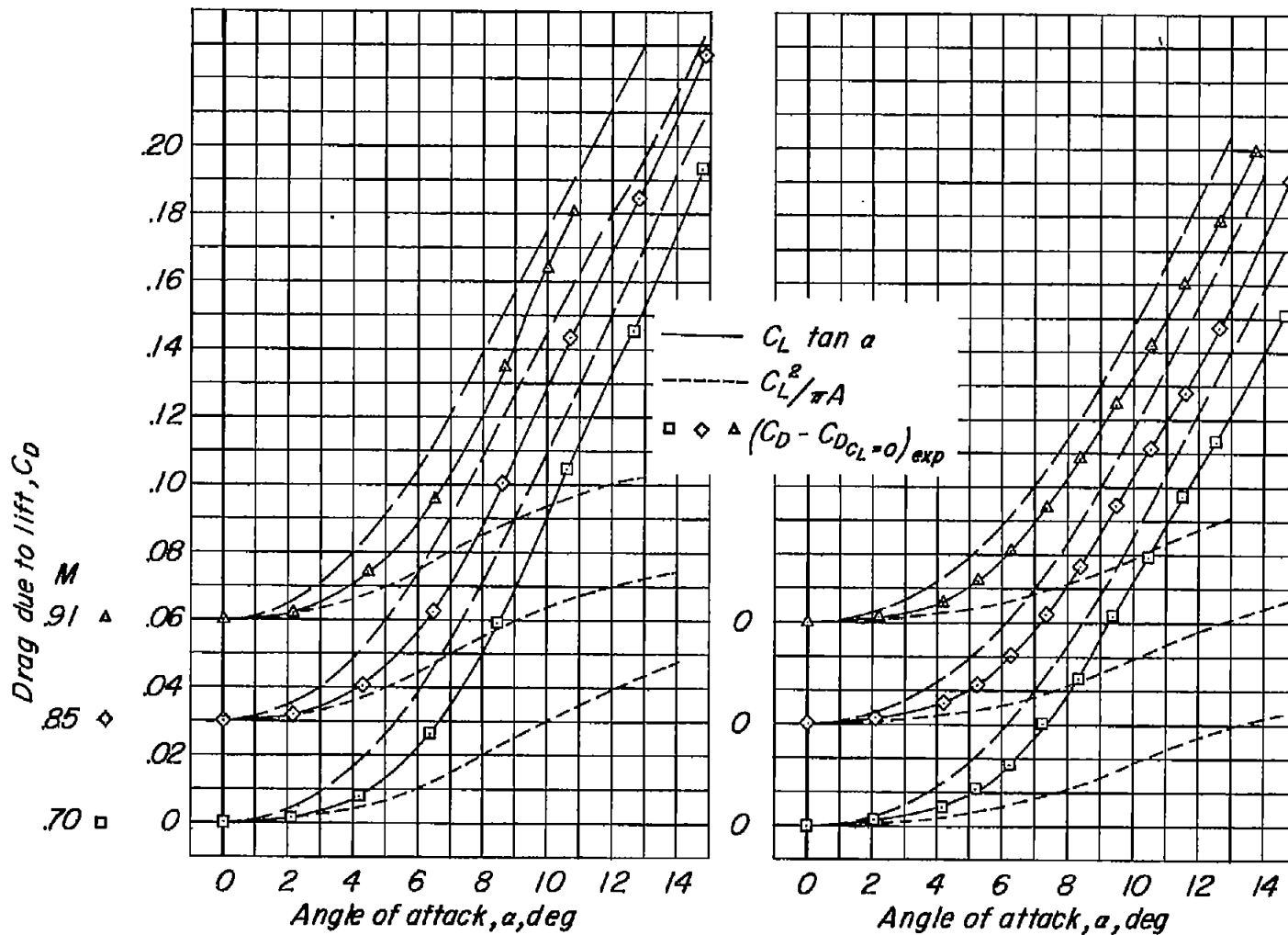
(c) 45-4-.6-006 wing.
