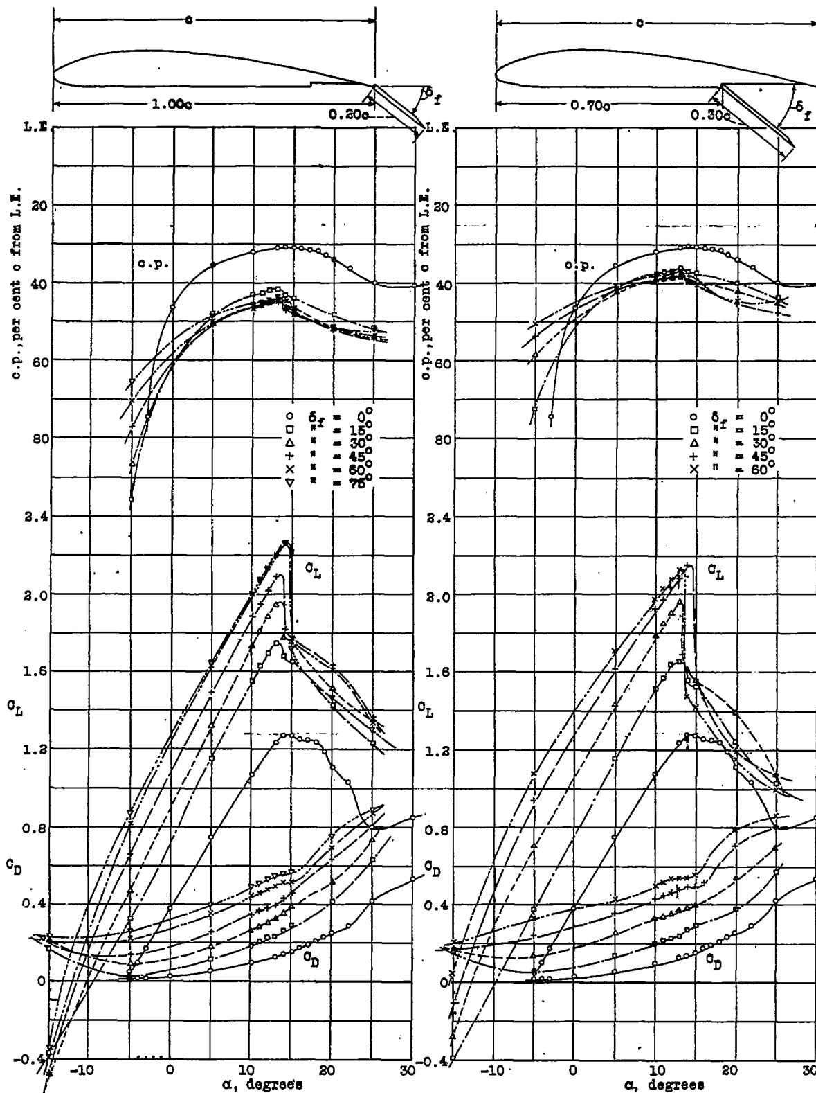
Fig. 4 The 20 per cent c flap hinged at 100 per cent c
