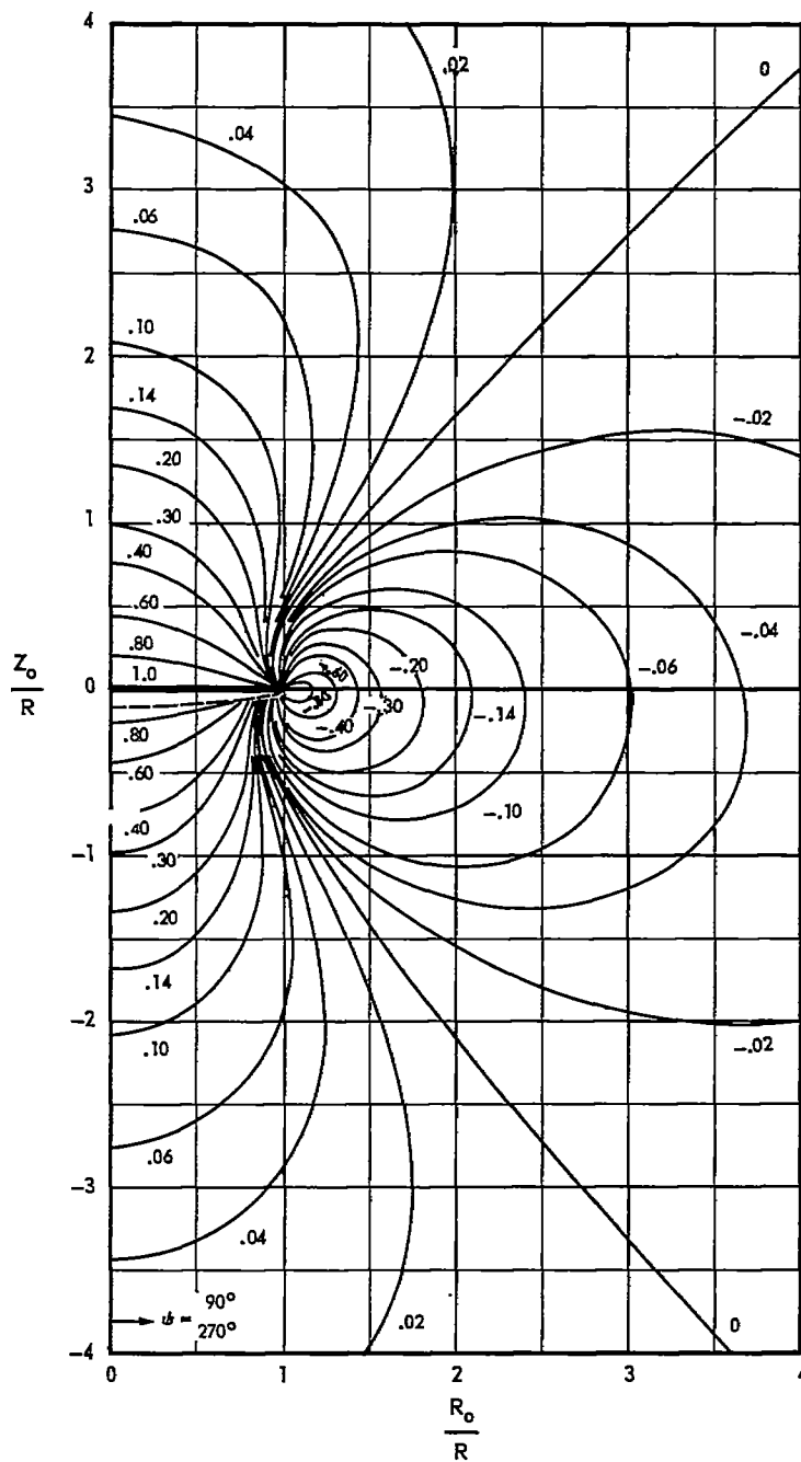
(d) Lines of constant values of V_1/v in lateral plane \psi = 90^\circ and 270^\circ .
