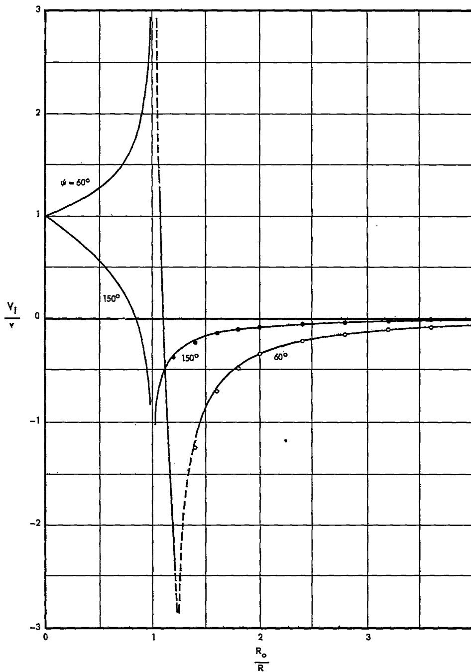
(c) V_1/v in rotor plane for \psi = 60^\circ and 150^\circ .
