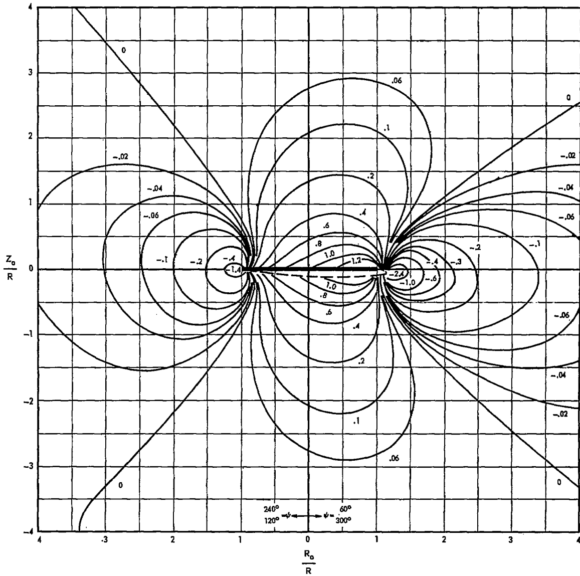
(c) Lines of constant values of V_1/v in azimuth planes \psi = 60^\circ and 240^\circ and \psi = 120^\circ and 300^\circ .
