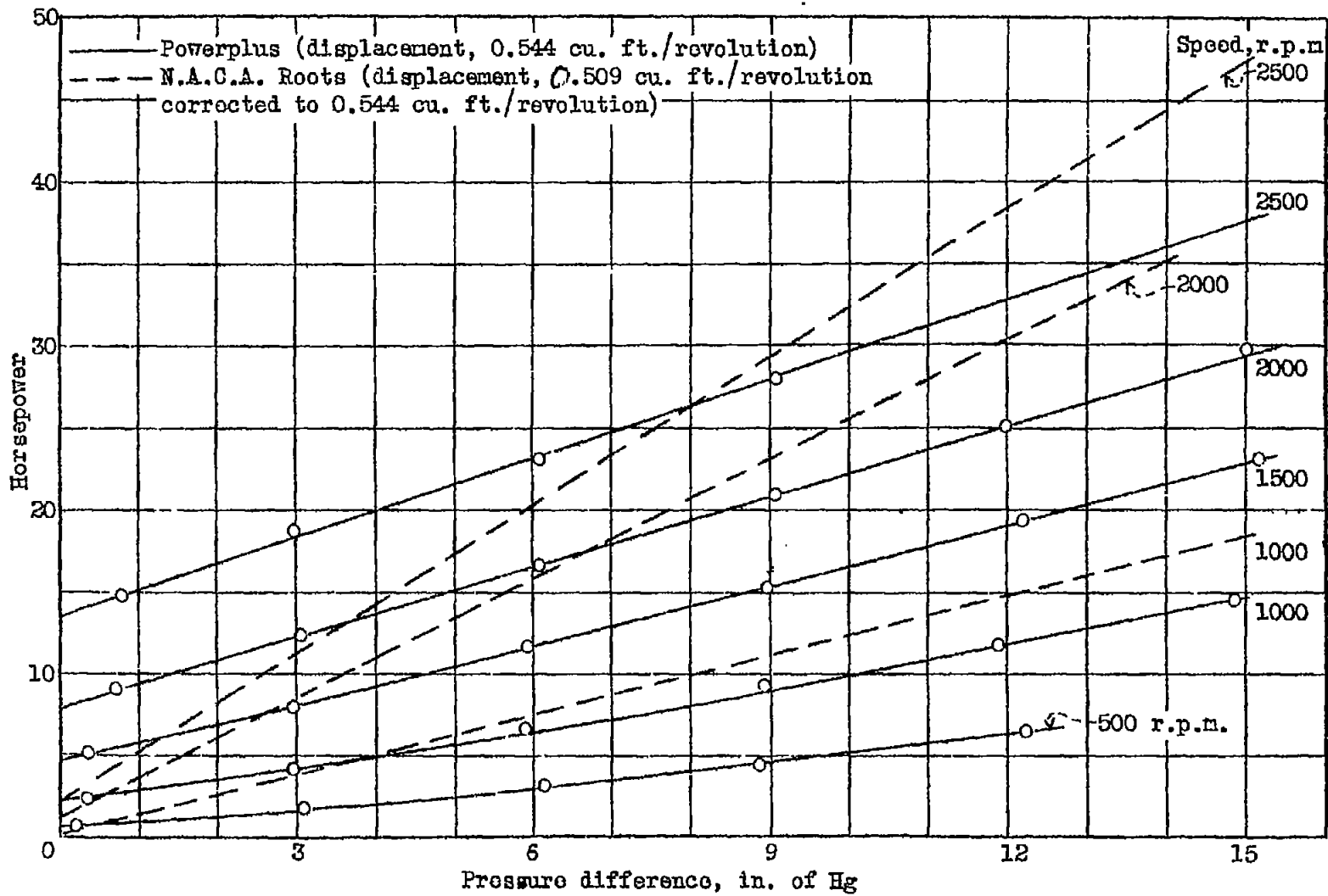
Fig. 7 Horsepower required by Powerplus and N.A.C.A. Roots superchargers at various speeds and pressure differences
