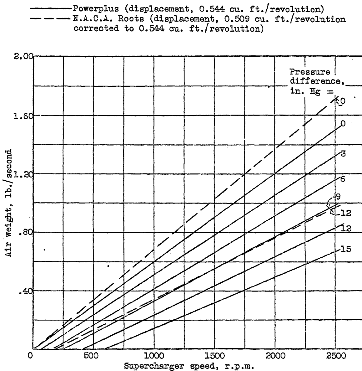
Fig.8 Weight of air delivered by Powerplus and N.A.C.A. Roots superchargers at various speeds and pressure differences. Discharge pressure at sea level.
