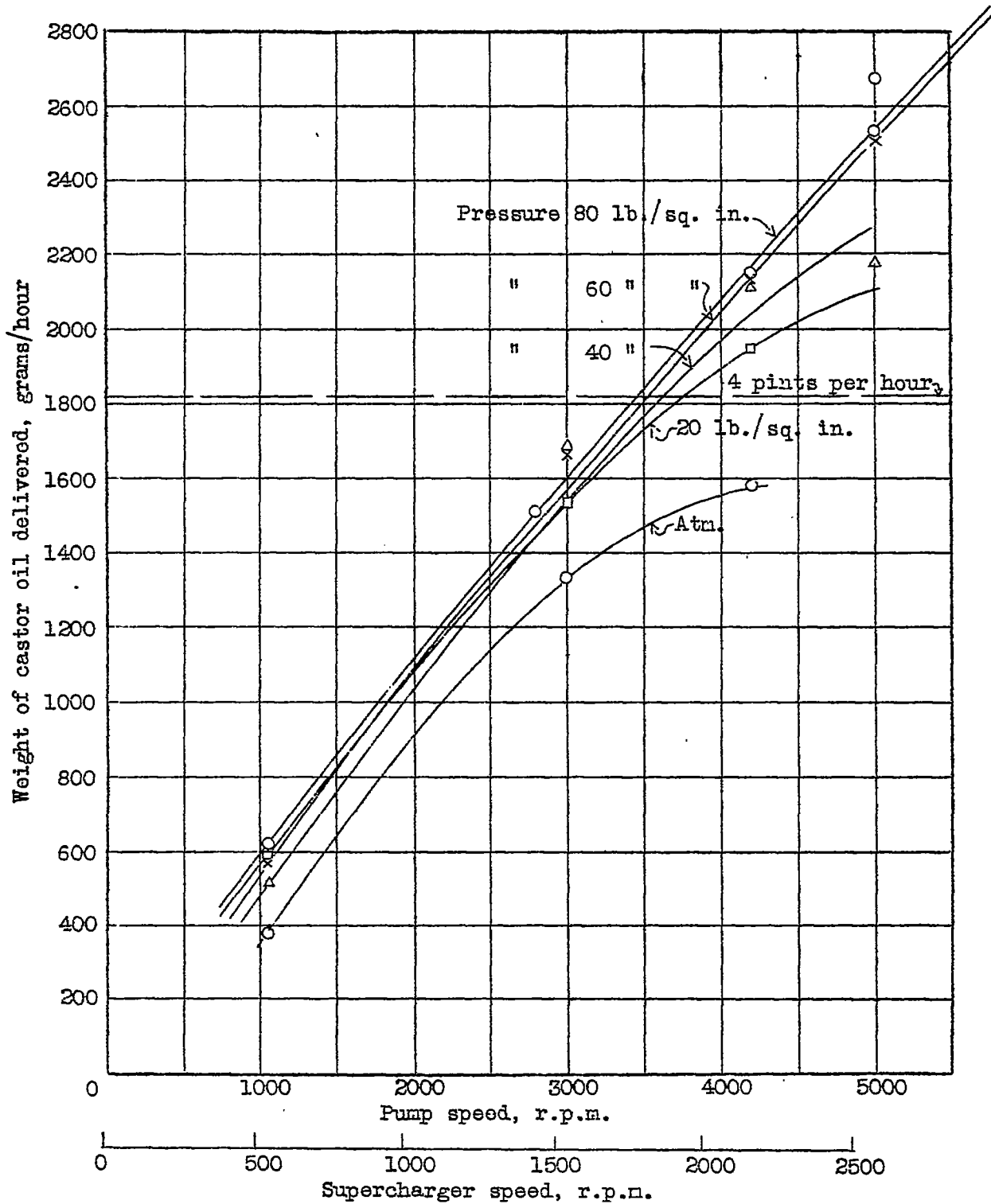
Fig.5 Rate of discharge of Bosch pump at various speeds and with various pressures on supply tank
