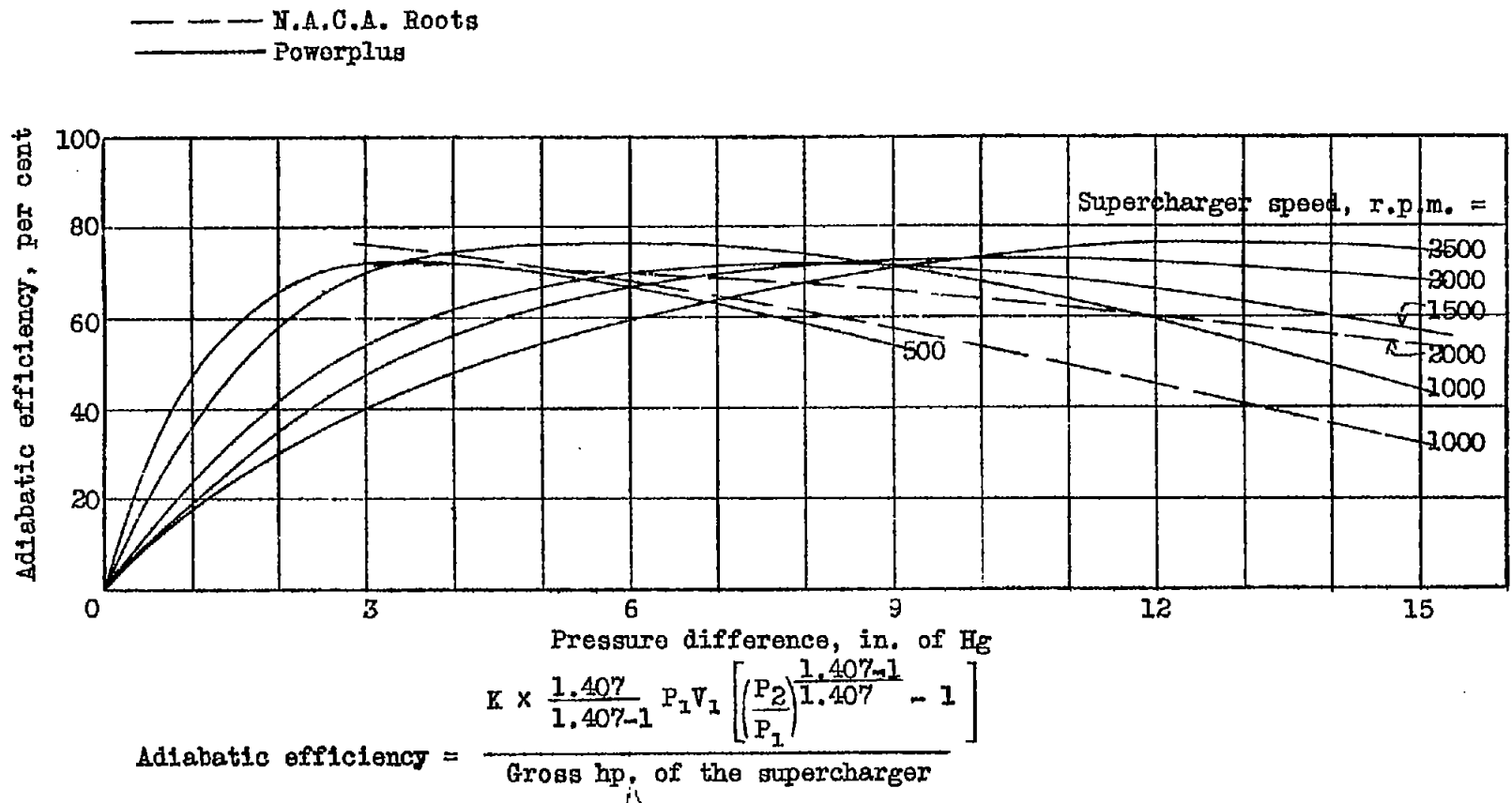
Fig.11 Adiabatic efficiency of Powerplus and N.A.C.A. Roots superchargers at various speeds and pressure differences
