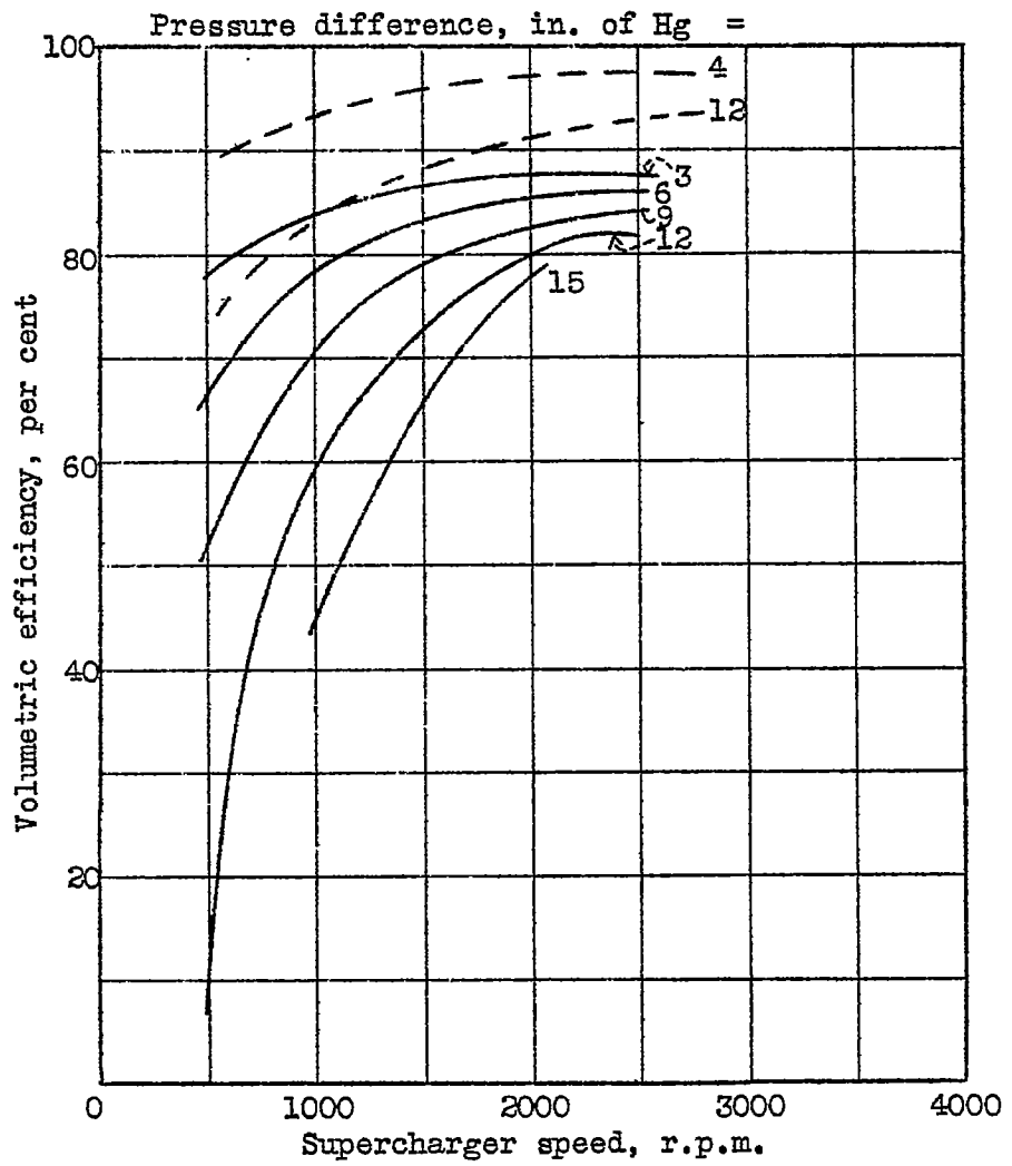
Fig.9 Volumetric efficiency of Powerplus and N.A.C.A. Roots superchargers at various speeds and pressure differences
