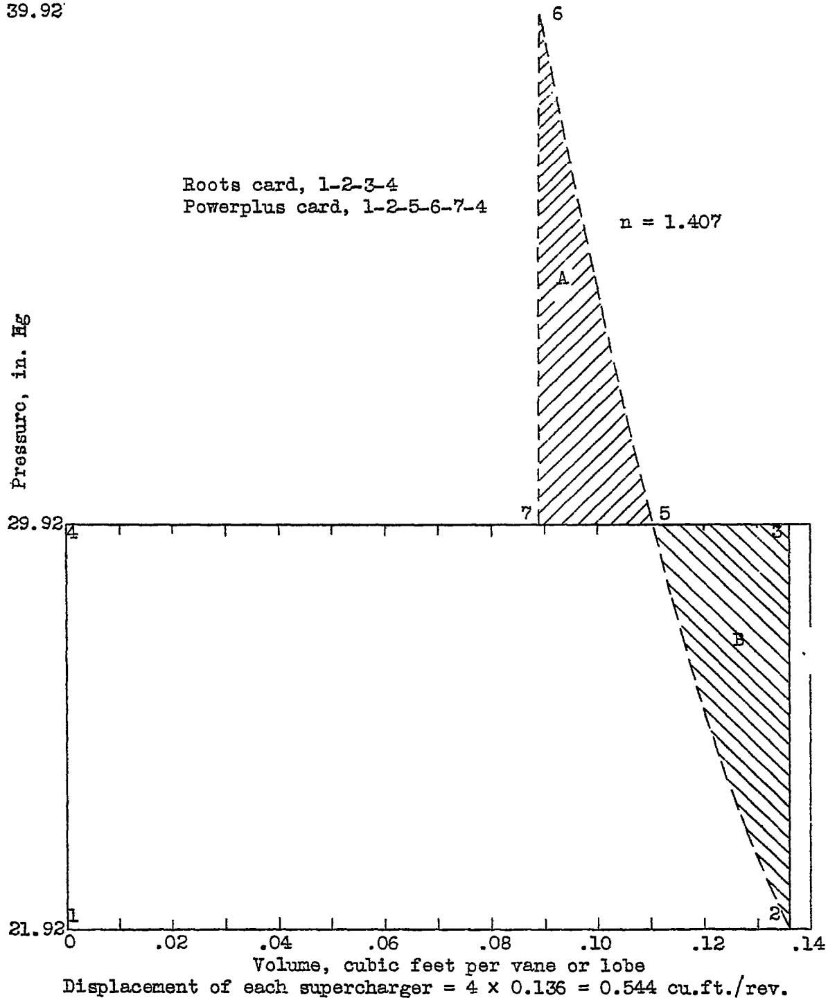
Fig.6 Comparison of pressure-volume cards of Powerplus and N.A.C.A. Roots superchargers neglecting slip
