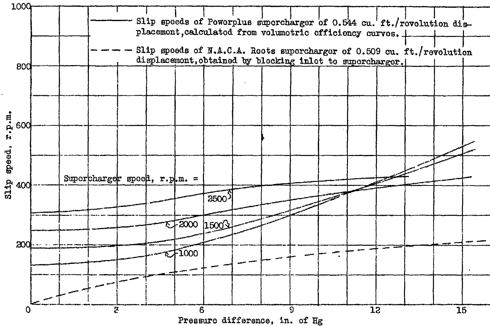
Fig.10 Slip speeds of Powerplus and N.A.C.A. Roots superchargers at various speeds and pressure differences
