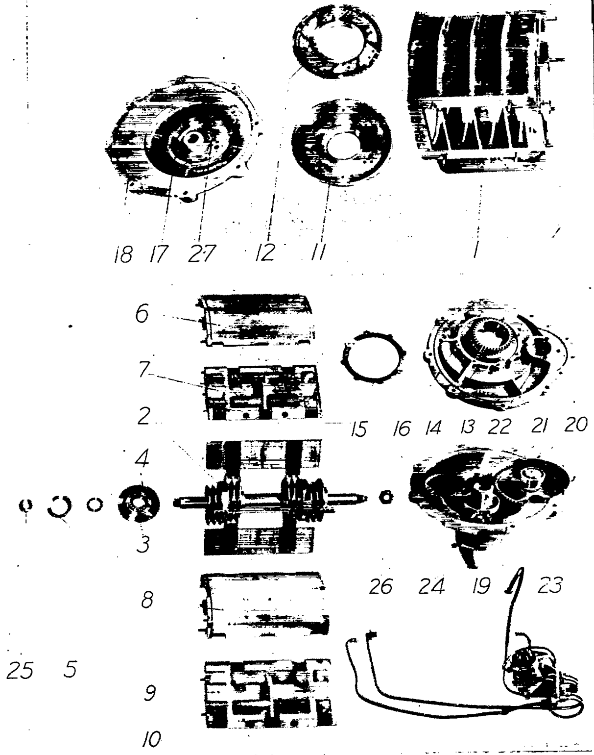
Fig.4 Exploded view of Powerplus vane-type supercharger.
