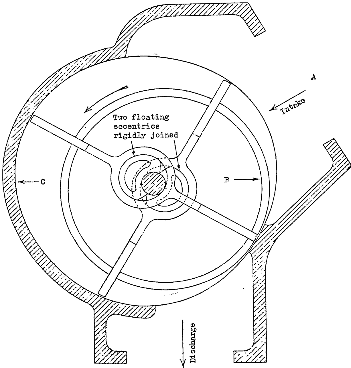
Fig. 3 Sketch of Powerplus vane-type supercharger.
