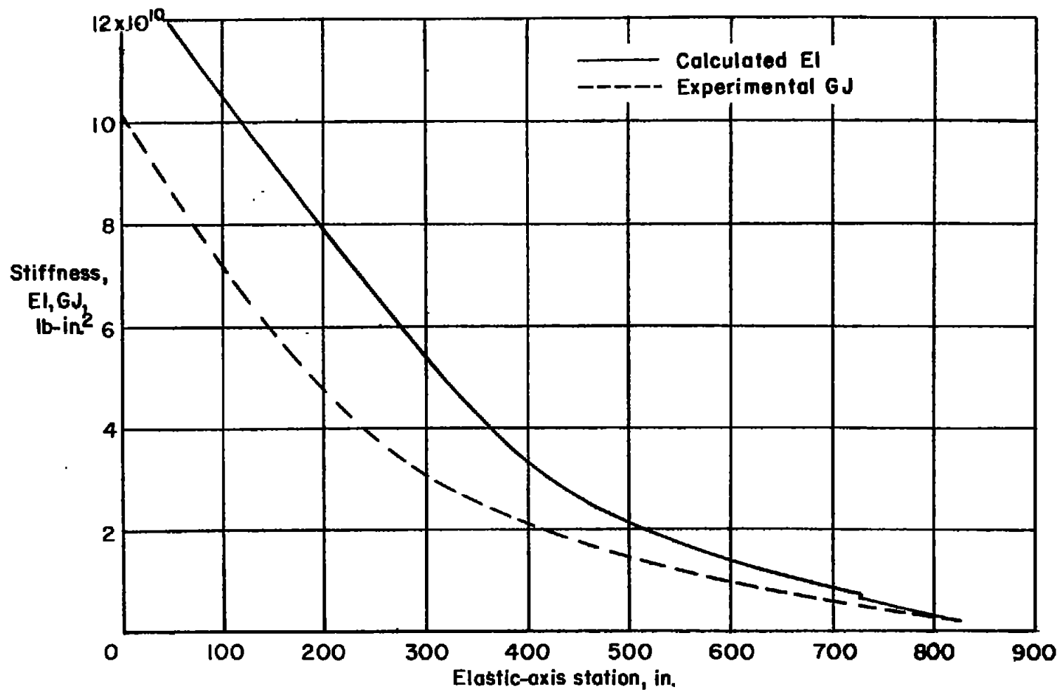
Figure 4.- Bending and torsional stiffness distributions of wing.
