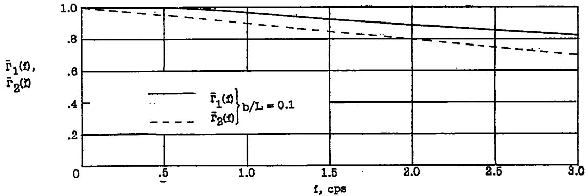
Figure 16.- Span averaging functions \bar{F}_1(f) and \bar{F}_2(f) .
