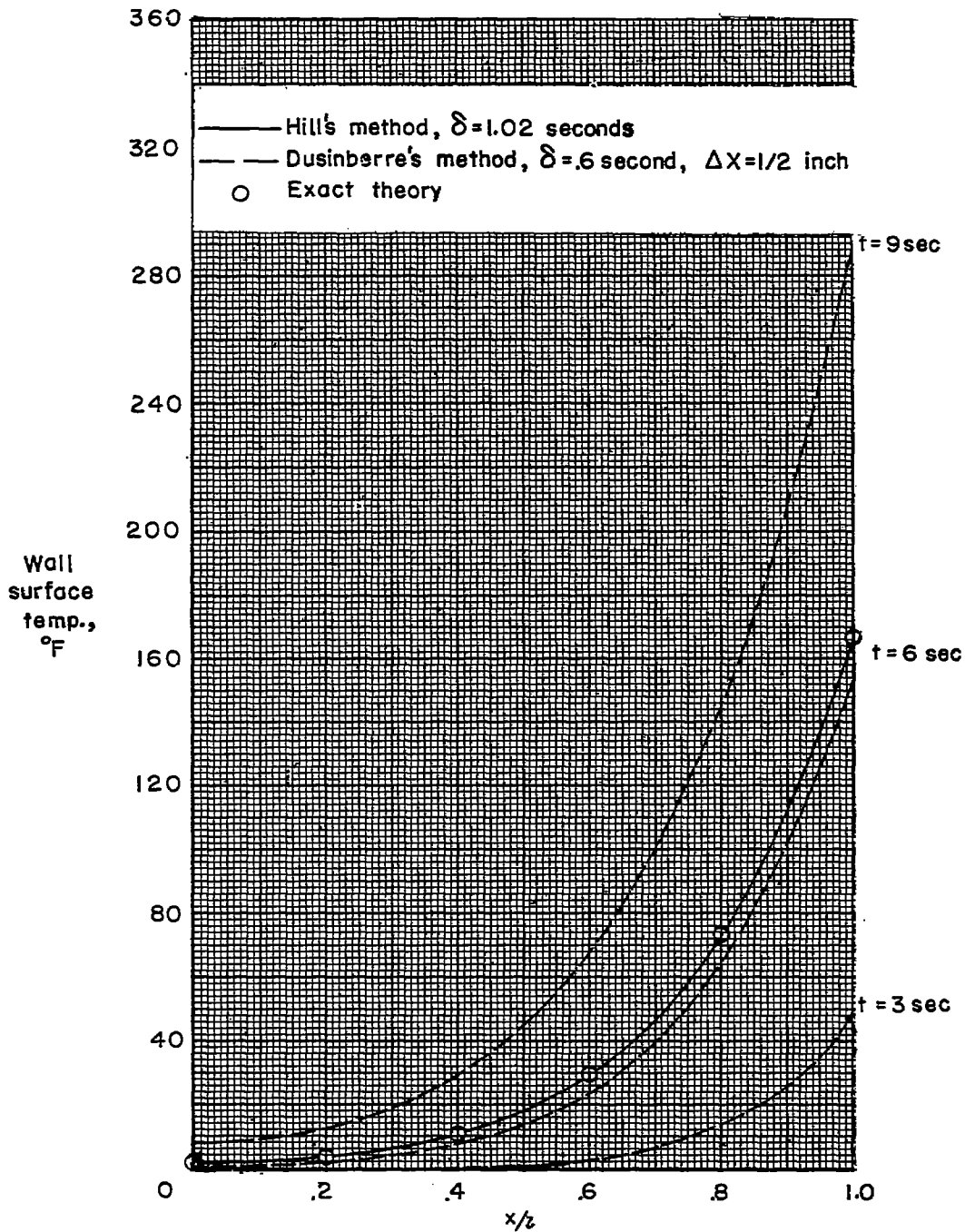
Figure 6.- Case I. Temperature profiles through 3-inch copper wall. Adiabatic-wall temperature varies linearly from 0^{\circ} to 10,000^{\circ} in 10 seconds; h = 100 Btu/(hr)(sq ft)(°F).
