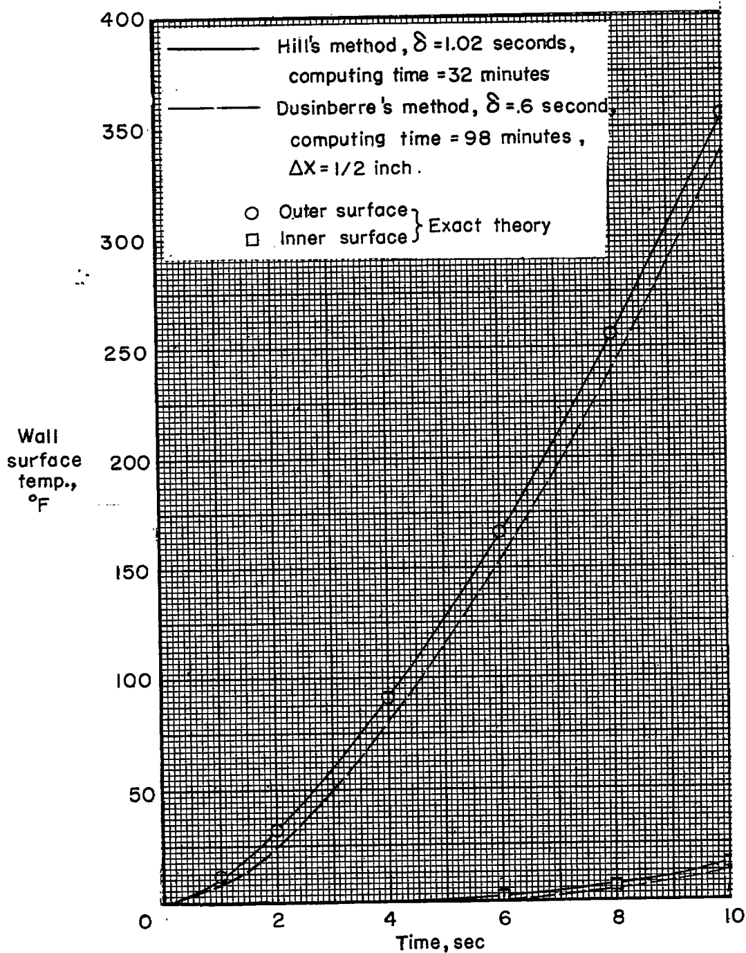
Figure 3.- Case I. Temperatures of 3-inch copper wall surfaces. Adiabatic-wall temperature varies linearly from 0^{\circ} to 10,000^{\circ} in 10 seconds; h = 100 Btu/(hr)(sq ft)( ^{\circ} F).
