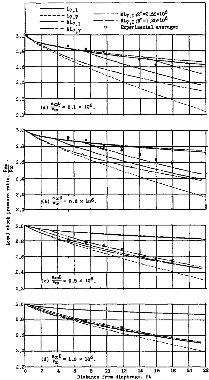
Figure 28.- Comparison of averaged experimental local shock pressure ratios with various theoretical predictions. \frac{p_{\beta 0}}{p_{\infty}} = 3.0 . Flagged and unflagged symbols are used to distinguish between averages from different days.
