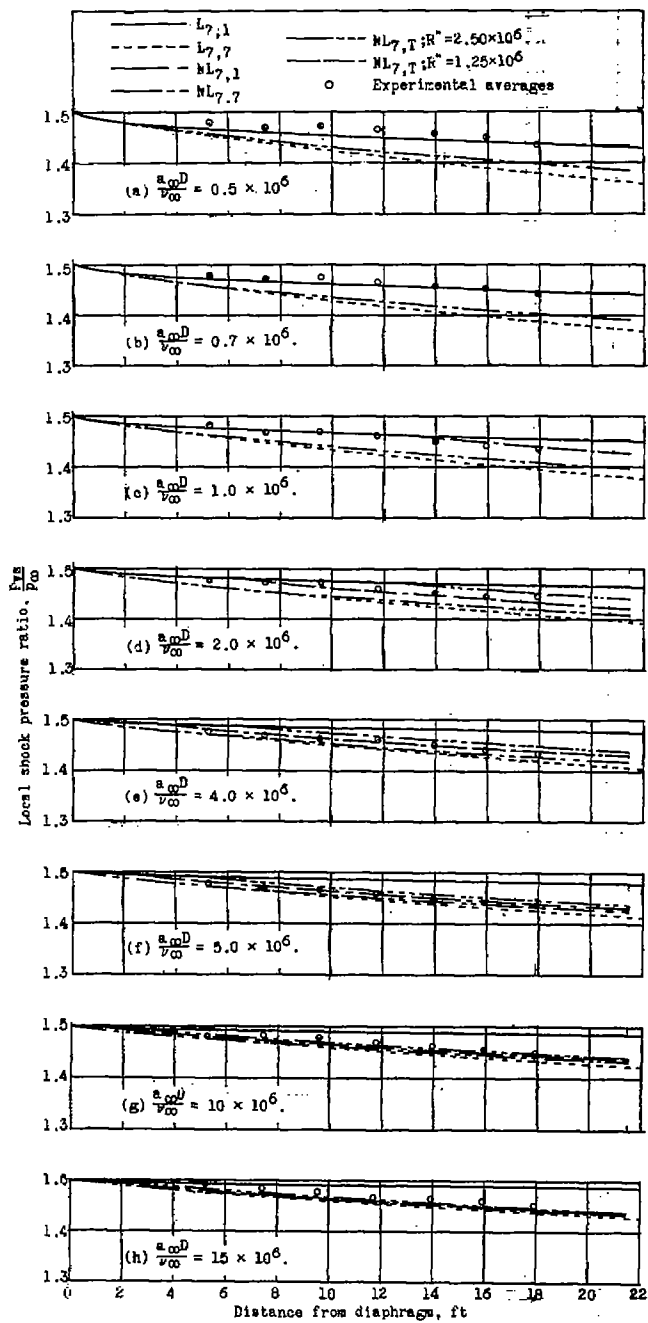
Figure 23.- Comparison of averaged experimental local shock pressure ratios with various theoretical predictions. \frac{P_{B0}}{P_{\infty}} = 1.5 .
