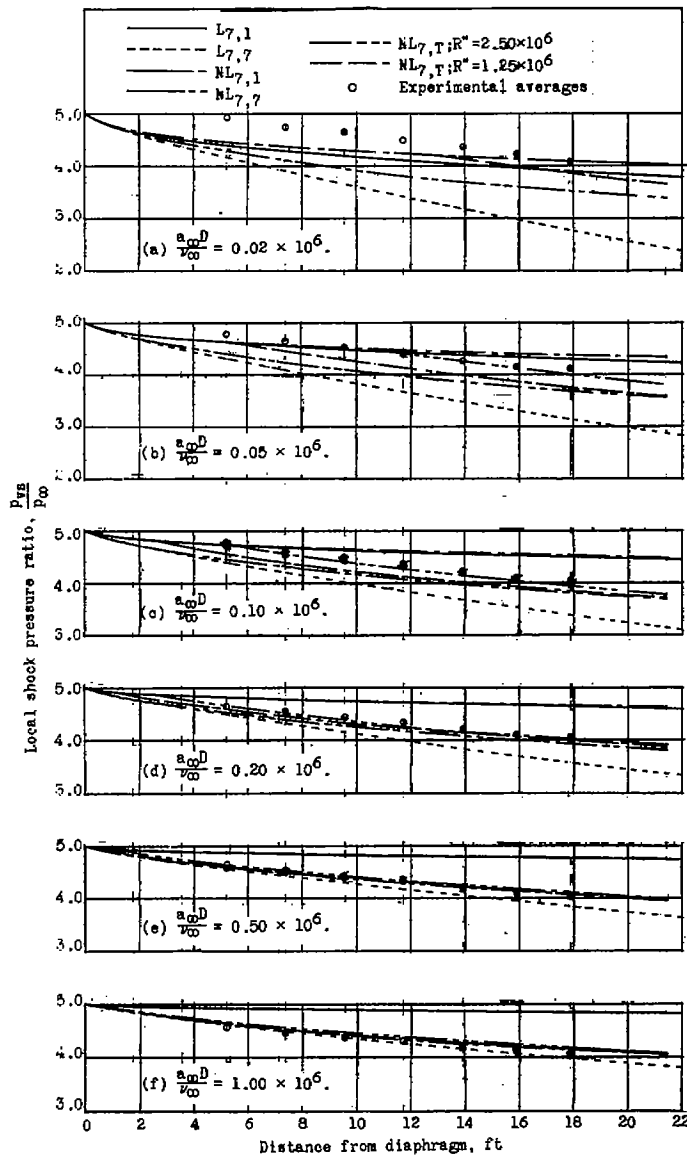
Figure 31.- Comparison of averaged experimental local shock pressure ratios with various theoretical predictions. \frac{P_{\beta 0}}{P_{\infty}} = 5.0 . Flagged and unflagged symbols are used to distinguish between averages from different days.
