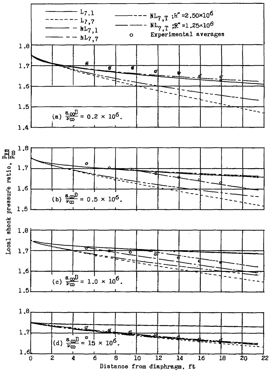
Figure 24.- Comparison of averaged experimental local shock pressure ratios with various theoretical predictions. \frac{p_{\beta 0}}{p_{\infty}} = 1.75 . Flagged and unflagged symbols are used to distinguish between averages from different days.
