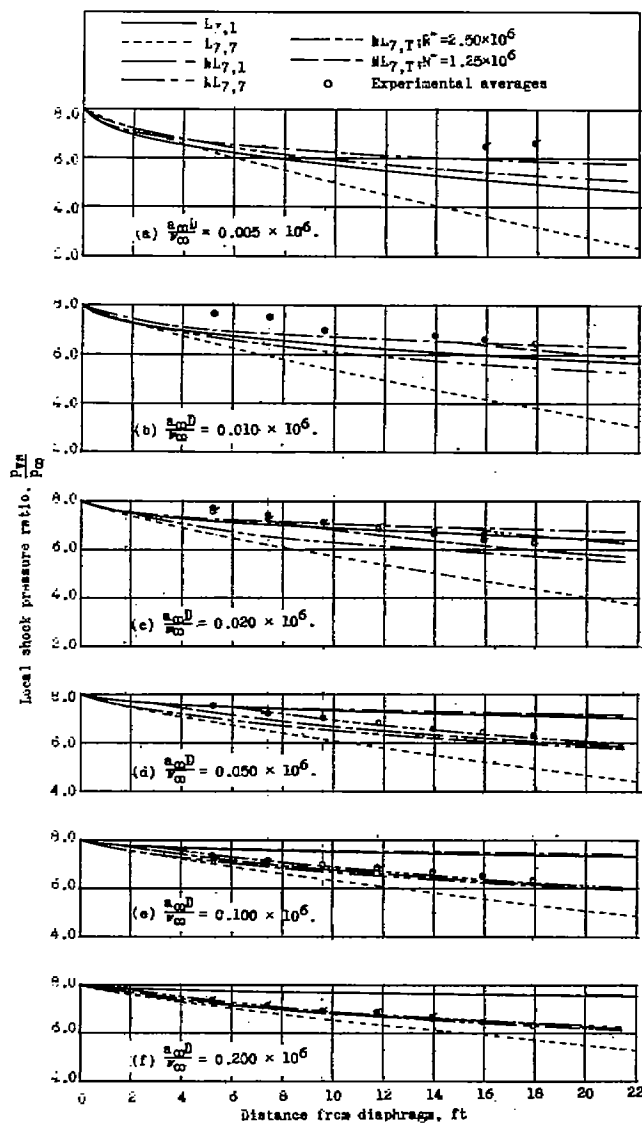
Figure 34.- Comparison of averaged experimental local shock pressure ratios with various theoretical predictions. \frac{p_{\beta 0}}{p_{\infty}} = 8.0 . Flagged and unflagged symbols are used to distinguish between averages from different days.
