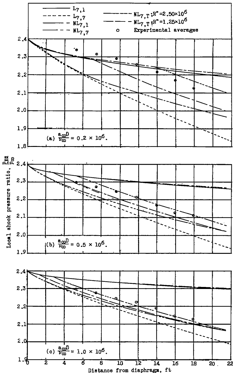
Figure 26.- Comparison of averaged experimental local shock pressure ratios with various theoretical predictions. \frac{P_{\beta 0}}{P_{\infty}} = 2.4 .
