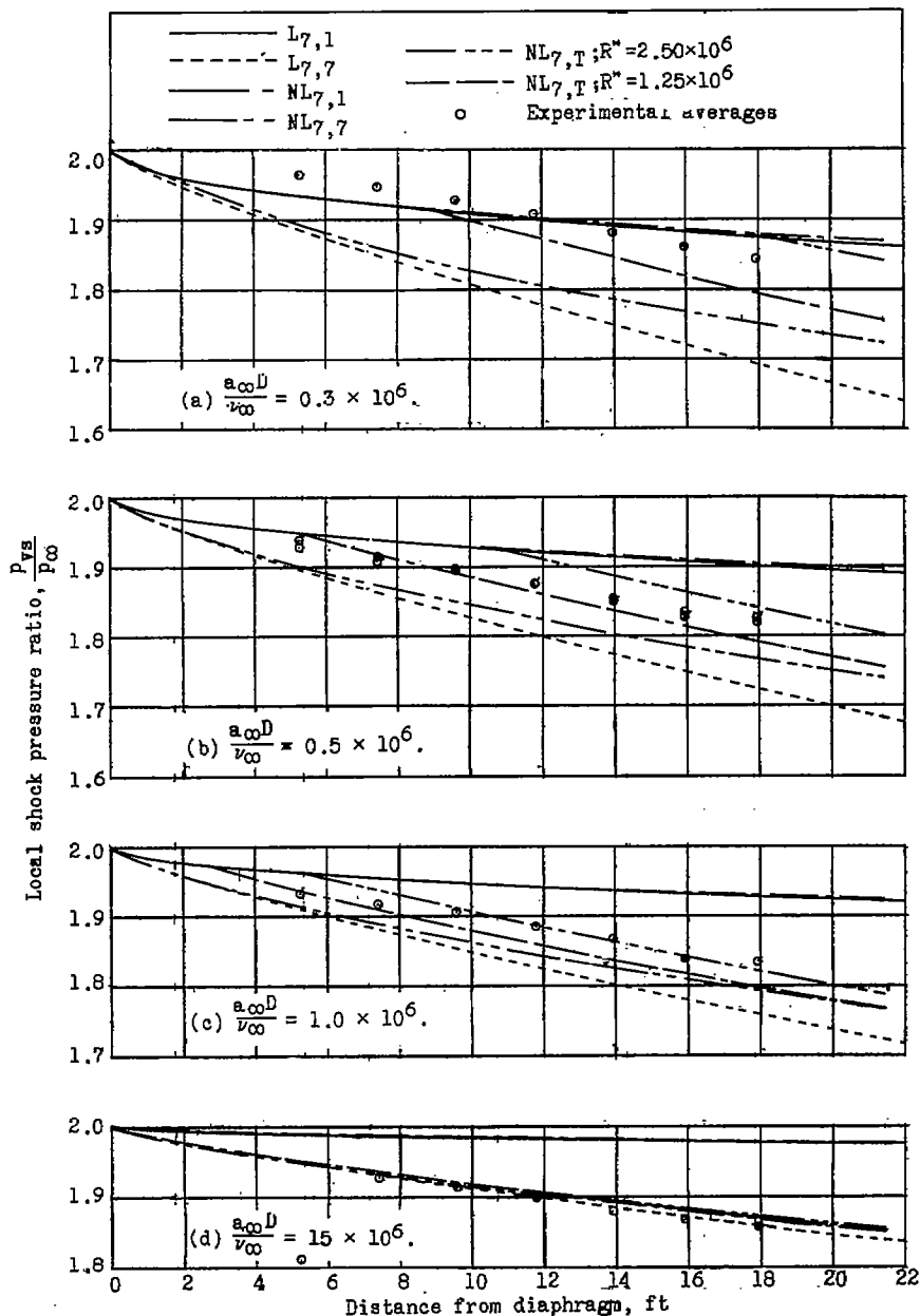
Figure 25.- Comparison of averaged experimental local shock pressure ratios with various theoretical predictions. \frac{P_{\beta 0}}{P_{\infty}} = 2.0 . Flagged and unflagged symbols are used to distinguish between averages from different days.
