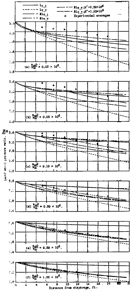
Figure 29.- Comparison of averaged experimental local shock pressure ratios with various theoretical predictions. \frac{p_{\beta 0}}{p_{\infty}} = 3.6 . Flagged and unflagged symbols are used to distinguish between averages from different days.
