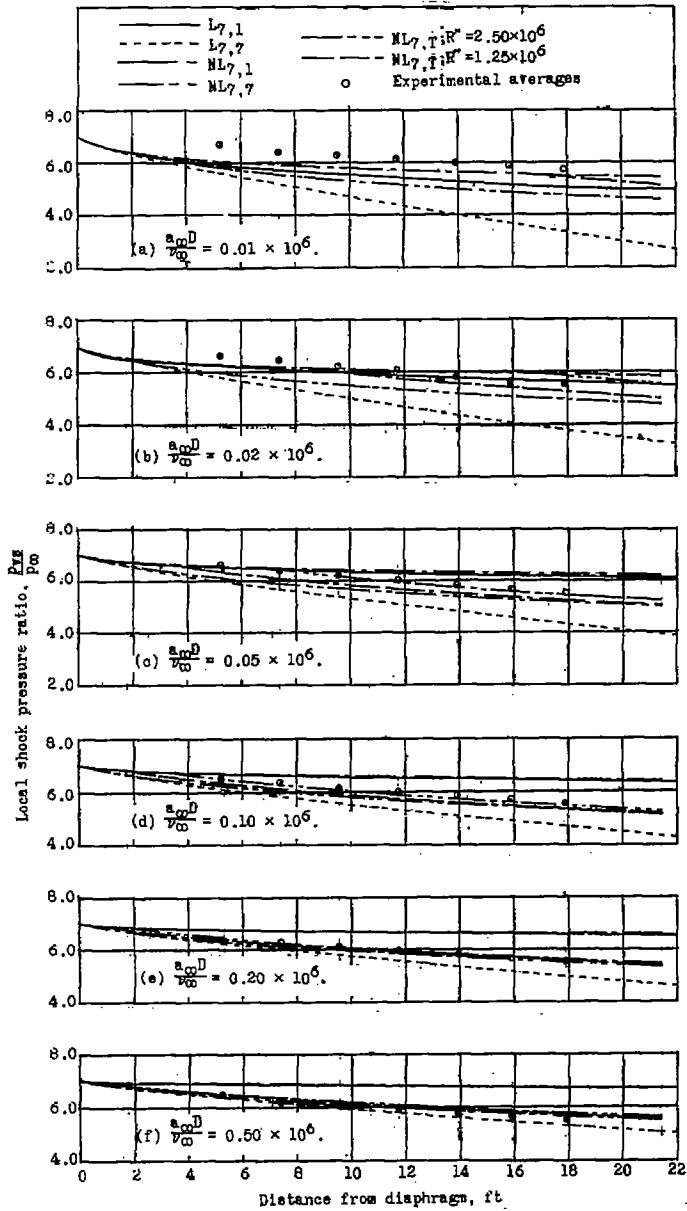
Figure 33.- Comparison of averaged experimental local shock pressure ratios with various theoretical predictions. \frac{P_{\beta 0}}{P_{\infty}} = 7.0 .
