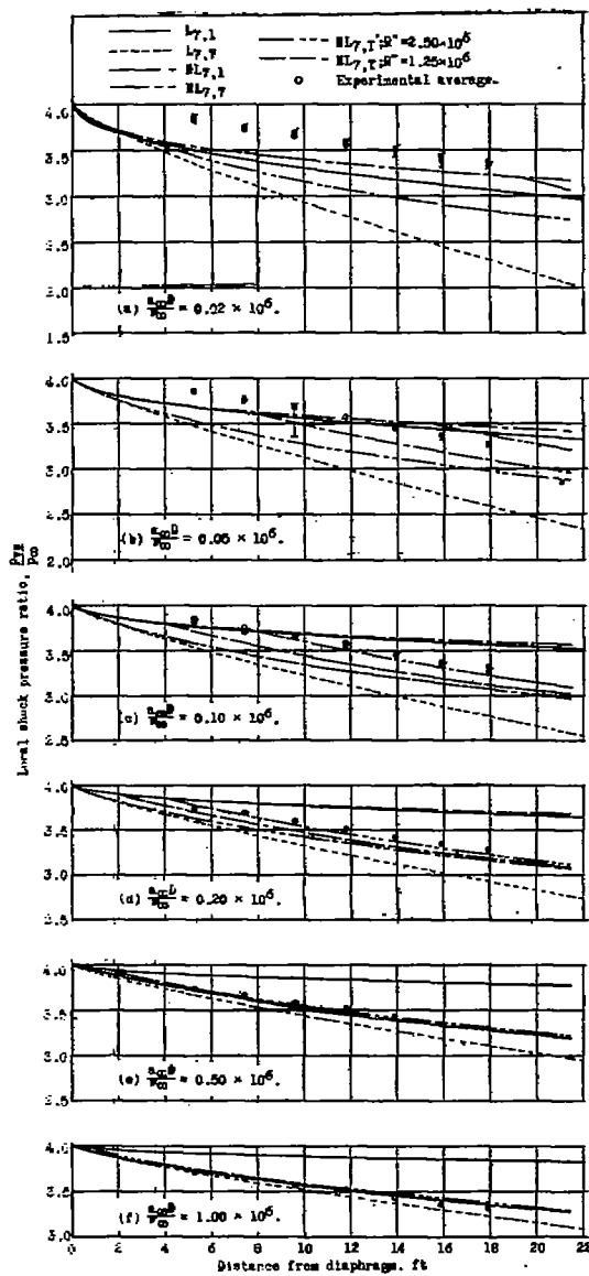
Figure 30.- Comparison of averaged experimental local shock pressure
