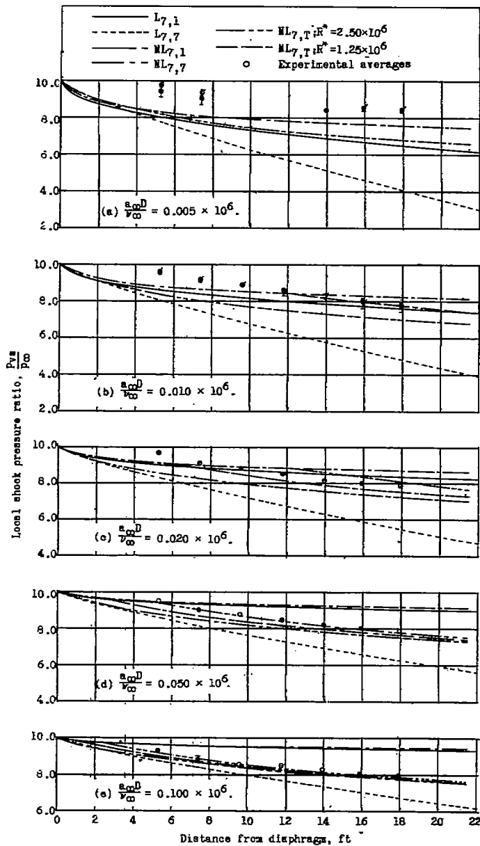
Figure 36.- Comparison of averaged experimental local shock pressure ratios with various theoretical predictions. \frac{P}{P_0} = 10.0 . The vertical lines in (a) and (b) show range of scatter in an averaged group when scatter exceeds symbol size. Flagged and unflagged symbols are used to distinguish between averages from different days.
