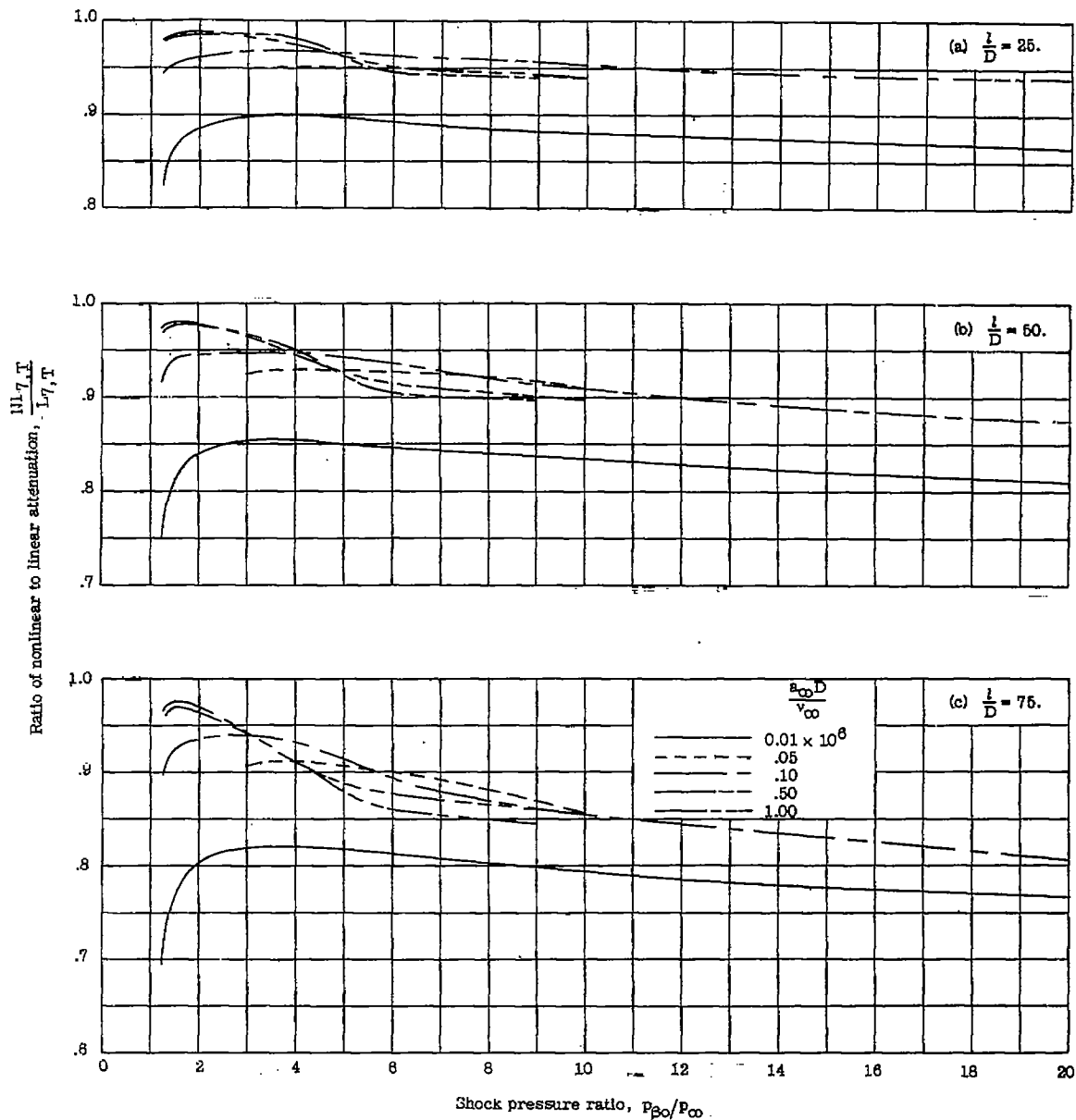
Figure 15.- Ratio of nonlinear attenuation to linear attenuation for region \alpha turbulent and region \beta transitional plotted against shock pressure ratio. R^* = 2.50 \times 10^6 . The shock wave is located at a distance l/D from the diaphragm station.
