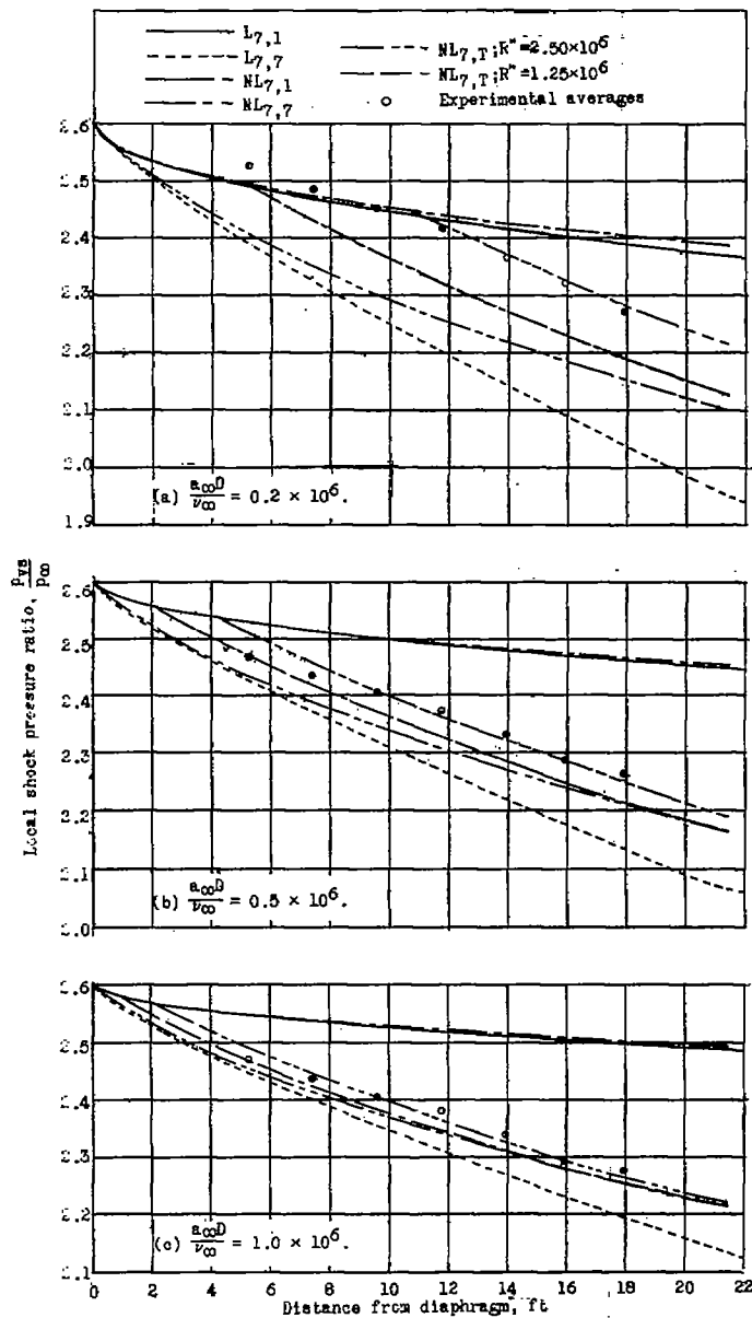
Figure 27.- Comparison of averaged experimental local shock pressure
