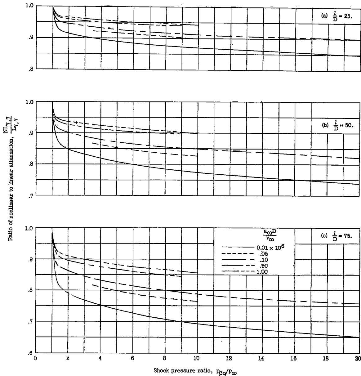
Figure 13.- Ratio of nonlinear attenuation to linear attenuation for both regions \alpha and \beta turbulent plotted against shock pressure ratio. The shock wave is located at a distance l/D from the diaphragm station.
