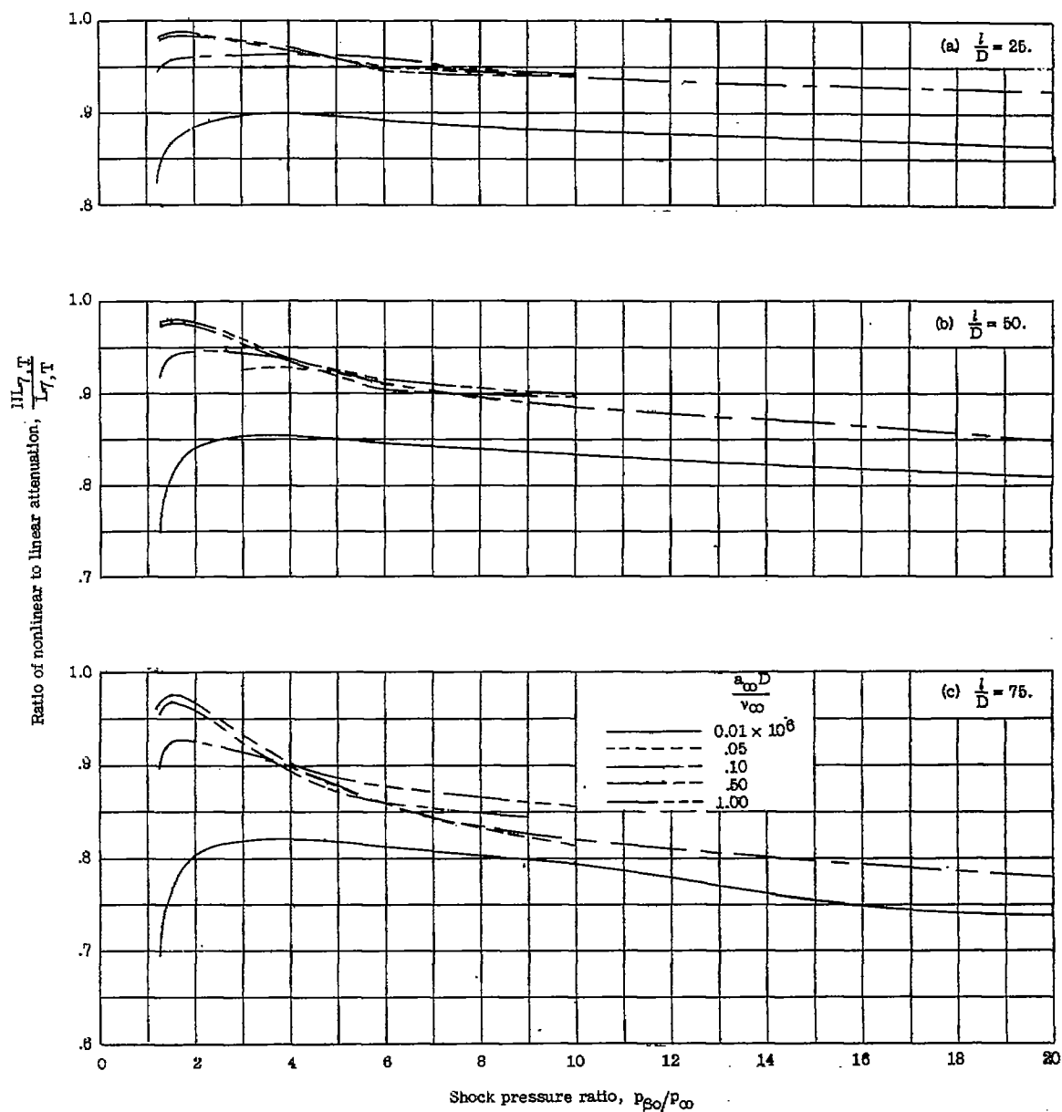
Figure 14.- Ratio of nonlinear attenuation to linear attenuation for region \alpha turbulent and region \beta transitional plotted against shock pressure ratio. R^* = 1.25 \times 10^6 . The shock wave is located at a distance l/D from the diaphragm station.
