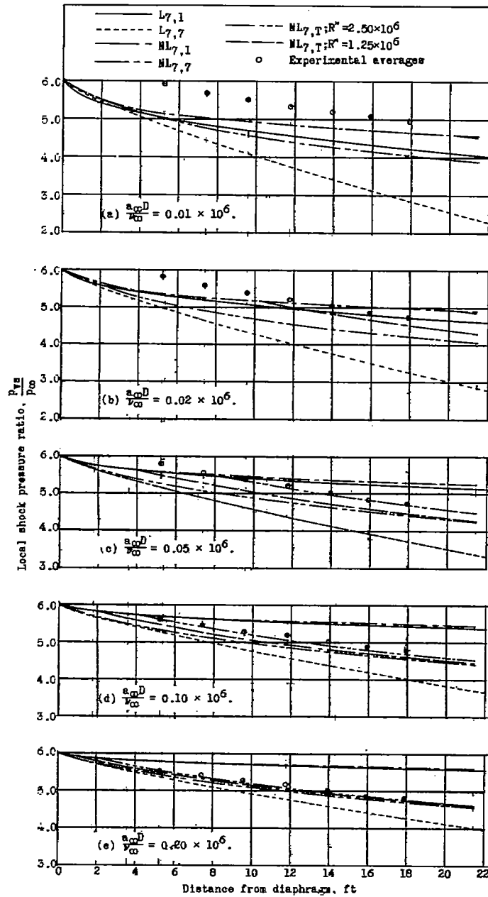
Figure 32.- Comparison of averaged experimental local shock pressure ratios with various theoretical predictions. \frac{p_{\beta 0}}{p_{\infty}} = 6.0 .
