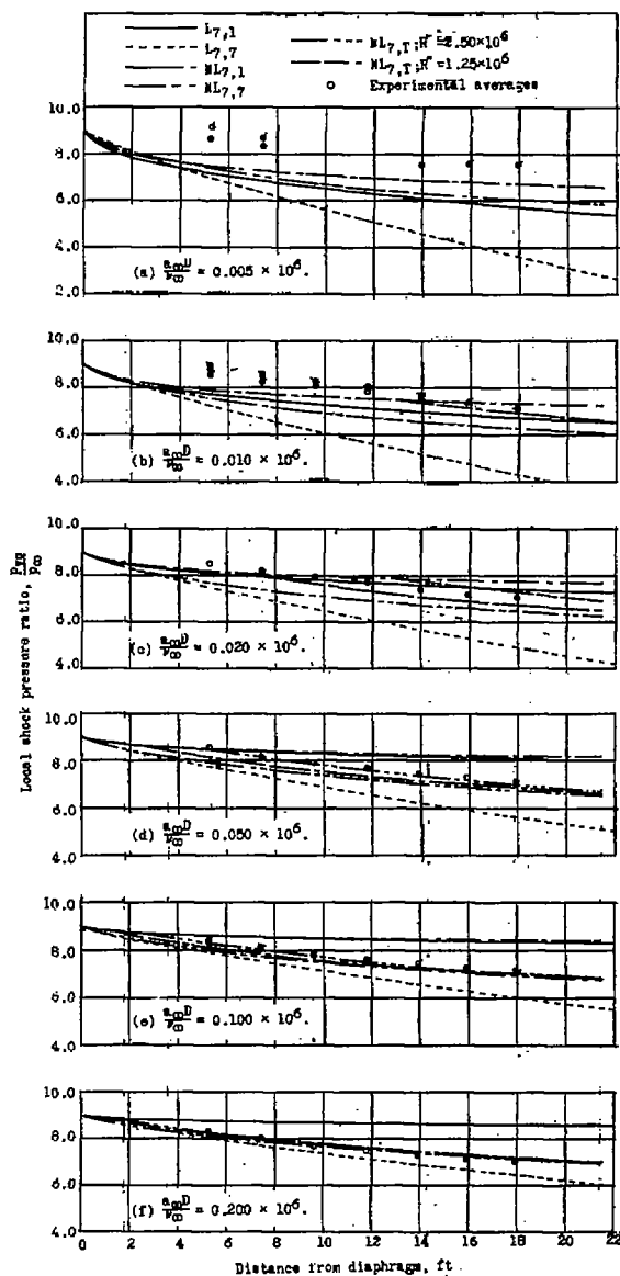
Figure 35.- Comparison of averaged experimental local shock pressure ratios with various theoretical predictions. \frac{P_{\beta 0}}{P_{\infty}} = 9.0 . Flagged and unflagged symbols are used to distinguish between averages from different days.
