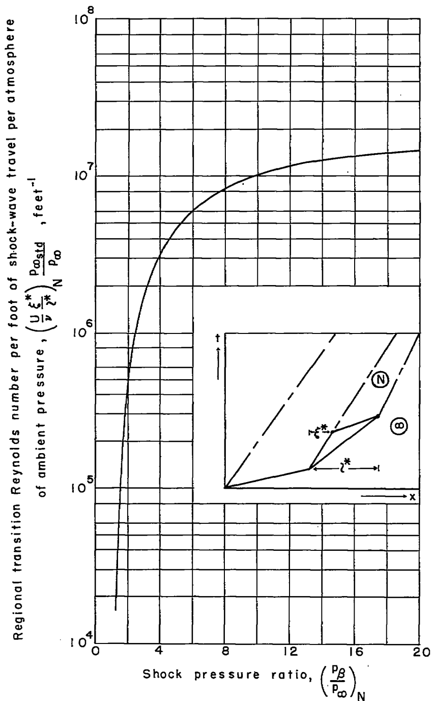
Figure 10.- Regional transition Reynolds number per foot of shock-wave travel per atmosphere of ambient pressure plotted against shock pressure ratio. Circled symbols denote regions.
