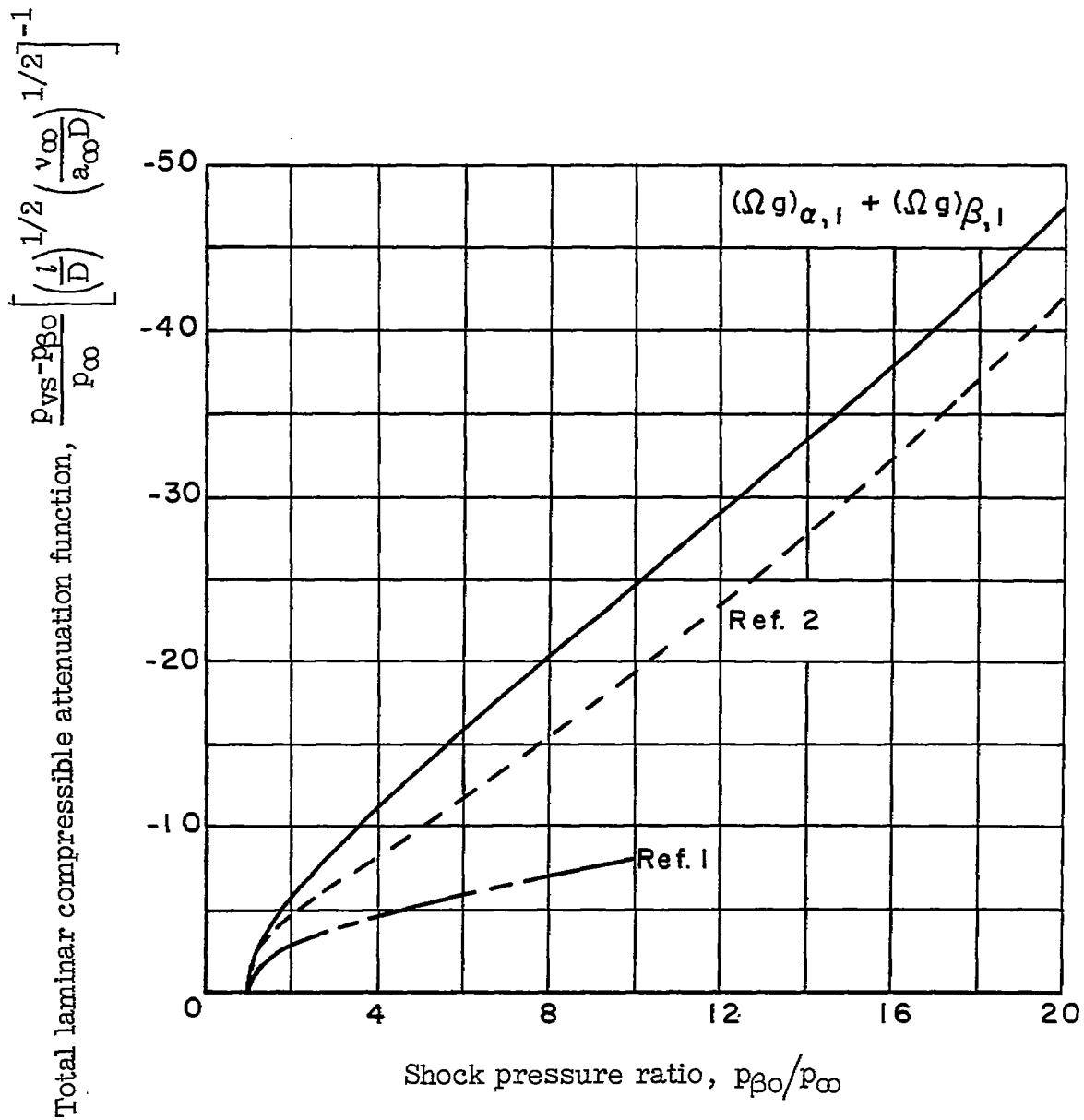
Figure 6.- Plot of total compressible linear attenuation functions against shock pressure ratio. \gamma = 1.4 ; \omega = 0.8 .
