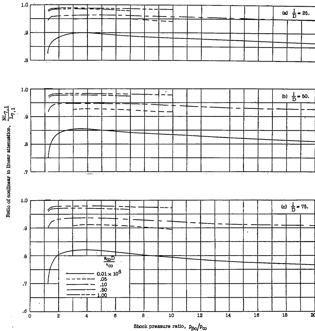
Figure 12.- Ratio of nonlinear attenuation to linear attenuation for region \alpha turbulent and region \beta laminar plotted against shock pressure ratio. The shock wave is located at a distance l/D from the diaphragm station.
