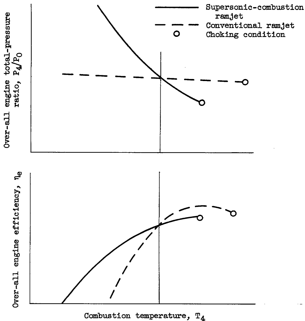
Figure 9. - Effect of combustion temperature on conventional and supersonic-combustion ramjets.
