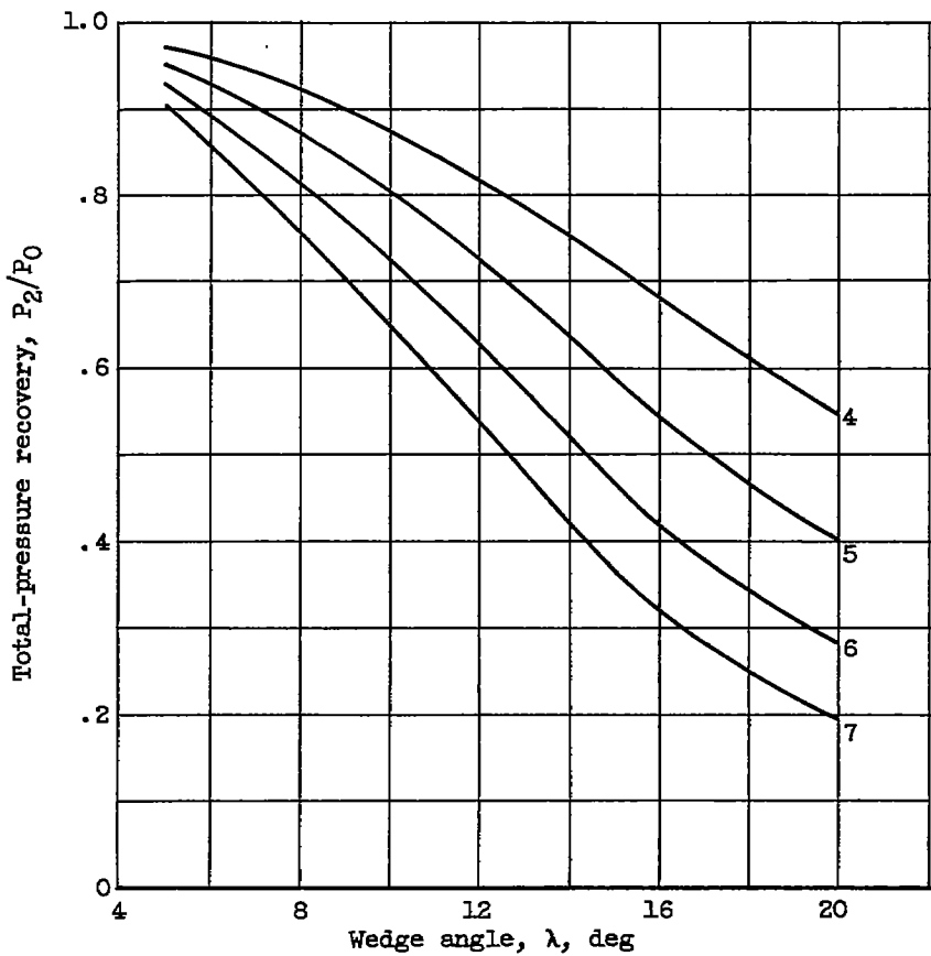
(a) Wedge inlet for SCRJ.
