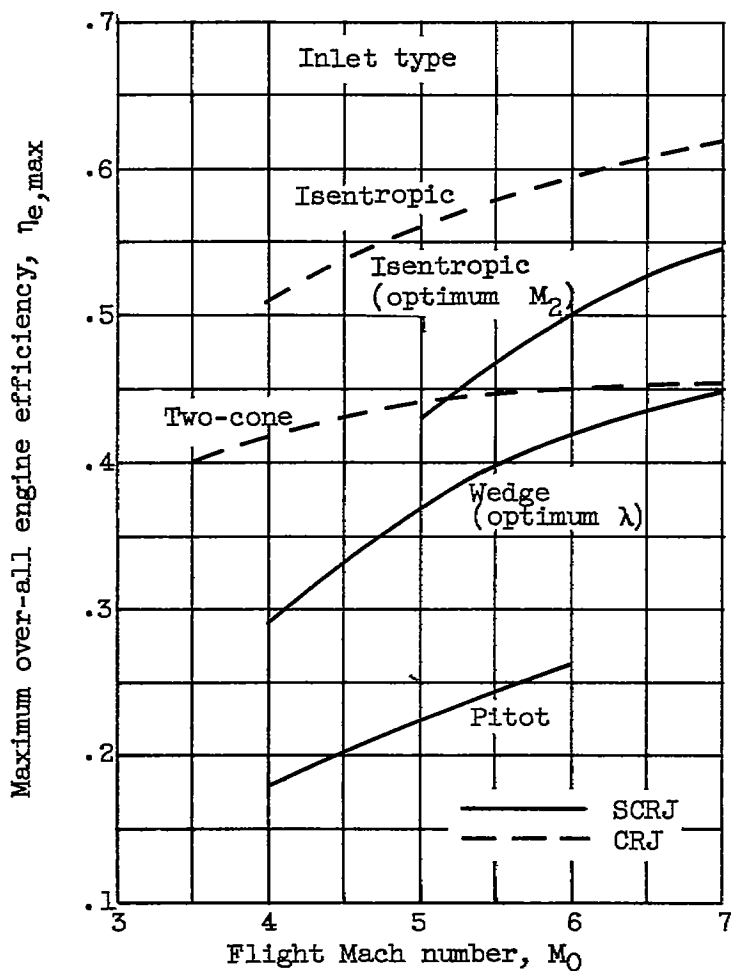
Figure 12. - Comparison of CRJ and SCRJ with various inlet types. A_4/A_2 , 1.0; \eta_c , 0.95; M_4 , 1.0 for all SCRJ; C_V , 0.96; real gas.
