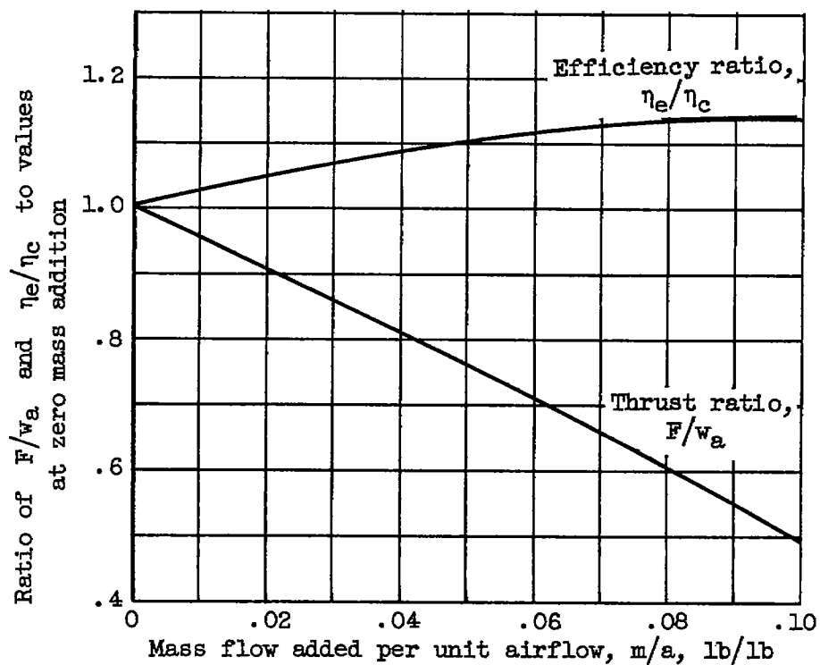
Figure 13. - Effect of mass addition on performance of SCRJ. Pitot inlet; M_0 , 6.0; A_4/A_2 , 1.0; M_4 , 1.0; C_v , 0.96; ideal gas.
