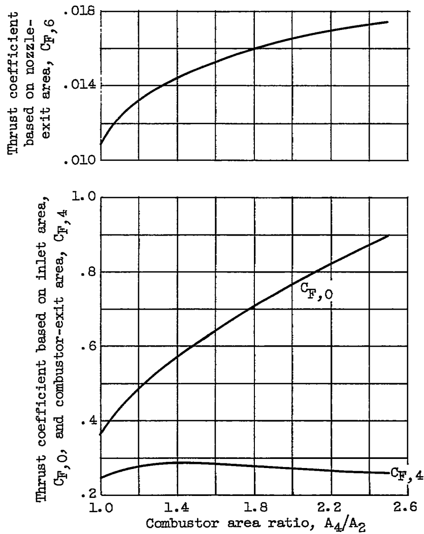
Figure 20. - Effect of combustor area ratio on various SCRJ thrust coefficients. Wedge inlet ( \lambda , 15^\circ ); M_0 , 6.0; \eta_c , 0.95; n , 0.5; M_4 , 1.0; C_v , 0.96; real gas.
