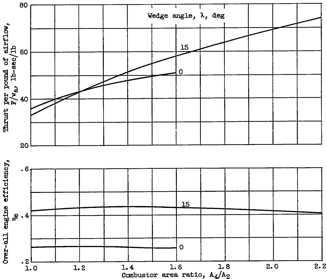
(a) Wedge inlet. Flight Mach number, 6.0.
