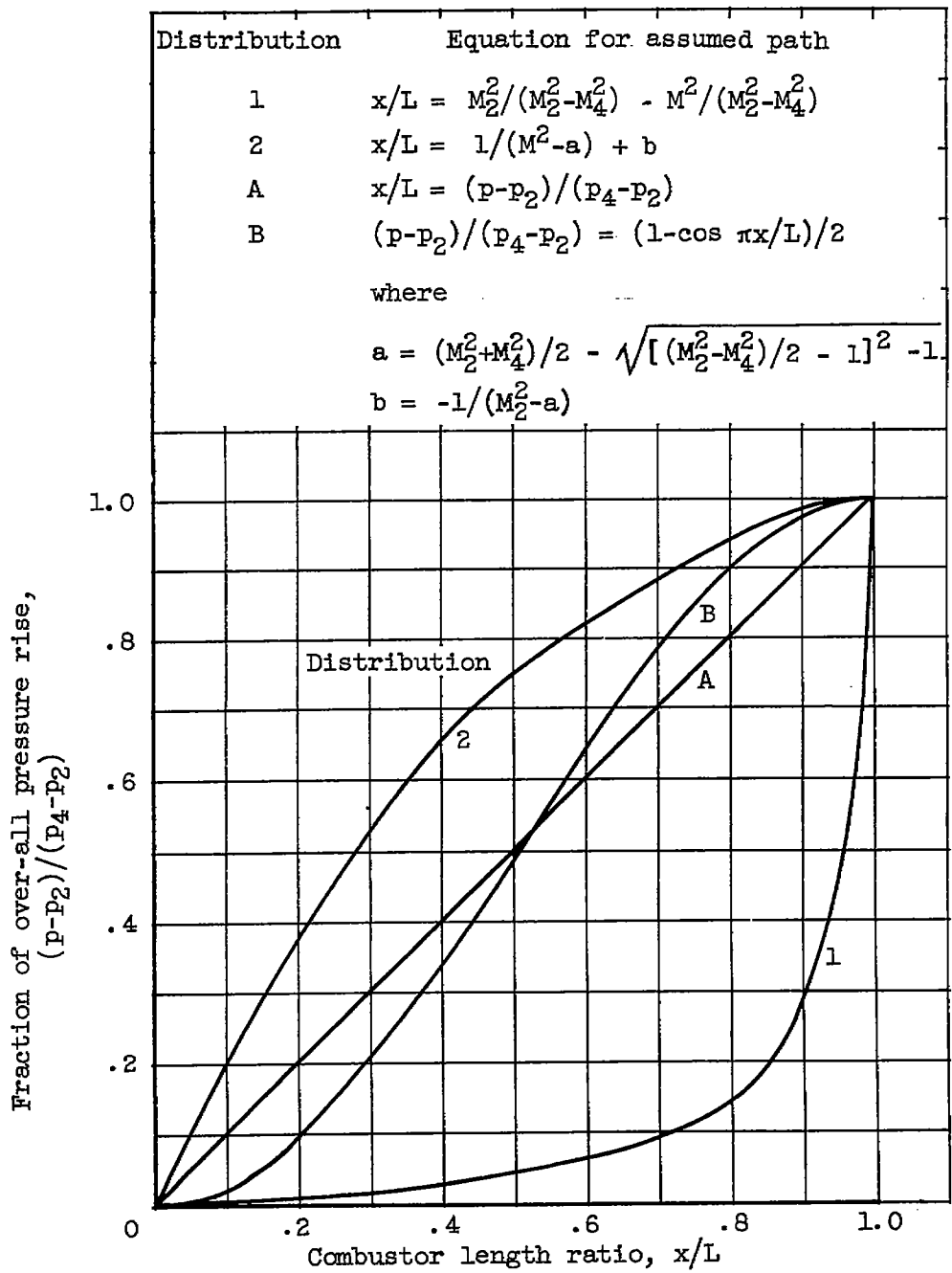
(a) Pressure distribution.
