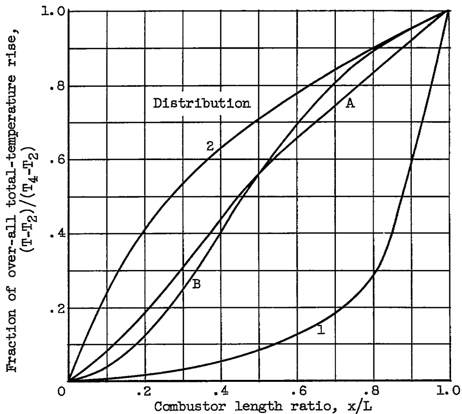
(b) Total-temperature distribution.
