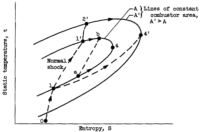
Figure 3. - Combustion with variable combustor area.
