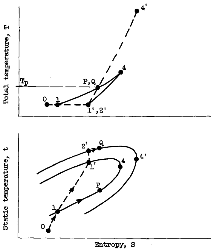
Figure 4. - Comparison of supersonic and conventional ramjet cycles.
