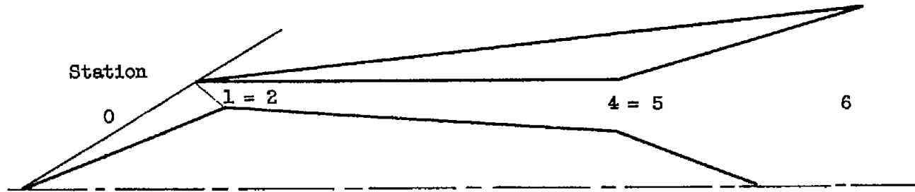
(a) Supersonic-combustion ramjet.
