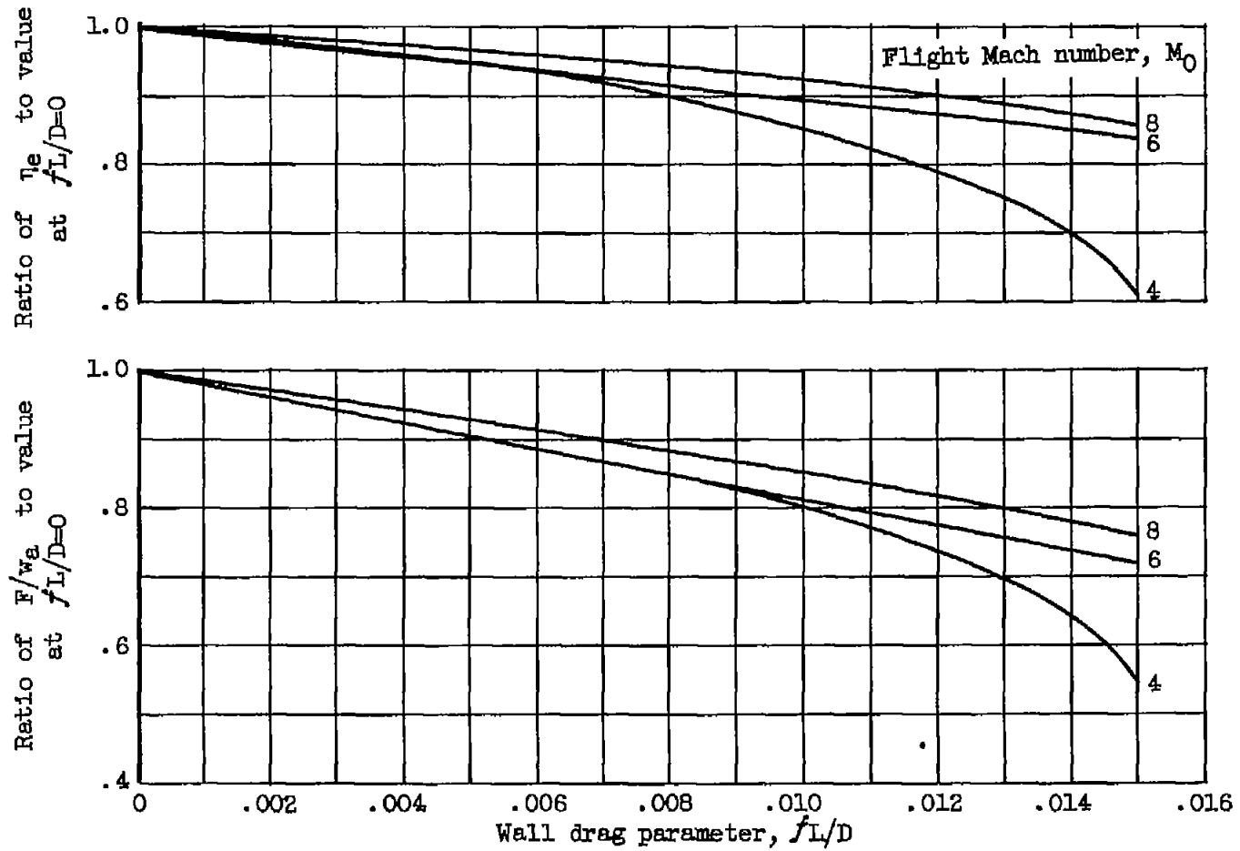
Figure 22. - Effect of wall friction loss on performance of SCRJ. Pitot inlet; A_4/A_2 , 1.0; M_4 , 1.0; C_V , 0.96; ideal gas.
