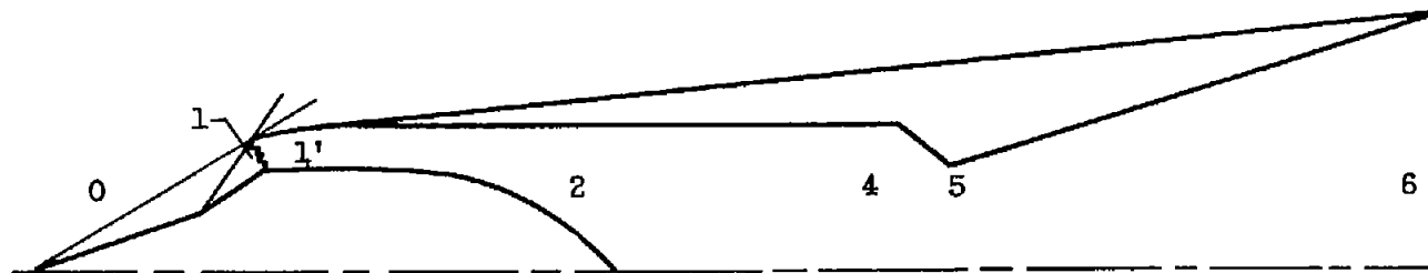
(b) Conventional ramjet.
