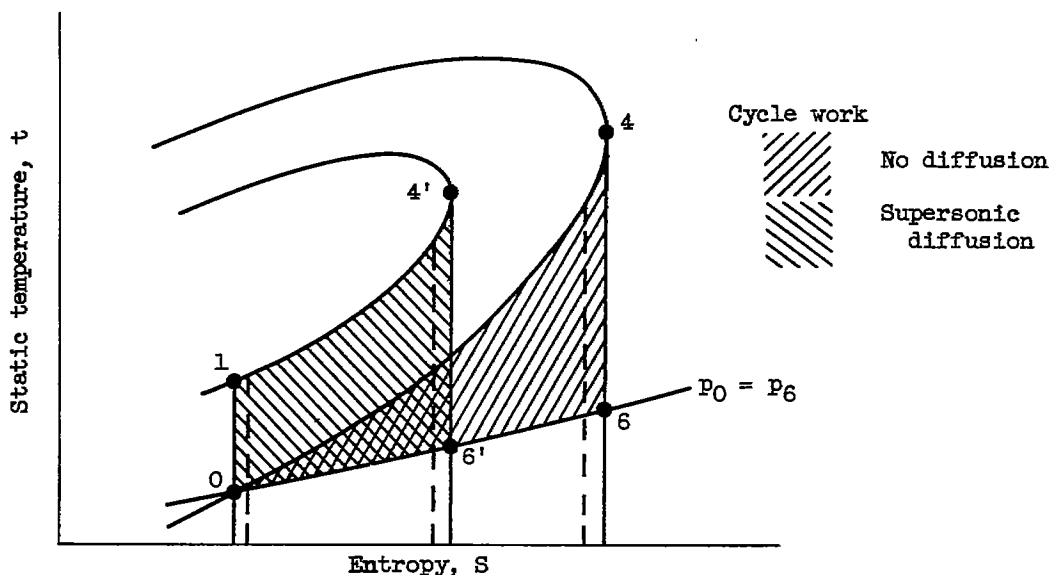
Figure 2. - Temperature-entropy diagram comparing work output with and without supersonic diffusion prior to supersonic combustion. Maximum heat addition; no inlet or exit losses shown.
