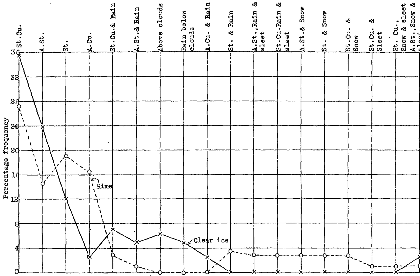
Fig.5 Percentage frequencies of clear ice and rime formations for various cloud and weather conditions.
