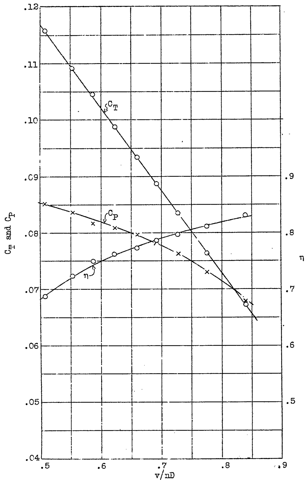
Figure 5.--Model propeller "F" with counter-propeller on shaft.
