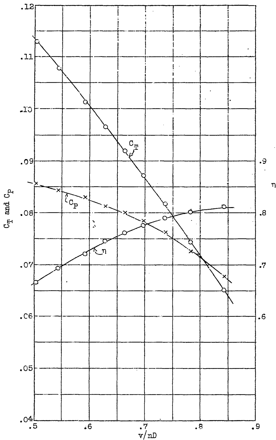
Figure 4.-Model propeller "F" alone.
