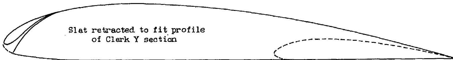
Figure 3.-Section showing special slat and Fowler flap retracted.
