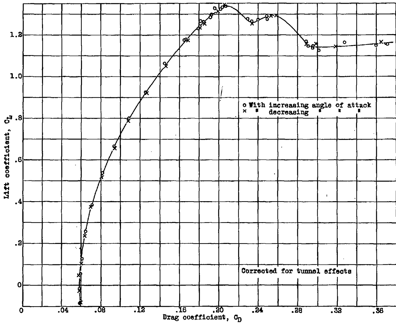
Figure 21.-Polar for McDonnell airplane with large fillet and N.A.C.A. engine cowling.
