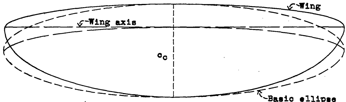
(b) Distorted elliptical.
