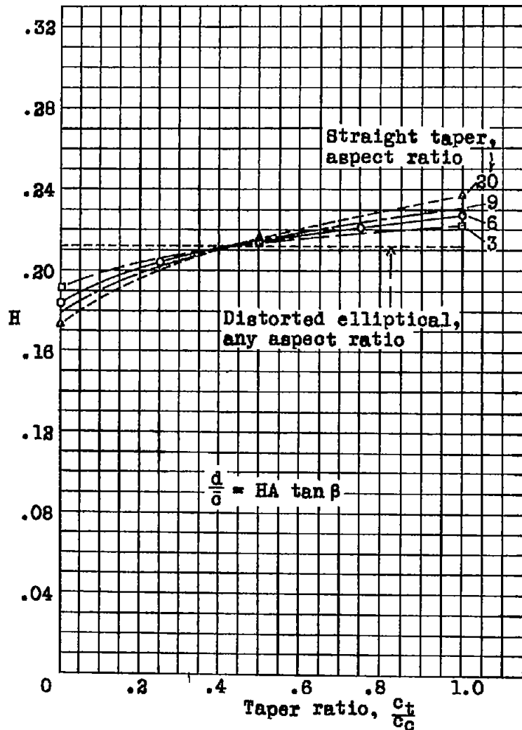
Figure 5.- Chart for calculating the location of the aerodynamic center, for wings of various plan forms.
