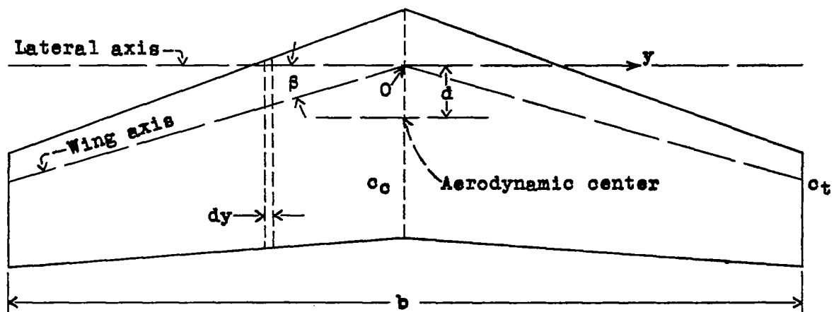
(a) Straight taper.
