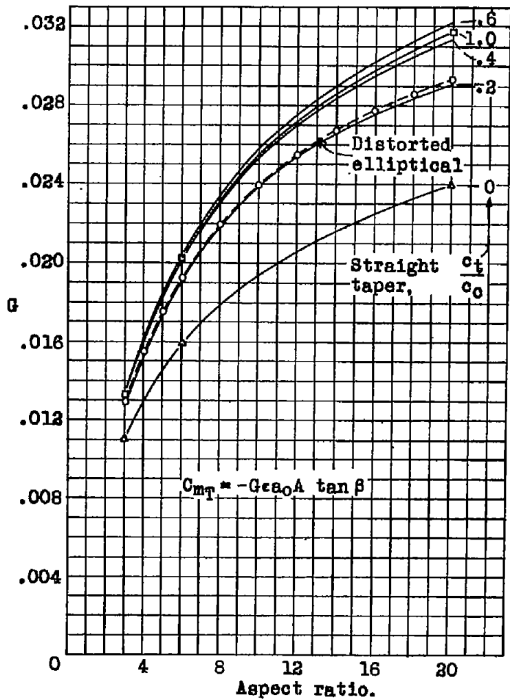
Figure 4.- Chart for calculating the pitching moment due to twist, for wings of various plan forms.
