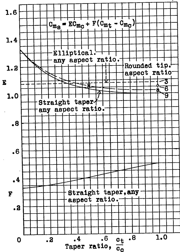
Figure 2.- Chart for calculating the pitching moment due to the sections, for wings of various plan forms.
