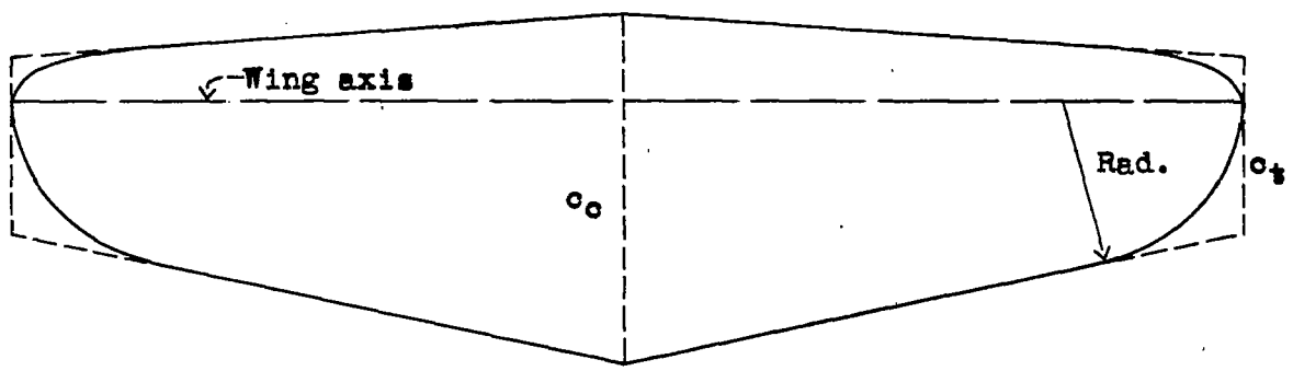
(c) Rounded tip.
