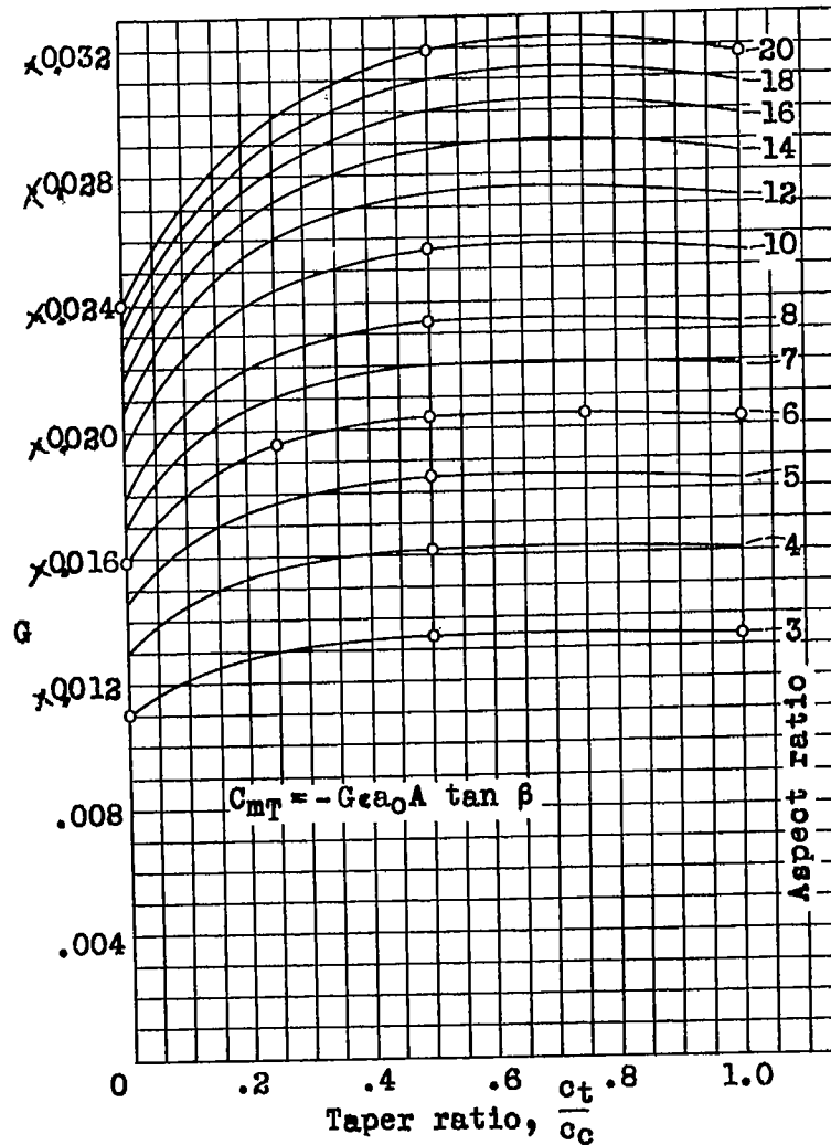
Figure 3.- Chart for calculating the pitching moment due to twist for wings with straight-taper plan forms.
