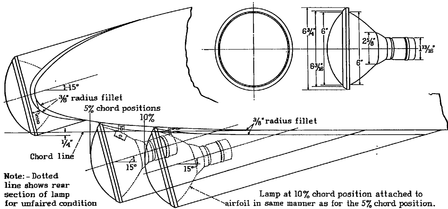
Figure 2.- Lamp installations on airfoil.
