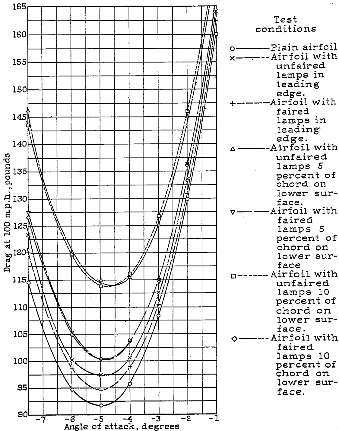
Figure 4.- Airfoil drag at 100 miles per hour for the lamp arrangements tested. Results not corrected for tunnel jet boundary effect.
