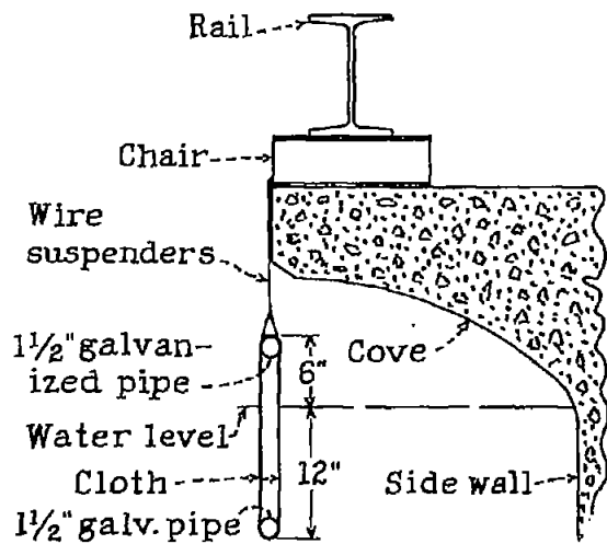
Figure 1. - Vertical screen.
