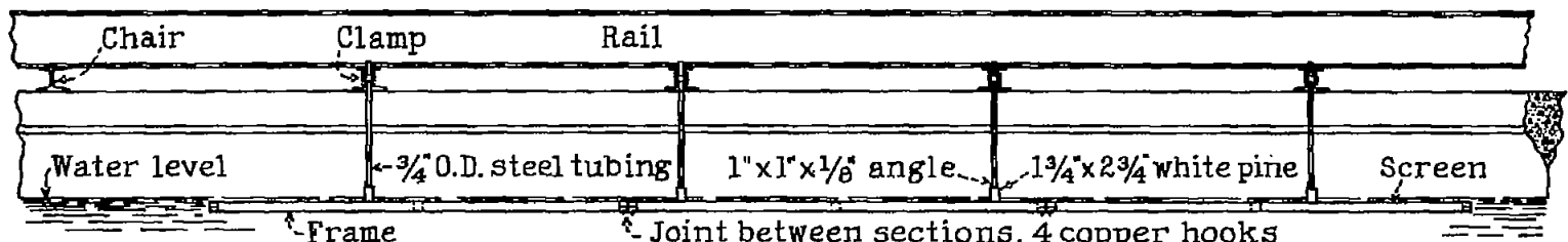
Side elevation. Three sections of fixed horizontal screen installed. Joint between sections, 4 copper hooks
