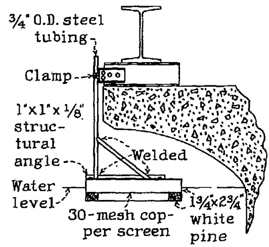
Figure 3. - Fixed horizontal screen.
