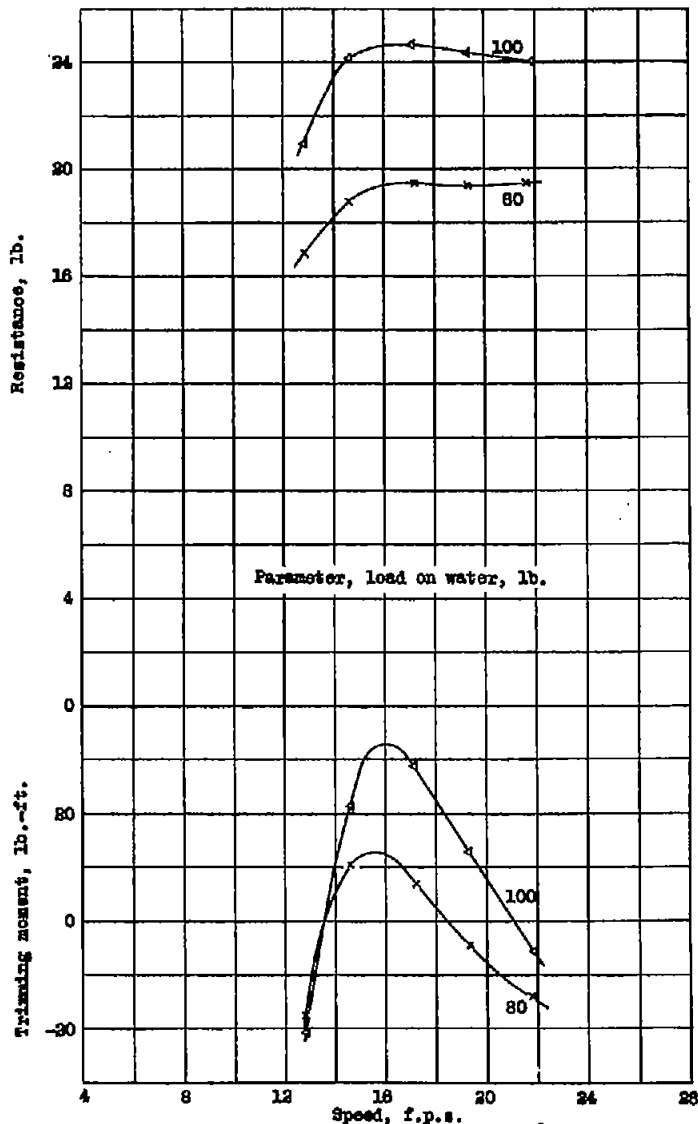
Figure 27.- Resistance and trimming moment, \tau = 11^\circ , Model 11-0-8 ( 7^\circ angle of afterbody keel.)
