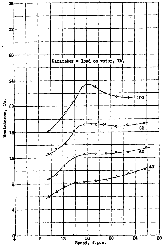
Figure 20a.-Resistance. \tau = 9^\circ . Model 11-0. ( 5\frac{1}{2}^\circ angle of afterbody keel)
