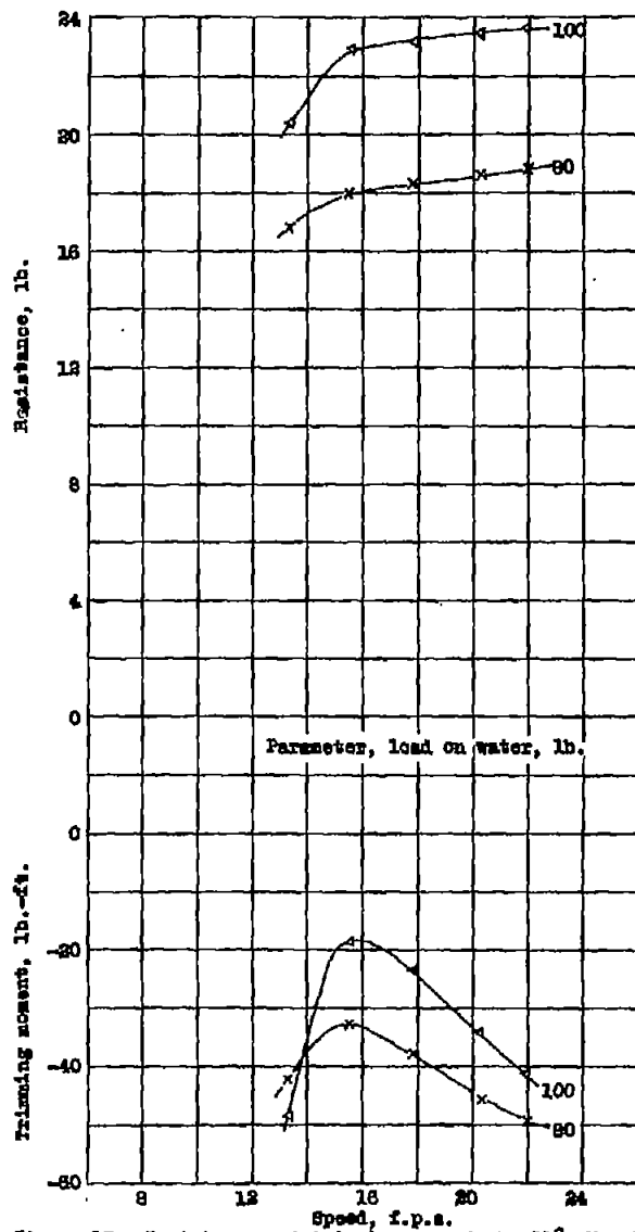
Figure 15.- Resistance and trimming moment, \tau = 110^\circ , Model 11-0-8 ( 4^\circ angle of afterbody keel.)
