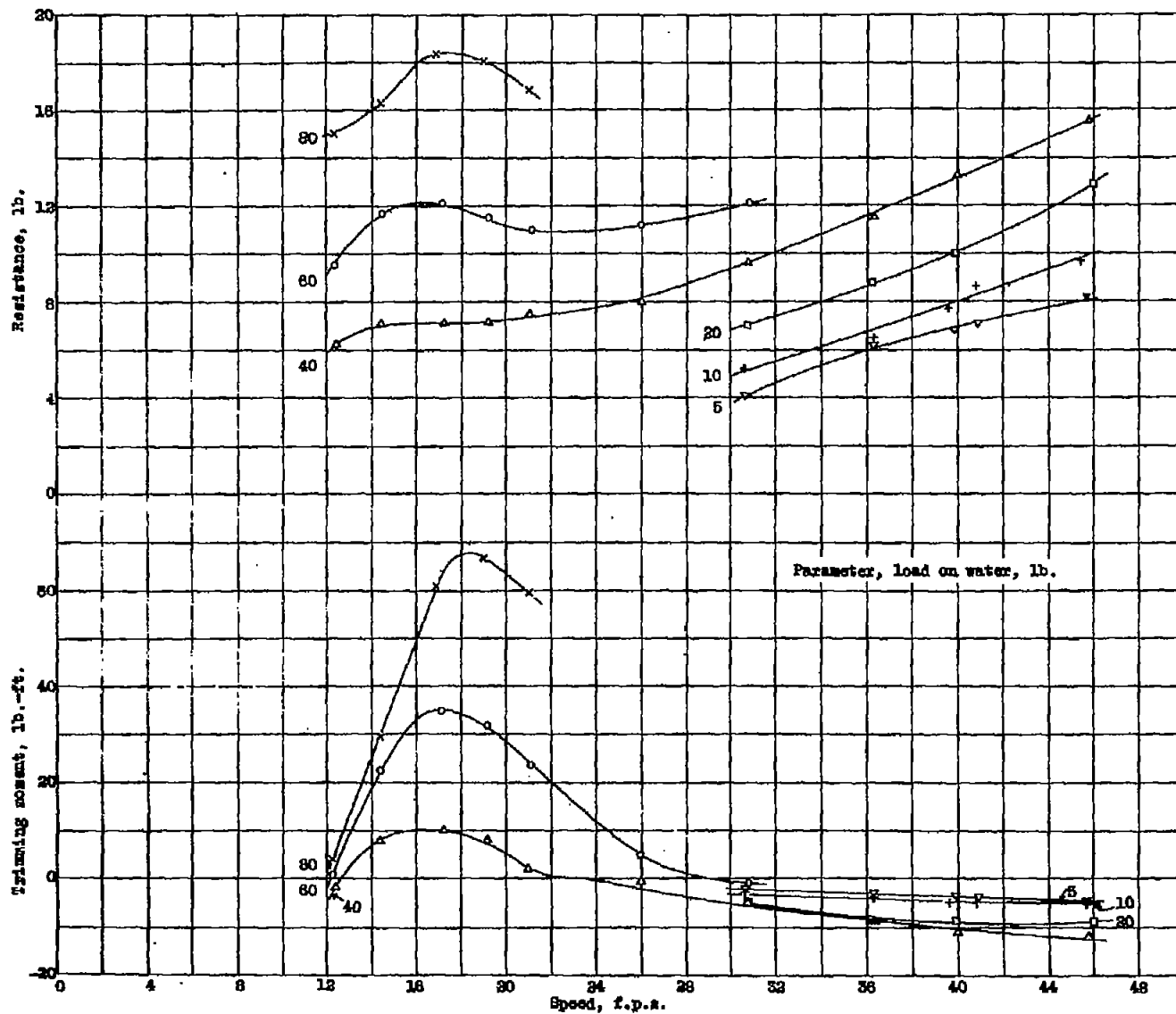
Figure 12.- Resistance and trimming moment, \tau = 5^\circ . Model 11-0-8 ( 4^\circ angle of afterbody keel).
