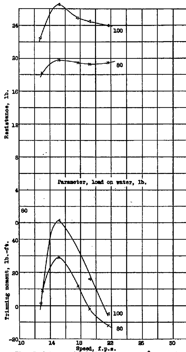
Figure 33. - Resistance and trimming moment, T = 11^\circ , Model 11-C-10 ( 9^\circ angle of afterbody keel.)
