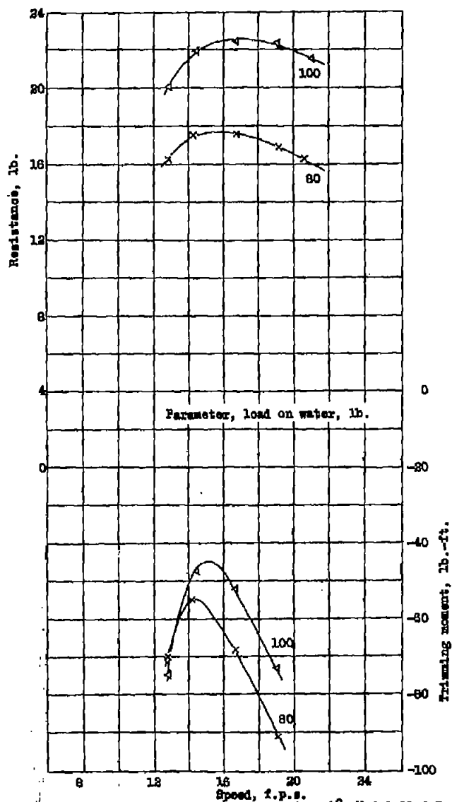
Figure 9.- Resistance and trimming moment, \tau = 11^\circ , Model 11-0-7 ( 2\text{-}1/2^\circ angle of afterbody keel.)
