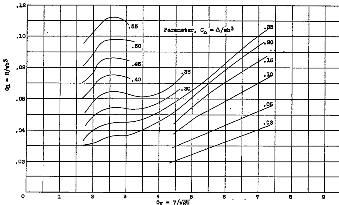
Figure 34.- Resistance coefficient at best trim angle, Model 11-C-7 (2-1/2° angle of afterbody keel.)
