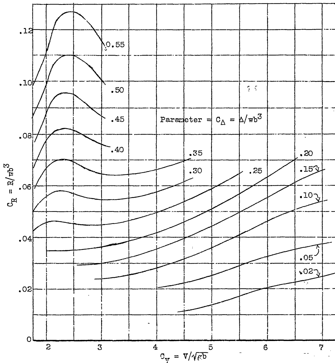
Figure 36.-Resistance coefficient at best trim angle. Model 11-C. ( 5 \frac{1}{2}^\circ angle of afterbody keel.)
