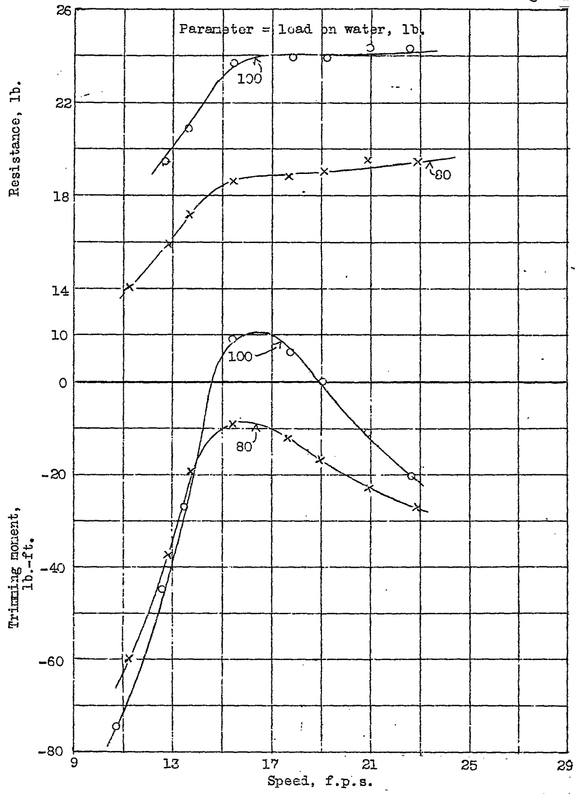
Figure 21 .-. Resistance and trimming moment, \tau = 11^\circ . Model 11-C. 5\frac{1}{2}^\circ angle of afterbody keel
