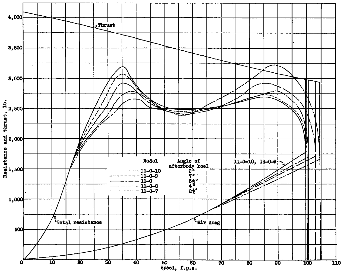
Figure 48.—Resistance and thrust of 15,000 lb. flying boat with various angles of afterbody keel.
