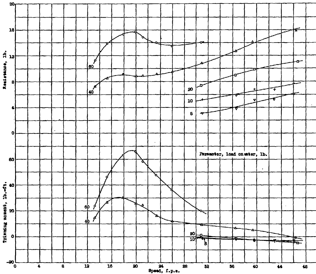
Figure 11.- Resistance and trimming moment, \tau = 5^\circ . Model 11-0-8 ( 4^\circ angle of afterbody keel).
