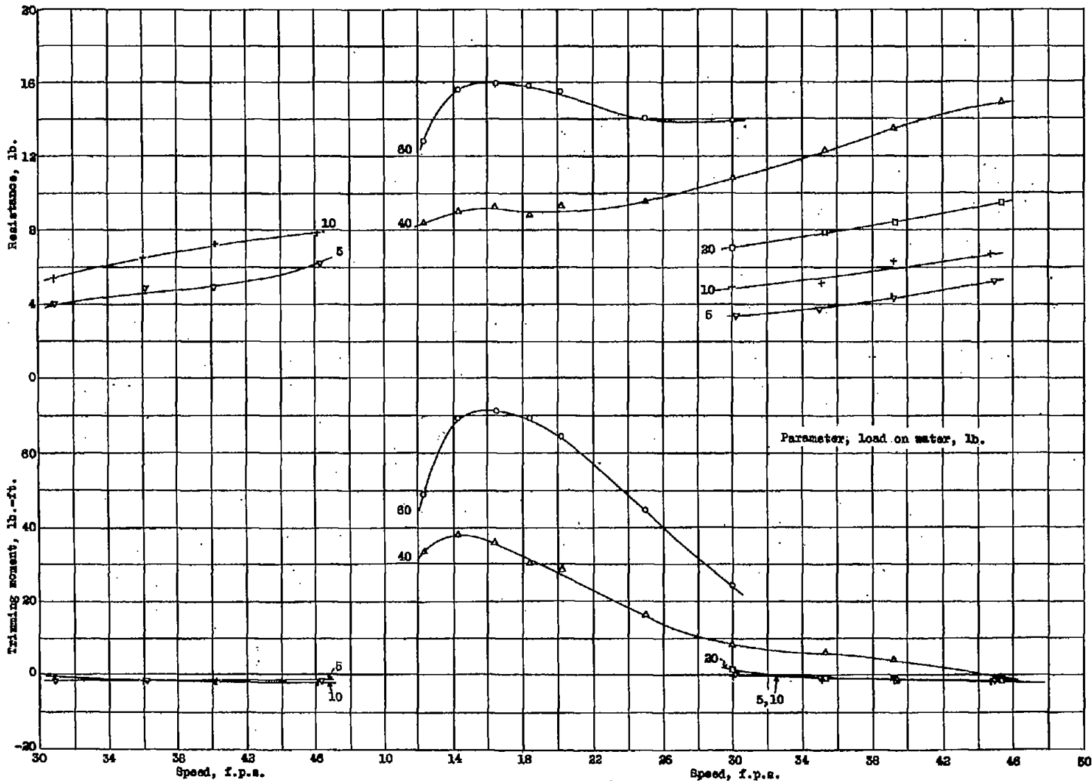
Figure 28.- Resistance and trimming moment, \tau = 2^\circ . Model 11-G-10 ( 9^\circ angle of afterbody keel).
