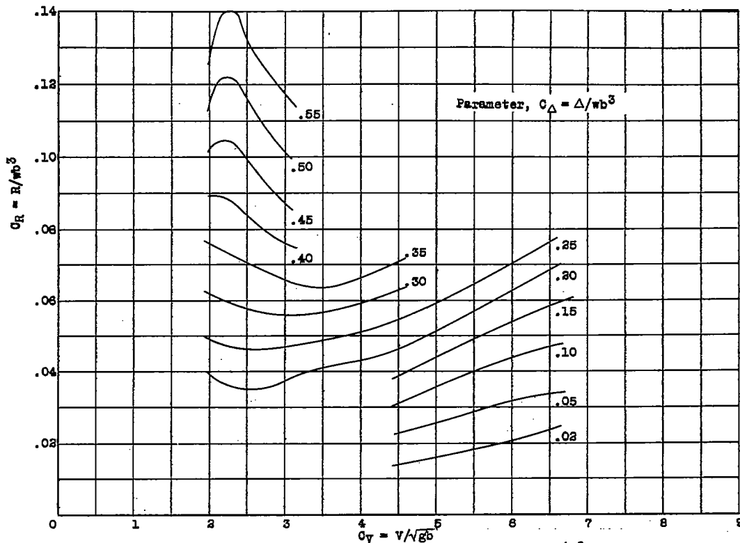
Figure 38.- Resistance coefficient at best trim angle, Model 11-C-10 ( 9^\circ angle of afterbody keel.)
