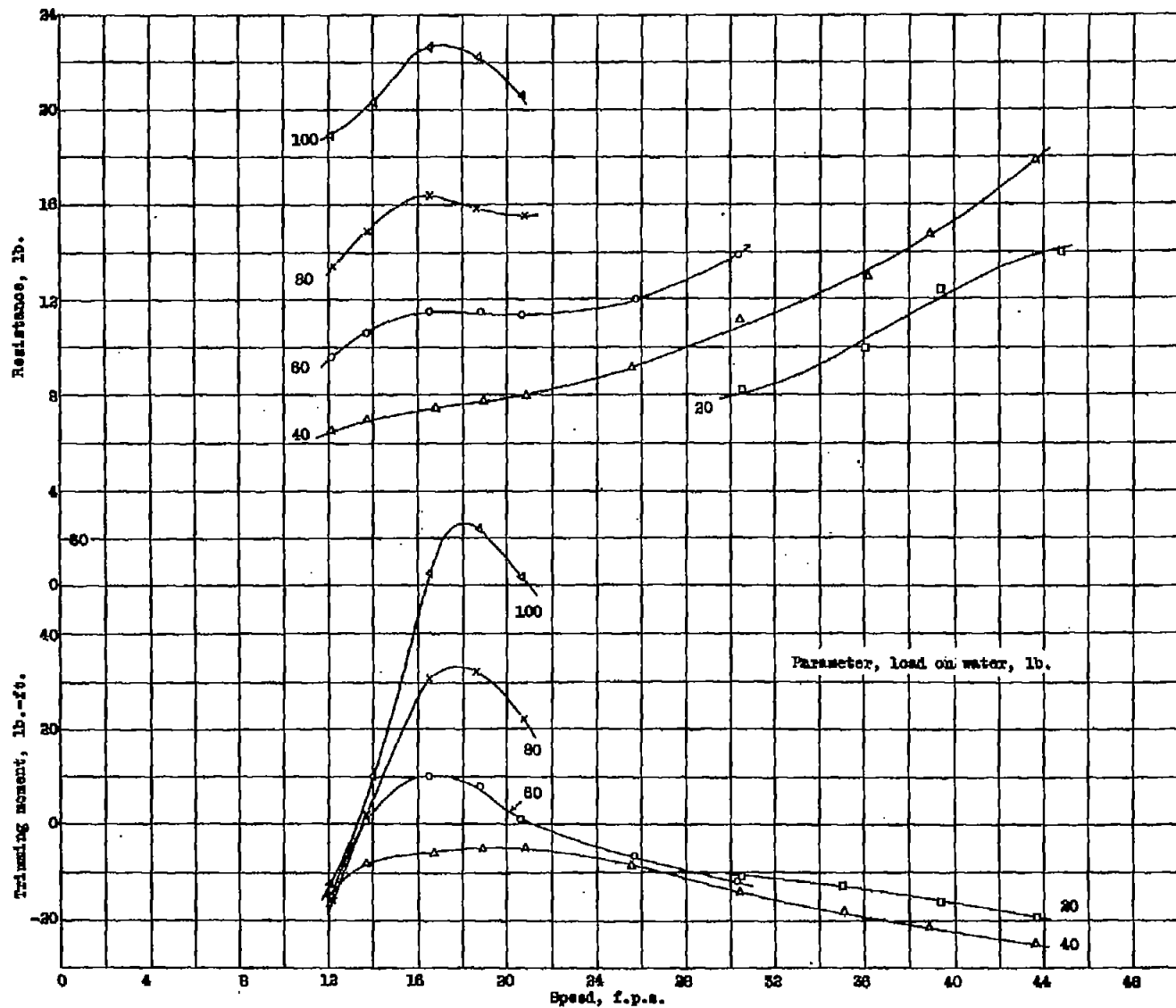
Figure 13.-- Resistance and trimming moment, \tau = 7^\circ , Model 11-0-8 ( 4^\circ angle of afterbody keel).
