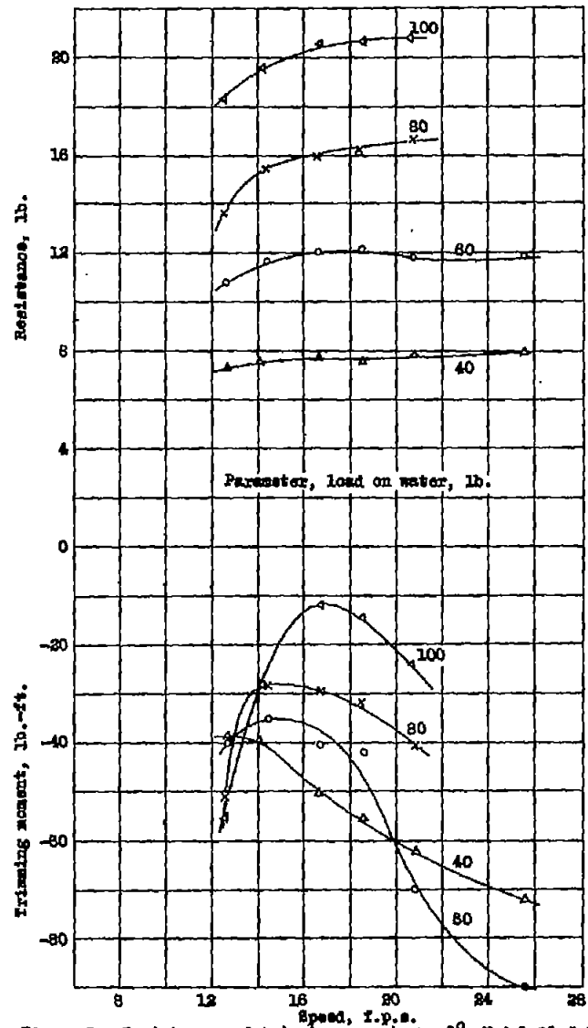
Figure 8.- Resistance and trimming moment, \tau = 9^\circ , Model 11-0-7 ( 2\frac{1}{2}^\circ angle of afterbody keel.)
