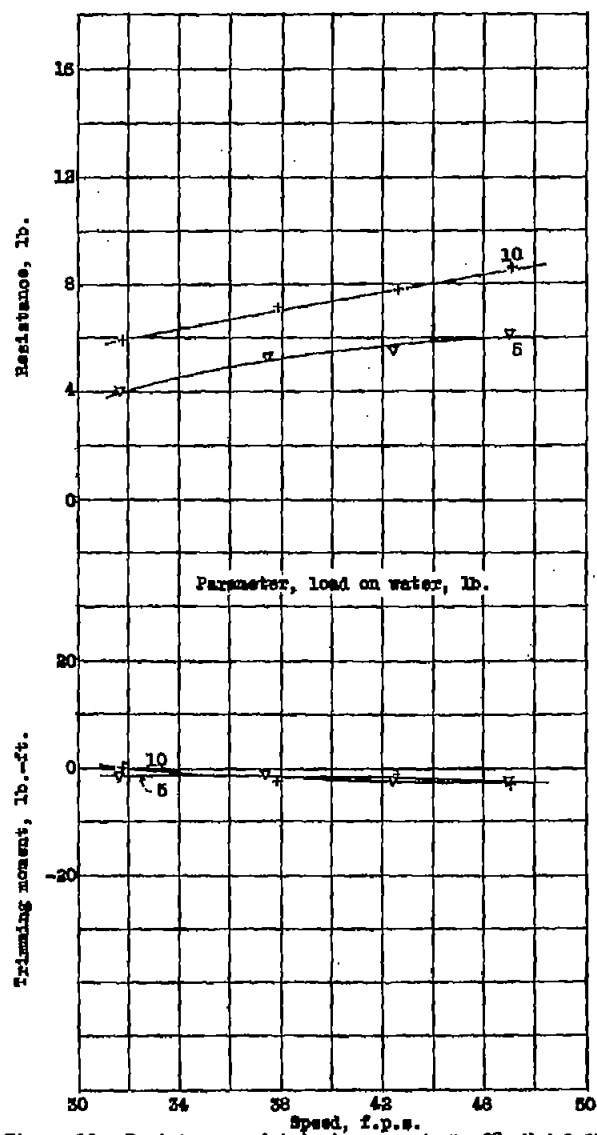
Figure 10.- Resistance and trimming moment, \tau = 20^\circ , Model 11-0-8 ( 4^\circ angle of afterbody keel.)
