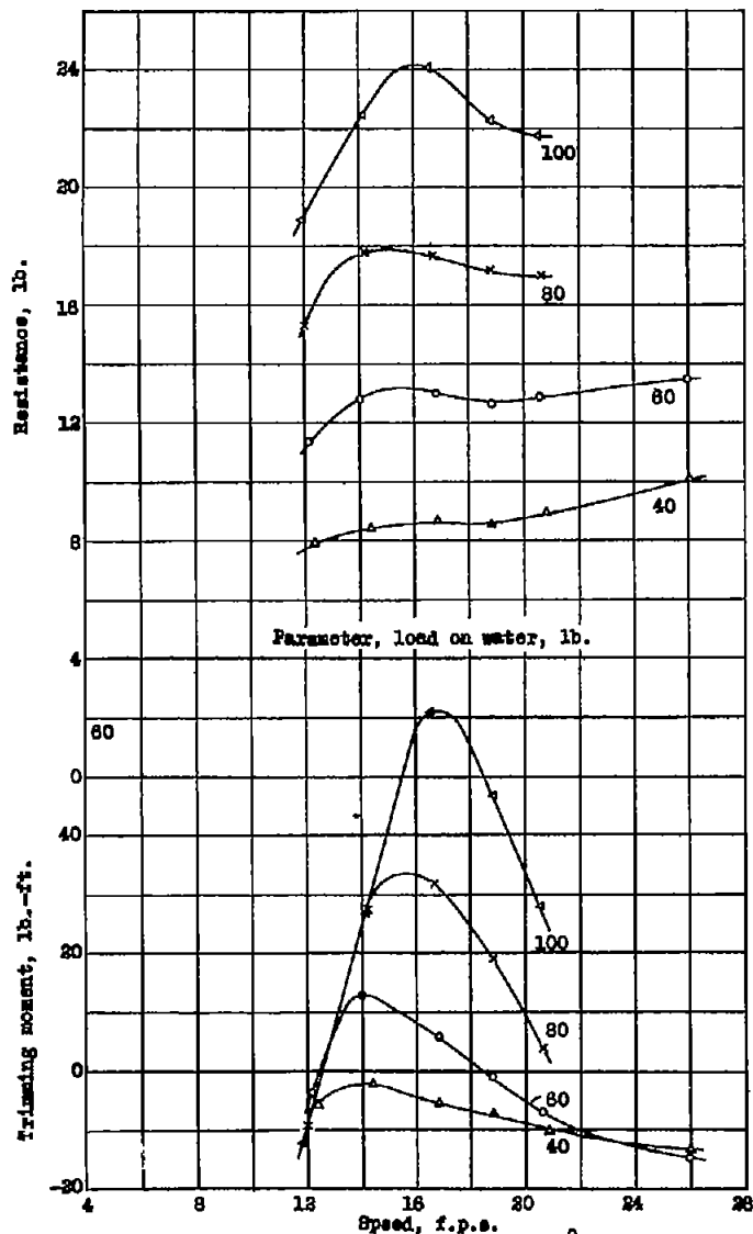
Figure 26.- Resistance and trimming moment, \tau = 9^\circ , Model 11-0-8 ( 7^\circ angle of afterbody keel.)
