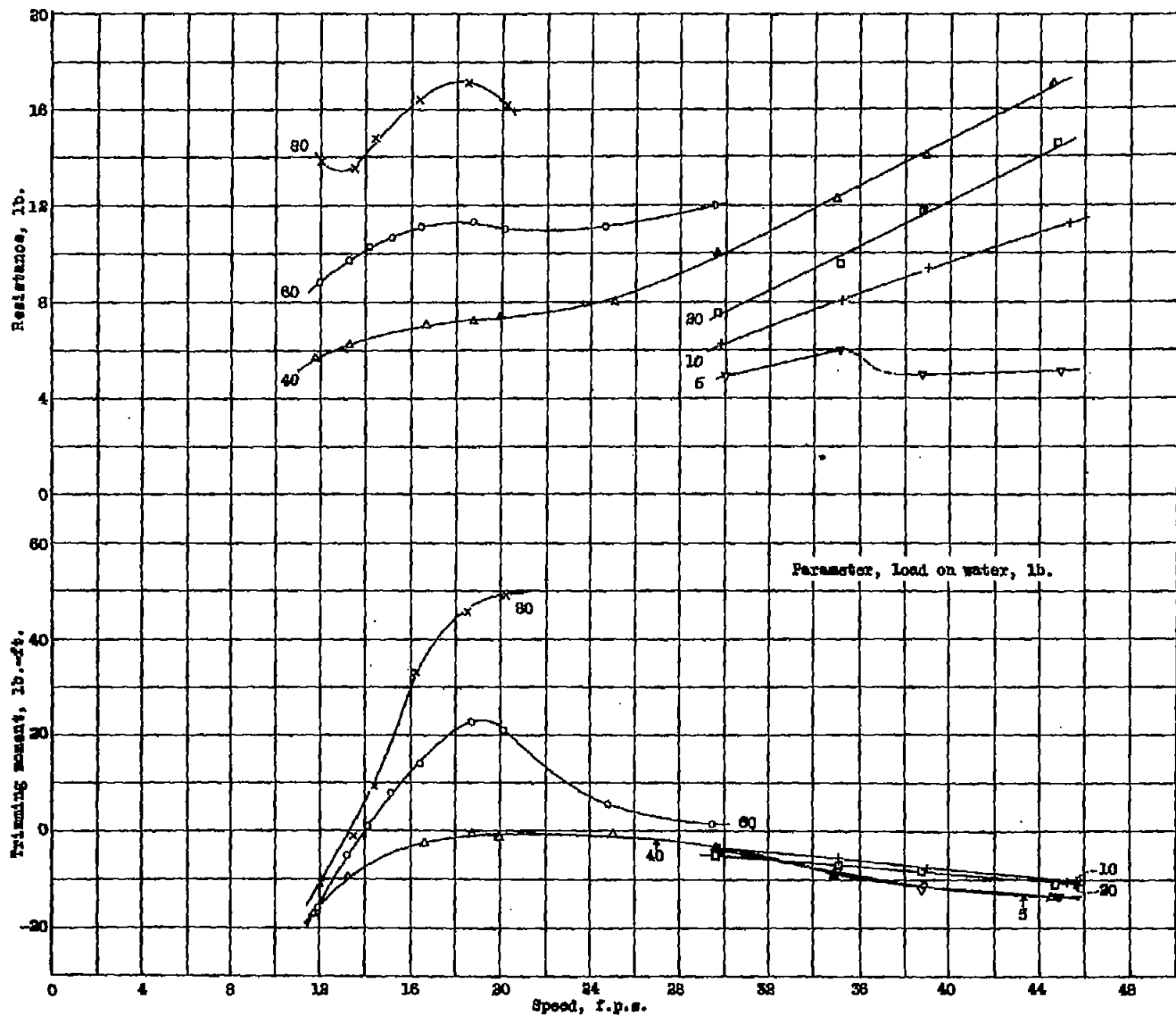
Figure 6.- Resistance and trimming moment, \tau = 5^\circ , Model 11-0-7 ( 21/2^\circ angle of afterbody keel).
