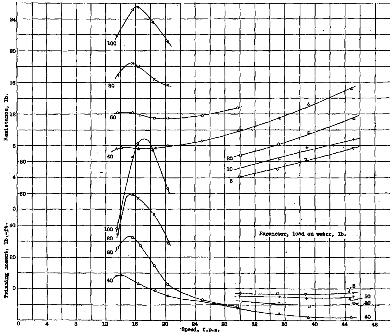
Figure 25.- Resistance and trimming moment, \tau = 7^\circ . Model 11-0-0, ( 7^\circ angle of afterbody keel).
