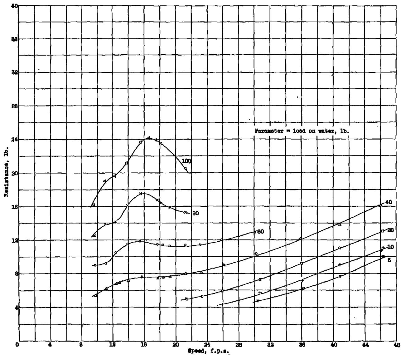
Figure 19a.-Resistance. \gamma = 7^\circ . Model 11-C. ( 5\frac{10}{2} angle of afterbody keel)
