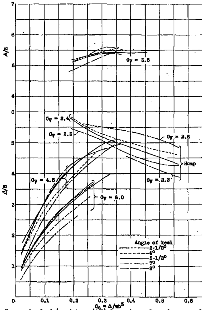
Figure 39.- Load / resistance ( \Delta/R ) for various values of speed coefficient
