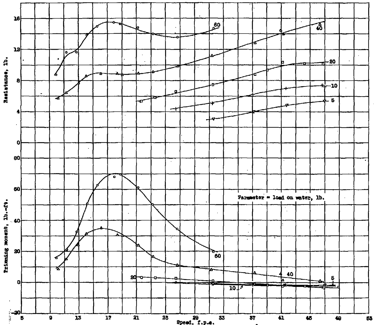
Figure 17.-Resistance and trimming moment, \tau = 3^\circ . Model 11-C. ( 5\frac{1}{2}^\circ angle of afterbody keel)
