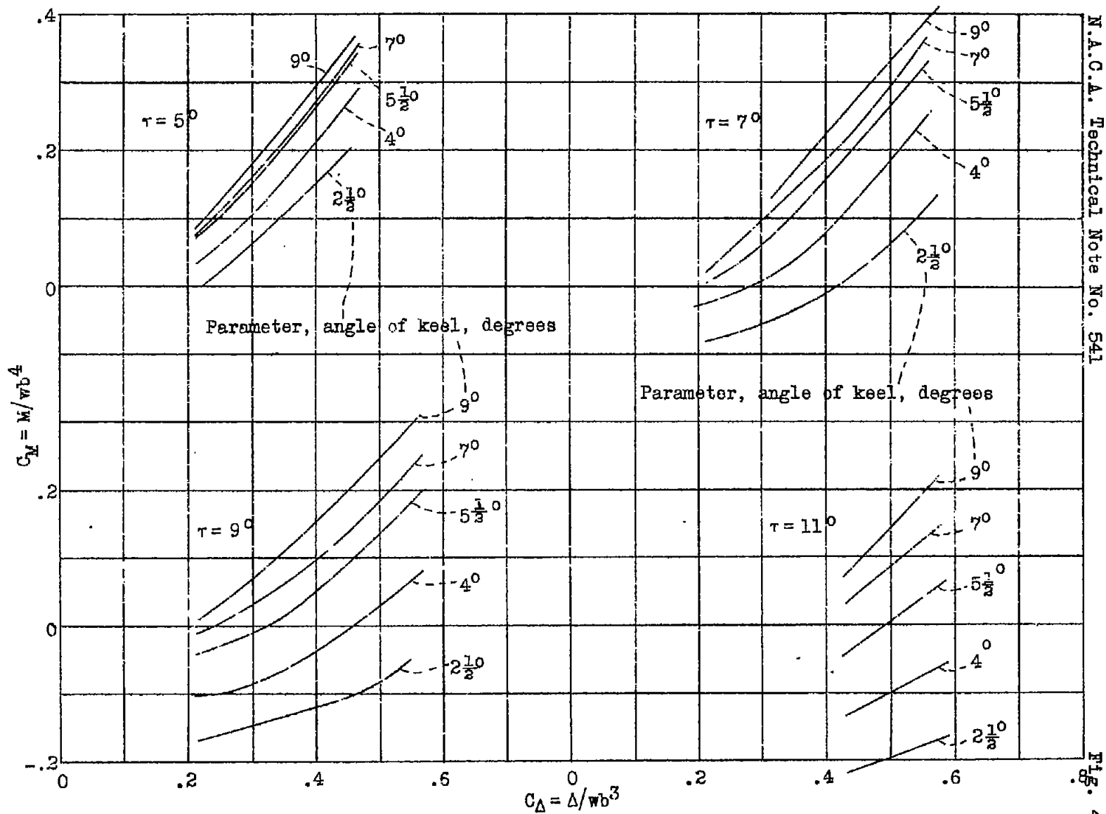
Figure 41.- Maximum trimming moment coefficient, positive direction.
