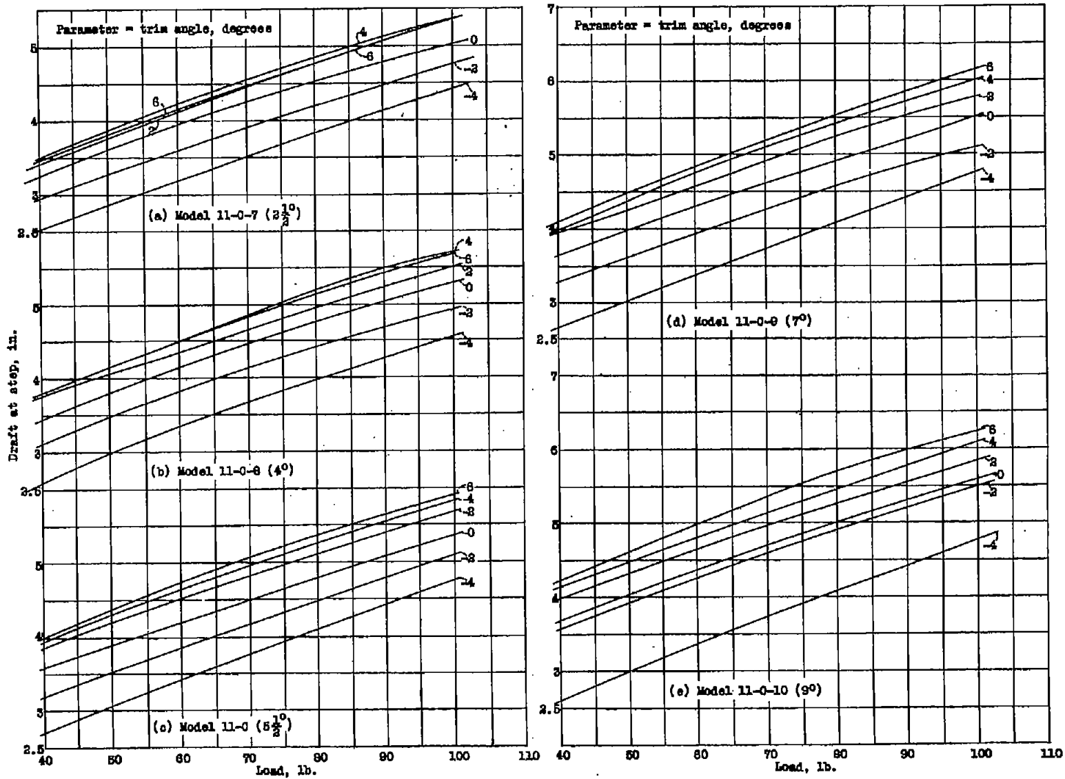
Figure 43.--Drafts at rest for various angles of afterbody heel.
