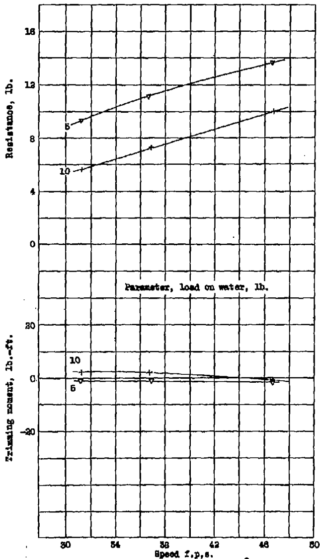
Figure 2.- Resistance and trimming moment, T = 1^\circ , Model 11-C-7 ( 2\text{-}1/2^\circ angle of afterbody keel.)
