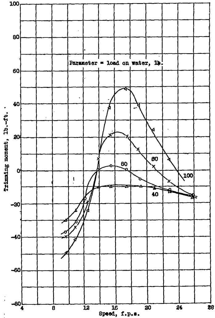
Figure 20b.-Trimming moment. \tau = 9^\circ . Model 11-0. ( 5\frac{1}{2}^\circ angle of afterbody keel.)
