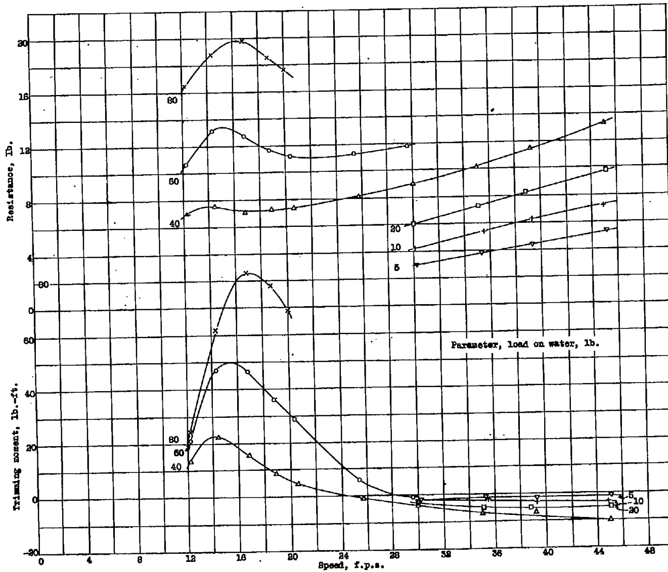
Figure 24.- Resistance and trimming moment, \tau = 5^\circ . Model 11-0-9 ( 7^\circ angle of afterbody keel).
