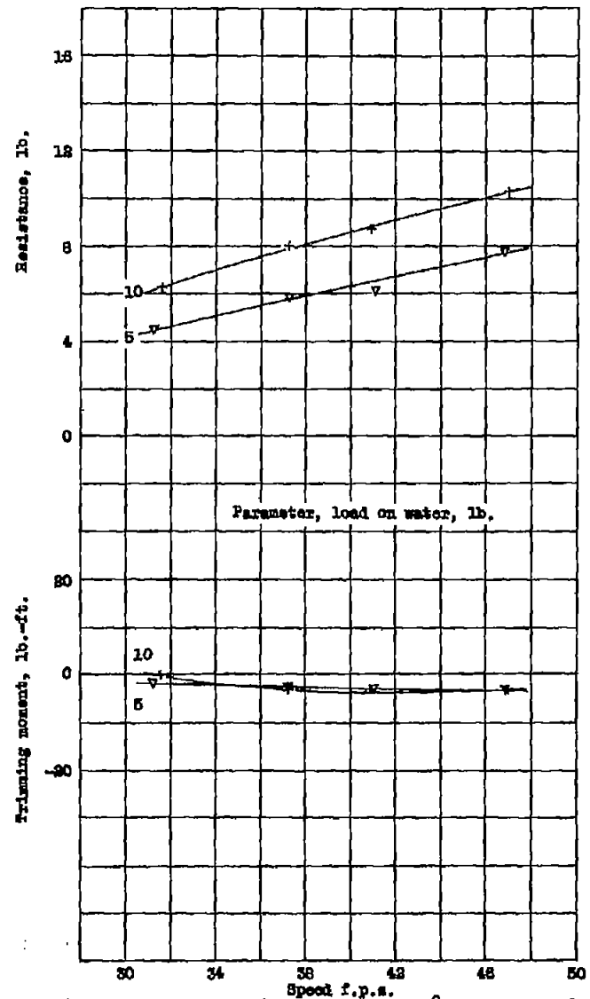
Figure 3.- Resistance and trimming moment, T = 2^\circ , Model 11-C-10 ( 2\text{-}1/2^\circ angle of afterbody keel.)
