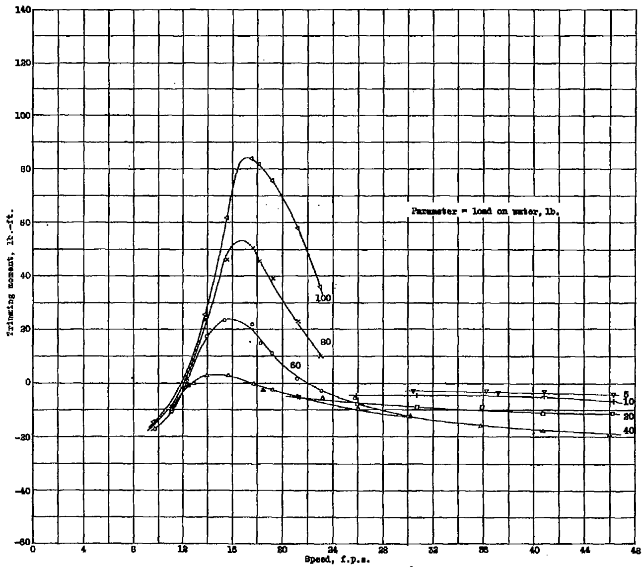
Figure 19b.-Trimming moment. \gamma = 7^\circ . Model 11-0. ( 5\frac{1}{8}^\circ angle of afterbody keel)
