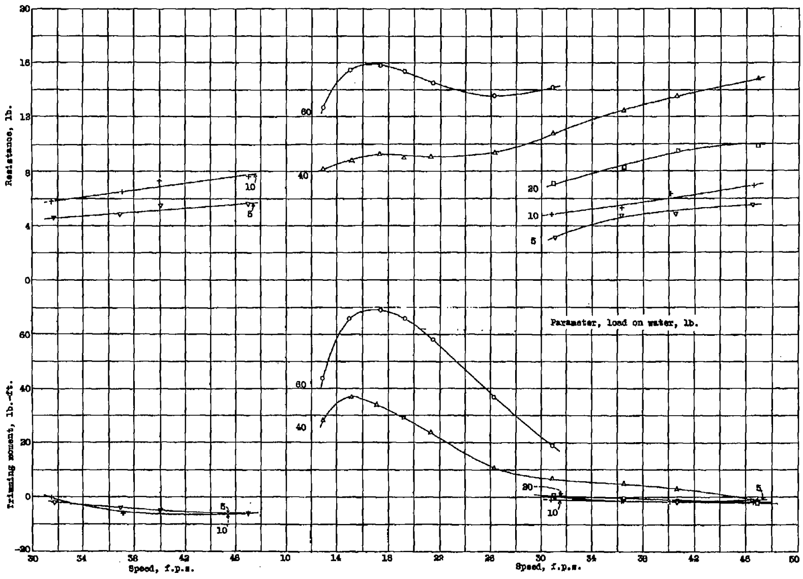
Figure 22.- Resistance and trimming moment, \gamma = 20^\circ , Model 11-C-9 (70° angle of afterbody keel)
