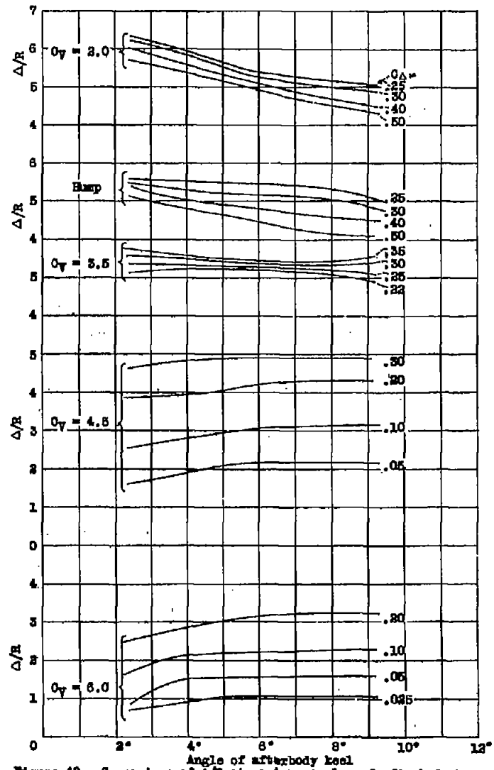
Figure 40.- Comparison of \Delta/R at various angles of afterbody keel
