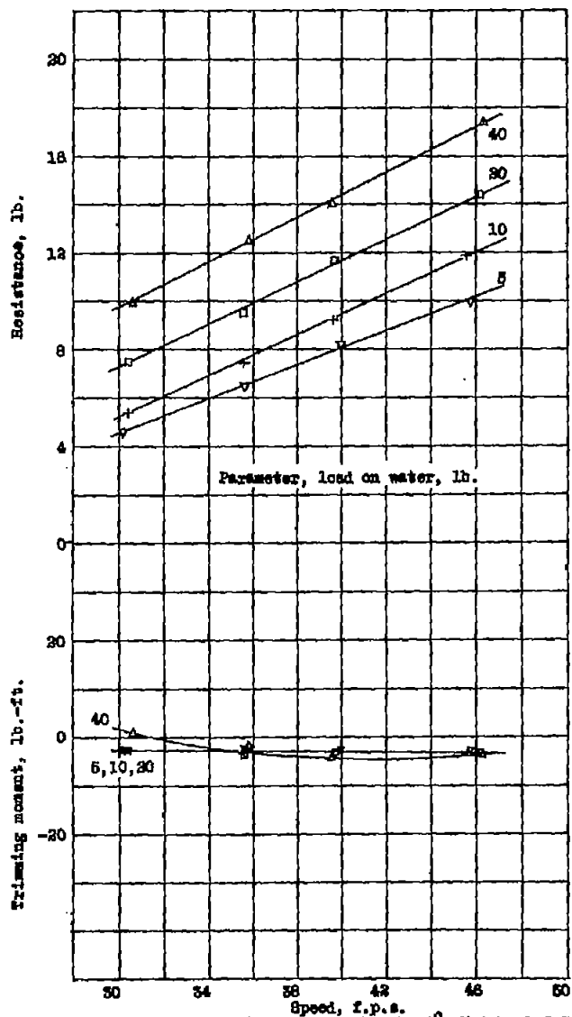
Figure 5.- Resistance and trimming moment, \tau = 4^\circ , Model 11-0-7 ( 2\frac{1}{2}^\circ angle of afterbody keel.)
