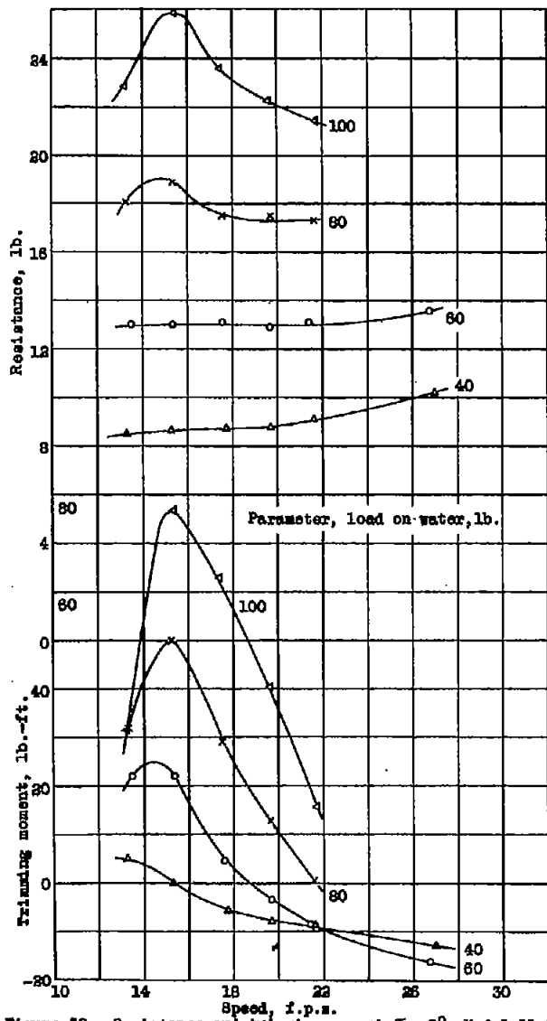
Figure 32.- Resistance and trimming moment, T = 9^\circ , Model 11-C-10 ( 9^\circ angle of afterbody keel.)
