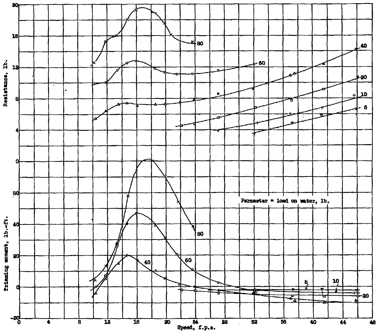
Figure 18.-Resistance and trimming moment. \tau = 5^\circ . Model 11-0. ( 5\frac{1}{2}^\circ angle of afterbody keel)
