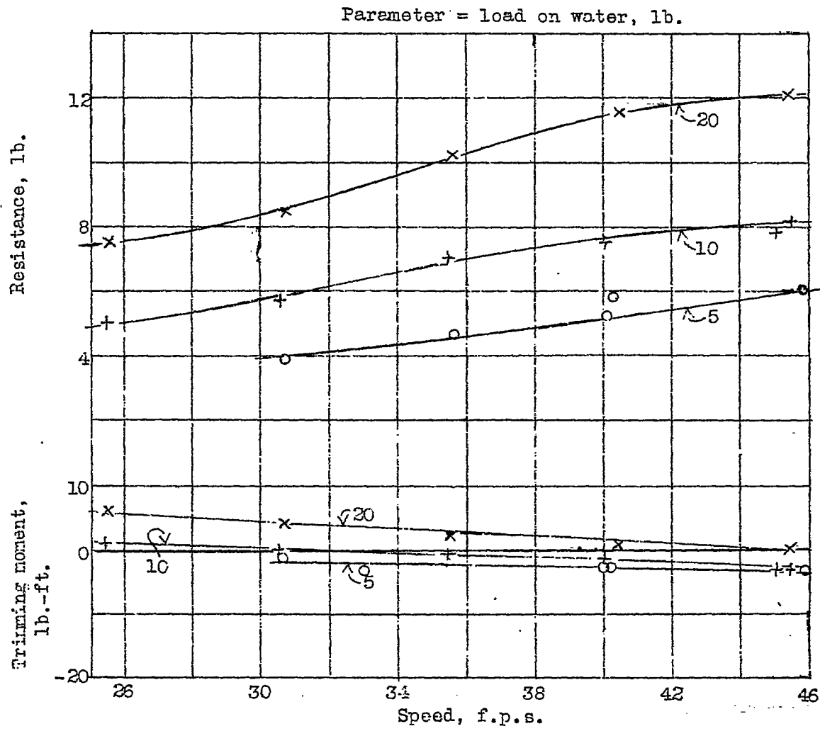
Figure 16 -Resistance and trimming moment, \tau = 2^\circ . Model 11-C. ( 5\frac{1}{2}^\circ angle of afterbody keel).
