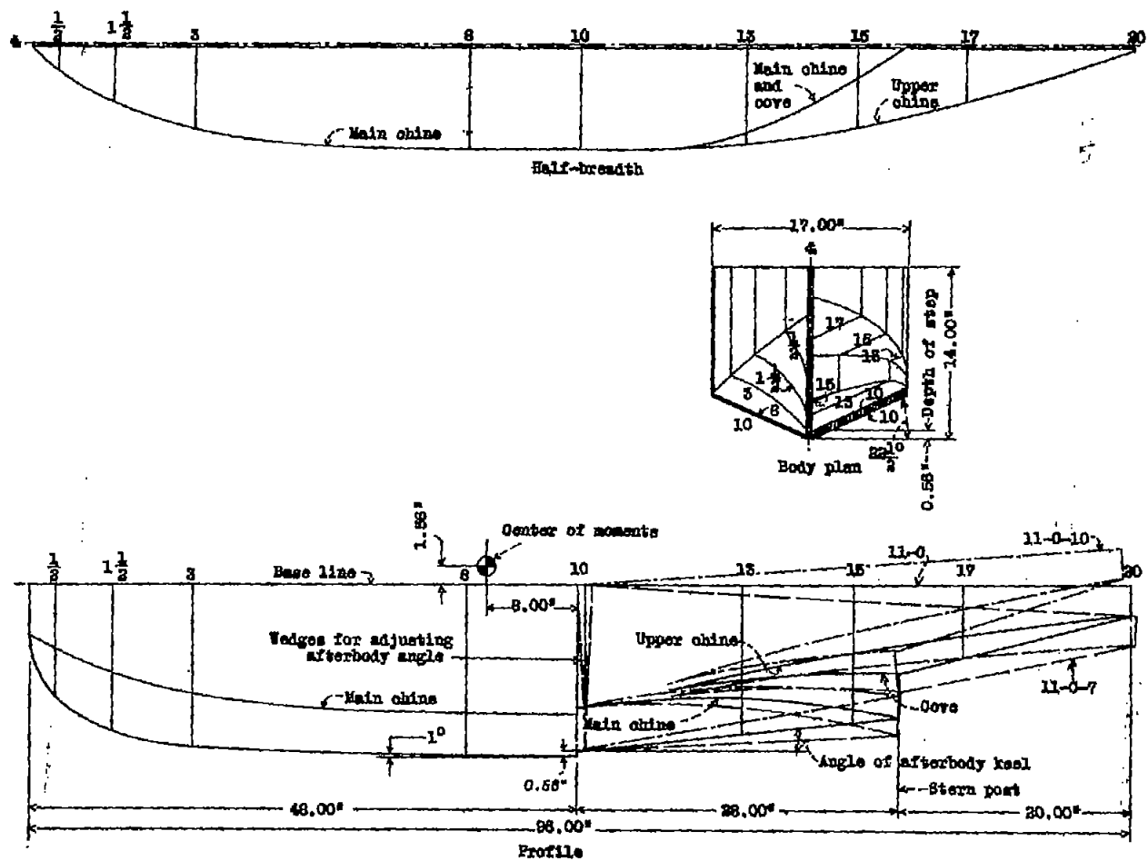
Figure 1.-Model 11-0 Angle of keel variations
