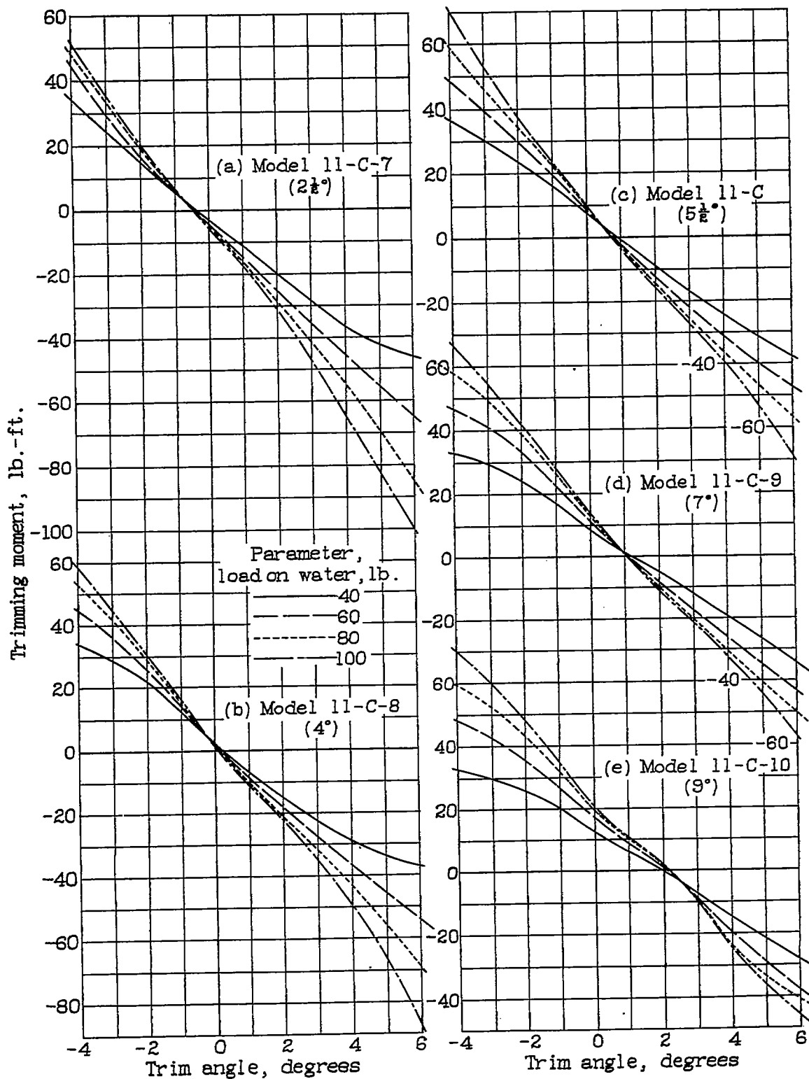
Figure 42-Static trimming moments for various angles of afterbody keel.
