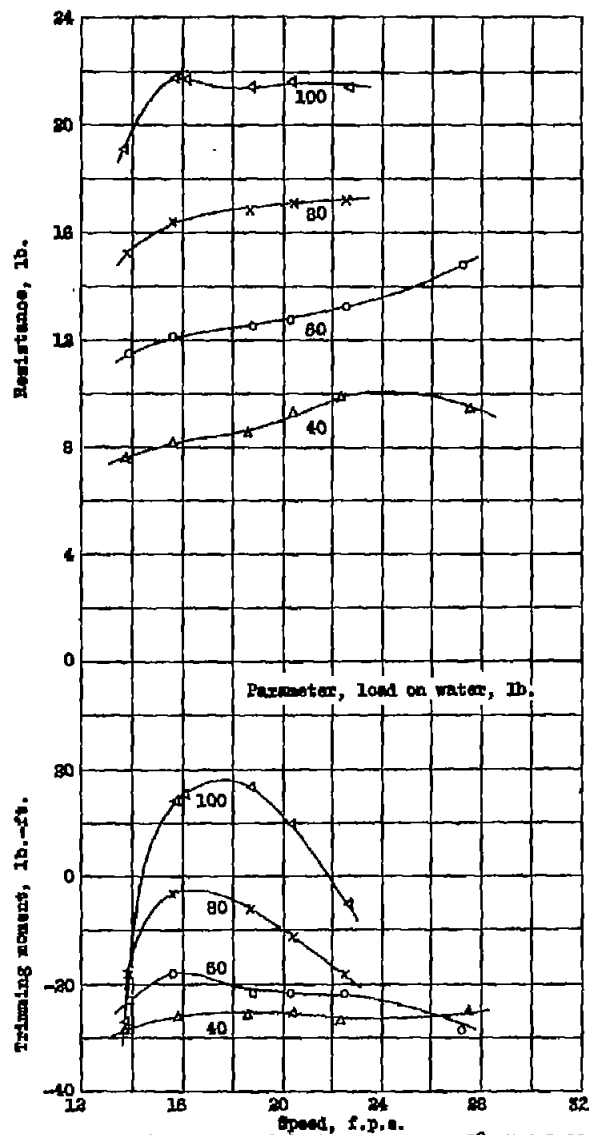
Figure 14.- Resistance and trimming moment, \tau = 90^\circ , Model 11-0-8 ( 4^\circ angle of afterbody keel.)
