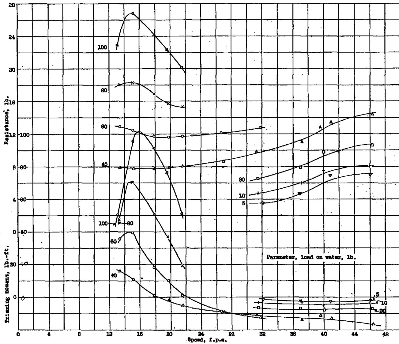
Figure 31.- Resistance and trimming moment, \tau = 9^\circ . Model 11-0-10 ( 9^\circ angle of afterbody keel)
