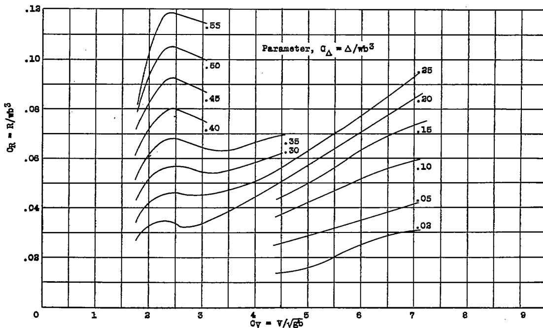
Figure 35.- Resistance coefficient at best trim angle, Model 11-C-8 (4° angle of afterbody keel.)
