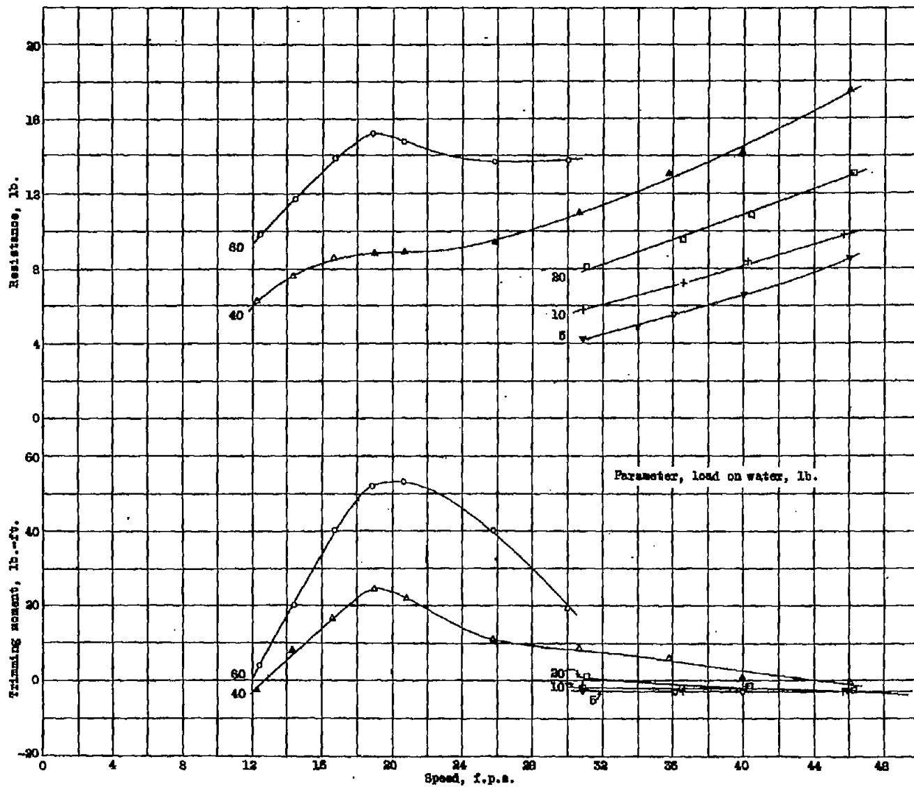
Figure 4.- Resistance and trimming moment, \tau = 3^\circ . Model 11-0-7 ( 2\frac{1}{2}^\circ angle of afterbody keel).
