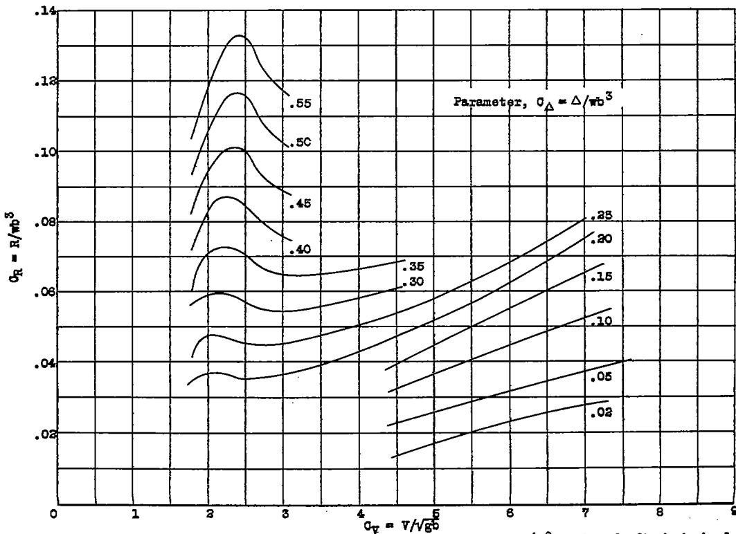
Figure 37.- Resistance coefficient at best trim angle, Model 11-C-9 ( 7^\circ angle of afterbody keel.)
