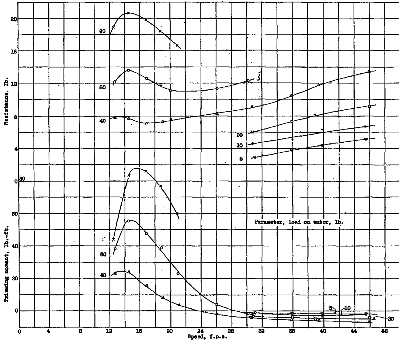
Figure 30.- Resistance and trimming moment, \tau = 5^\circ . Model 11-C-10, ( 90^\circ angle of afterbody keel)
