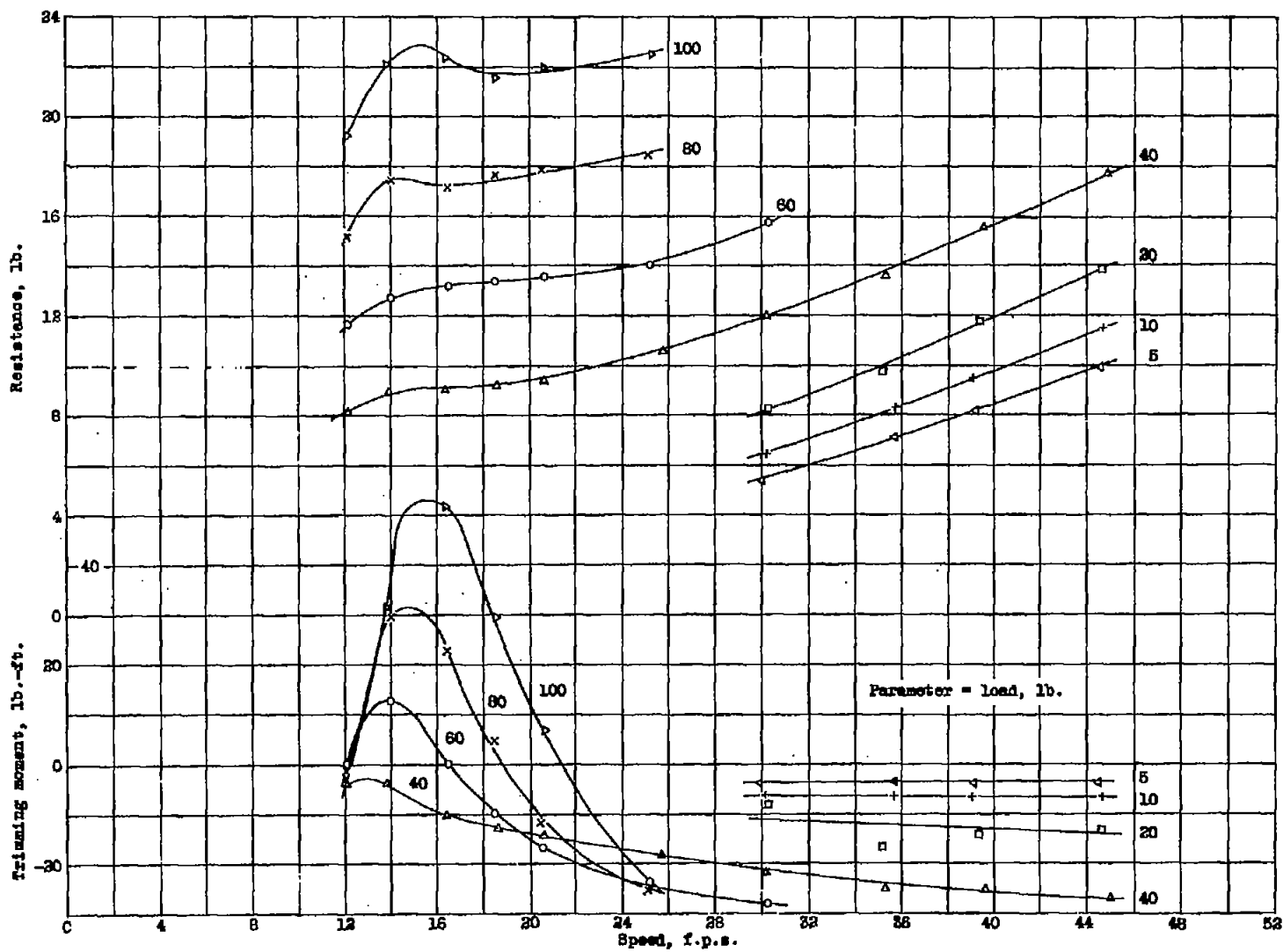
Figure 6.- Resistance and trimming moment, \tau = 7^\circ
