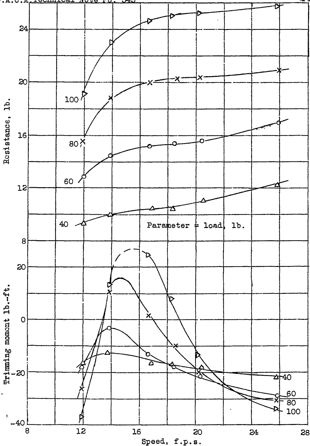
Figure 7.- Resistance and trimming moment, \tau = 9^\circ
