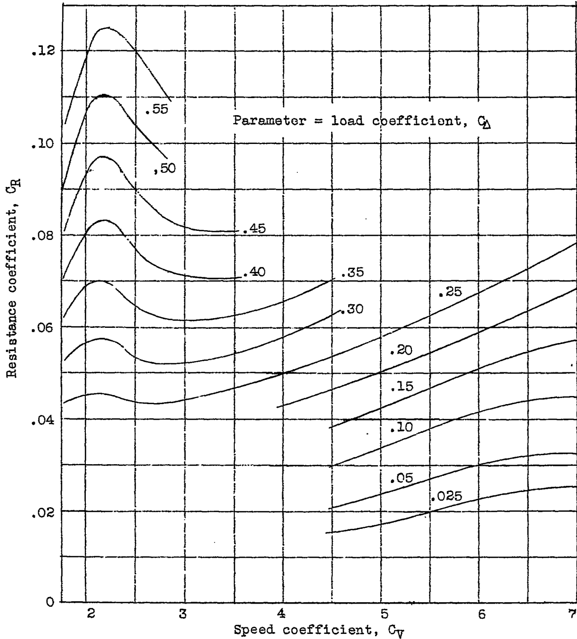
Figure 8.- Resistance coefficient at best trim angle.
