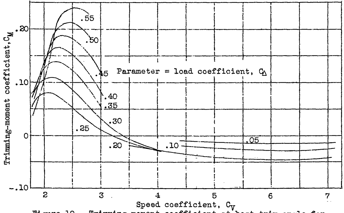
Figure 10.- Trimming moment coefficient at best trim angle for center of moments 47.06 percent beam forward of the step and 97.41 percent beam above the keel at the step.
