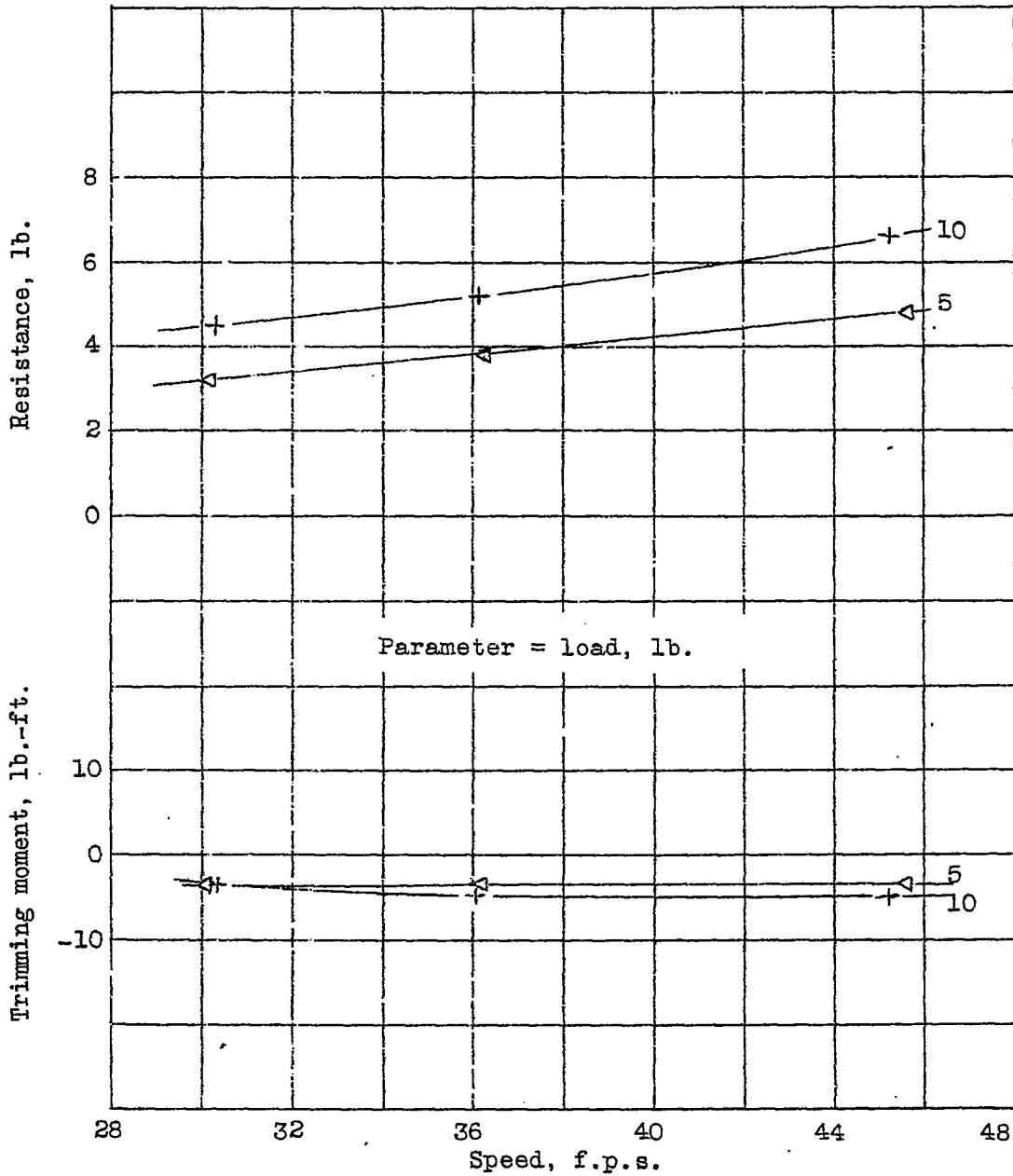
Figure 2.- Resistance and trimming moment. Trim angle, \tau = 0^\circ
