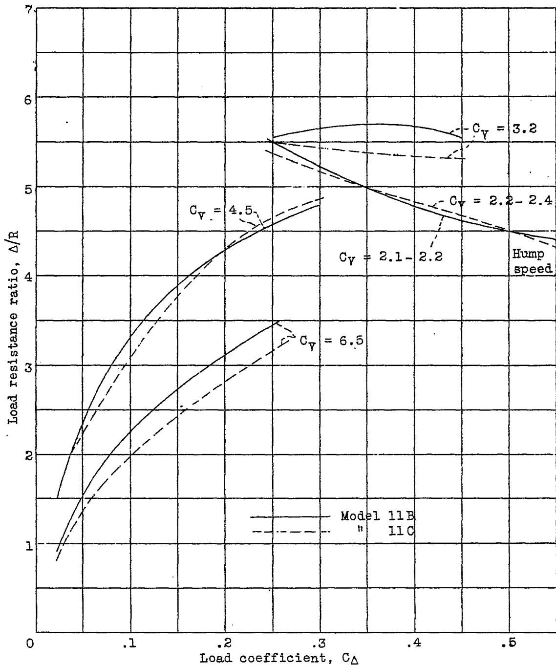
Figure 11.- Effect of concave planing bottom on \Delta/R at best trim angle.
