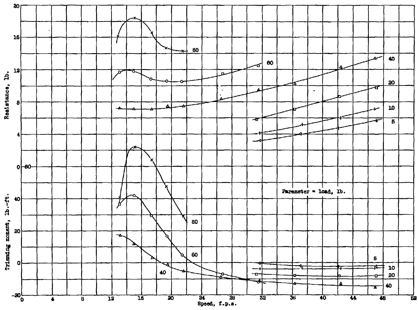
Figure 4.- Resistance and trimming moment, \gamma = 30^\circ
