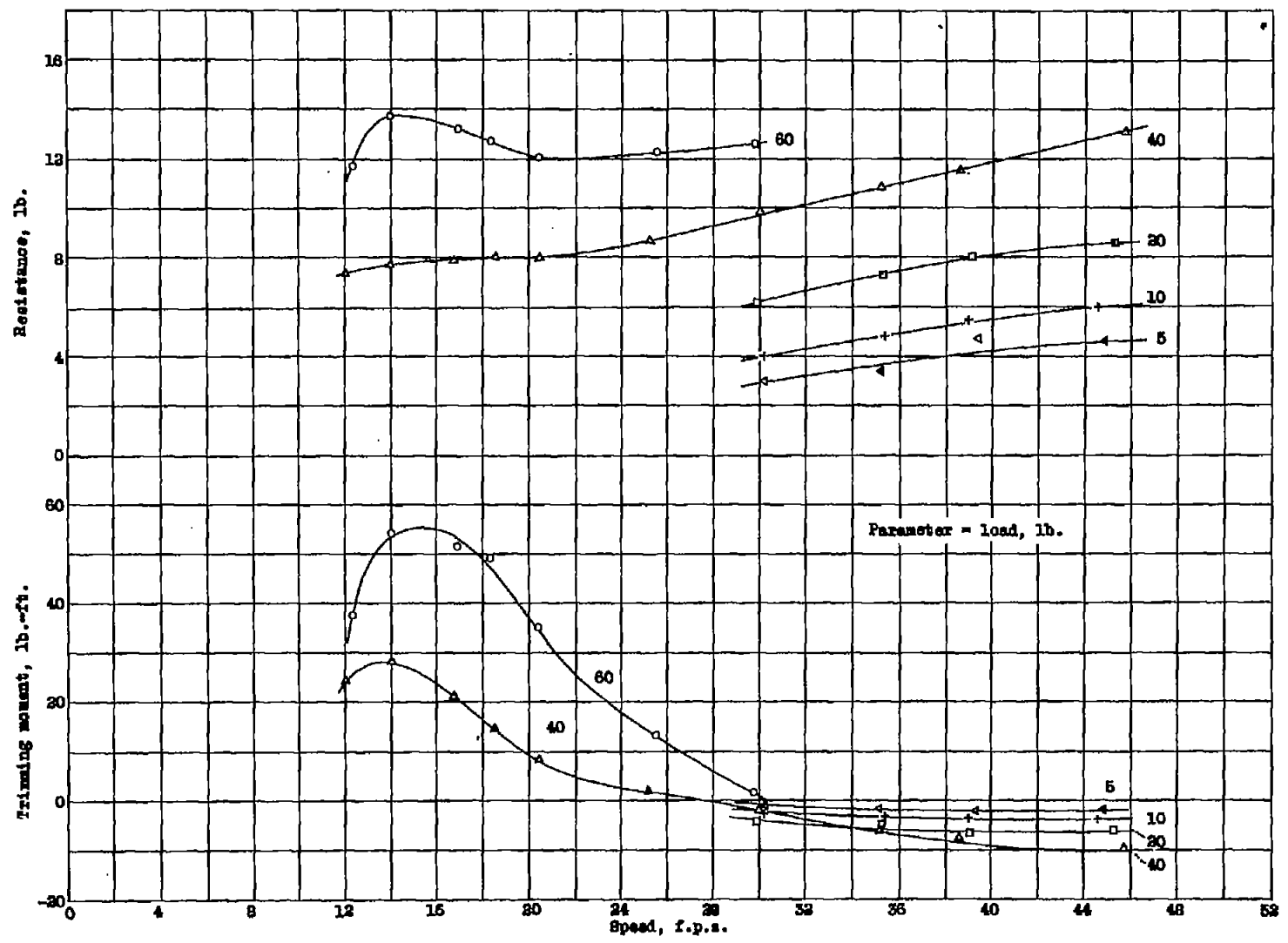
Figure 3.- Resistance and trimming moment, \tau = 1^\circ
