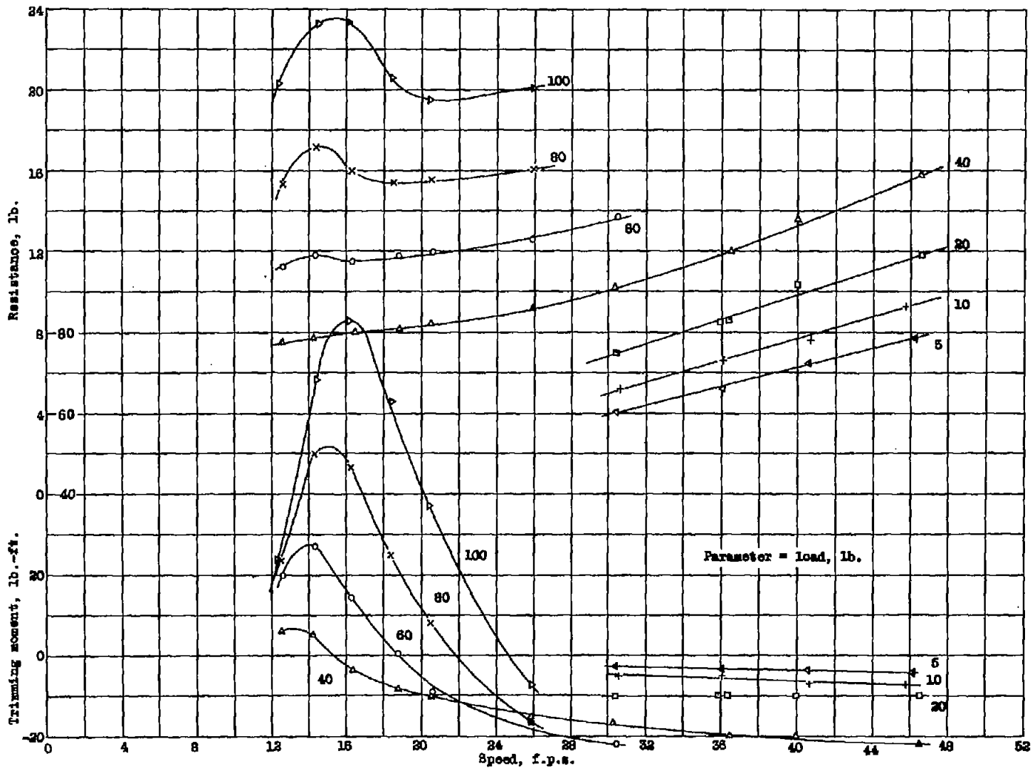
Figure 5.- Resistance and trimming moment, \gamma = 5^\circ
