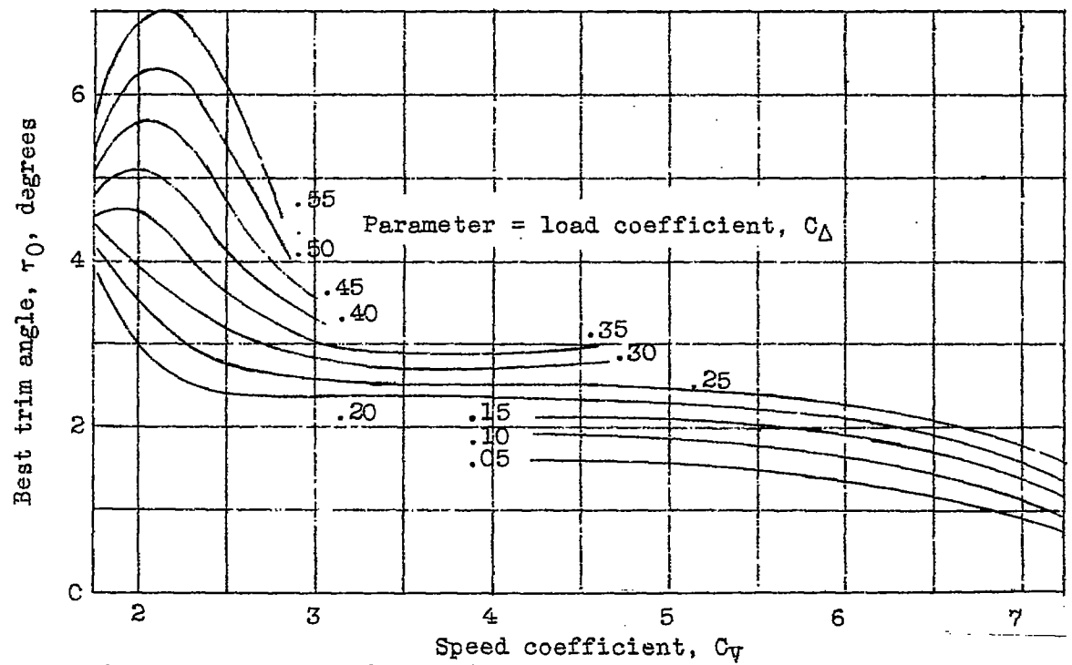
Figure 9.- Angle of trim for minimum resistance
