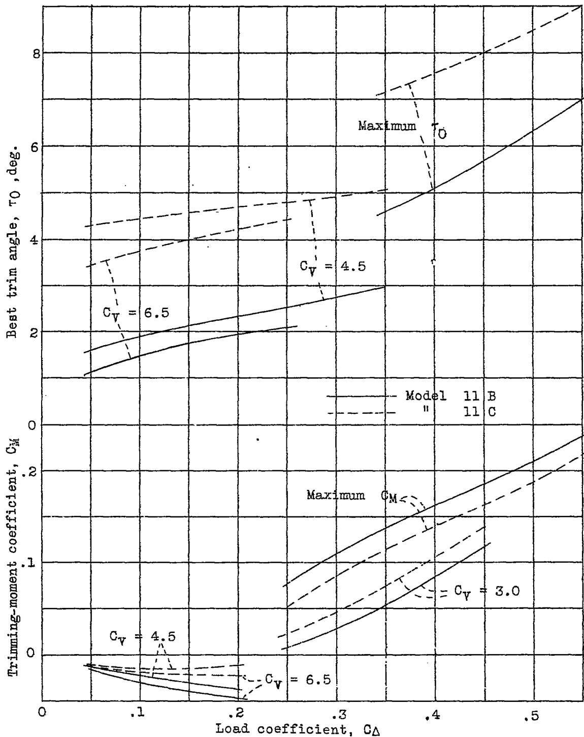
Figure 12.- Effect of concave planing bottom on best trim angle and trimming moment coefficient at best trim angle.
