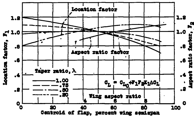
Figure 1.- Lift increments for ordinary flaps.
