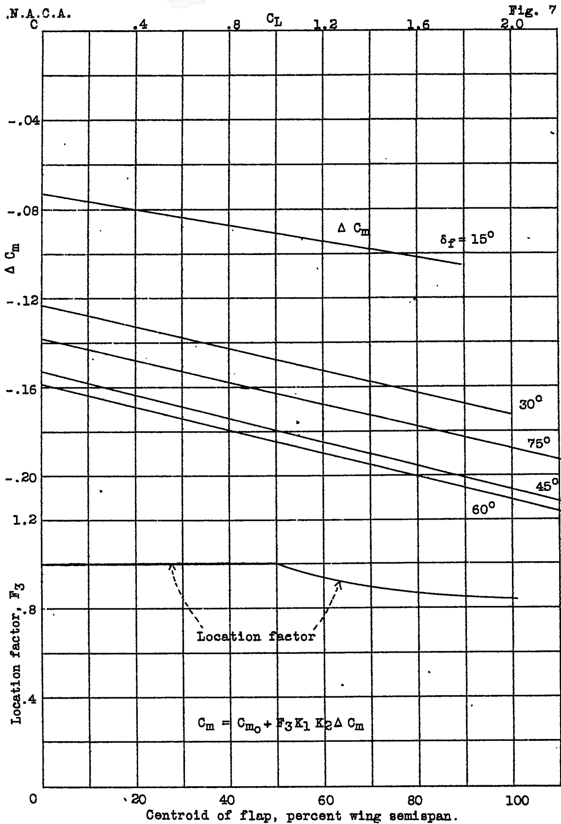
Figure 7.- Pitching-moment increments for simple split flaps.
