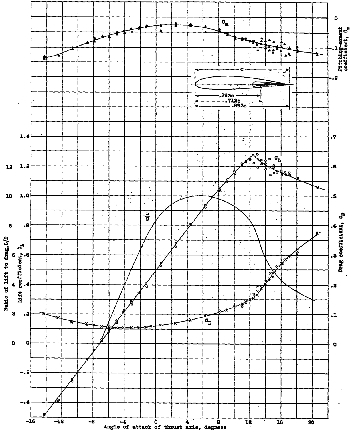
Figure 8a.- Aerodynamic characteristics of Fairchild-22 airplane with 30-percent Fowler flap. Flap retracted. Propeller and horizontal tail surfaces removed. Results corrected for tunnel effects. Test velocity, approximately 69 m.p.h.
