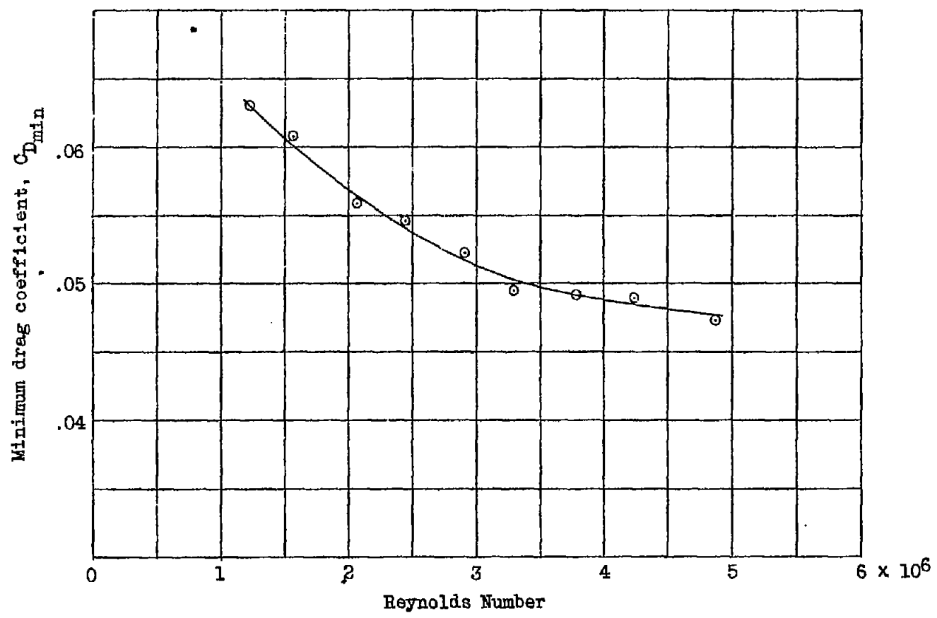
Figure 12.- Scale effect on the minimum drag coefficient with flap retracted. Fairchild 22 airplane with 30-percent Fowler flap. Flap fully retracted. Propeller and horizontal tail surfaces removed.
