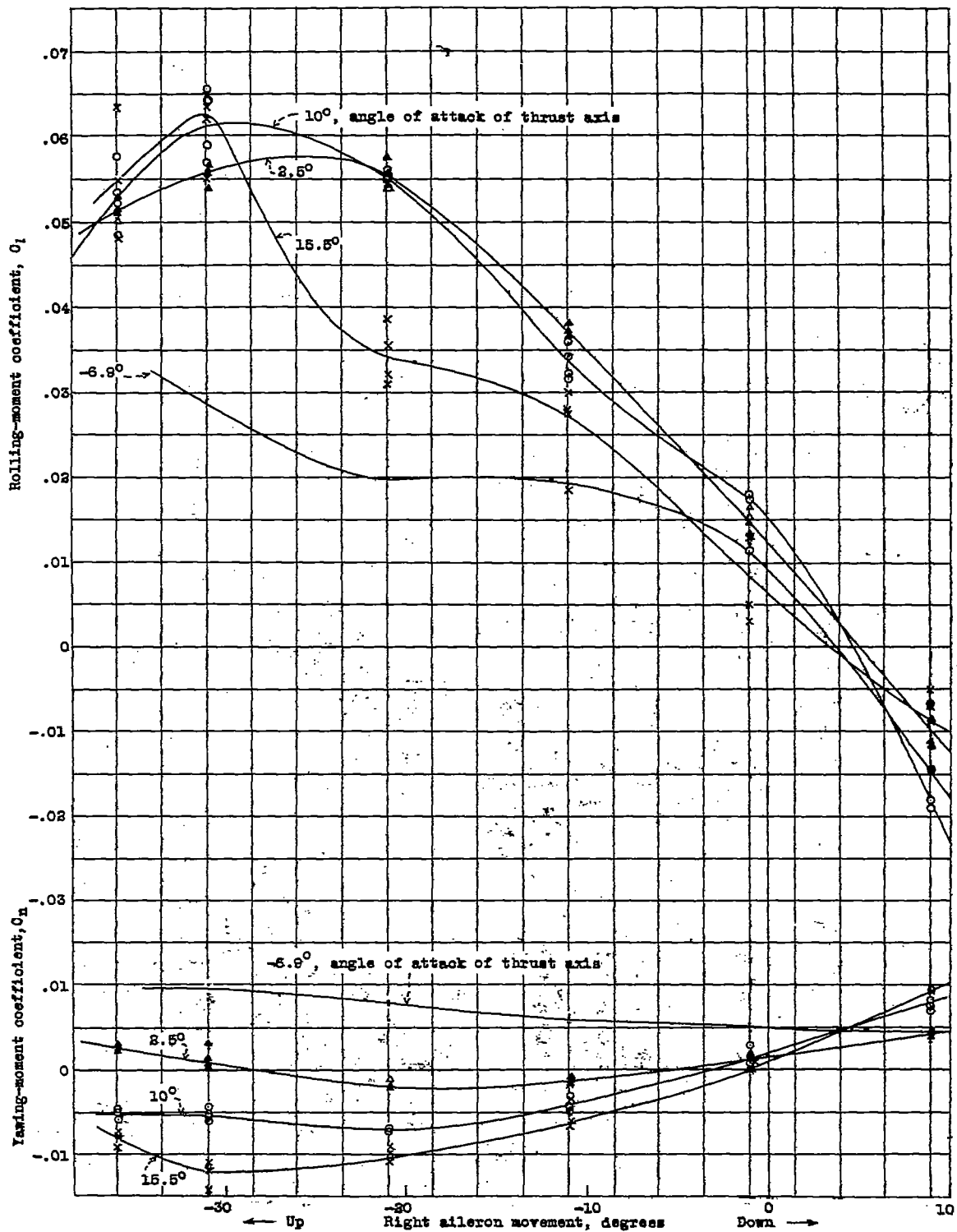
Figure 15.- Rolling- and yawing-moment coefficients due to ailerons. Flap retracted. Fairchild-22 airplane with 20-percent Fowler flap. Propeller and horizontal tail surfaces removed.
