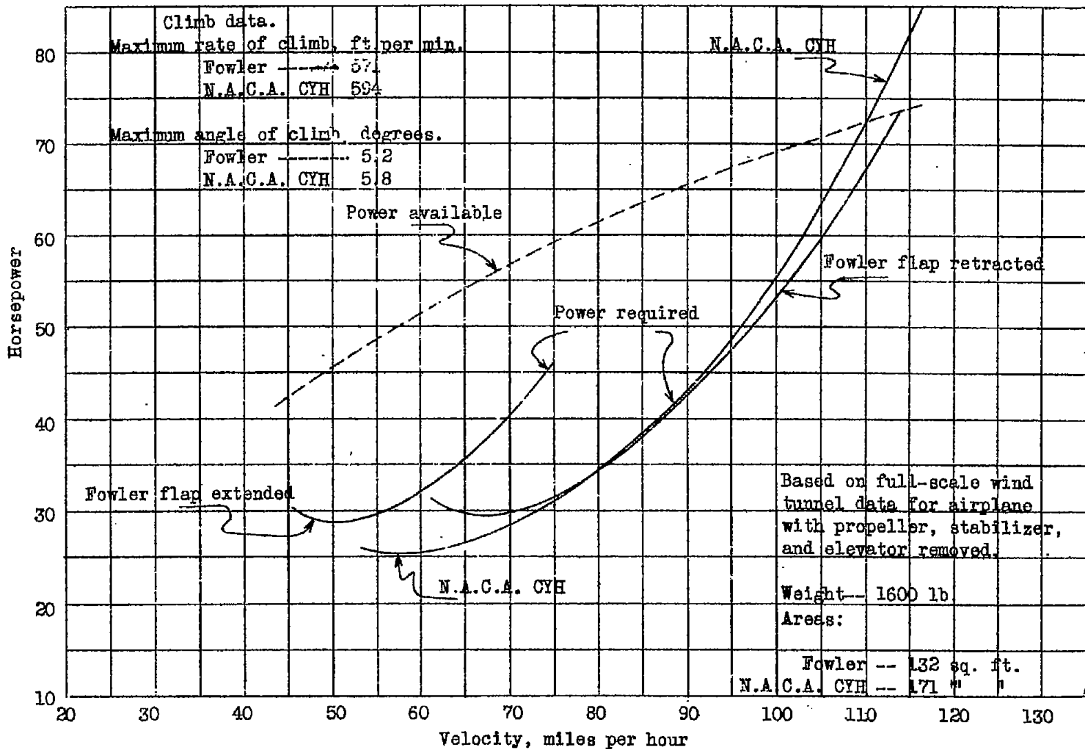
Figure 16.- Power curves for Fairchild 22 airplane for extreme positions of Fowler flap.
