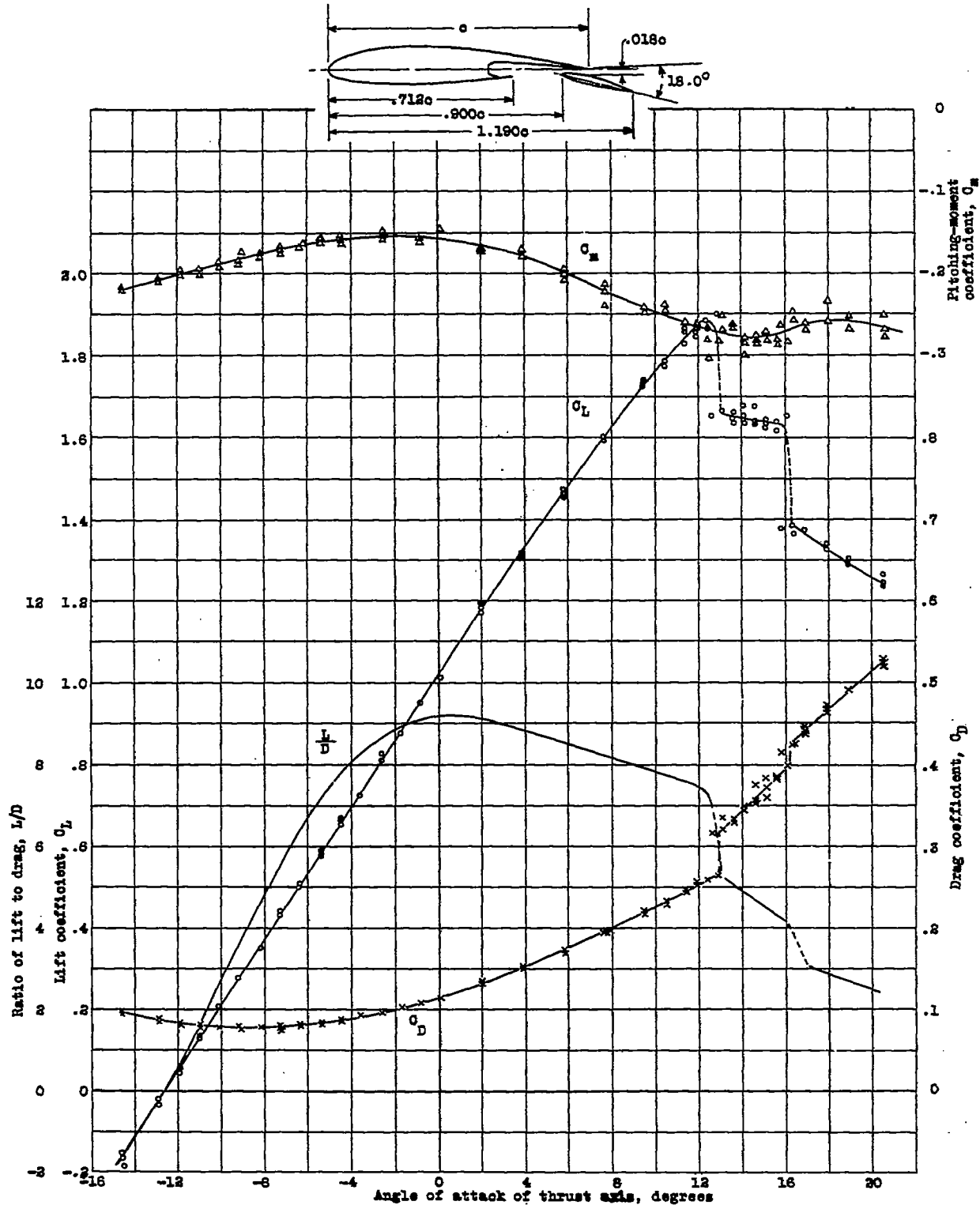
Figure 9c.- Aerodynamic characteristics of Fairchild 22-airplane with 30-percent Fowler flap. Flap extended 4.25 turns of crank. Propeller and horizontal tail surfaces removed. Results corrected for tunnel effects. Test velocity, approximately 58 m.p.h.
