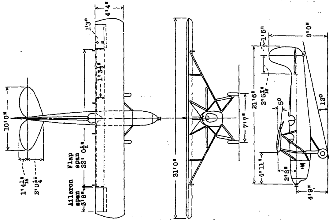
Figure 1.-Installation of Fowler wing on Fairchild-22 airplane.
