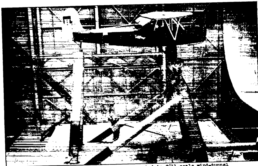
Figure 8.-Fairchild 22 airplane mounted in full-scale wind-tunnel
