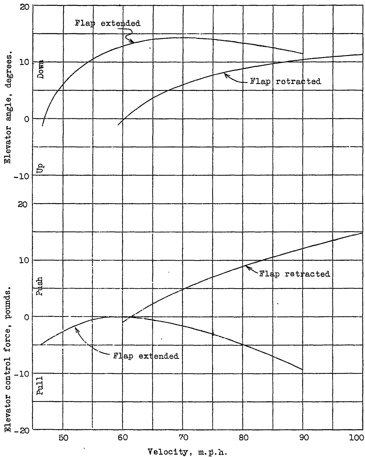
Figure 23.- Effect of Fowler flap on elevator angles and stick forces. Power-off. Stabilizer, full tail heavy.
