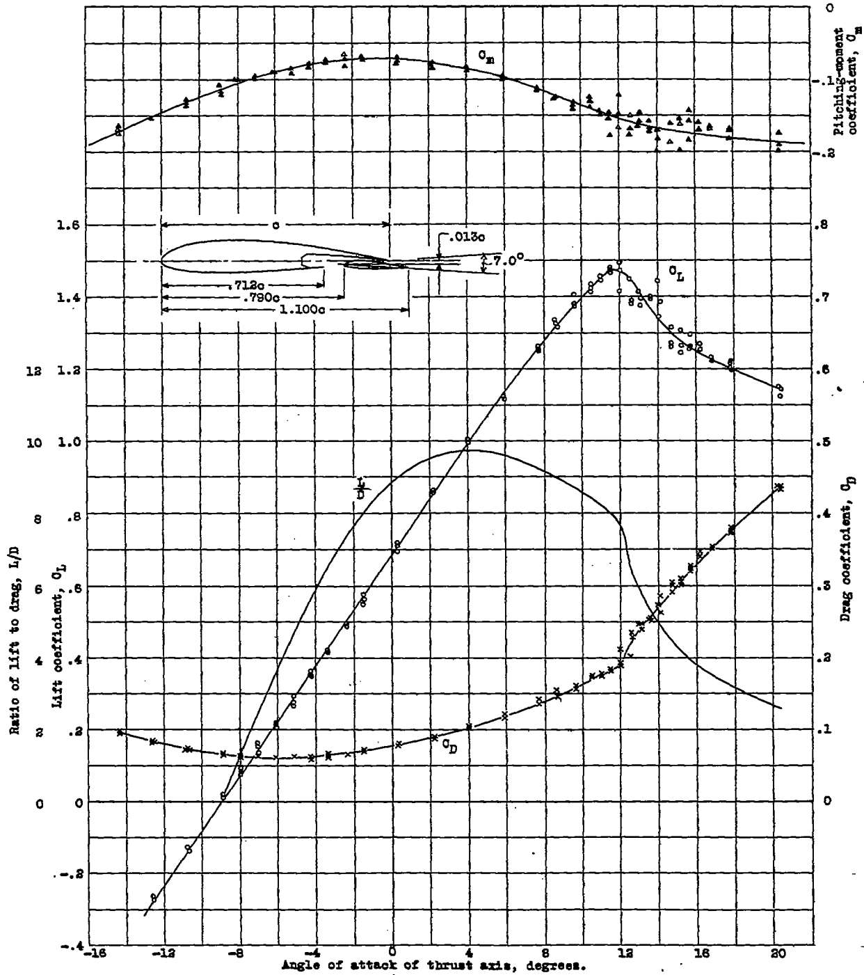
Figure 9b.- Aerodynamic characteristics of Fairchild-28 airplane with 30-percent Fowler flap. Flap extended 2.35 turns of crank. Propeller and horizontal tail surfaces removed. Results corrected for tunnel effects. Test velocity, approximately 55 m.p.h.
