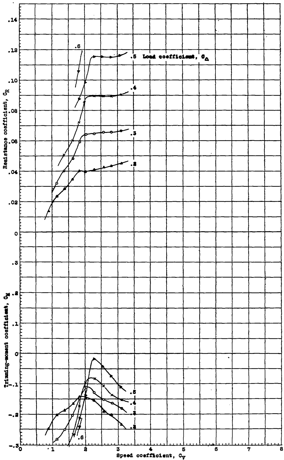
Figure 10. Resist- ance and trimming- moment coeffi- cients. N.A.C.A. model 47. \tau = 13^\circ
