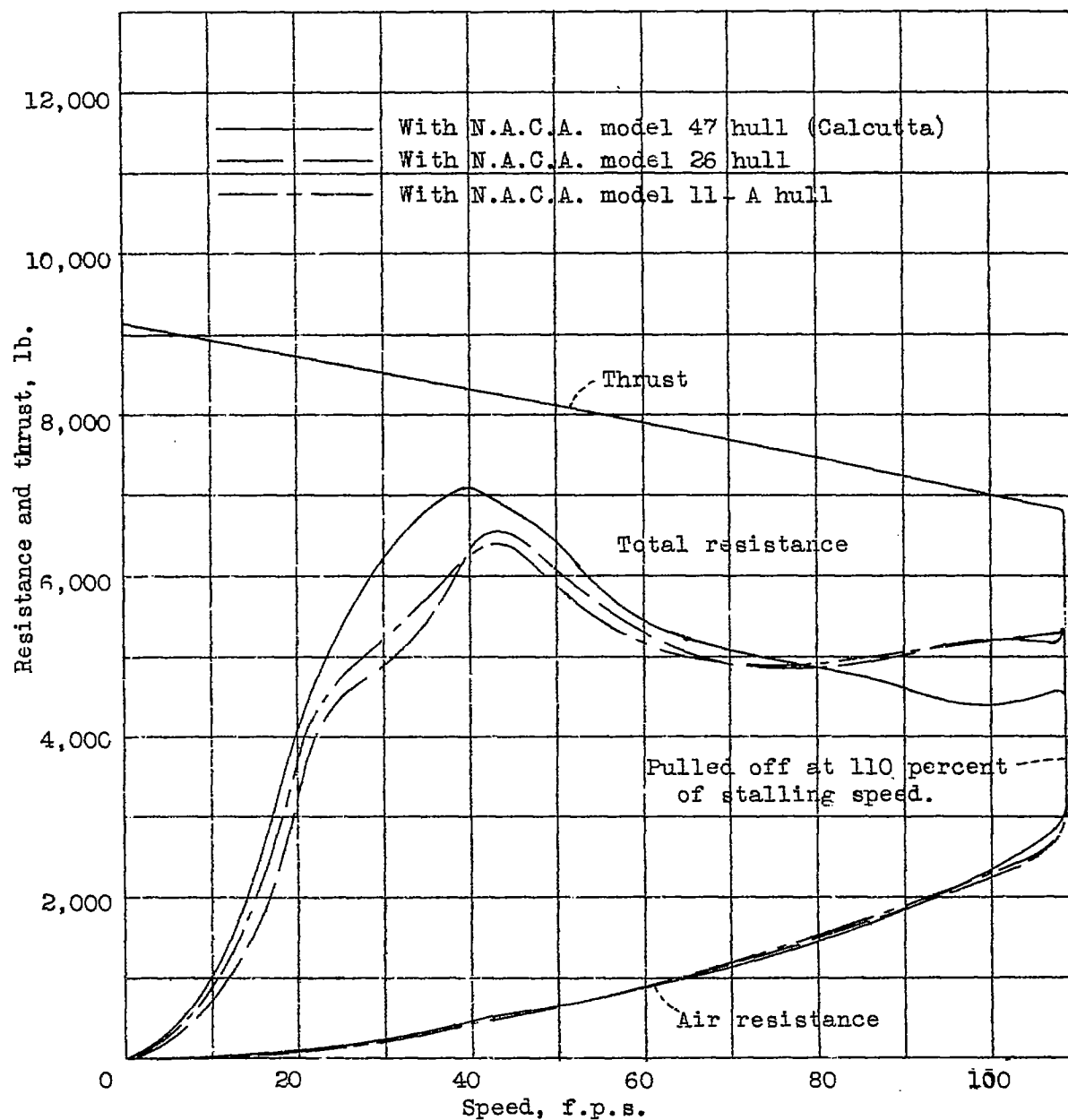
Figure 21.- Resistance and thrust for take-off with 35,000 lb. load.
