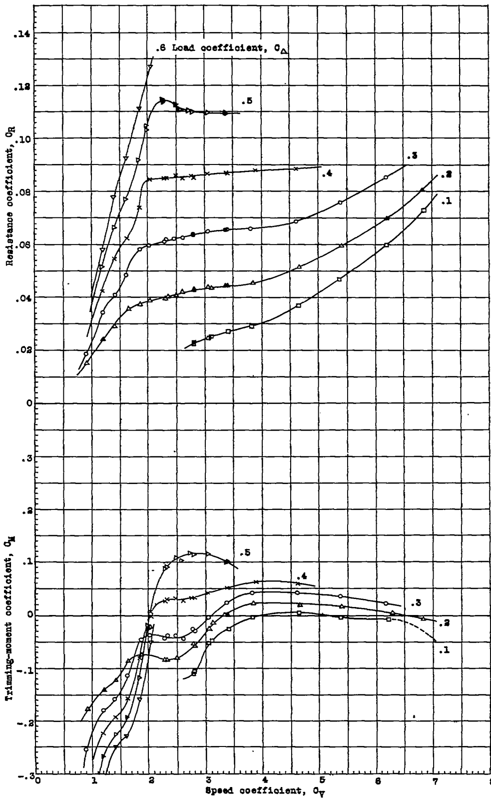
Figure 9. Resist- ance and trimm- ing- moment coeffi- cients, \tau = 11^\circ . N.A.C.A. model 47
