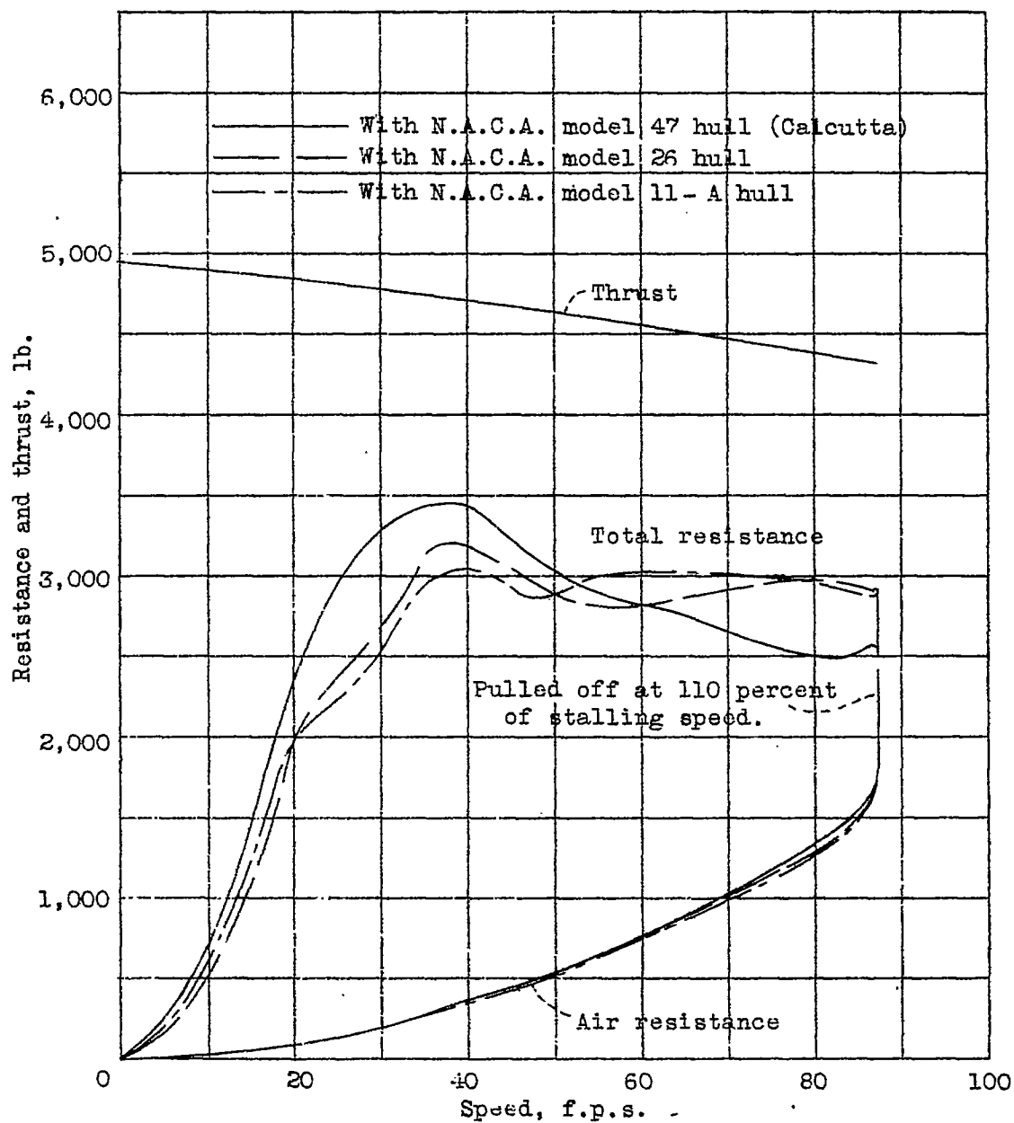
Figure 20.- Resistance and thrust for take-off with 20,000 lb. load.
