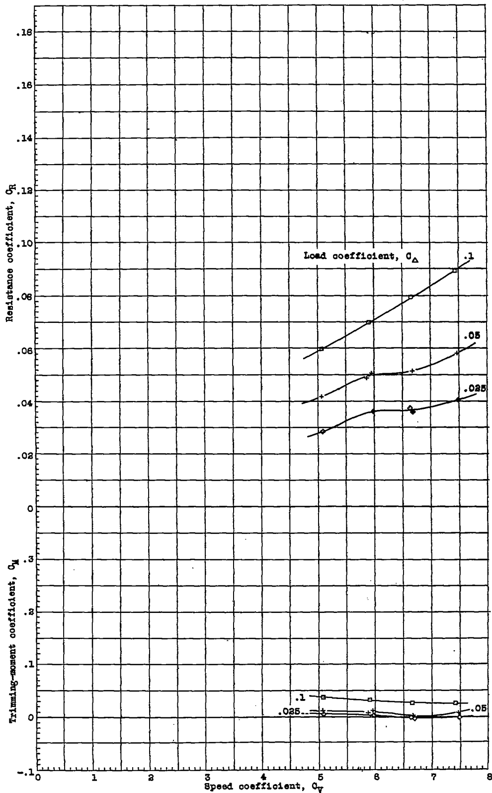
Figure 5. Resist- ance and trimming- moment coeffi- cients, \tau = 3^\circ . N.A.C.A. model 47
