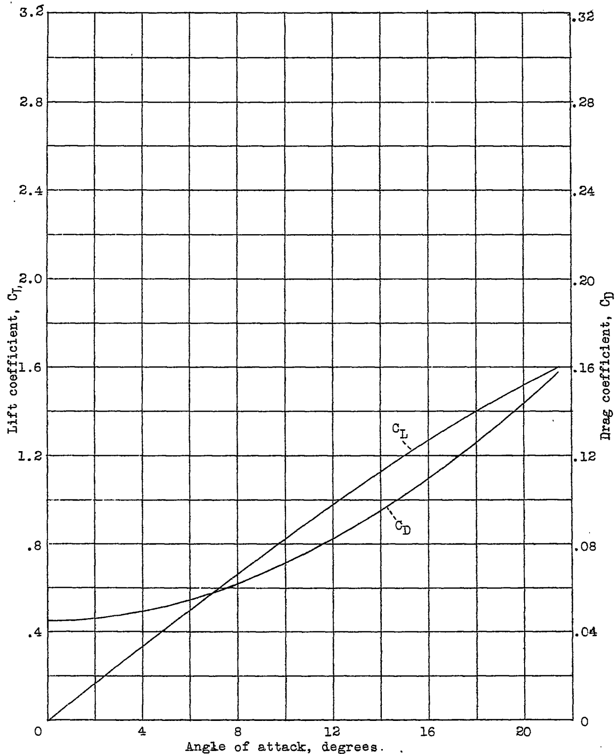
Figure 19.- Lift and drag coefficients for assumed wing.
