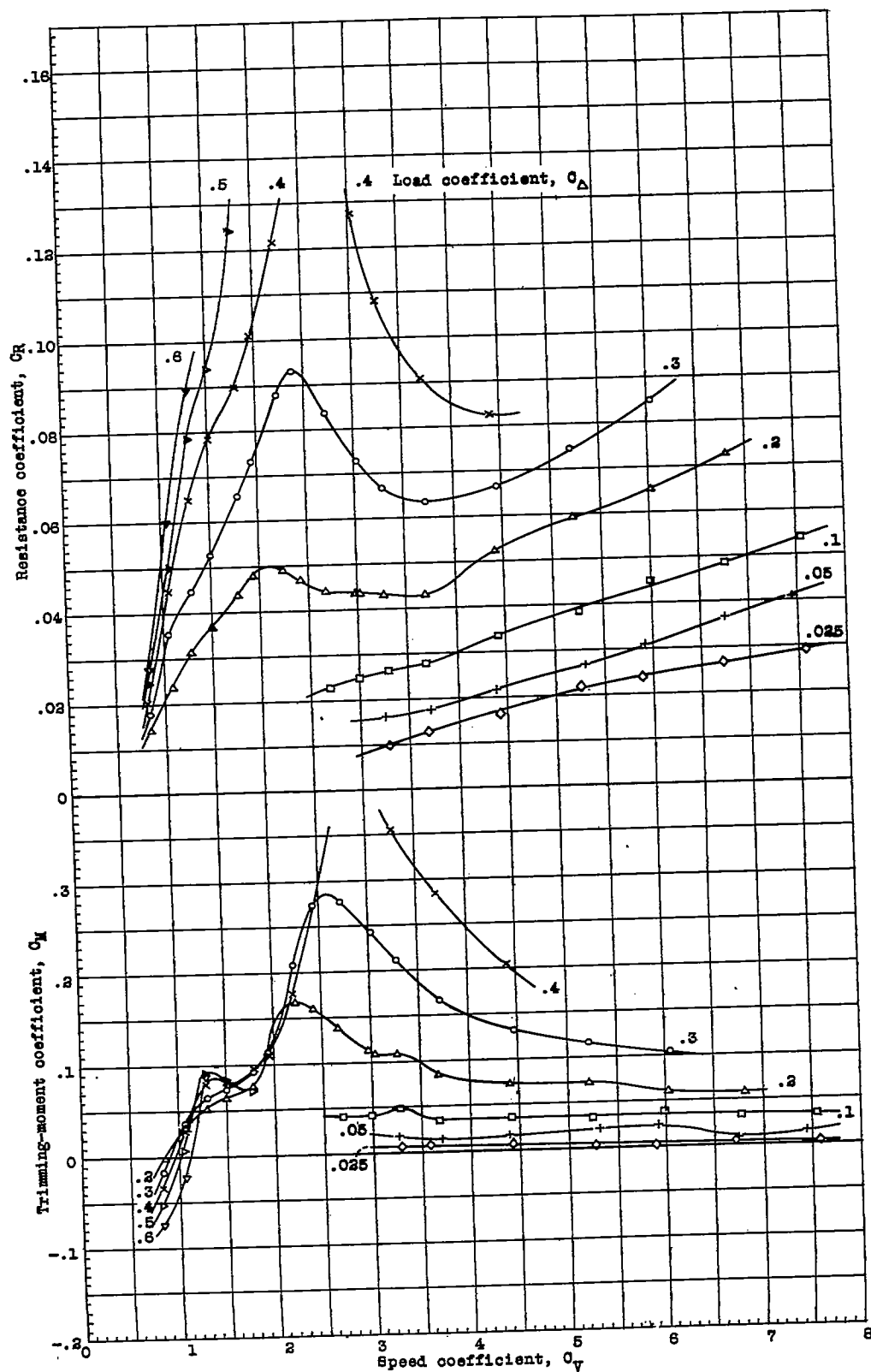
Figure 6. Resist- ance and trimming- moment coefficients, \tau = 5^\circ . N.A.C.A. model 47
