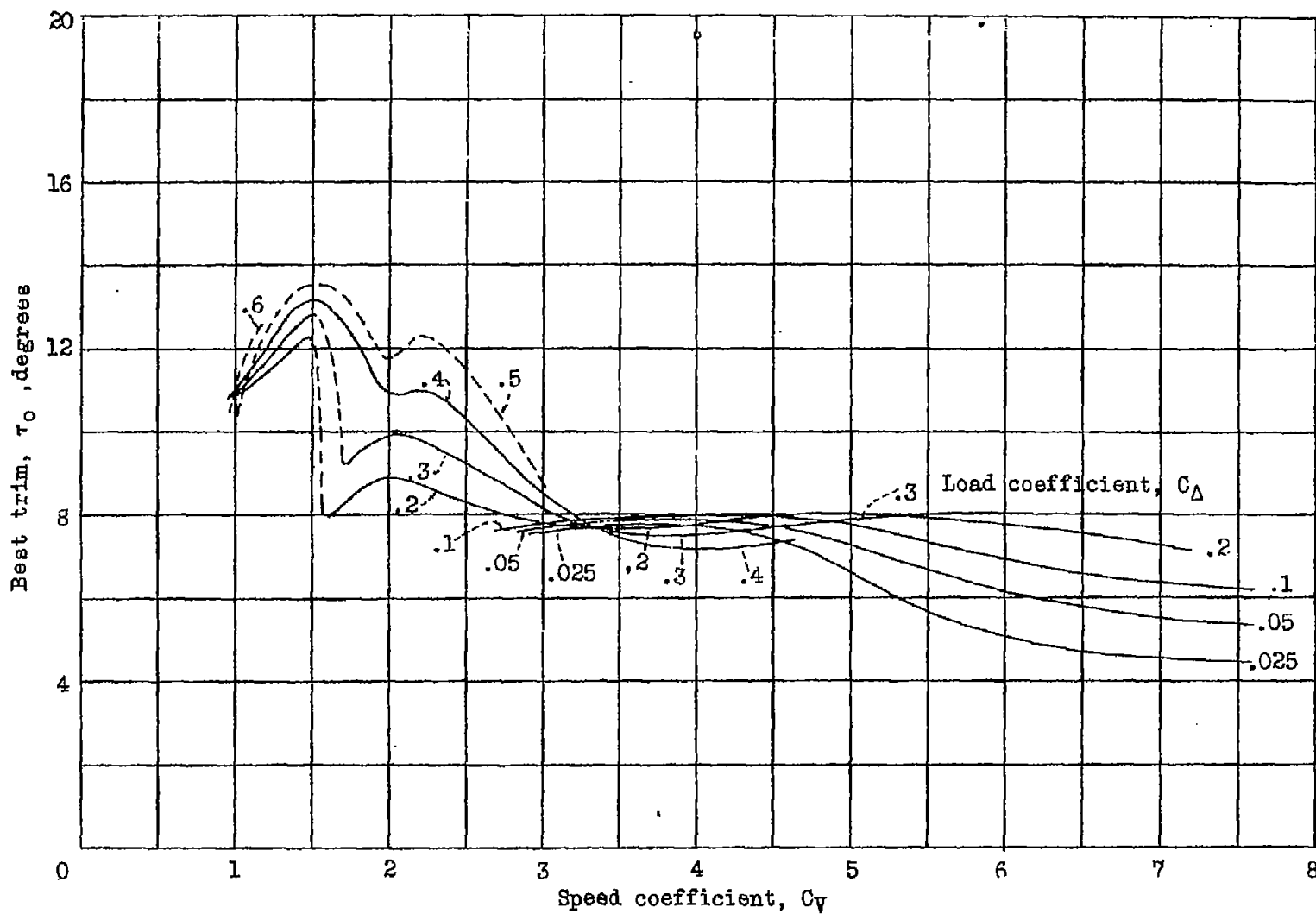
Figure 12.- Best trim (trim for minimum resistance). N.A.C.A. model 47
