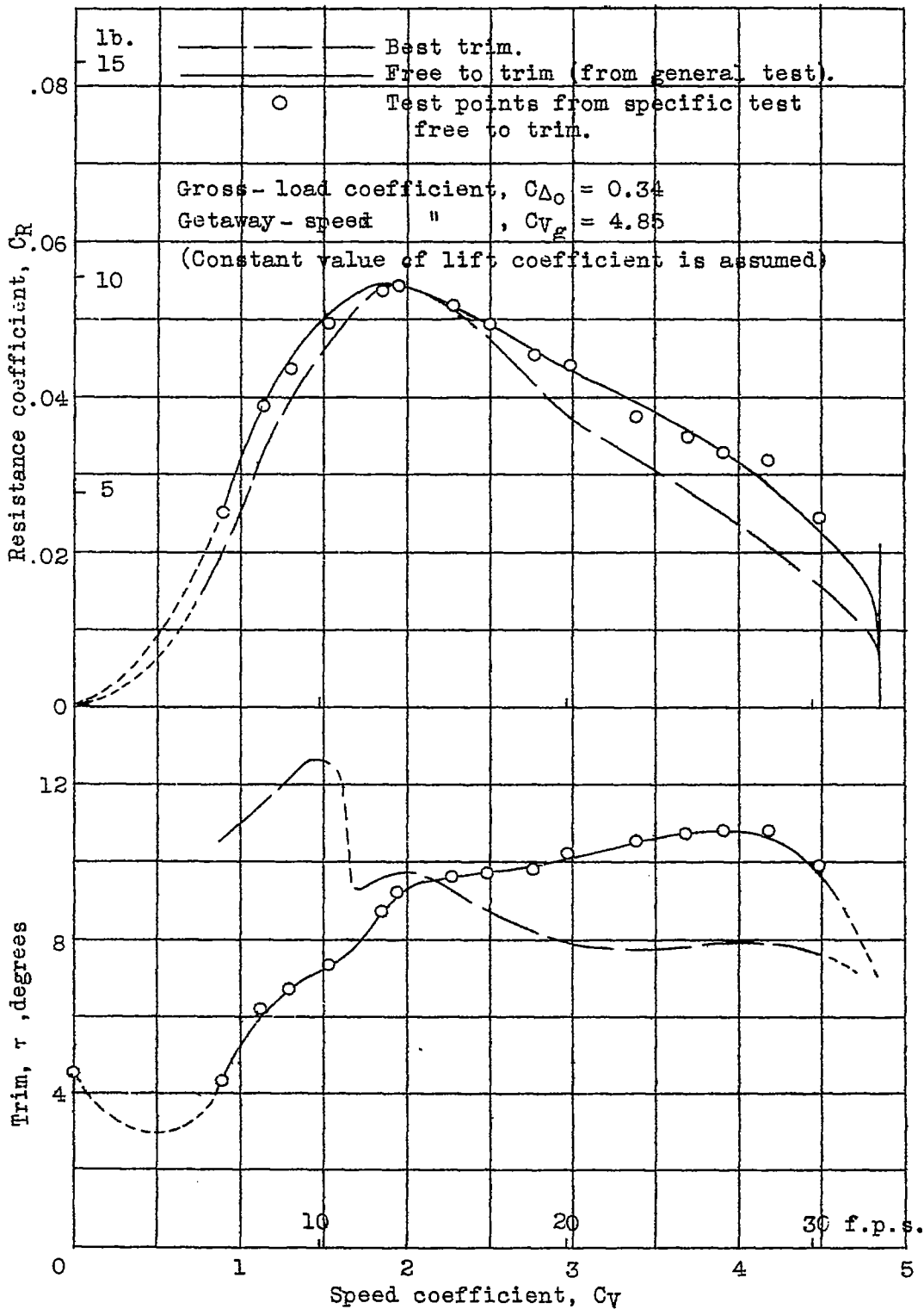
Figure 16.- Comparison of resistance and trim during take-off for model at best trim and free to trim. N.A.C.A. model 47.
