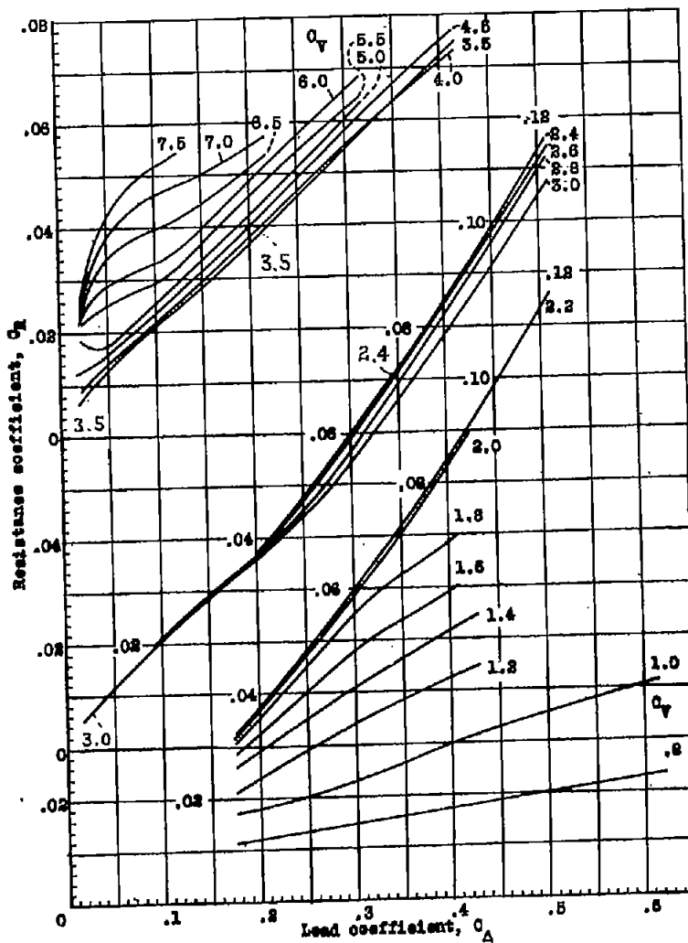
Figure 15.- Variation of resistance with load at best trim. N.A.C.A. model 47.
