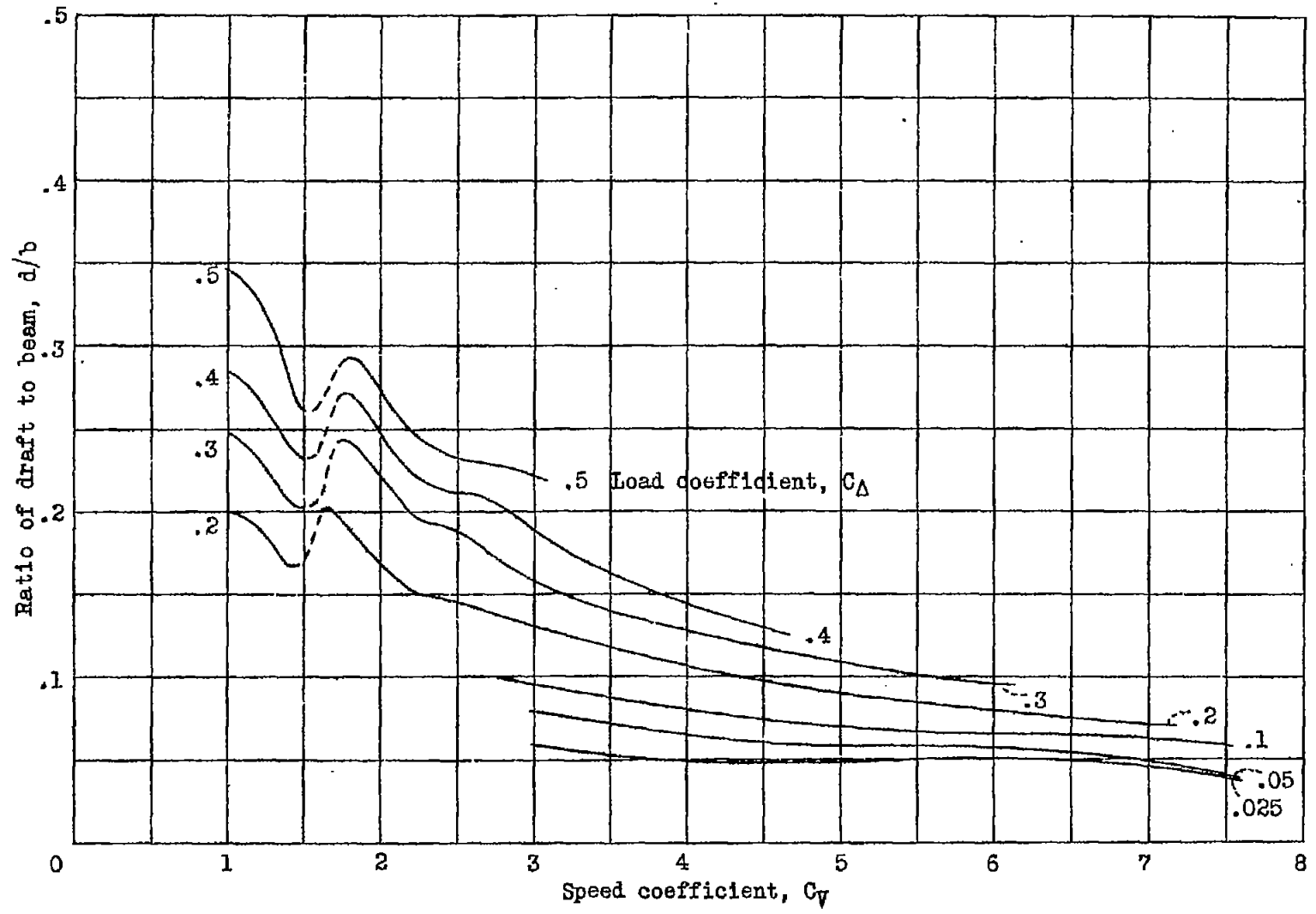
Figure 17.- Draft-beam ratio at best trim. N.A.C.A. model 47
