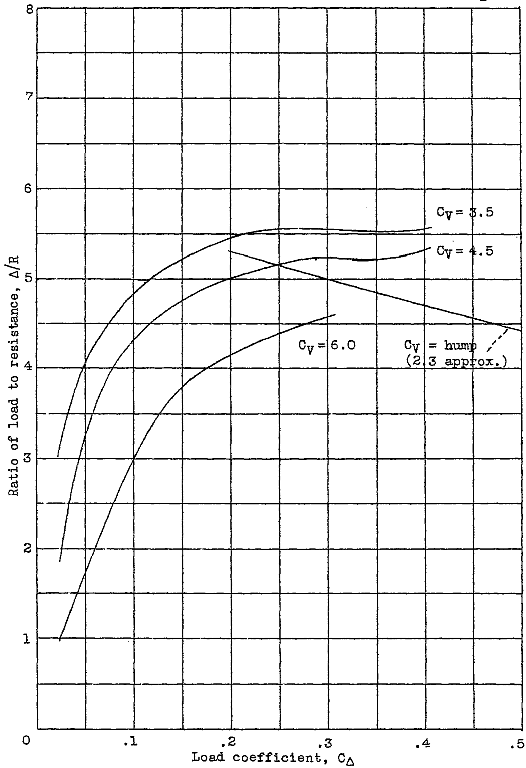
Figure 13.- Load-resistance ratio at best trim. N.A.C.A. model 47.
