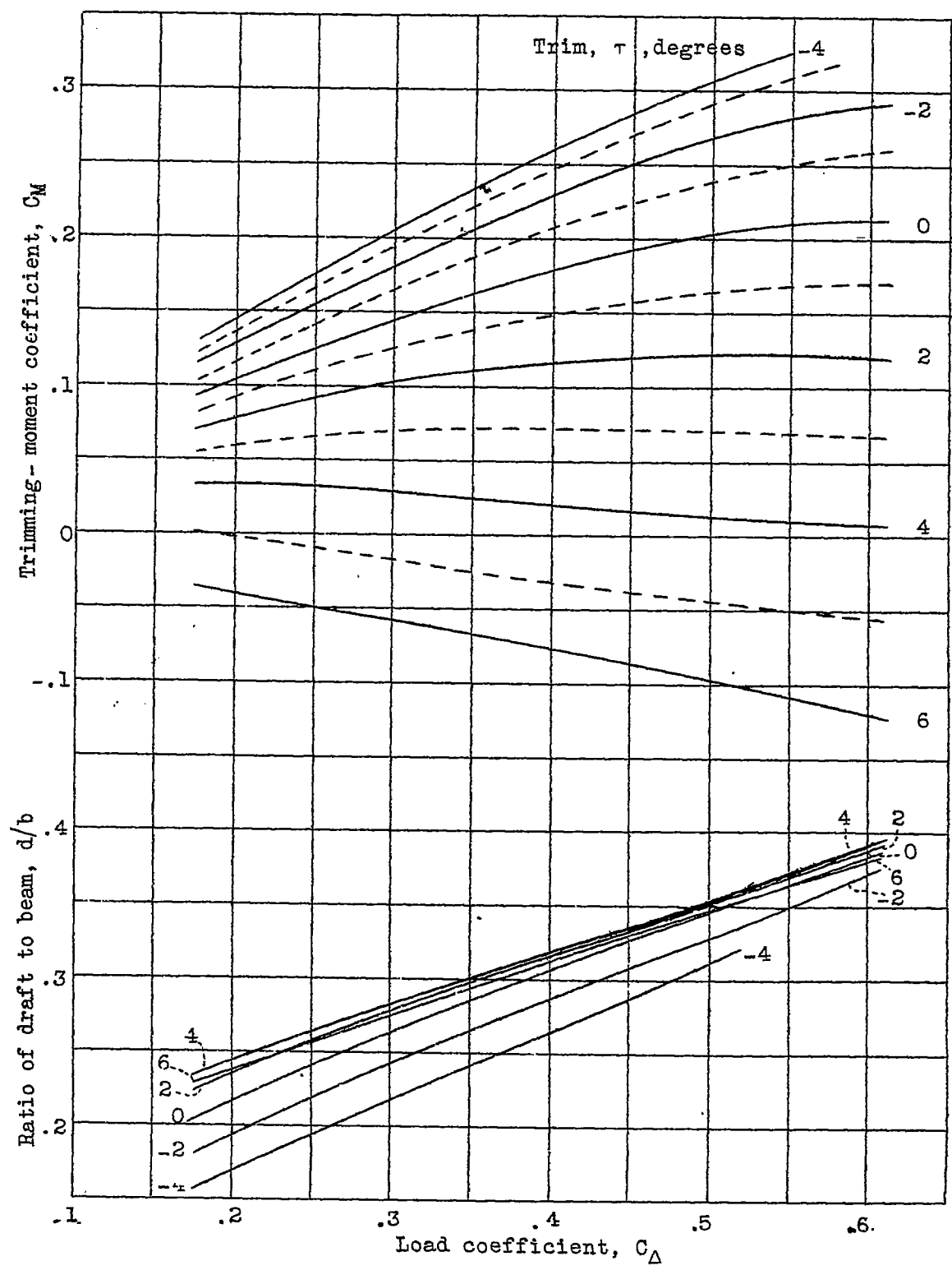
Figure 3.- Trimming-moment coefficient and draft-beam ratio, at rest. N.A.C.A. model 47
