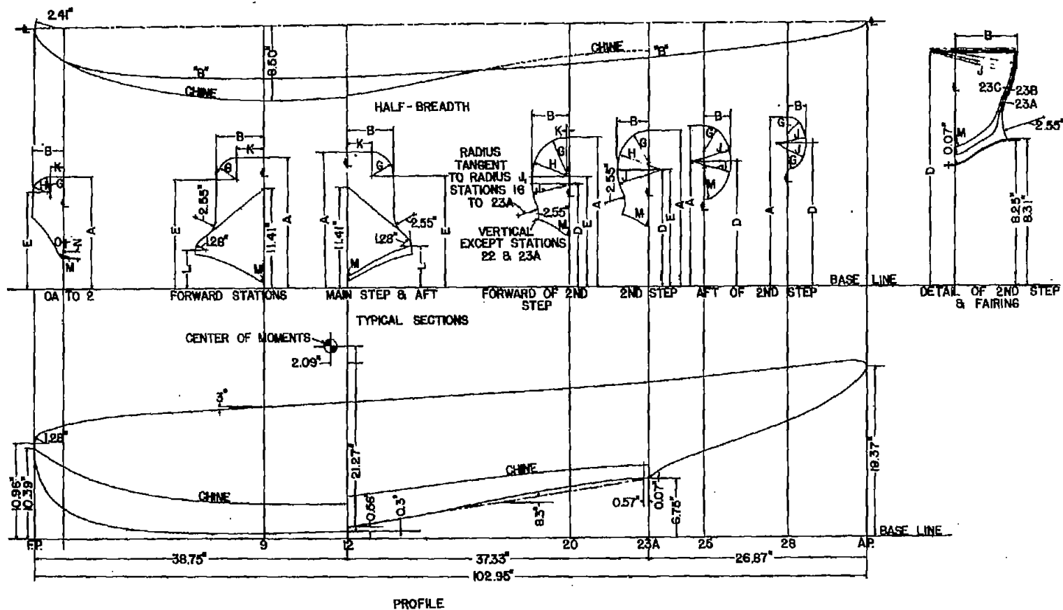
Figure 1. Lines of N.A.C.A. model 47 (Short Bros. Calcutta)
