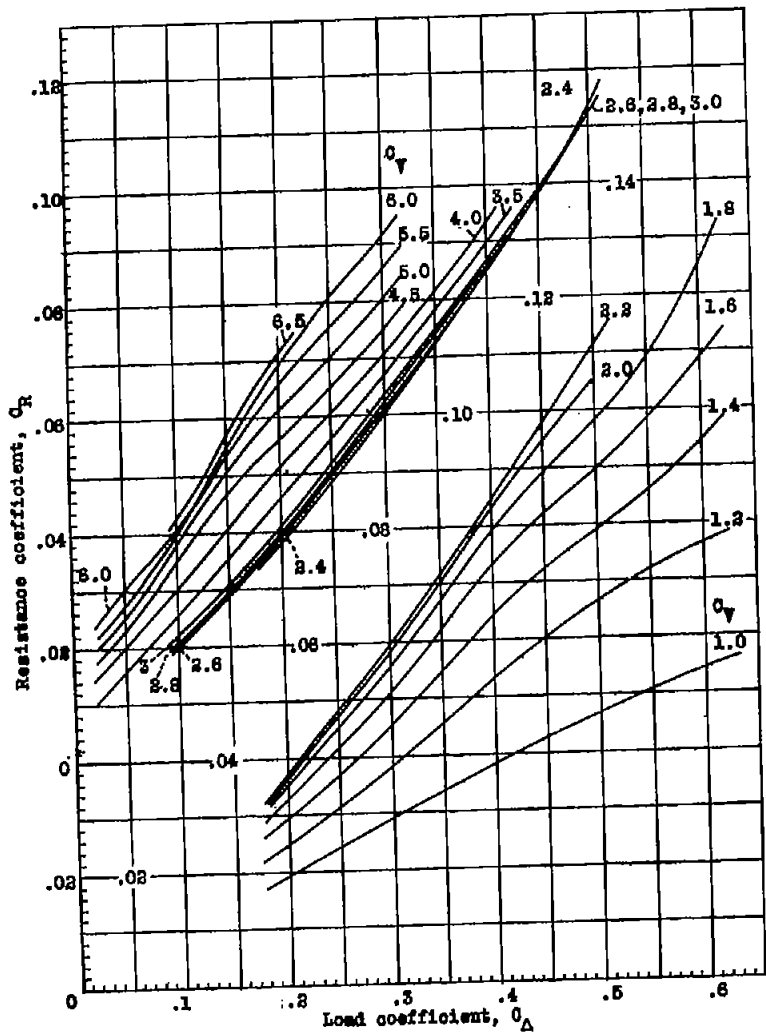
Figure 14.- Variation of resistance with load, free to trim. N.A.C.A. model 47.
