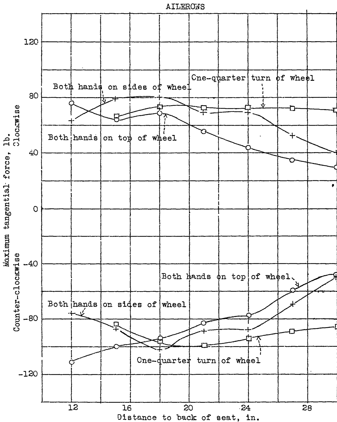
Figure 17.- Variation of tangential force with various two-hand grips, 12 inch wheel, center of wheel 14 inches above seat, pilot secure, pilot B.
