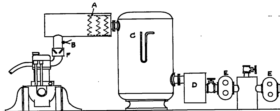
Figure 1.—Diagrammatic layout of test unit. A, electrical air heaters. B, thermocouple for intake temperature. C, surge tank. D, air cooler. E, Roots blower. F, carburetor.
