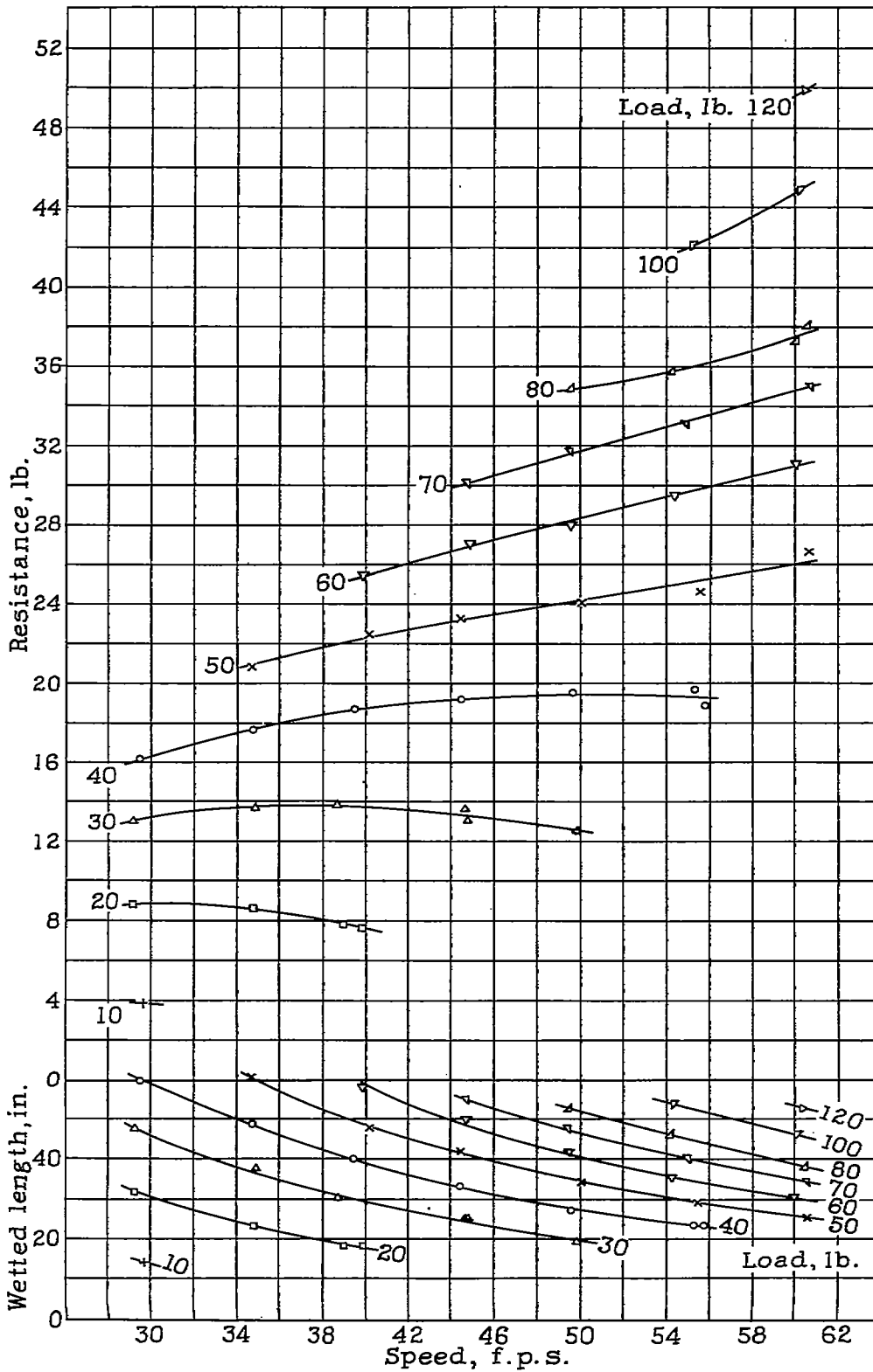
Fig.9.- Model 56-C. Variation of resistance with speed.
