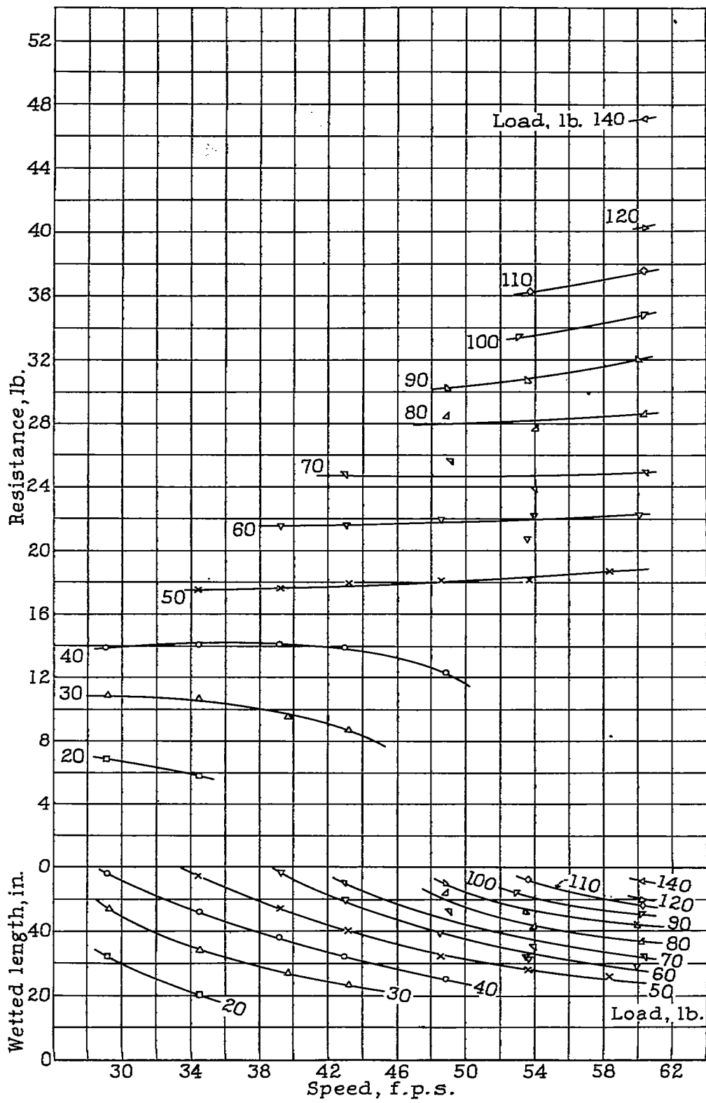
Fig.5.- Model 56-A. Varia- tion of re- sist- ance with speed.
