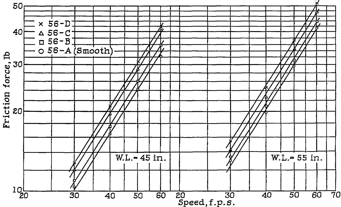
Figure 15.- Variation of friction force with speed
