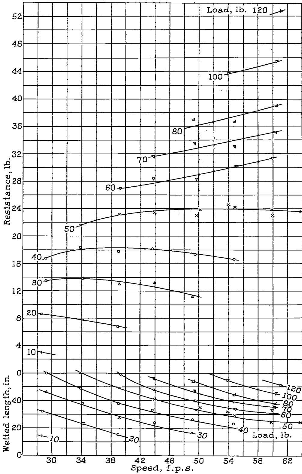
Fig. 11.- Model 56-D. Varia- tion of re- sist- ance with speed.
