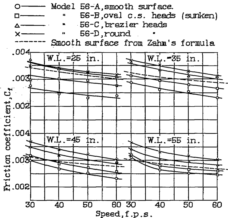
Figure 14.- Variation of friction coefficient with speed.
