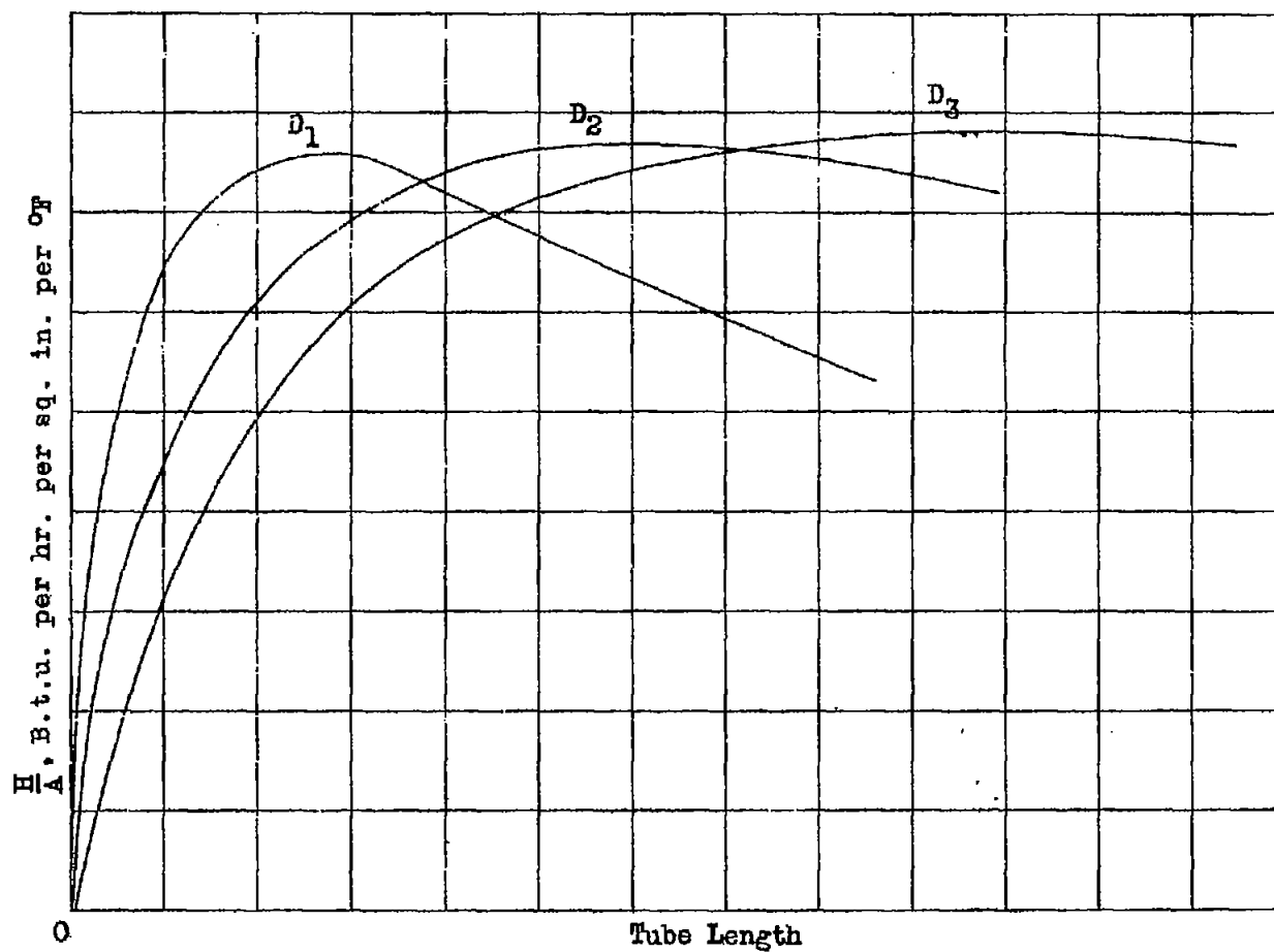
Figure 1.- Variation of heat dissipated per unit frontal area with radiator length for three tube diameters.
