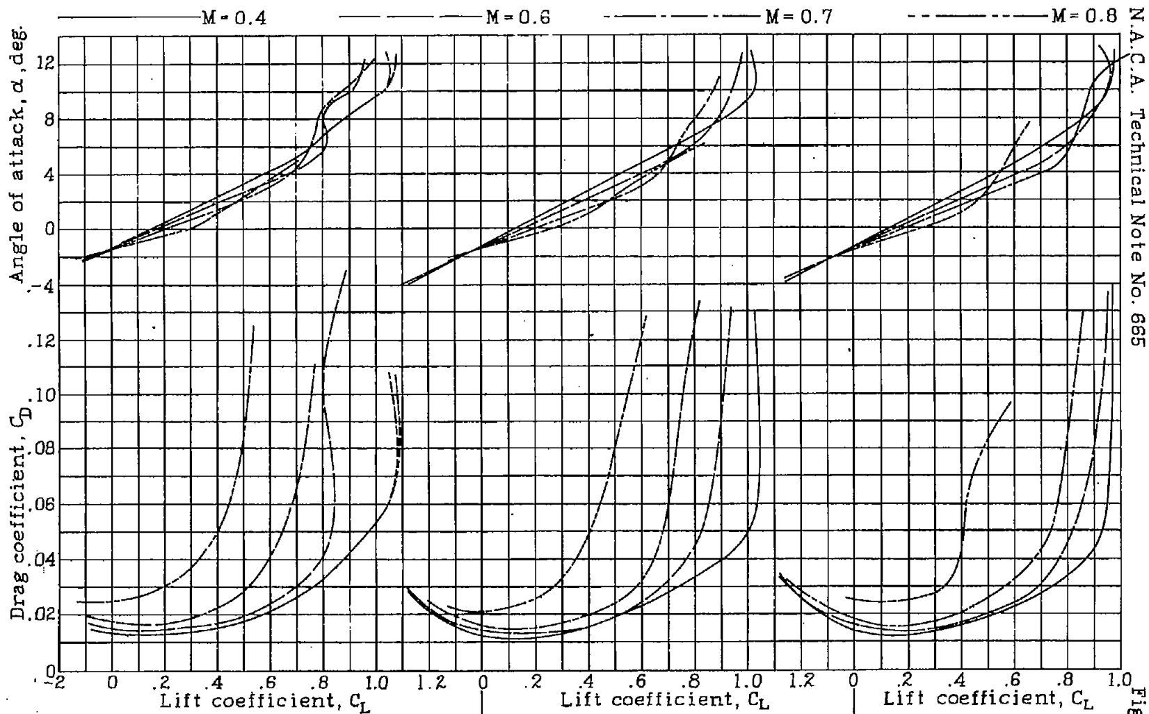
Figure 5.- Aerodynamic characteristics of the N-85 airfoil.
