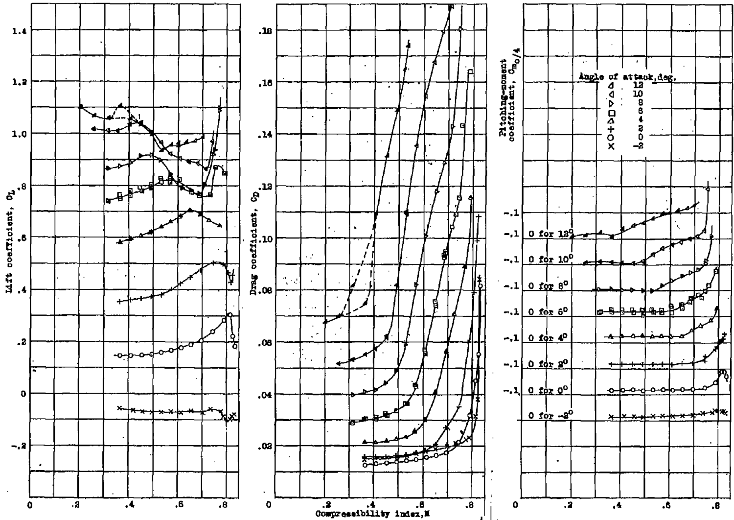
Figure 2.- Effect of compressibility on the aerodynamic characteristics of the N-85 airfoil.
