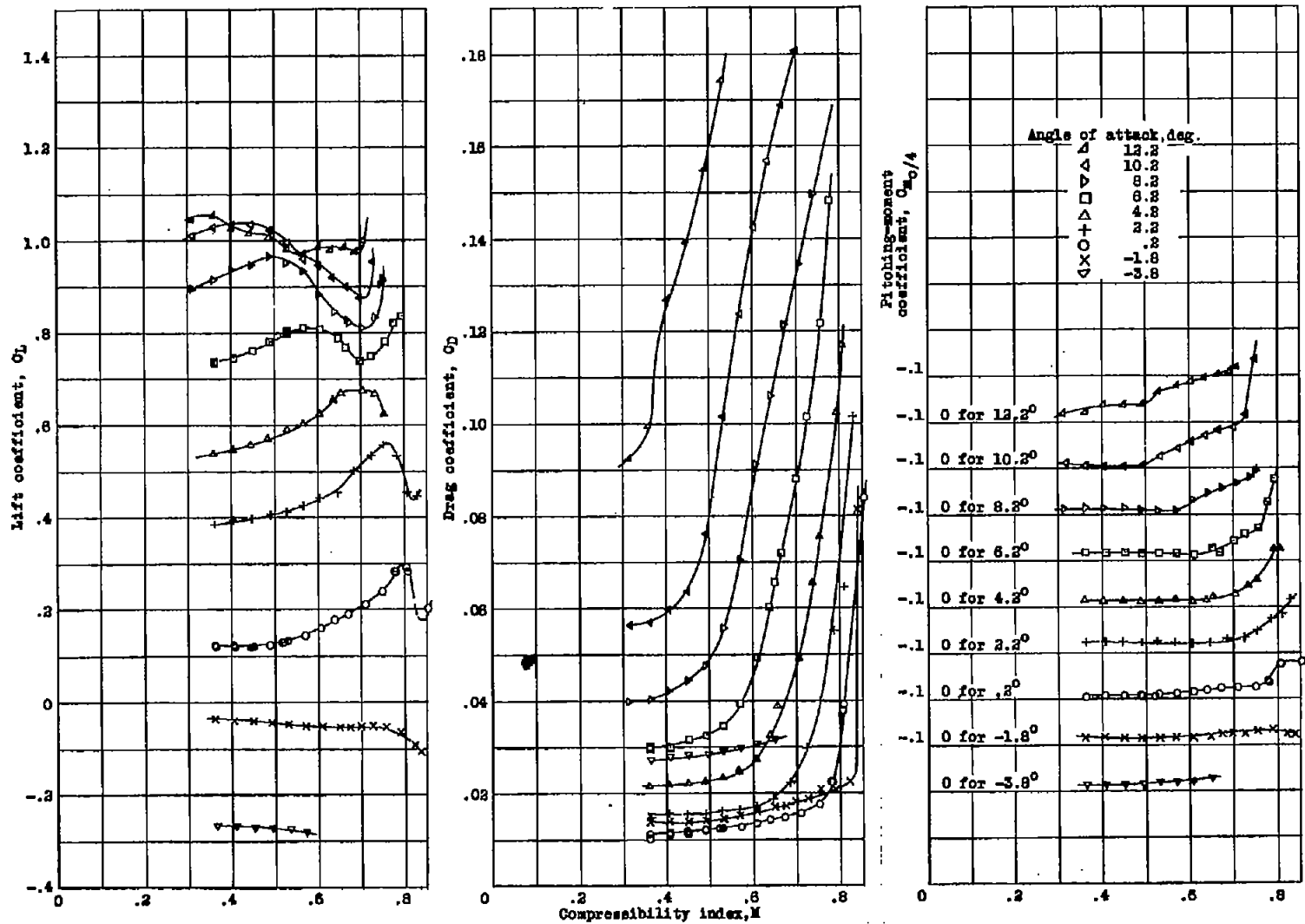
Figure 3.- Effect of compressibility on the aerodynamic characteristics of the N-66 airfoil.
