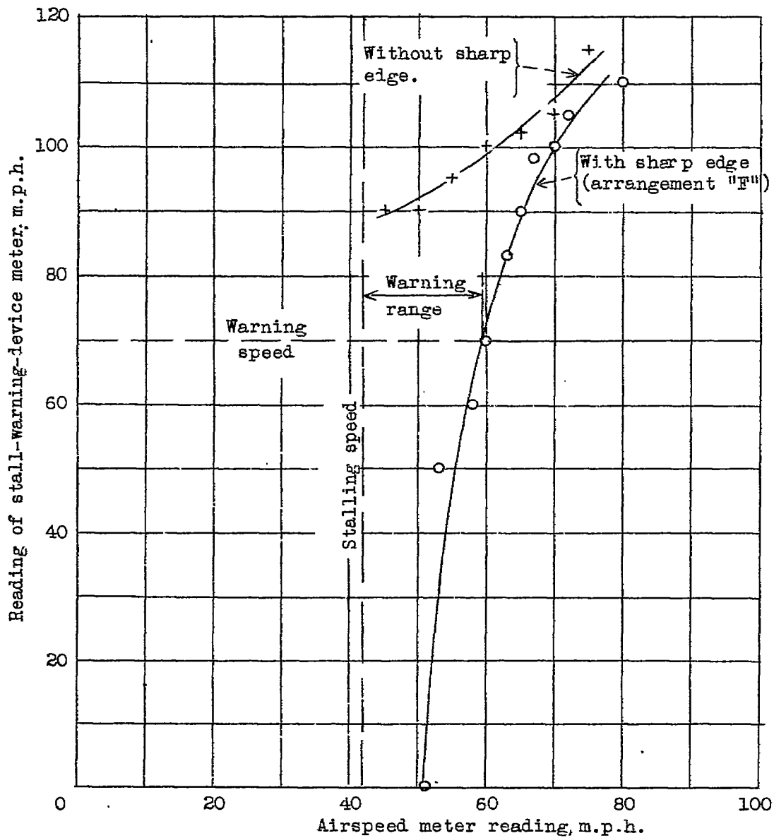
Figure 5.- Characteristics of stall-warning device for typical case.
