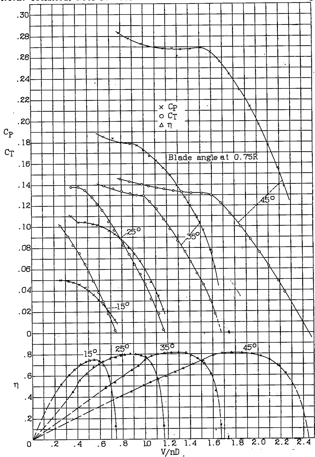
Figure 4.- Three-blade E-propeller.
