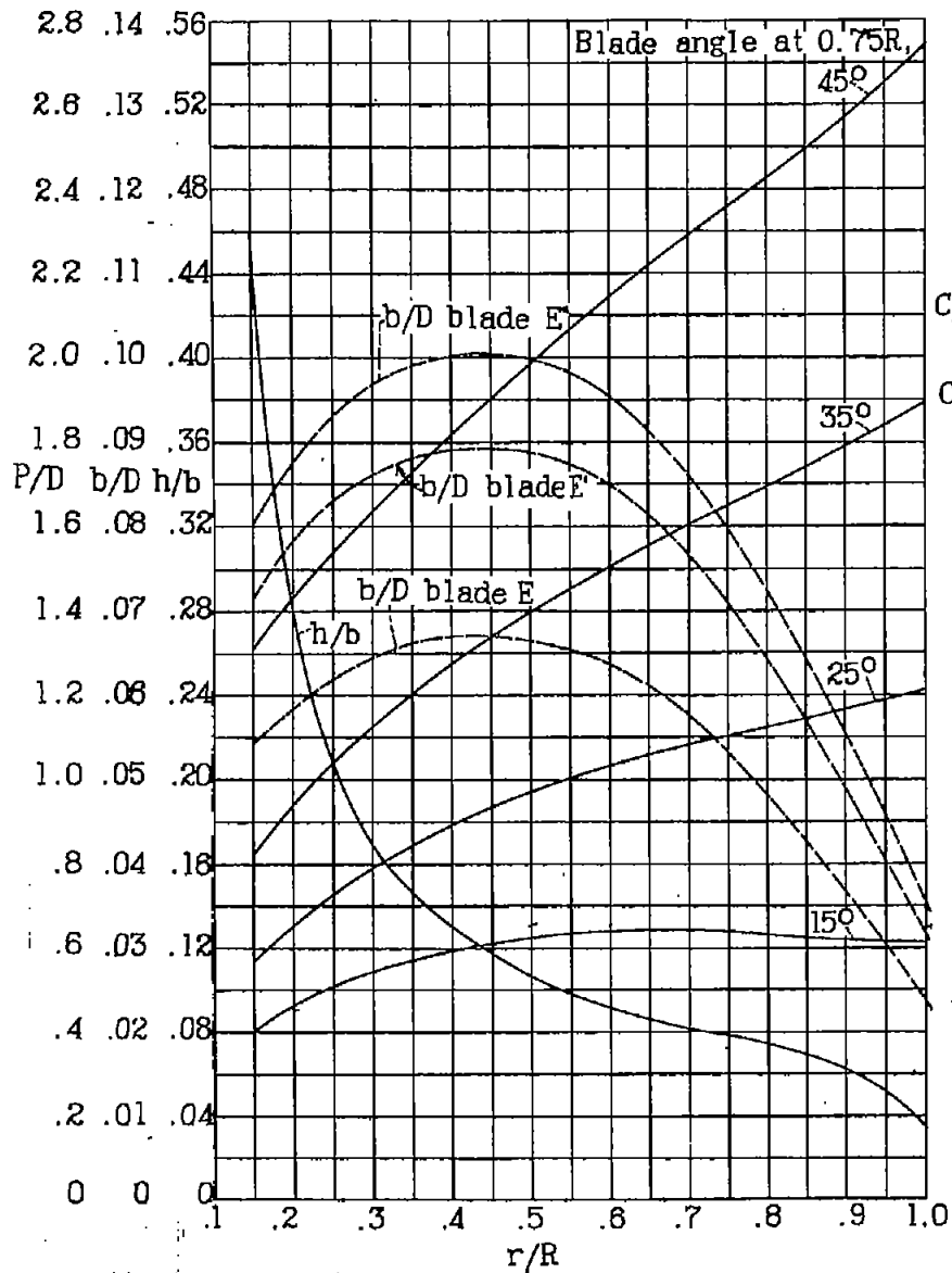
Figure 3.- Blade-form curves.
