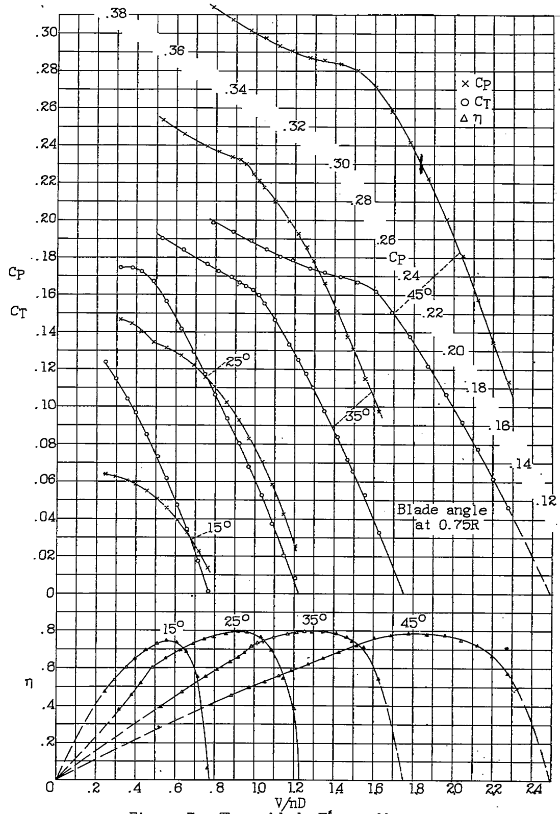
Figure 7.- Three-blade E^4 propeller.
