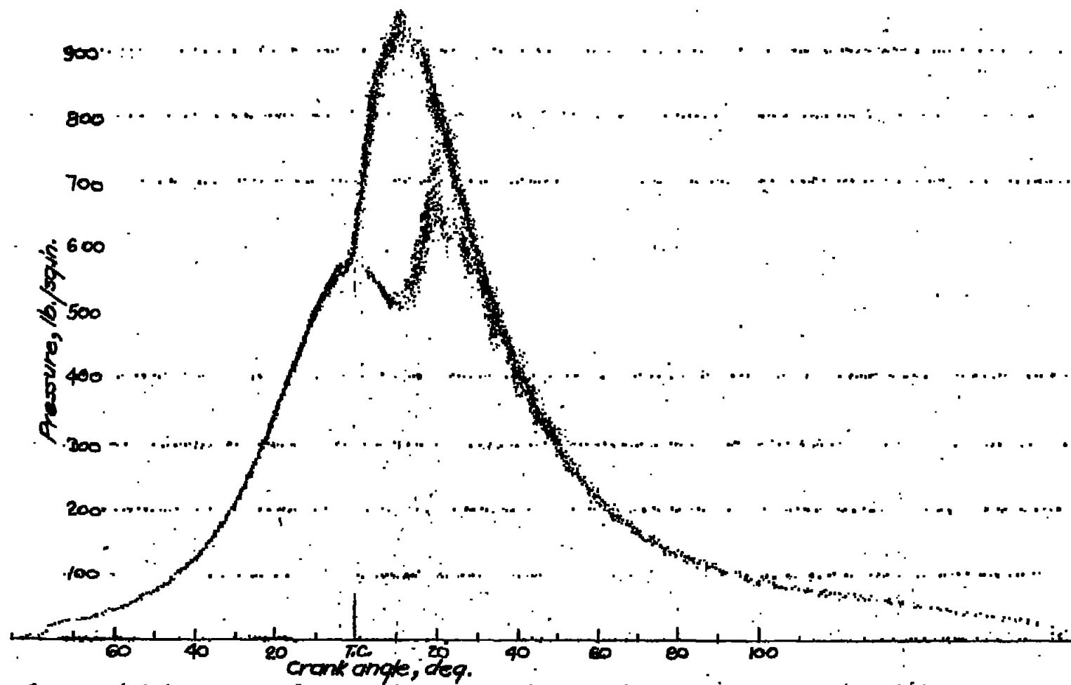
Figure 7- Indicator card, No. 3 furnace oil + 1 percent ethyl nitrate; quantity, 0.00037 lb./cycle; lap., 12.0° and 2.5°; ignition lag, 10°; maximum rate of pressure rise, 54 lb./sq.in./deg.
