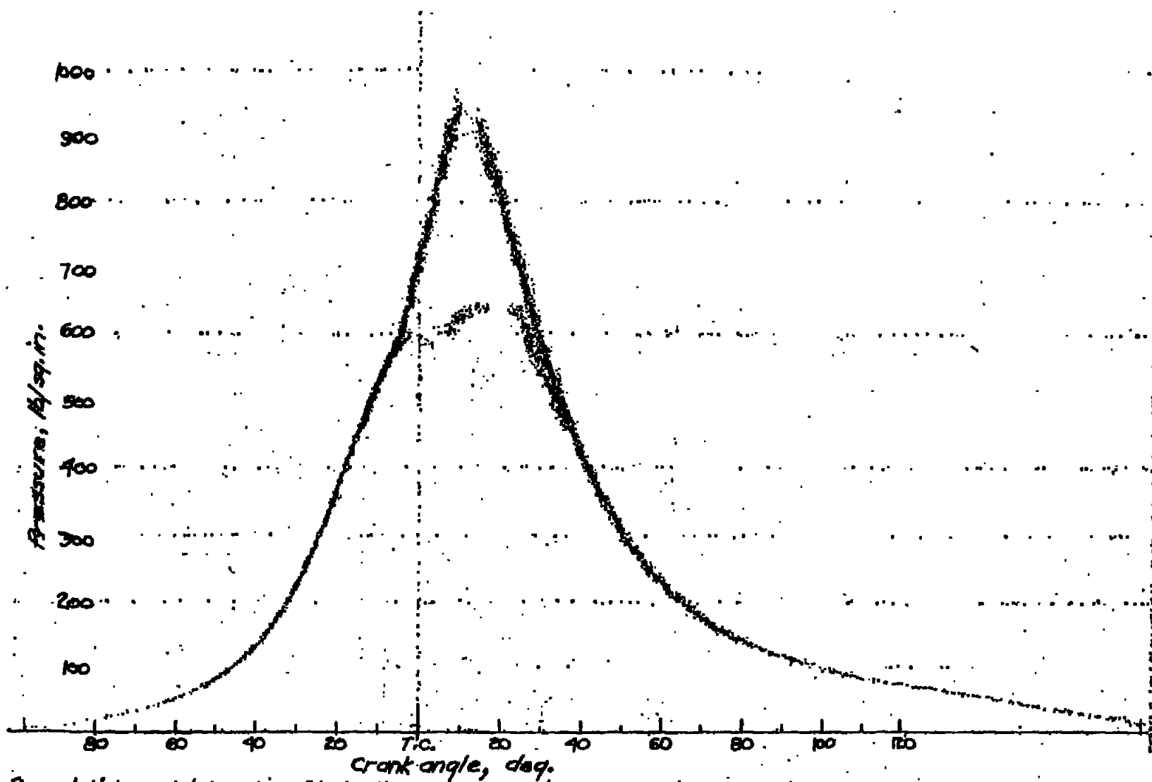
Figure indicator card, laboratory fuel oil + 4 percent tetranitromethane; quantity, 0.00039 lb/cycle; i.a.c., 12.0 and 4.5; ignition lag, 6.5; maximum rate of pressure rise, 20 lb/sq.in./deg.
