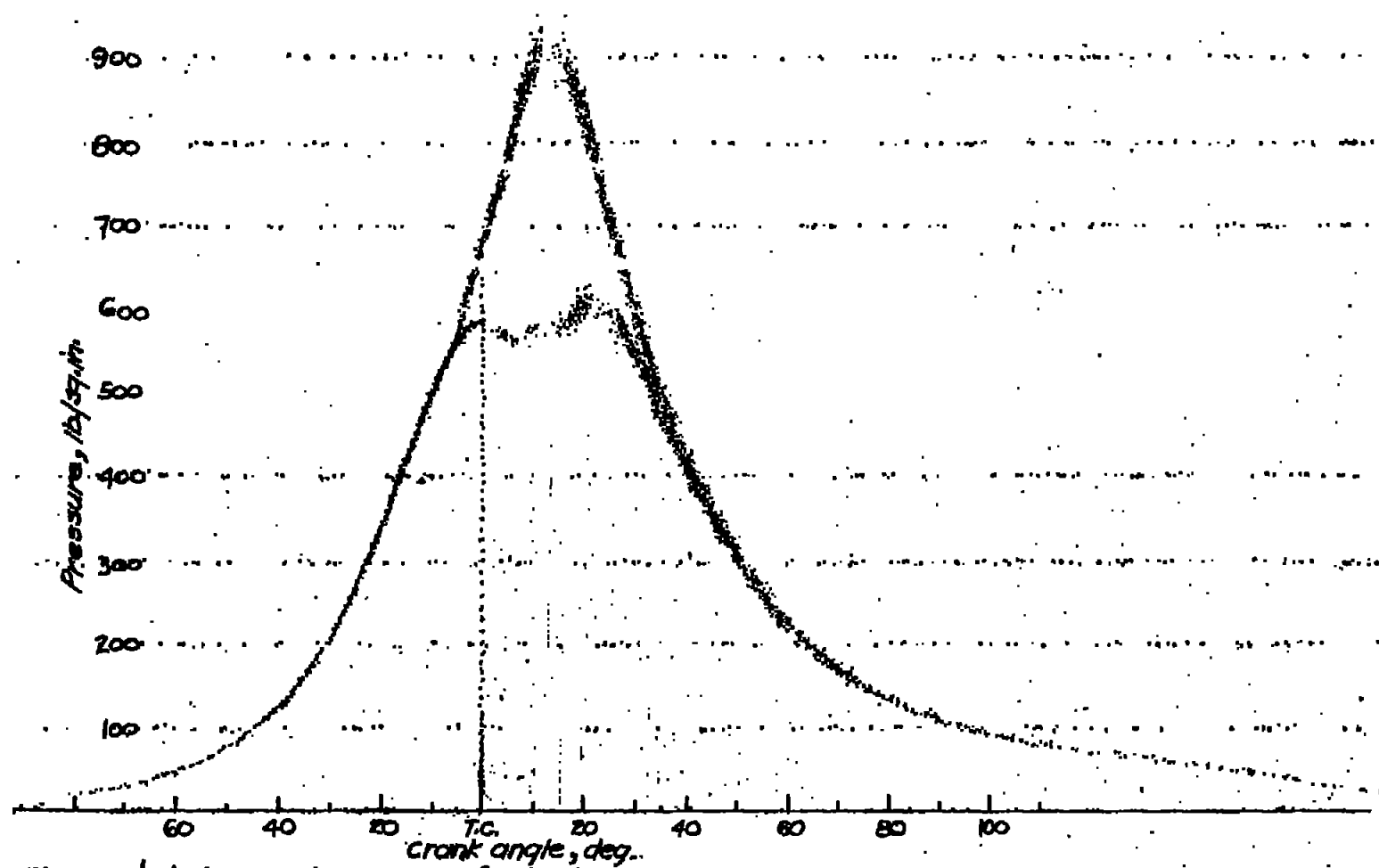
Figure 8. Indicator card, laboratory fuel oil + 2.5 percent iso-amyl nitrate; quantity, 0.000376 lb./cycle; \lambda_{0.9} , 12.0 and 2.5°; ignition lag, 6.5°; maximum rate of pressure rise, 23 lb./sq.in./deg.
