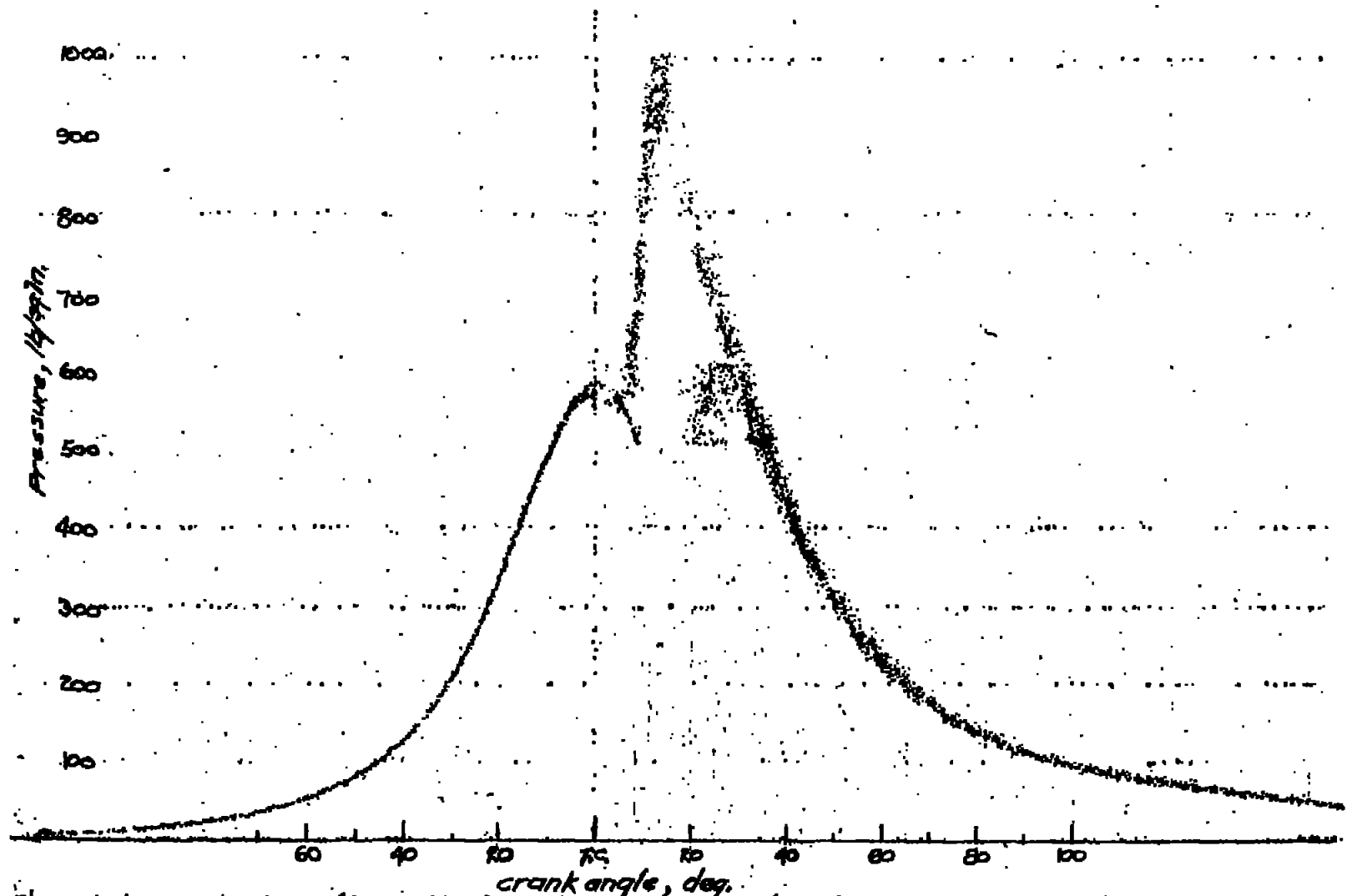
Figure 14—Indicaboard, mixture of laboratory fuel oil + 40 percent alcohol; quantity, 0.000365 lb./cycle, 1000, 12° and 4°; ignition lag, 16°; maximum rate of pressure rise, 97 lb./sq.in./deg.
