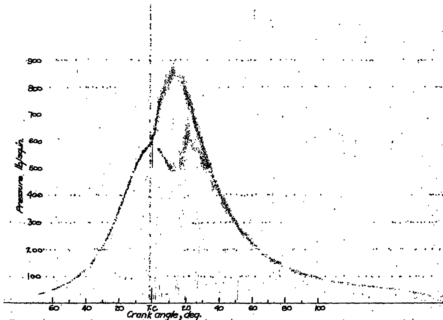
Figure 13. Indicator card, laboratory fuel oil + 25 percent 87 octane gasoline; quantity, 0.000573 lb/cycle; i.a.c., 12.0 and 2.5; ignition lag, 10°; maximum rate of pressure rise, 57 lb/sq.in./deg.
