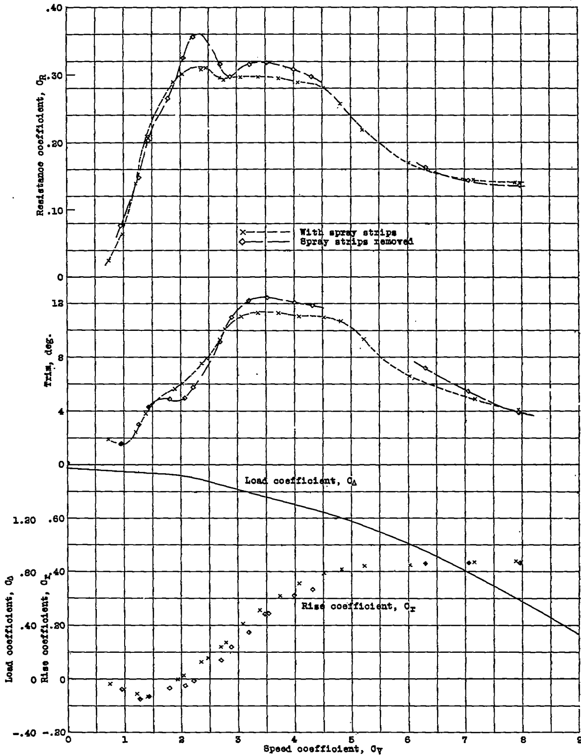
Figure 6.- Effect of spray strips on free-to-trim characteristics. Model 57-A.
