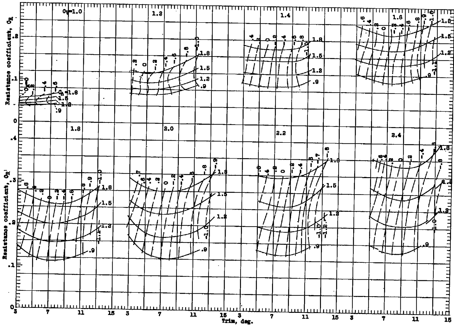
Figure 15a.- Model 57-B-5. Working charts for the determination of resistance and trimming moment.
