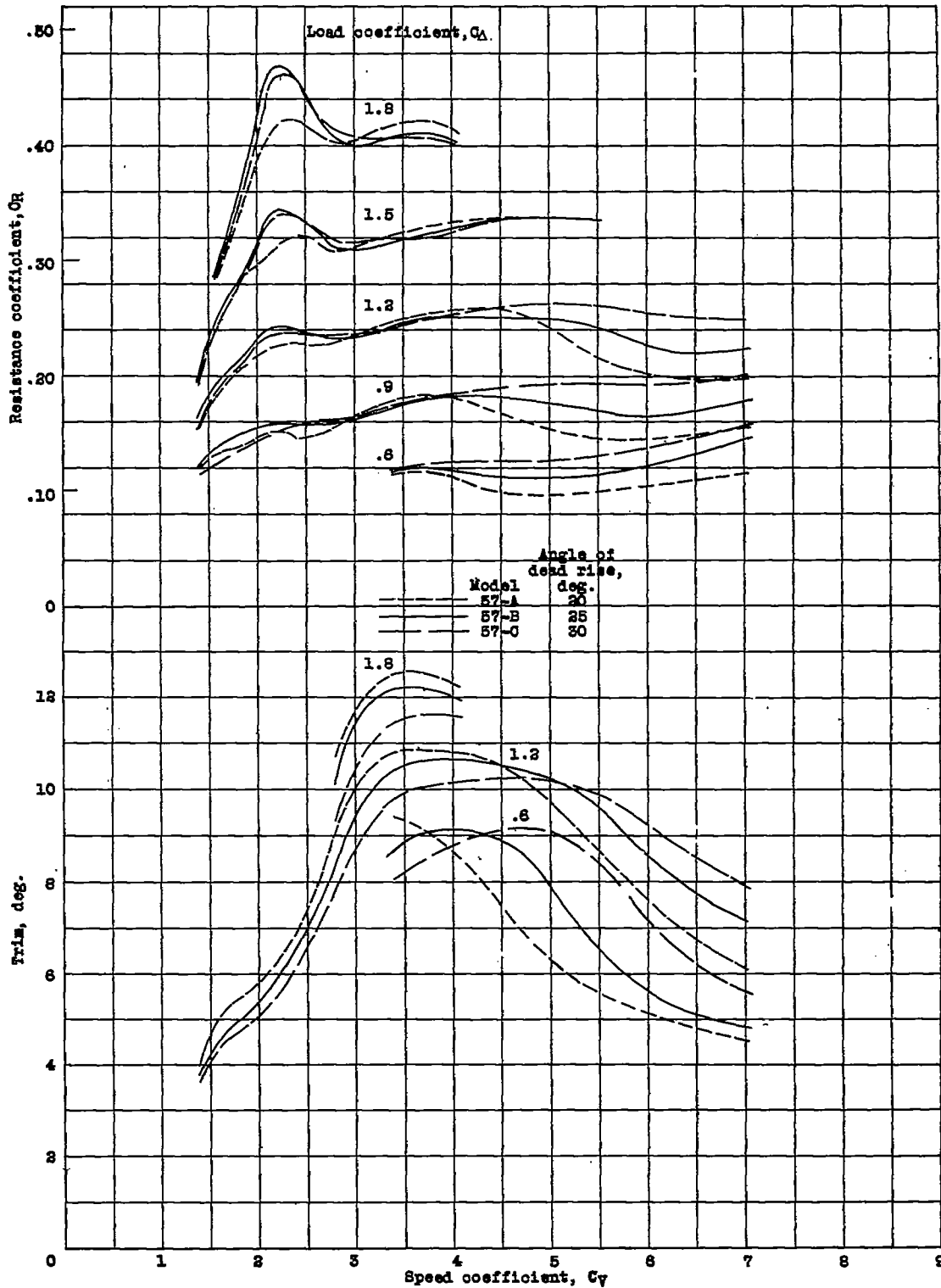
Figure 9.- Effect of angle of dead rise on characteristics at zero trimming moment.
