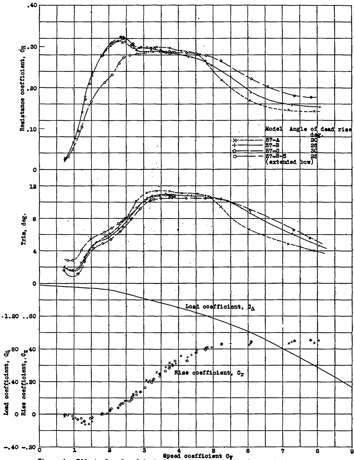
Figure 4.- Effect of angle of dead rise and extended bow on free-to-trim characteristics.
