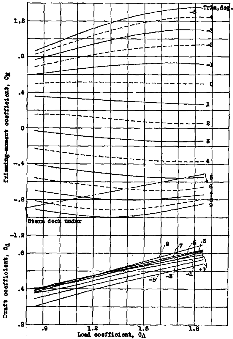
Figure 16.- Model 57-R. Static properties.
