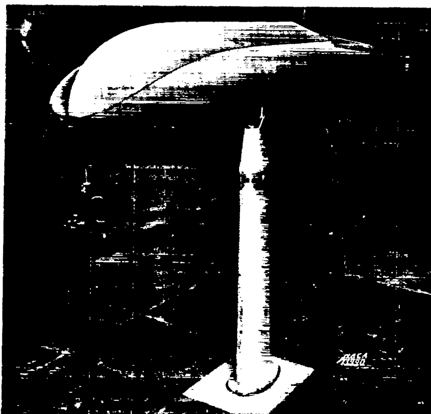
Figure 18.- Model 57-B mounted in the wind tunnel.
