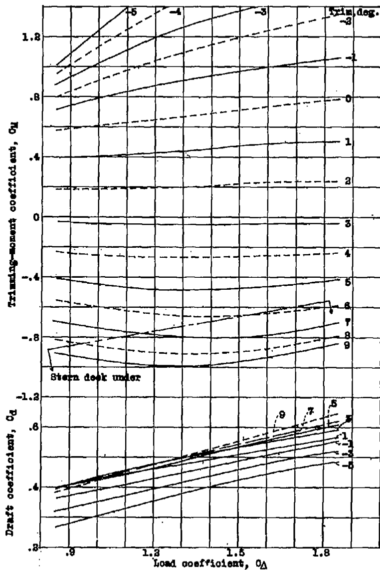
Figure 17.- Model 57-B-S. Static properties.
