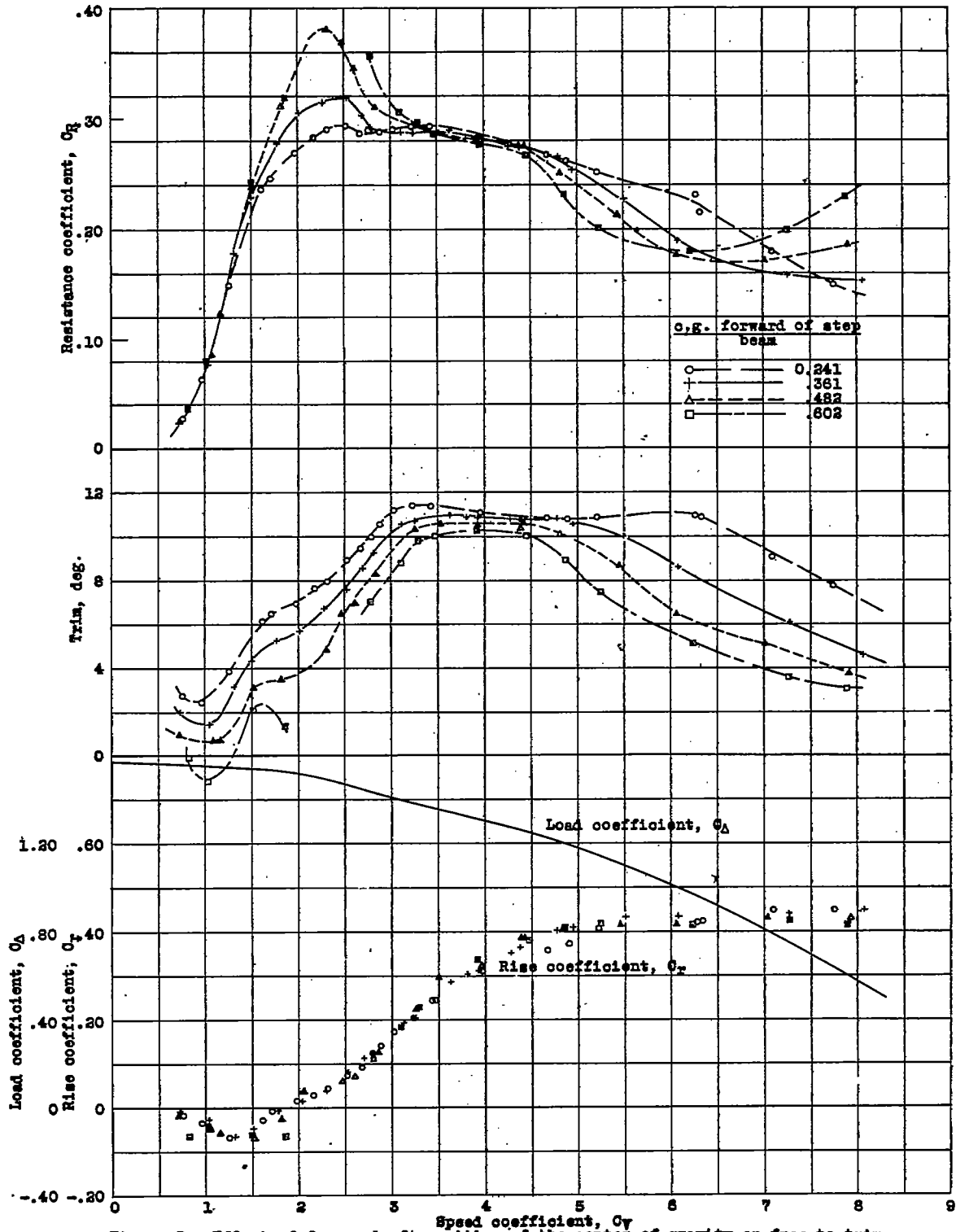
Figure 3.- Effect of fore-and-aft position of the center of gravity on free-to-trim characteristics. Model 57-B.
