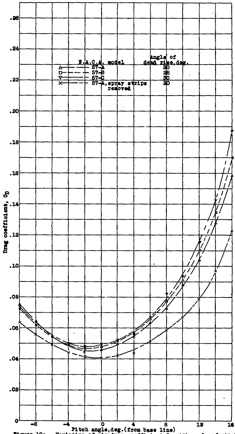
Figure 19a.- Variation of air drag coefficient C_D with angle of pitch.
