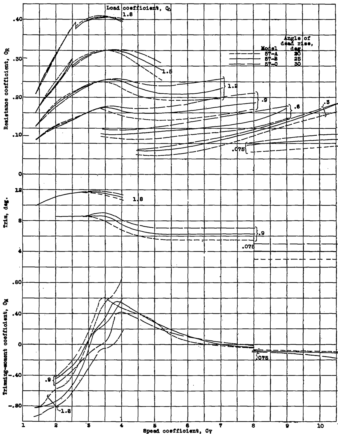
Figure 10.- Effect of angle of dead rise on characteristics at best trim.
