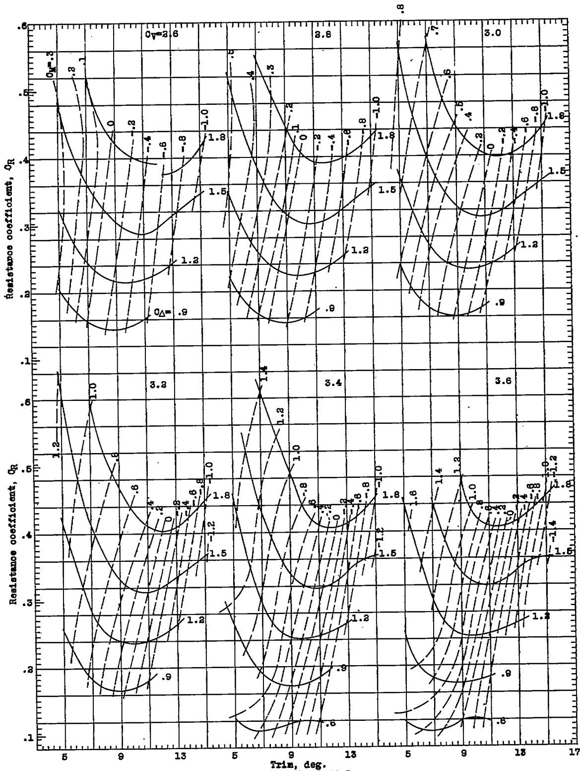
Figure 14b- Model 57-B.
