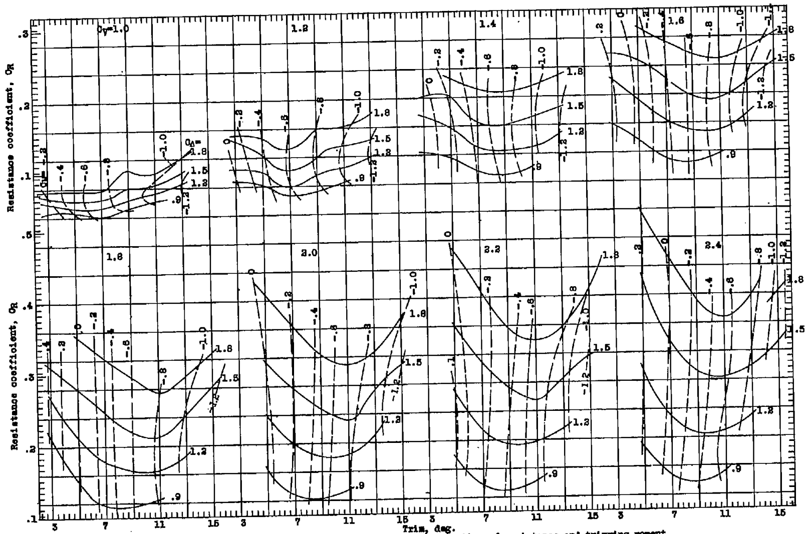
Figure 14a.-Model 57-B. Working charts for the determination of resistance and trimming moment.
