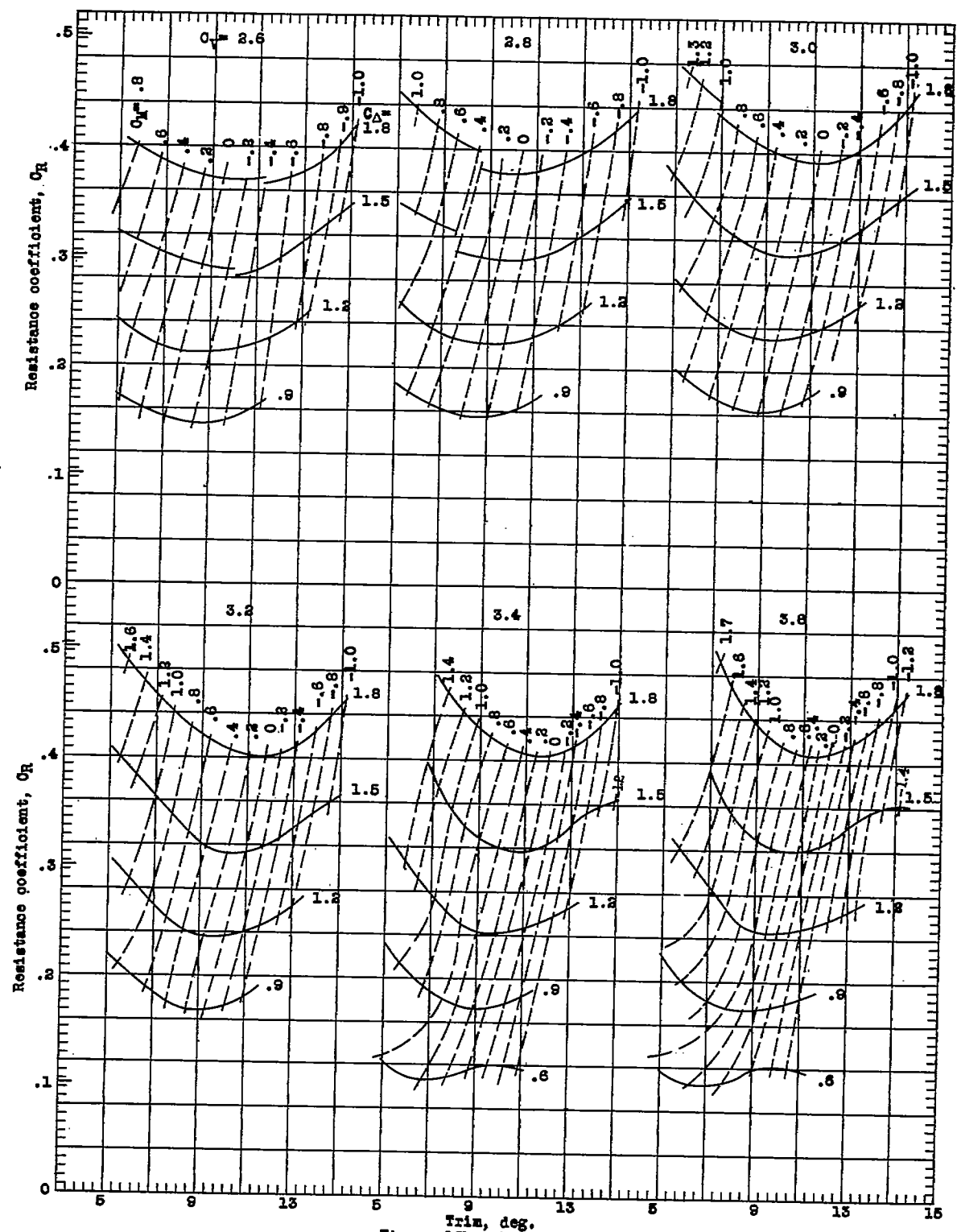
Figure 15b.- Model 57-B-5.
