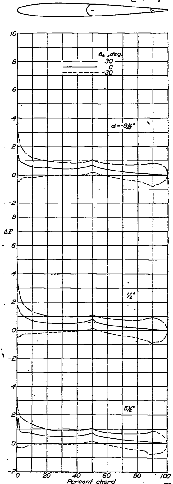
Figure 6.- Increments of resultant pressures for various angles of attack and various deflections of a 0.20c f tab on a 0.50c plain flap deflected 5°.
