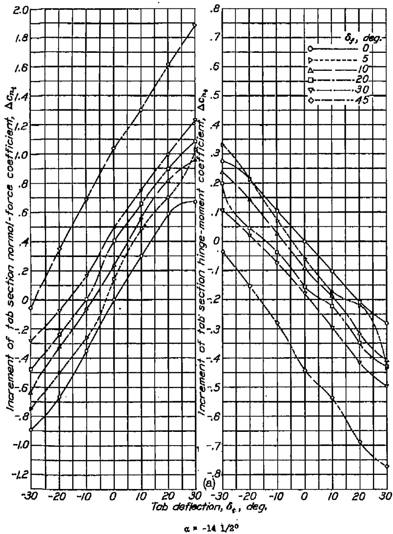
Figure 20, a to f.- Increments of tab section normal-force and hinge-moment coefficients for various deflections of a 0.50c t plain flap and a 0.50c t tab.
