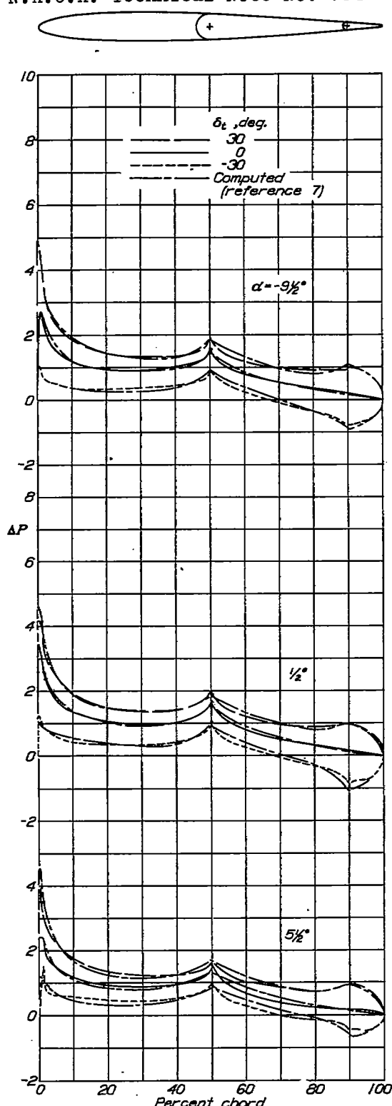
Figure 7.- Increments of resultant pressures for various angles of attack and various deflections of a 0.20c flap on a 0.50c plain flap deflected 10°.
