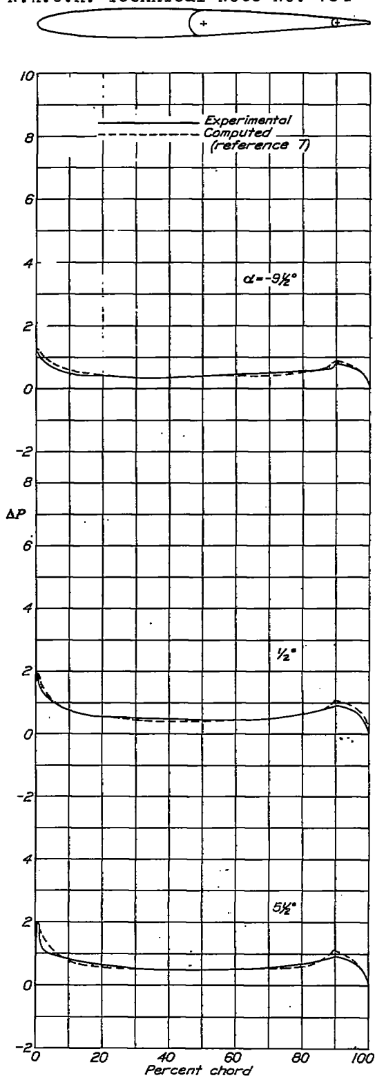
Figure 5.- Increments of resultant pressures for various angles of attack and various deflections of a 0.20c f tab on a 0.50c plain flap deflected 0°, 8 t , 30°.
