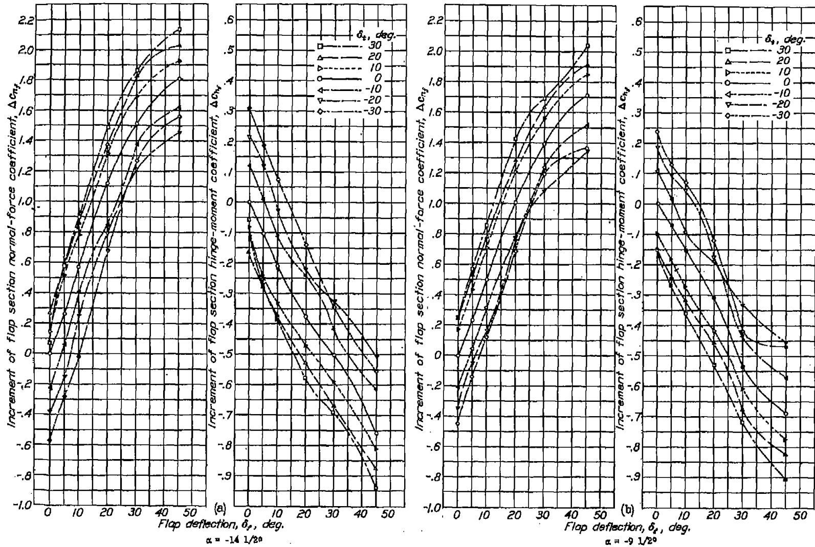
Figure 15, a to f.- Increments of flap section normal-force and hinge-moment coefficients for various deflections of a 0.50c plain flap and a 0.10c tab.
