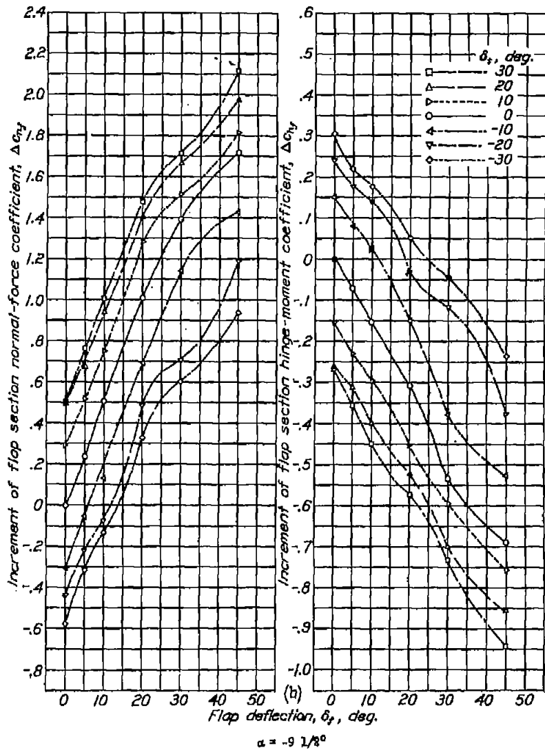
Figure 16, a to f.- Increments of flap section normal-force and hinge-moment coefficients for various deflections of a 0.50c plain flap and a 0.20c t tab.
