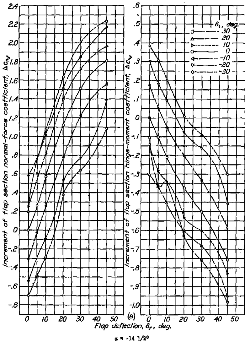
Figure 16, a to f.- Increments of flap section normal-force and hinge-moment coefficients for various deflections of a 0.50c plain flap and a 0.20c t tab.
