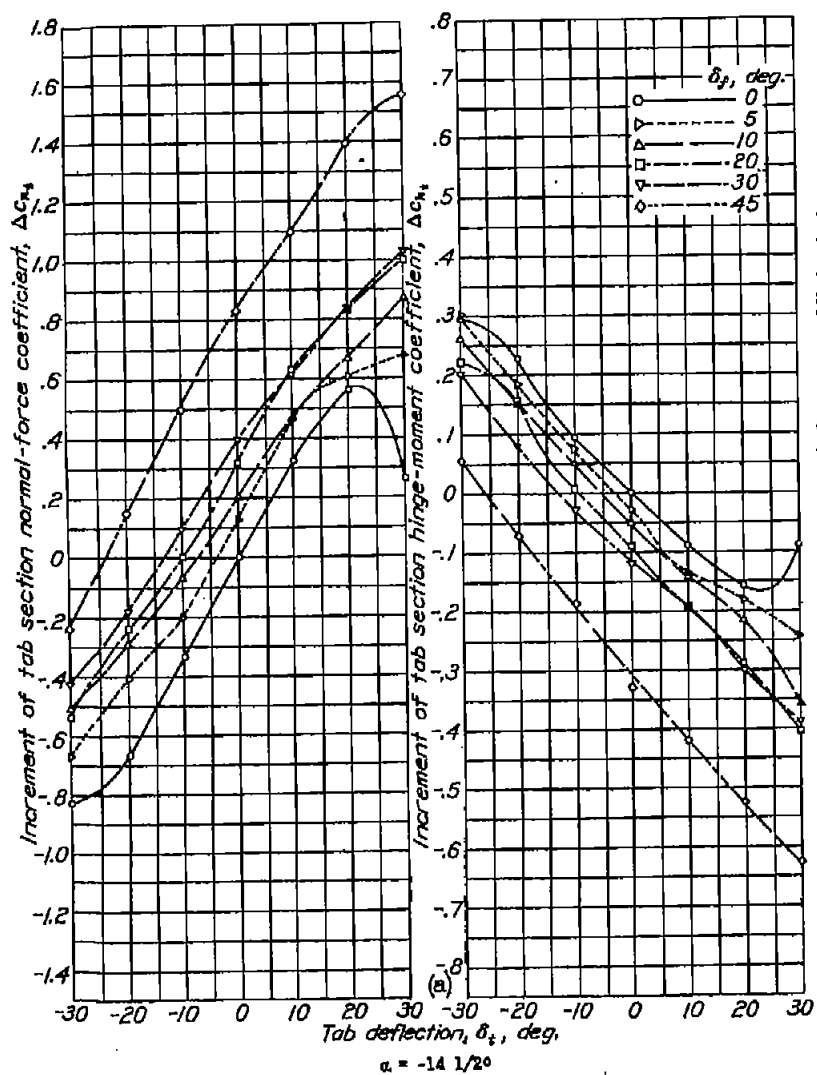
Figure 17, a to f.- Increments of tab section normal-force and hinge-moment coefficients for various deflections of a 0.50c plain flap and a 0.20c tab.
