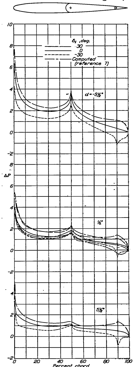
Figure 8.- Increments of resultant pressures for various angles of attack and various deflections of a 0.20c flap on a 0.50c plain flap deflected 20°.
