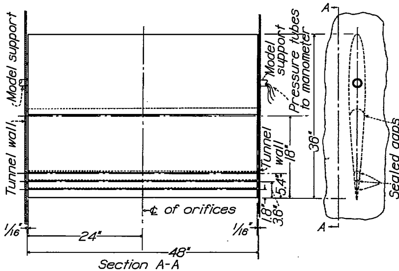
Figure 2.- The N.A.C.A. 0009 pressure-distribution model with 0.50c f plain flap and 0.10c f , 0.20c f , and 0.30c f tabs.
